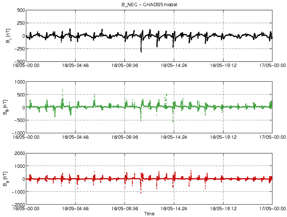
Figure 22 S/C C day 16/05 time series of B_{NEC} - B_{Chaos} residuals.
