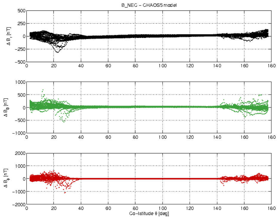
Figure 21 S/C C day 16/05 B_{NEC} - B_{Chaos} difference vs colatitude.
