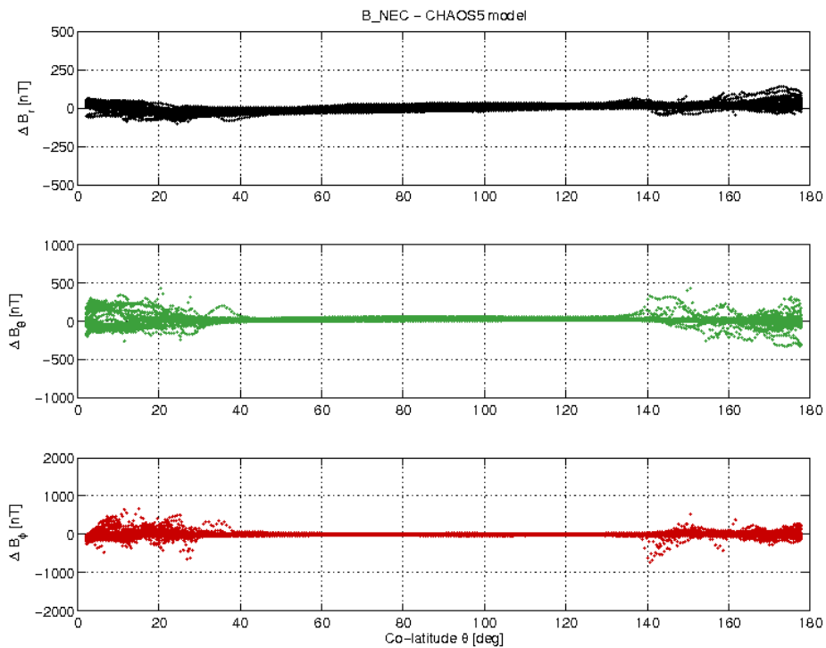
Figure 19: S/C B day 16/05 B_{NEC} - B_{Chaos} difference vs colatitude.
