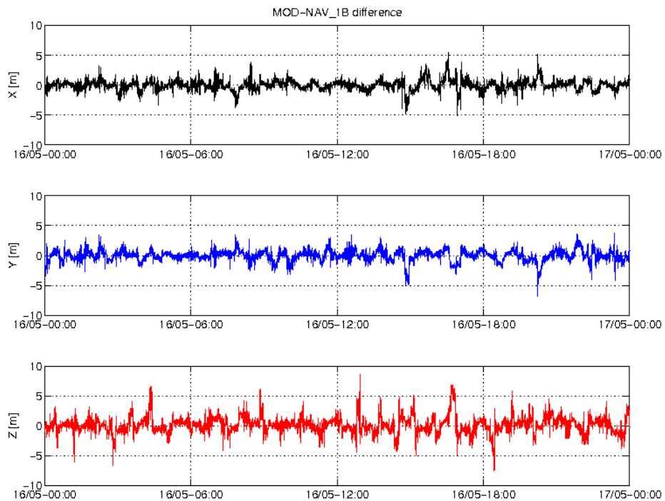
Figure 3: Difference MOD-GPSNAV, S/C A, 16/05. From top to bottom: X, Y and Z-axis
