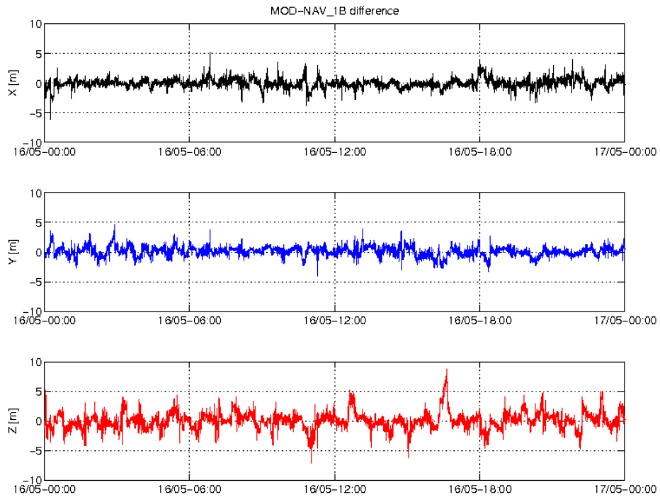
Figure 4: Difference MOD-GPSNAV, S/C B, 16/05. From top to bottom: X, Y and Z-axis
