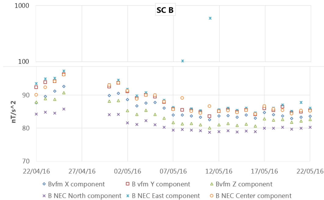
Figure 24: Plot of standard deviation of B components in VFM and NEC frames. Please note the mixed (linear + logarithmic) vertical axis (in range 100-1000 is given in logarithmic scale).
