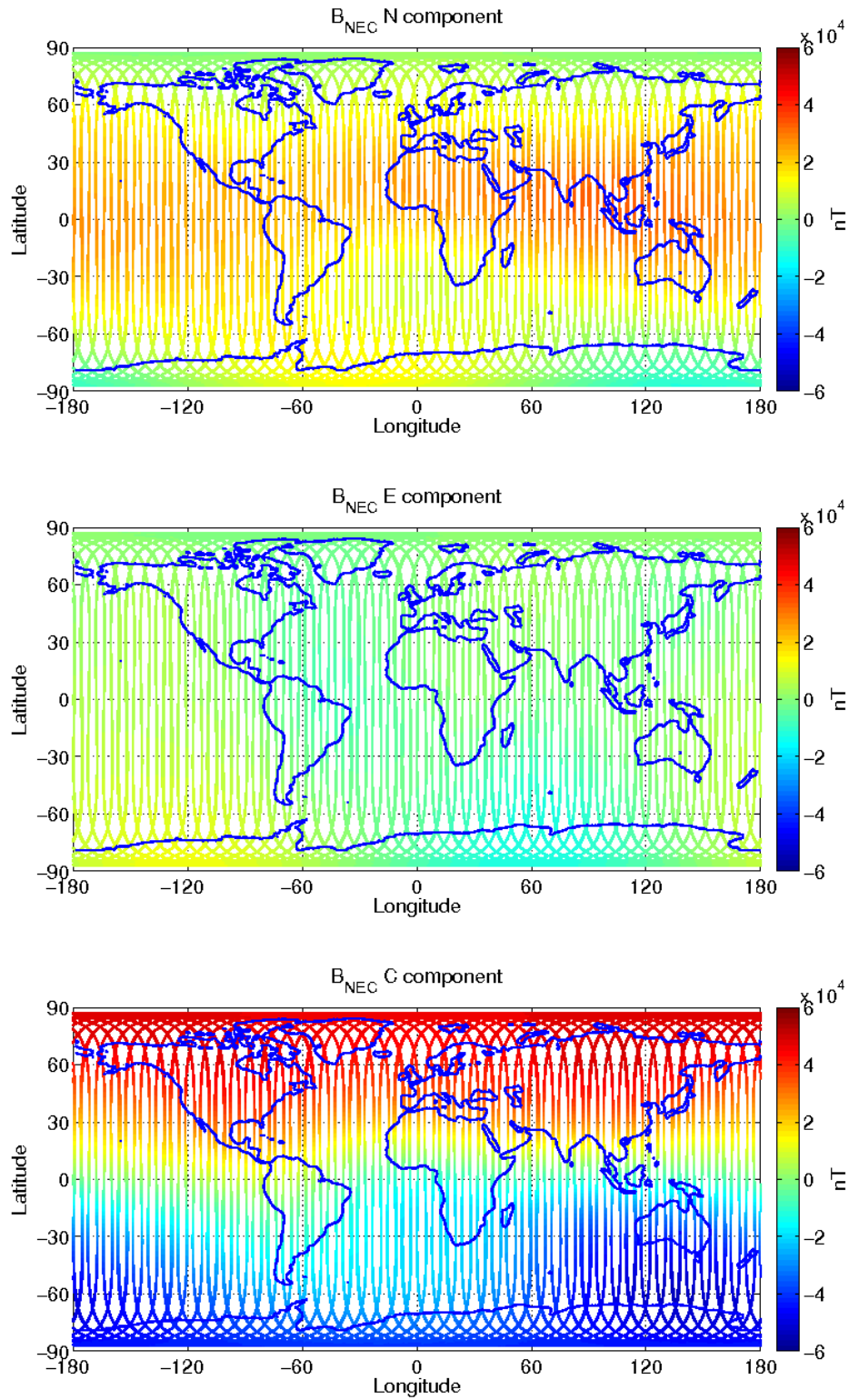
Figure 12: S/C C, world map plots of the geomagnetic field and components measured during monitoring period 16/05-22/05. From top to bottom: B_{NEC} components (North, East, and Centre) of magnetic field from VFM measurement.
