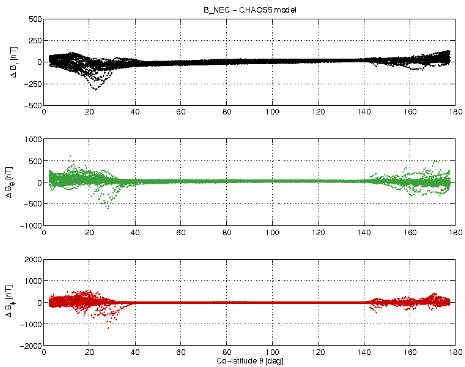
Figure 17: S/C A day 16/05 B_{NEC} - B_{Chaos} vs colatitude.
