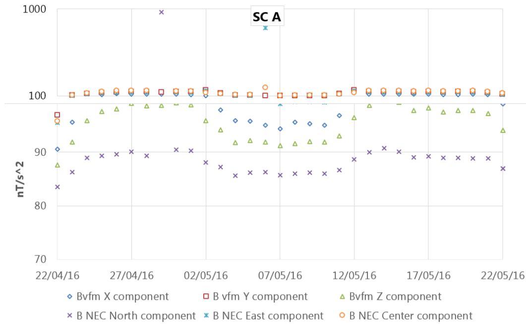
Figure 23: Plot of standard deviation of B components in VFM and NEC frames. Please note the mixed (linear + logarithmic) vertical axis (in range 100-1000 is given in logarithmic scale).
