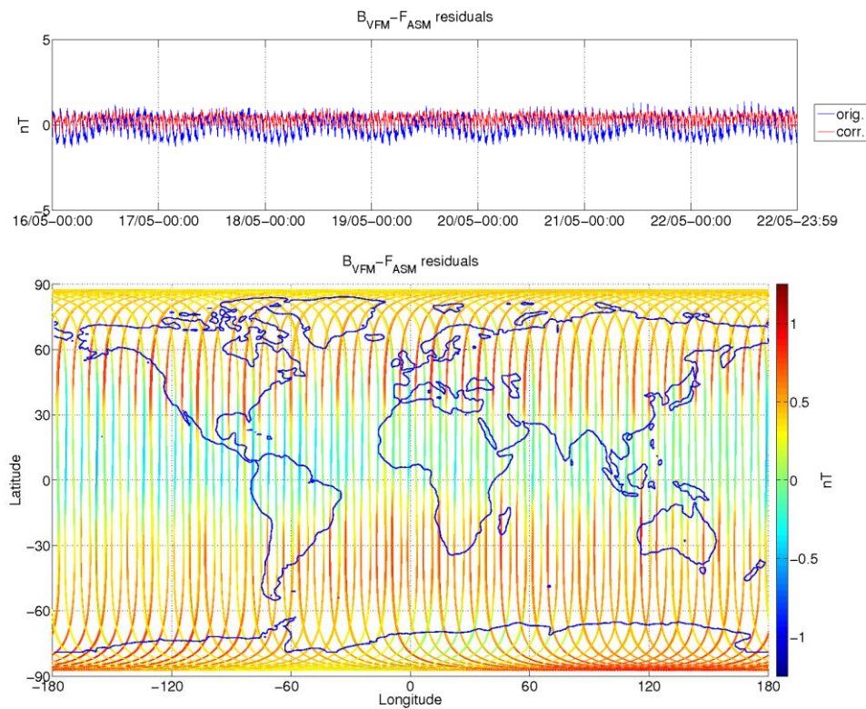
Figure 8: ASM-VFM residuals for S/C A, during monitoring period 16/05-22/05. In top figure are plotted: difference between |B_{VFM}| and F_{ASM} (without dB_{Sun} correction) (blue colour), and the residuals with dB_{Sun} corrections (red colour). In bottom figure residuals are presented on the world map.
