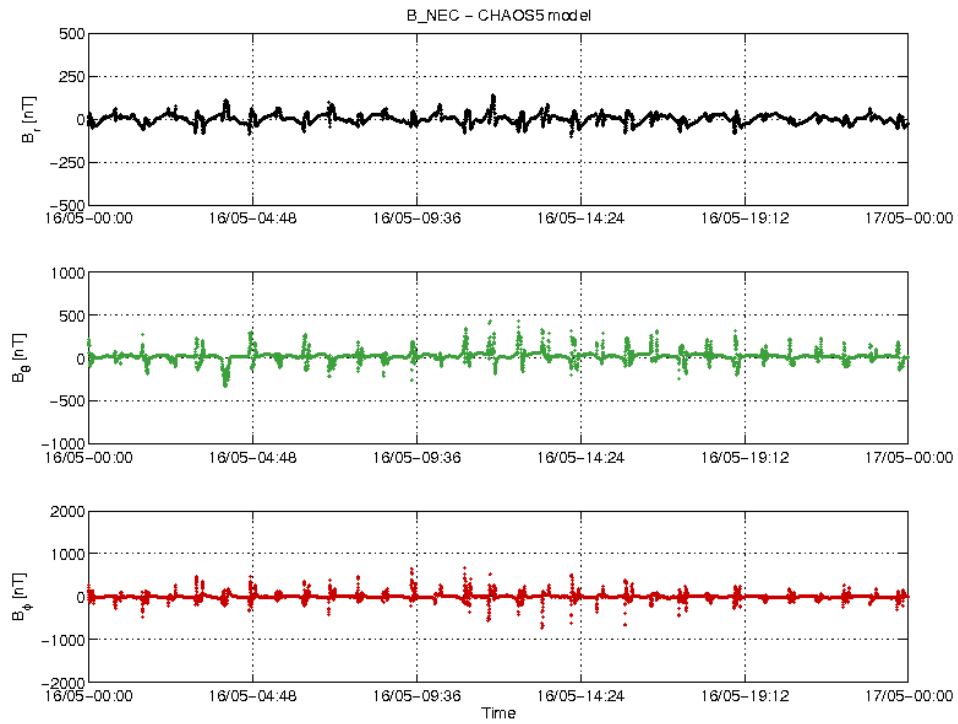
Figure 20 S/C B day 16/05 time series of B_{NEC} - B_{Chaos} residuals.
