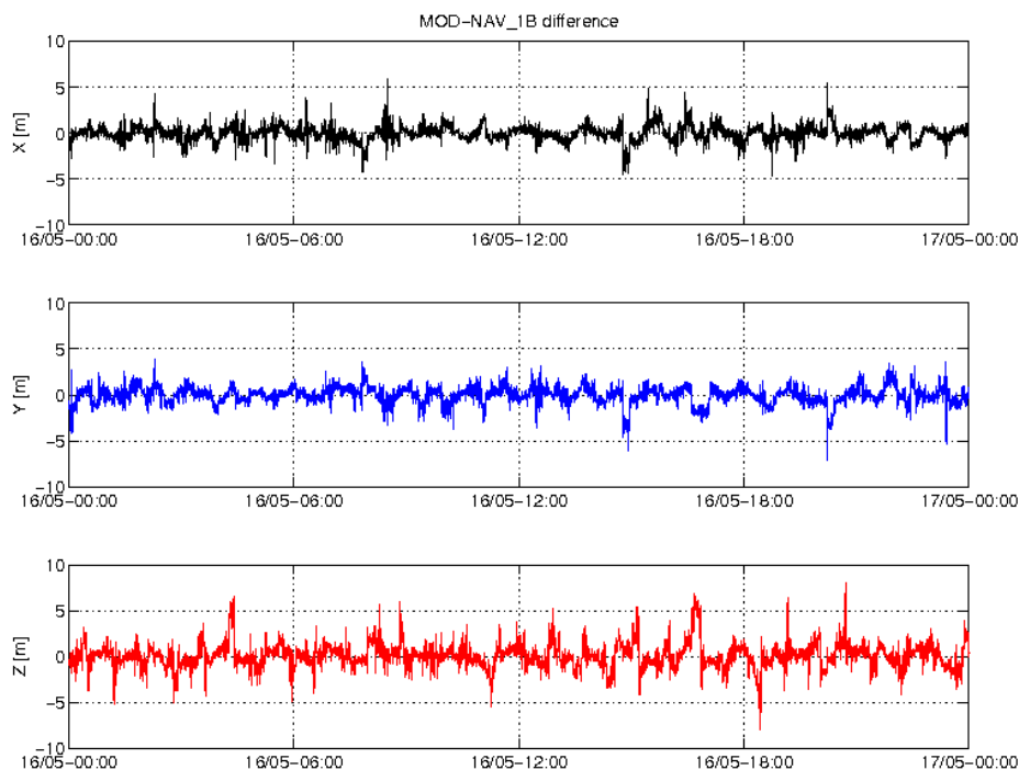
Figure 5: Difference MOD-GPSNAV, S/C C, 16/05. From top to bottom: X, Y and Z-axis
