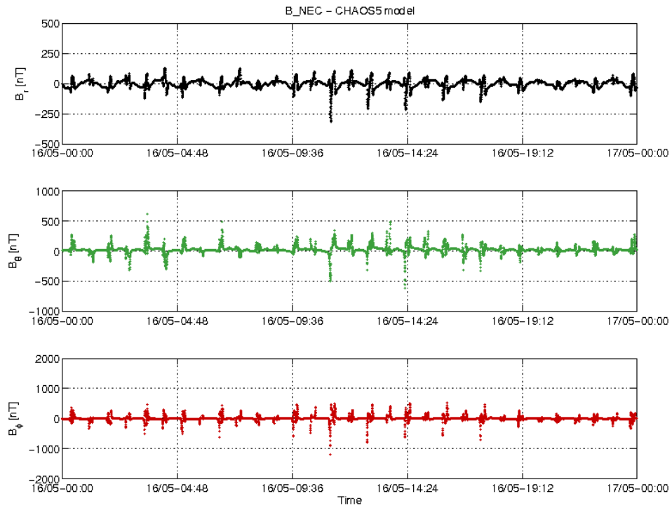
Figure 18: S/C A day 16/05: time series of B_{NEC} - B_{Chaos} residuals.
