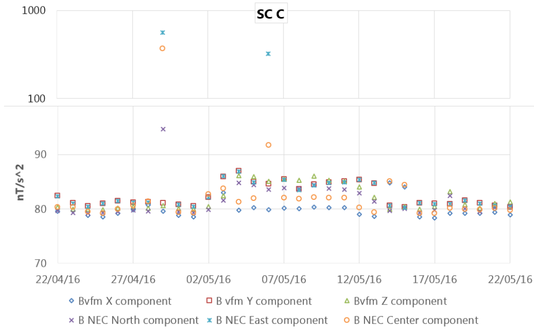
Figure 25: Plot of standard deviation of B components in VFM and NEC frames. Please note the mixed (linear + logarithmic) vertical axis (in range 100-1000 is given in logarithmic scale).
