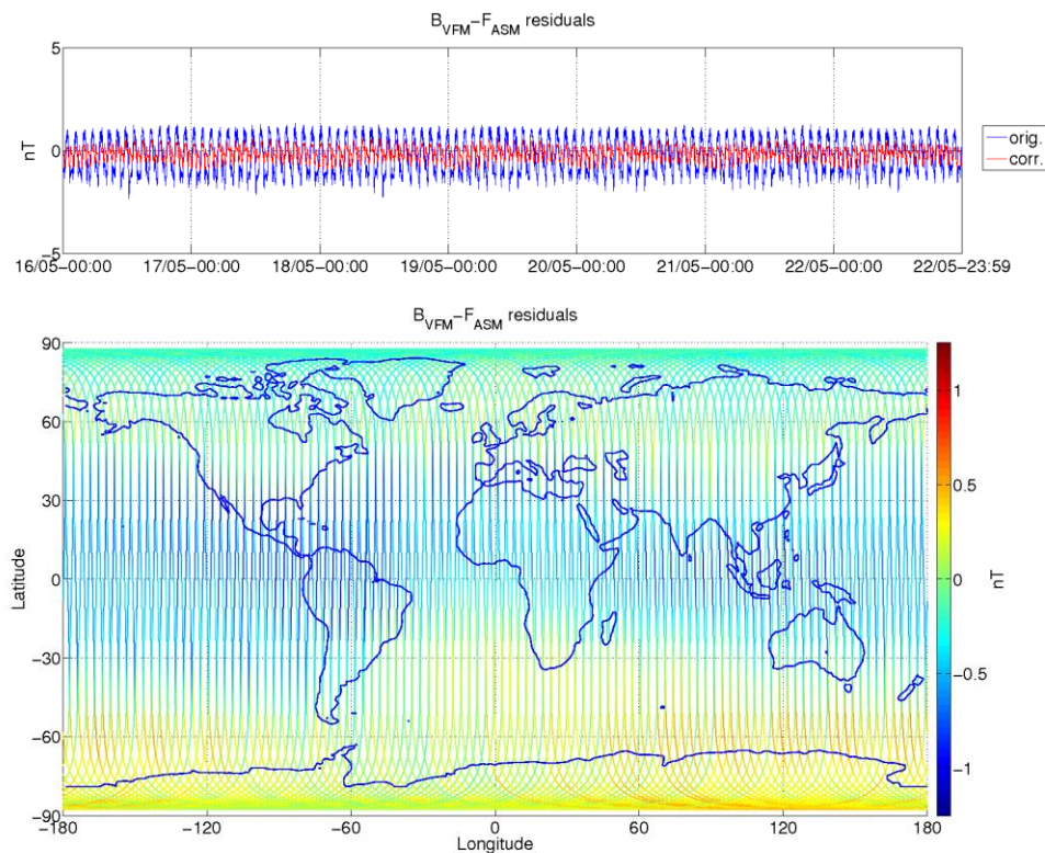
Figure 9: ASM-VFM residuals for S/C B, during monitoring period 16/05-22/05. In top figure are plotted: difference between |B_{VFM}| and F_{ASM} (without dB_{Sun} correction) (blue colour), and the residuals with dB_{Sun} corrections (red colour). In bottom figure residuals are presented on the world map.
