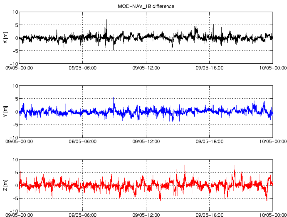
Figure 5: Difference MOD-GPSNAV, S/C C, 09/05. From top to bottom: X, Y and Z-axis
