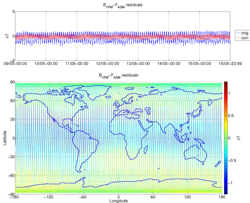
Figure 9: ASM-VFM residuals for S/C B, during monitoring period 09/05-15/05. In top figure are plotted: difference between |B_{VFM}| and F_{ASM} (without dB_Sun correction) (blue colour), and the residuals with dB_Sun corrections (red colour). In bottom figure residuals are presented on the world map.
