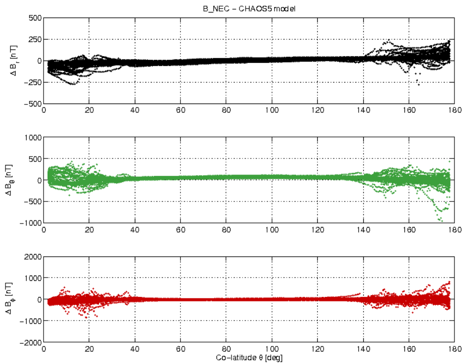
Figure 15: S/C B day 09/05 B_{NEC} - B_{Chaos} difference vs colatitude.
