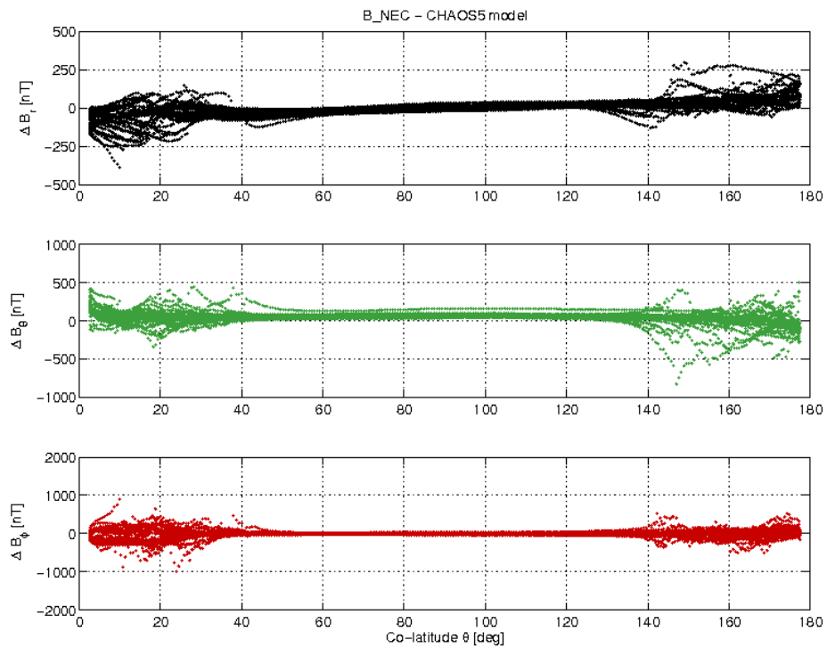
Figure 17 S/C C day 09/05 B_{NEC} - B_{Chaos} difference vs colatitude.
