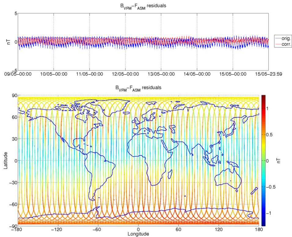
Figure 8: ASM-VFM residuals for S/C A, during monitoring period 09/05-15/05. In top figure are plotted: difference between |B VFM | and F ASM (without dB Sun correction) (blue colour), and the residuals with dB Sun corrections (red colour). In bottom figure residuals are presented on the world map.
