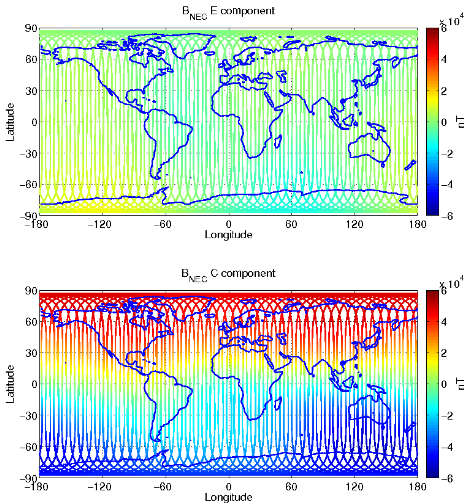
Figure 10: S/C A, world map plots of the geomagnetic field and components measured during monitoring period 09/05-15/05. From top to bottom: F-magnetic field from ASM measurement, B NEC components (North, East, and Centre) of magnetic field from VFM measurement.
