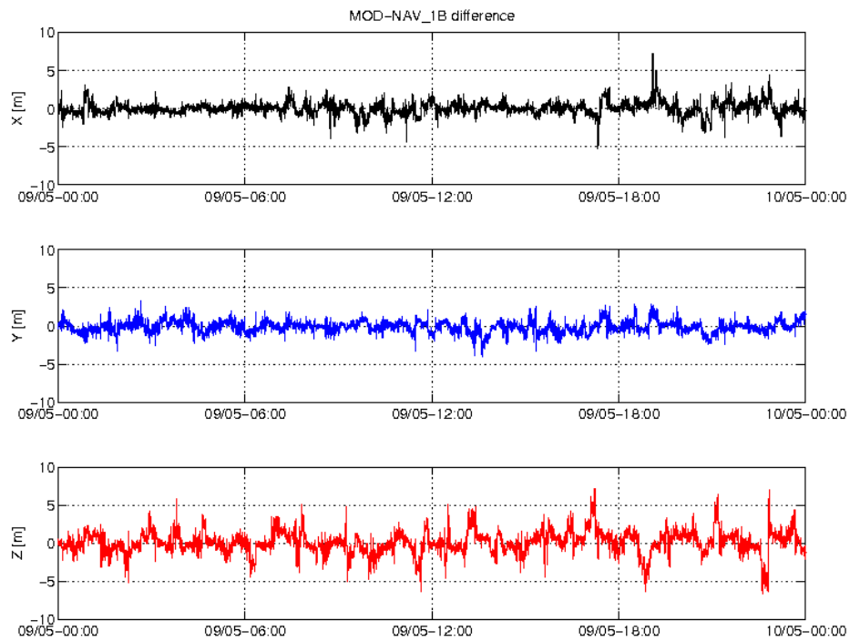
Figure 4: Difference MOD-GPSNAV, S/C B, 09/05. From top to bottom: X, Y and Z-axis
