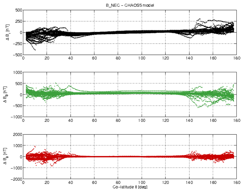
Figure 13: S/C A day 09/05 B_{NEC} - B_{Chaos} vs colatitude.
