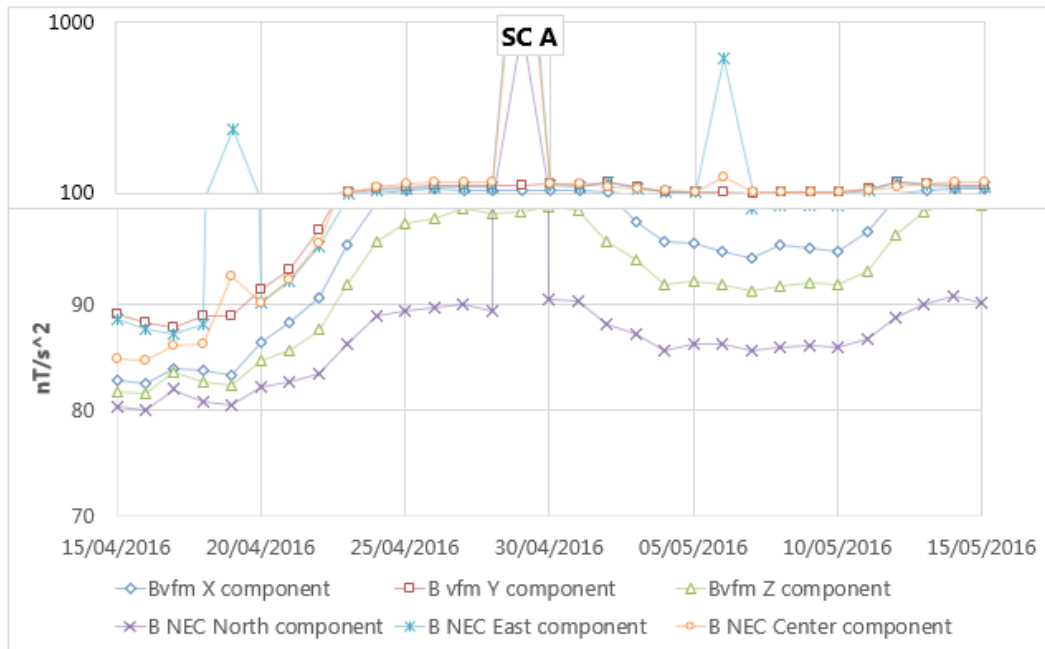
Figure 19: Plot of standard deviation of B components in VFM and NEC frames. Please note the mixed (linear + logarithmic) vertical axis (in range 100-1000 is given in logarithmic scale).
