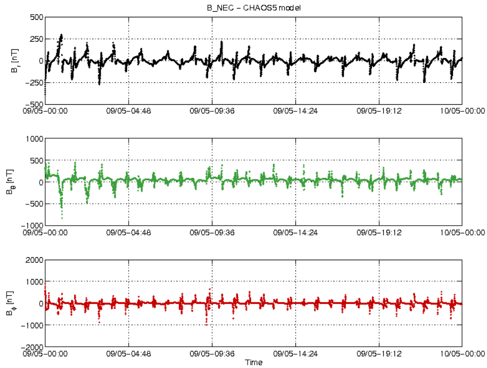
Figure 18 S/C C day 09/05 time series of B_{NEC} - B_{Chaos} residuals.
