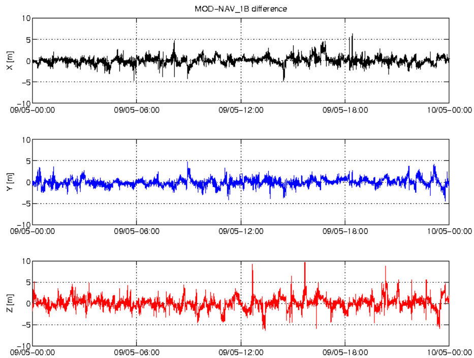
Figure 3: Difference MOD-GPSNAV, S/C A, 09/05. From top to bottom: X, Y and Z-axis
