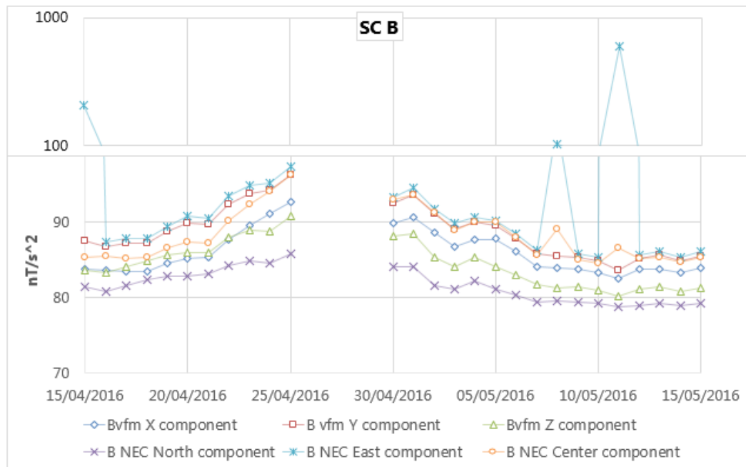
Figure 20: Plot of standard deviation of B components in VFM and NEC frames. Please note the mixed (linear + logarithmic) vertical axis (in range 100-1000 is given in logarithmic scale).
