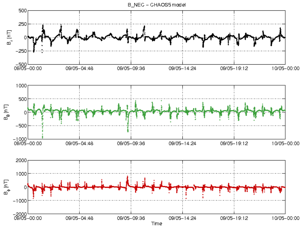
Figure 16 S/C B day 09/05 time series of B_{NEC} - B_{Chaos} residuals.
