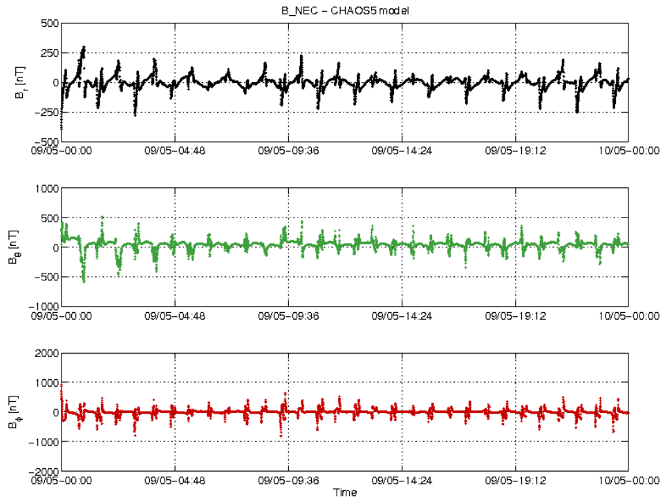
Figure 14: S/C A day 09/05: time series of B_{NEC} - B_{Chaos} residuals.
