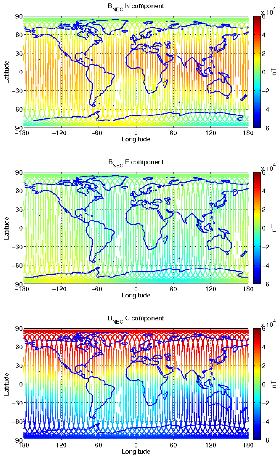
Figure 12: S/C C, world map plots of the geomagnetic field and components measured during monitoring period 09/05-15/05. From top to bottom: B_{NEC} components (North, East, and Centre) of magnetic field from VFM measurement.
