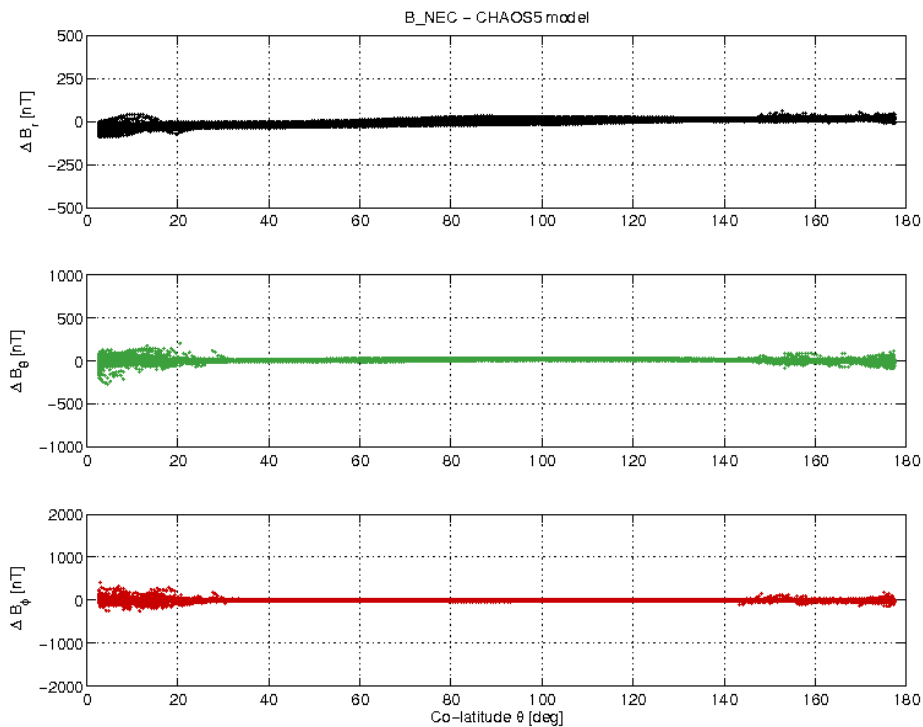
Figure 13: S/C A day 18/04 B_{NEC} - B_{Chaos} vs colatitude.
