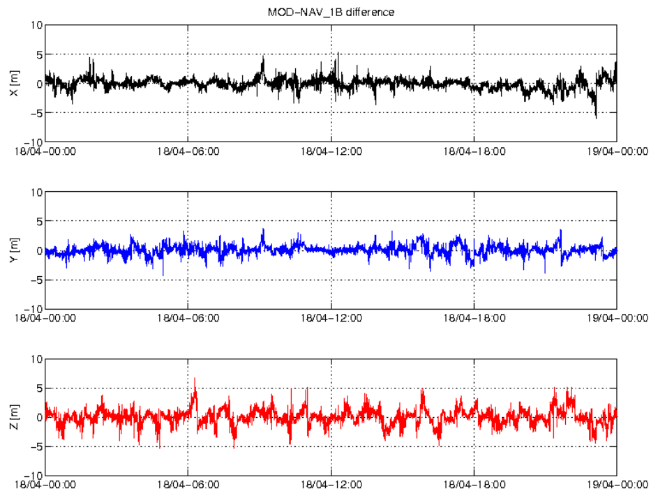
Figure 4: Difference MOD-GPSNAV, S/C B, 18/04. From top to bottom: X, Y and Z-axis
