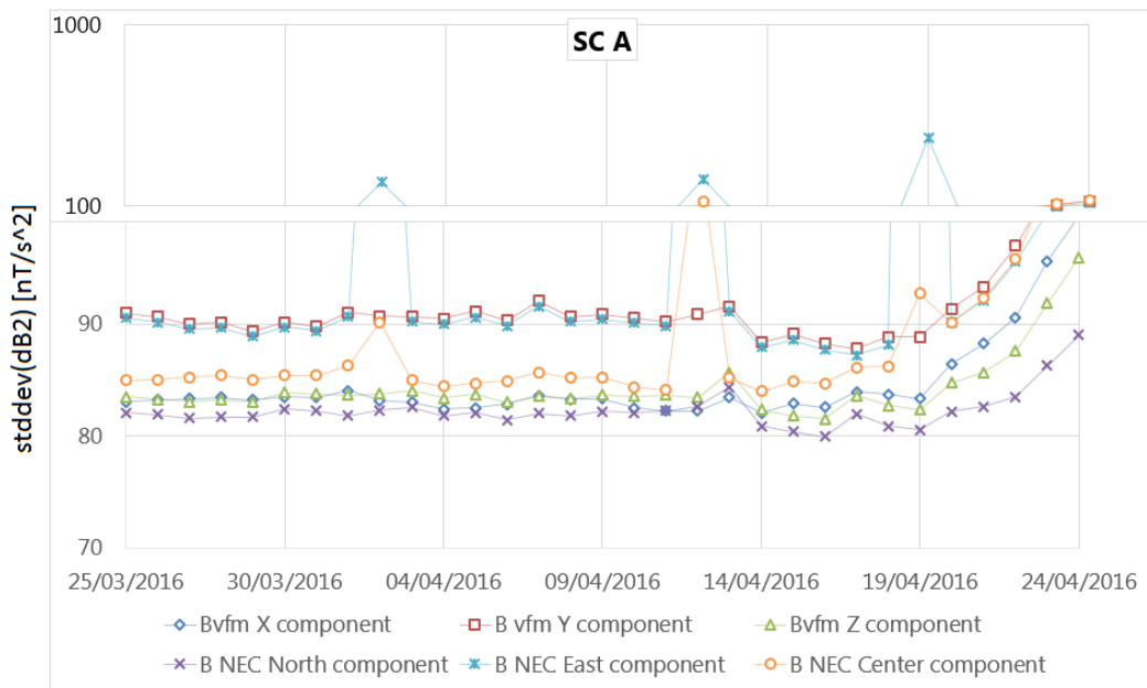
Figure 19: Plot of standard deviation of second derivatives of B components in VFM and NEC frames. Please note the mixed (linear + logarithmic) vertical axis (in range 100-1000 is given in logarithmic scale). The most disturbed components are East in NEC frame and Y in VFM frame.
