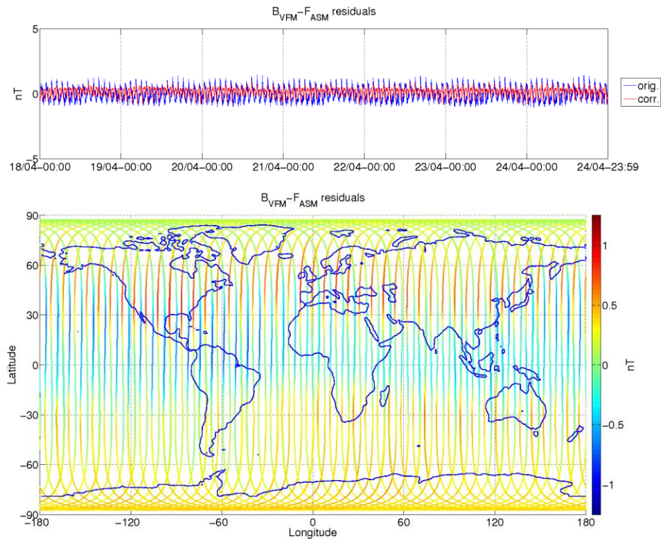
Figure 8: ASM-VFM residuals for S/C A, during monitoring period 18/04-24/04. In top figure are plotted: difference between |B_{VFM}| and F_{ASM} (without dB_{Sun} correction) (blue colour), and the residuals with dB_{Sun} corrections (red colour). In bottom figure residuals are presented on the world map.
