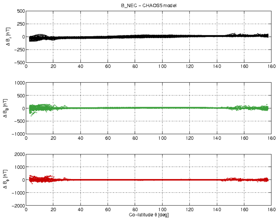
Figure 17: S/C C day 18/04 B_{NEC} - B_{Chaos} difference vs colatitude.
