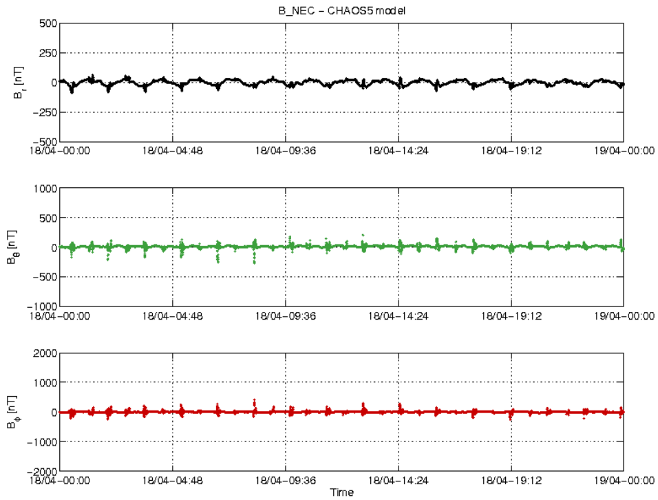
Figure 14: S/C A day 18/04: time series of B_{NEC} - B_{Chaos} residuals.
