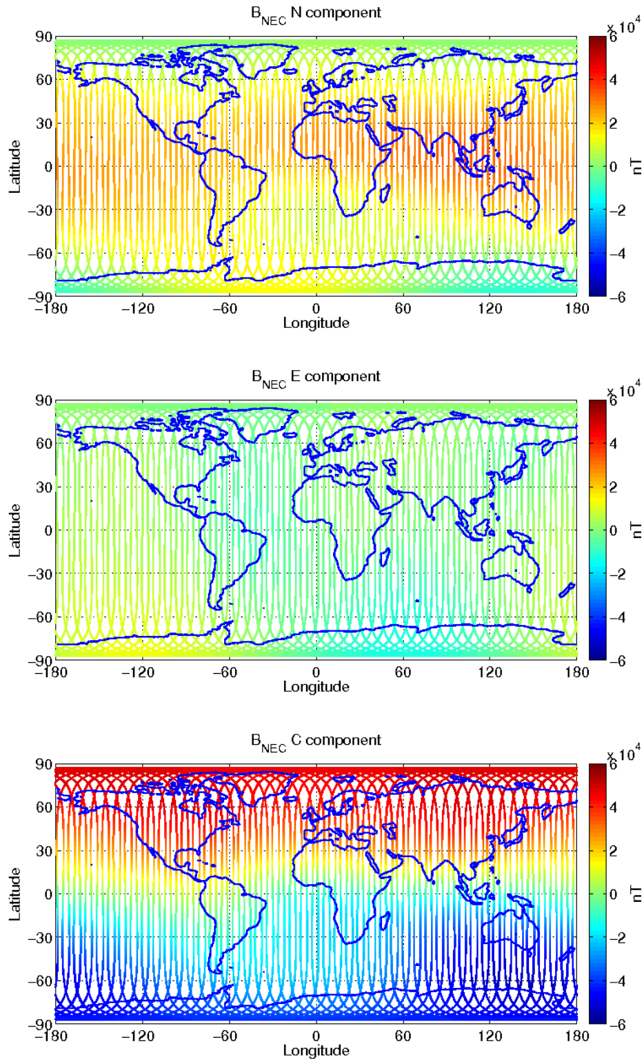
Figure 12: S/C C, world map plots of the geomagnetic field and components measured during monitoring period 18/04-24/04. From top to bottom: B_{NEC} components (North, East, and Centre) of magnetic field from VFM measurement.
