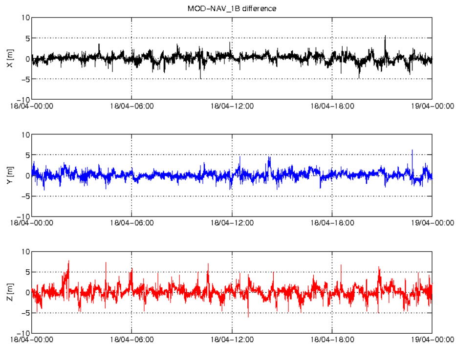
Figure 3: Difference MOD-GPSNAV, S/C A, 18/04. From top to bottom: X, Y and Z-axis
