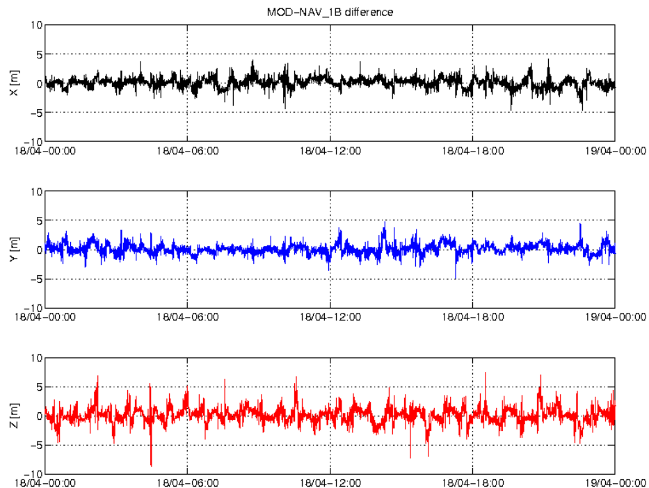
Figure 5: Difference MOD-GPSNAV, S/C C, 18/04. From top to bottom: X, Y and Z-axis
