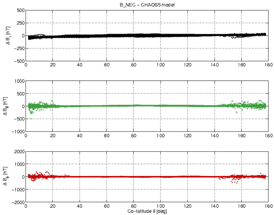
Figure 15: S/C B day 18/04 B_{NEC} - B_{Chaos} difference vs colatitude.
