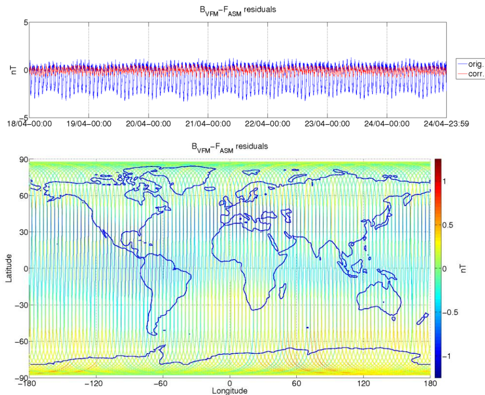
Figure 9: ASM-VFM residuals for S/C B, during monitoring period 18/04-24/04. In top figure are plotted: difference between |B_{VFM}| and F_{ASM} (without dB_Sun correction) (blue colour), and the residuals with dB_Sun corrections (red colour). In bottom figure residuals are presented on the world map.
