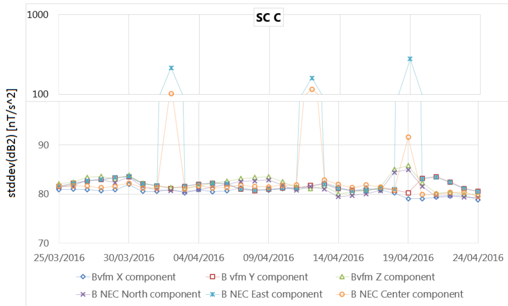
Figure 21: Plot of standard deviation of second derivatives of B components in VFM and NEC frames. Please note the mixed (linear + logarithmic) vertical axis (in range 100-1000 is given in logarithmic scale).
