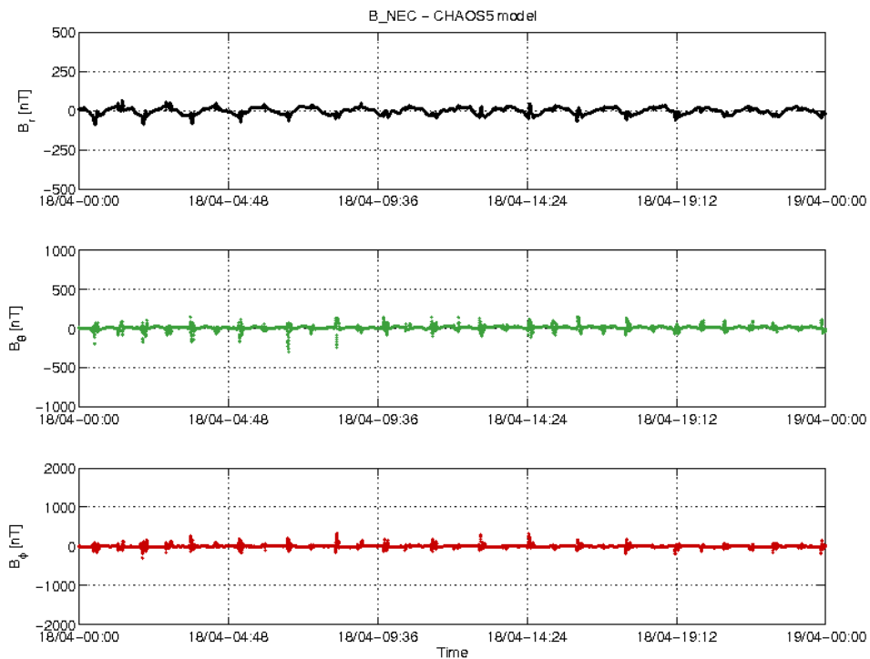
Figure 18: S/C C day 18/04 time series of B_{NEC} - B_{Chaos} residuals.
