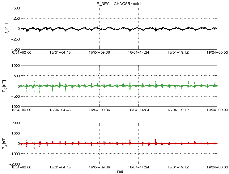
Figure 16: S/C B day 18/04 time series of B_{NEC} - B_{Chaos} residuals.
