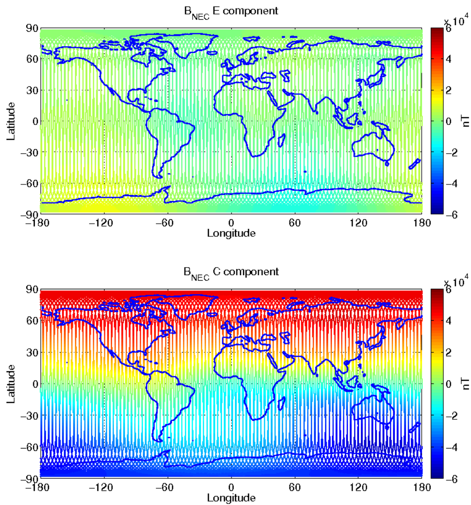
Figure 11: S/C B, world map plots of the geomagnetic field and components measured during monitoring period 18/04-24/04. From top to bottom: F-magnetic field from ASM measurement, B NEC components (North, East, and Centre) of magnetic field from VFM measurement.
