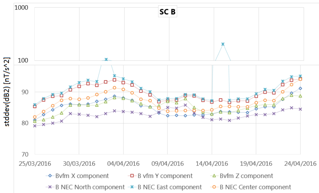
Figure 20: Plot of standard deviation of second derivatives of B components in VFM and NEC frames. Please note the mixed (linear + logarithmic) vertical axis (in range 100-1000 is given in logarithmic scale). The most disturbed components are East in NEC frame and Y in VFM frame.
