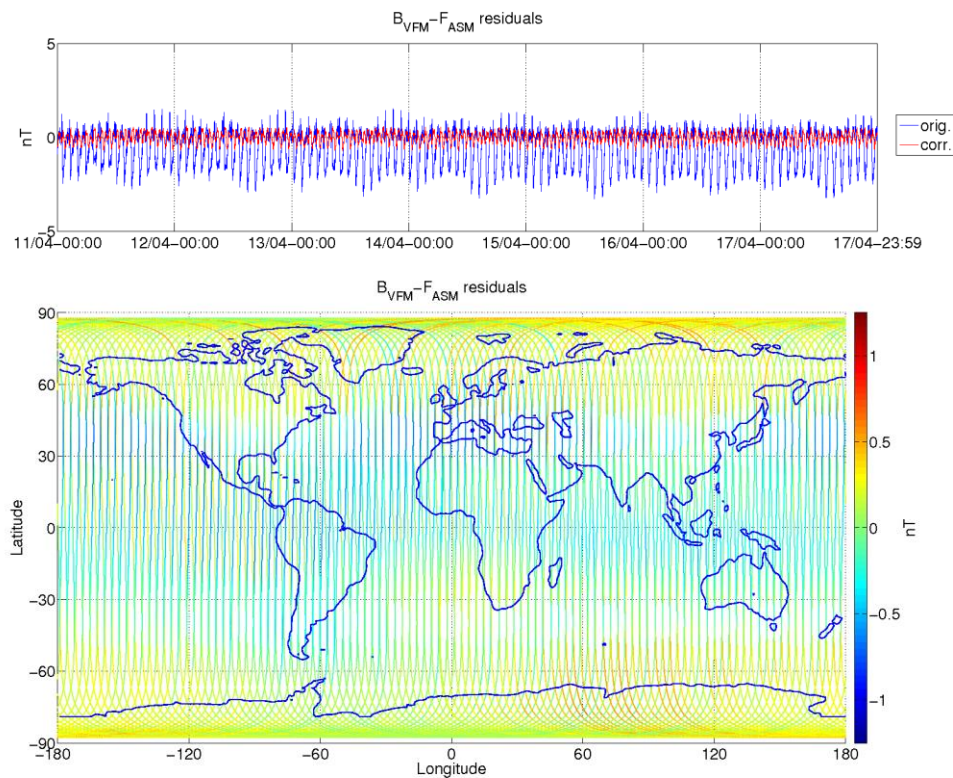
Figure 9: ASM-VFM residuals for S/C B, during monitoring period 11/04-17/04. In top figure are plotted: difference between |B_{VFM}| and F_{ASM} (without dB_{Sun} correction) (blue colour), and the residuals with dB_{Sun} corrections (red colour). In bottom figure residuals are presented on the world map.
