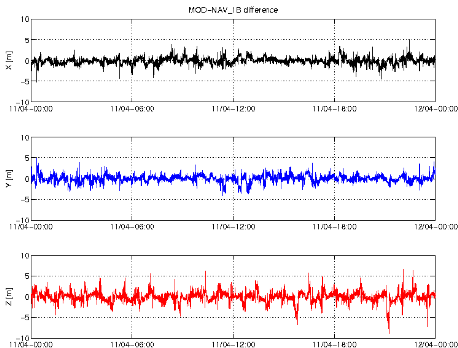
Figure 5: Difference MOD-GPSNAV, S/C C, 11/04. From top to bottom: X, Y and Z-axis
