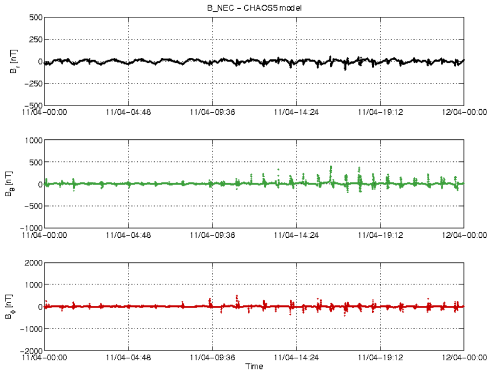
Figure 18: S/C C day 11/04 time series of B_{NEC} - B_{Chaos} residuals.
