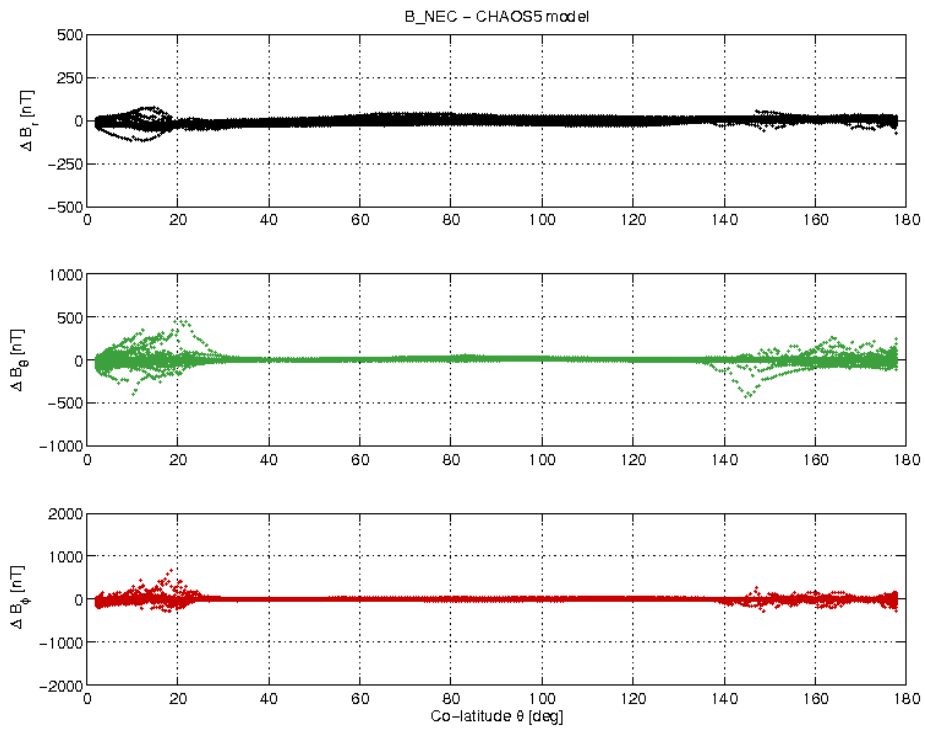
Figure 15: S/C B day 11/04 B_{NEC} - B_{Chaos} difference vs colatitude.
