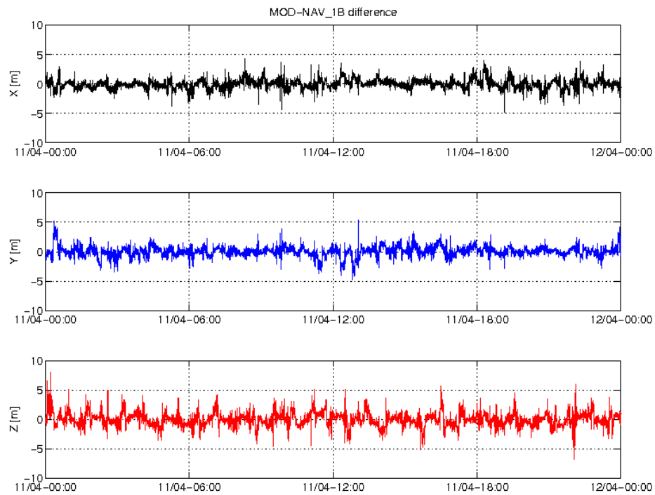
Figure 3: Difference MOD-GPSNAV, S/C A, 11/04. From top to bottom: X, Y and Z-axis
