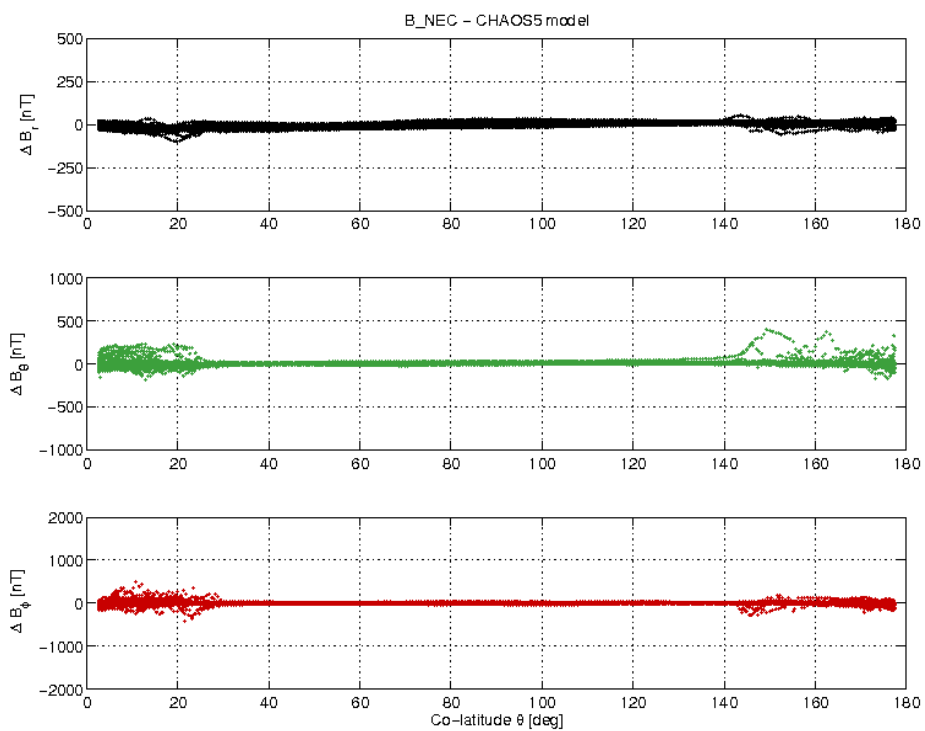
Figure 17: S/C C day 11/04 B_{NEC} - B_{Chaos} difference vs colatitude.
