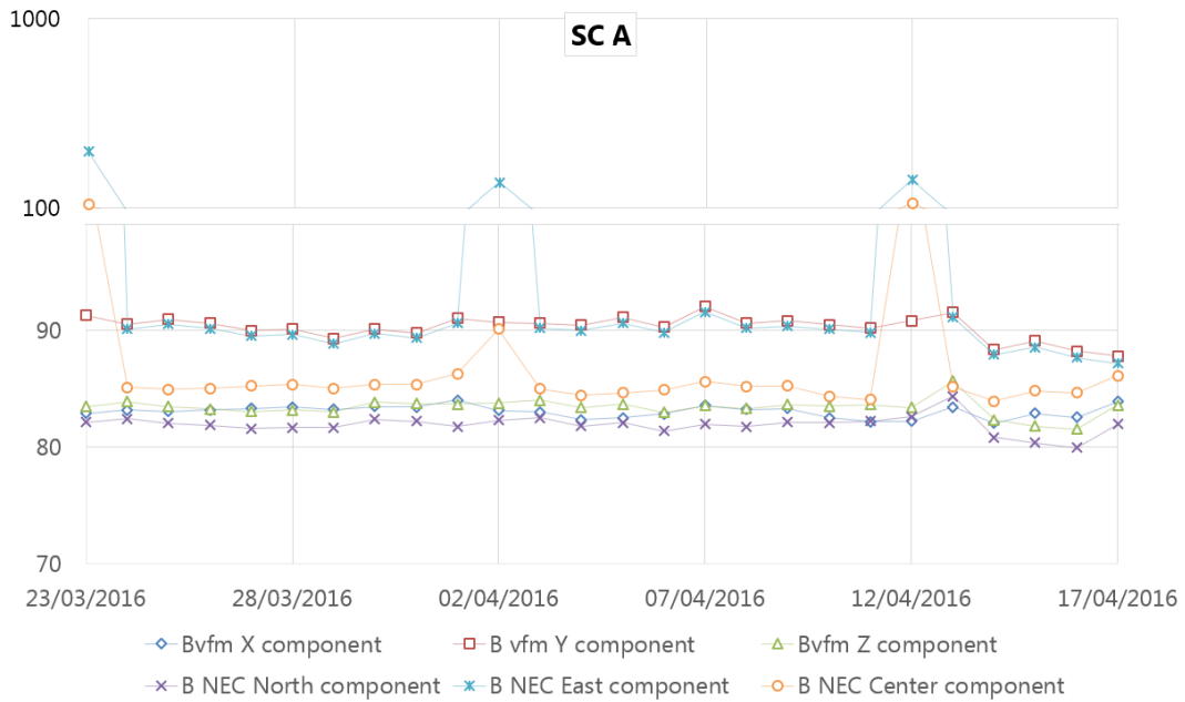
Figure 19: Plot of standard deviation of B components in VFM and NEC frames. Please note the mixed (linear + logarithmic) vertical axis (in range 100-1000 the scale is logarithmic). The most disturbed components are East in NEC frame and Y in VFM frame.
