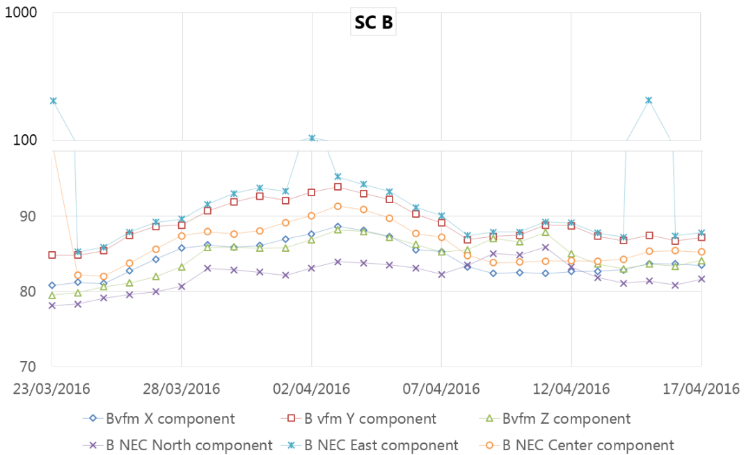
Figure 20: Plot of standard deviation of B components in VFM and NEC frames. Please note the mixed (linear + logarithmic) vertical axis (in range 100-1000 the scale is logarithmic). The most disturbed components are East in NEC frame and Y in VFM frame.
