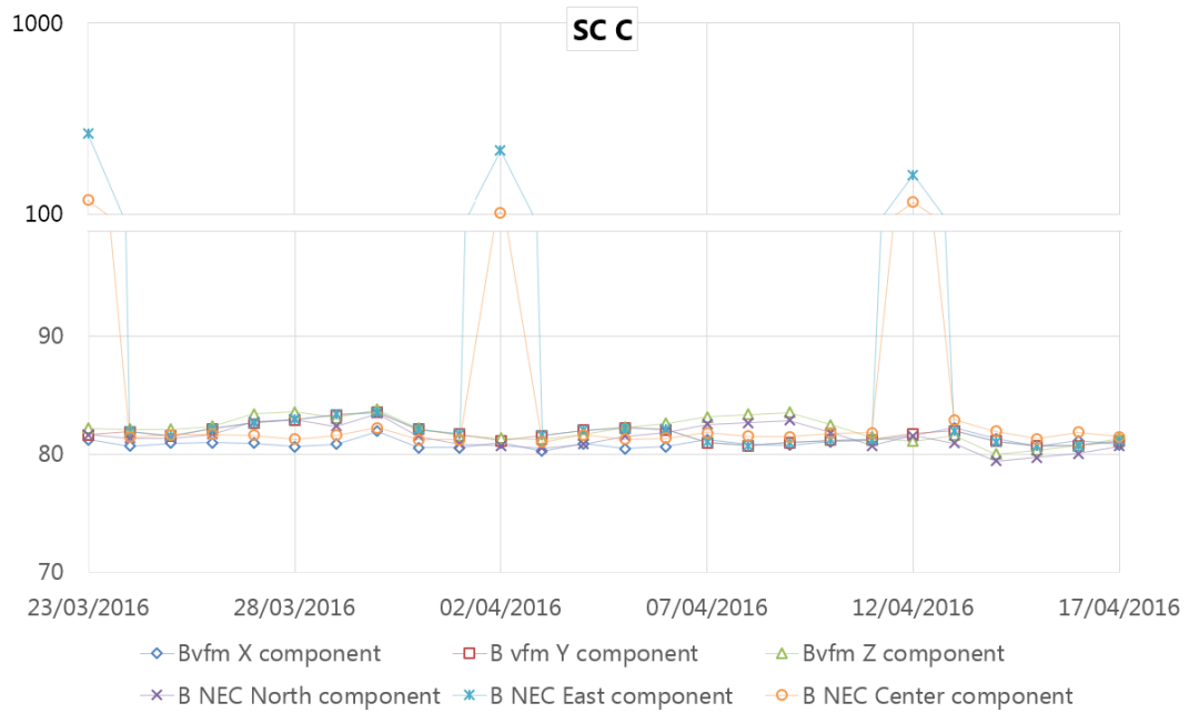
Figure 21: Plot of standard deviation of B components in VFM and NEC frames. Please note the mixed (linear + logarithmic) vertical axis (in range 100-1000 the scale is logarithmic).
