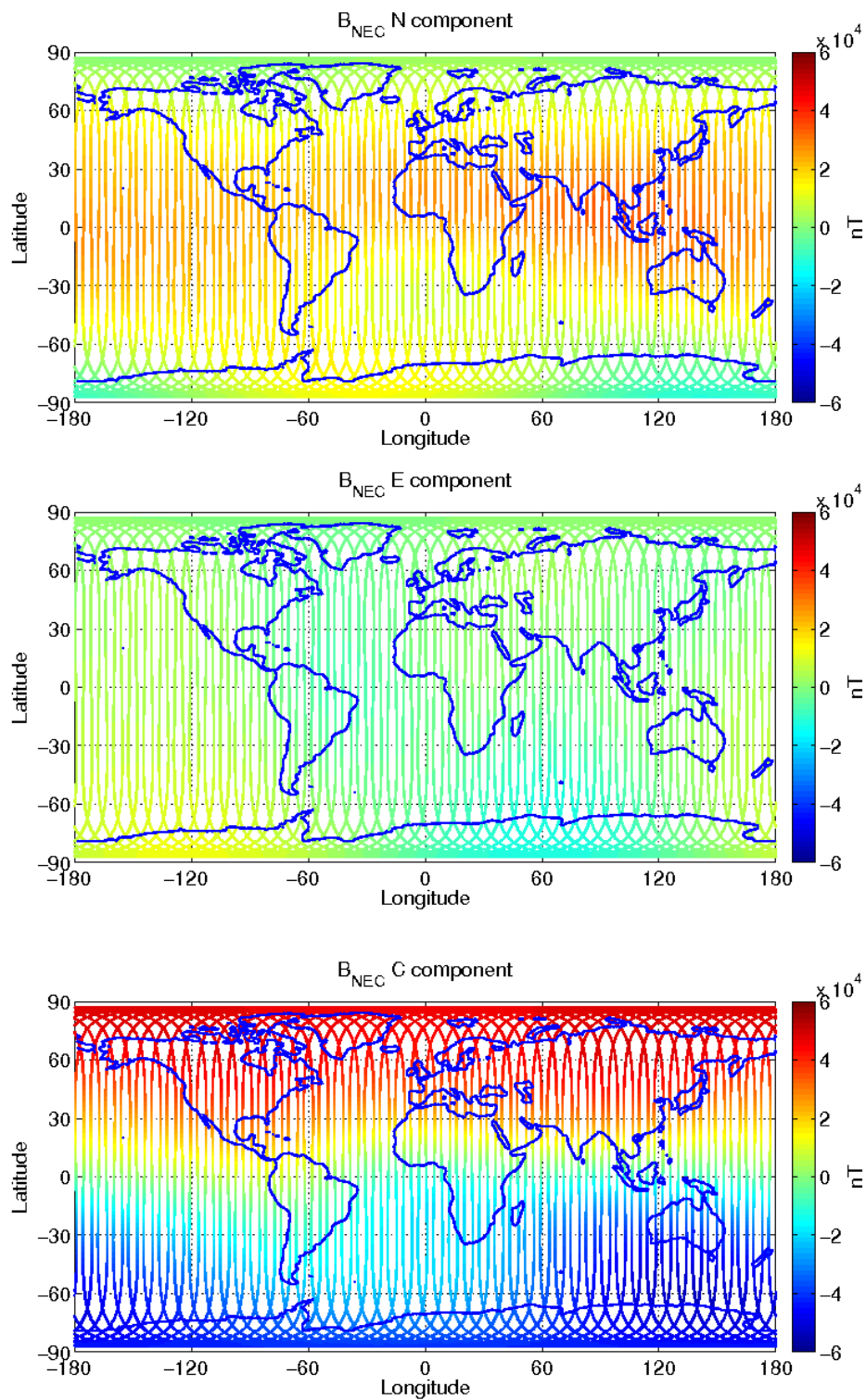
Figure 12: S/C C, world map plots of the geomagnetic field and components measured during monitoring period 11/04-17/04. From top to bottom: B_{NEC} components (North, East, and Centre) of magnetic field from VFM measurement.
