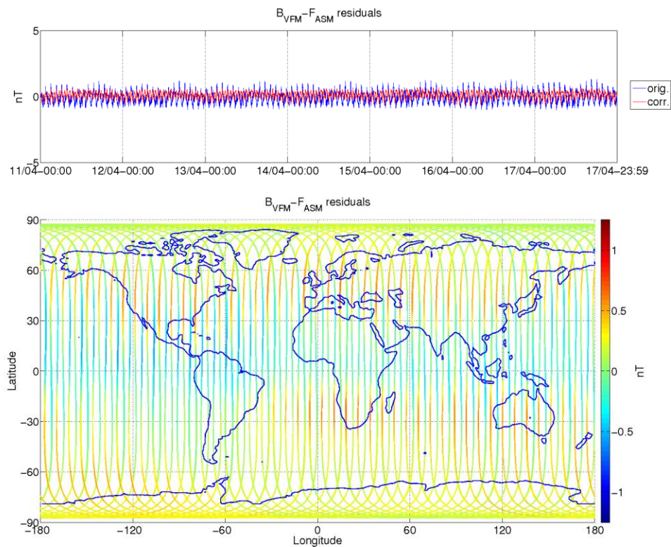
Figure 8: ASM-VFM residuals for S/C A, during monitoring period 11/04-17/04. In top figure are plotted: difference between |B_{VFM}| and F_{ASM} (without dB Sun correction) (blue colour), and the residuals with dB Sun corrections (red colour). In bottom figure residuals are presented on the world map.
