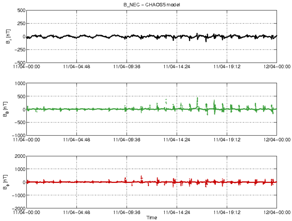
Figure 14: S/C A day 11/04: time series of B_{NEC} - B_{Chaos} residuals.
