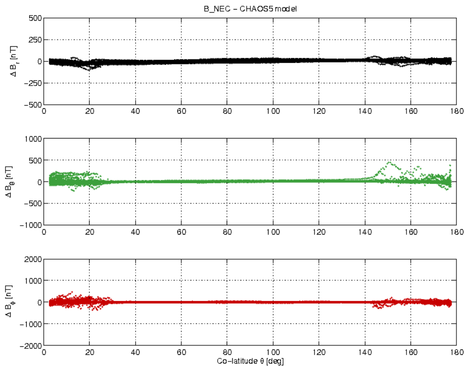
Figure 13: S/C A day 11/04 B_{NEC} - B_{Chaos} vs colatitude.
