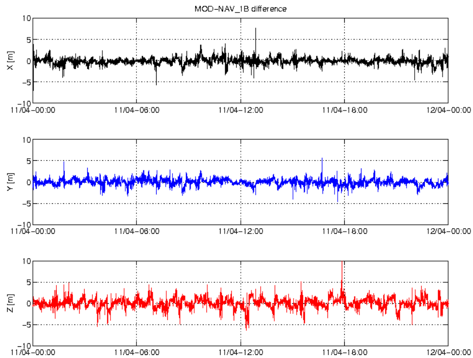
Figure 4: Difference MOD-GPSNAV, S/C B, 11/04. From top to bottom: X, Y and Z-axis
