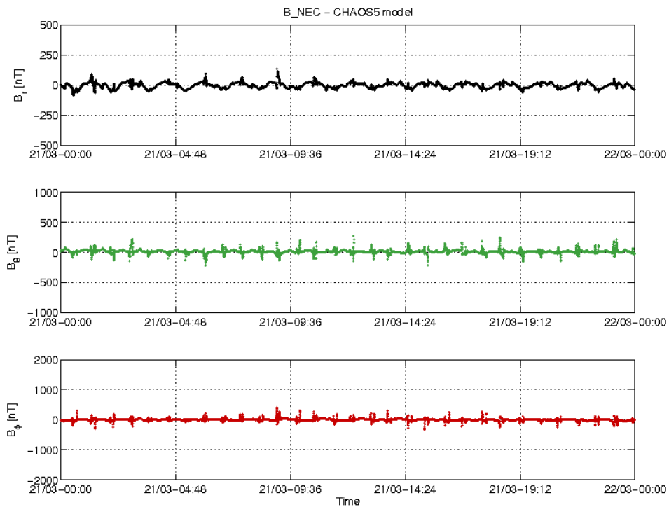
Figure 18: Swarm C day 21/03 time series of B_{NEC} - B_{Chaos} residuals.
