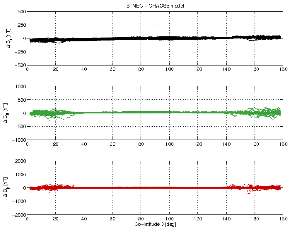
Figure 15: Swarm B day 21/03 B_{NEC} - B_{Chaos} difference vs colatitude.
