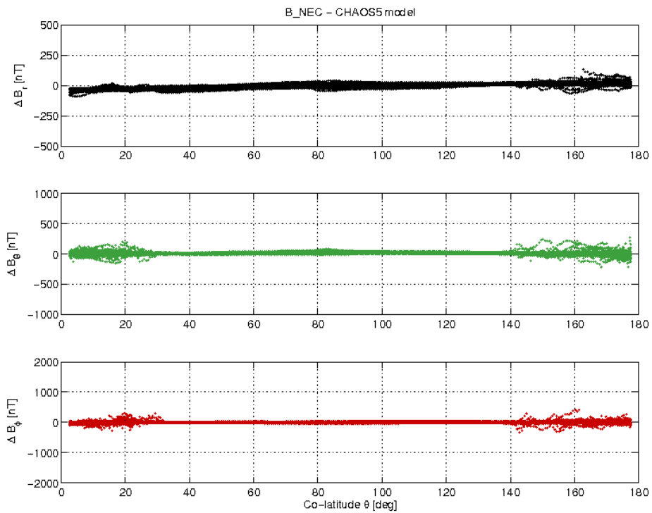
Figure 17: Swarm C day 21/03 B_{NEC} - B_{Chaos} difference vs colatitude.
