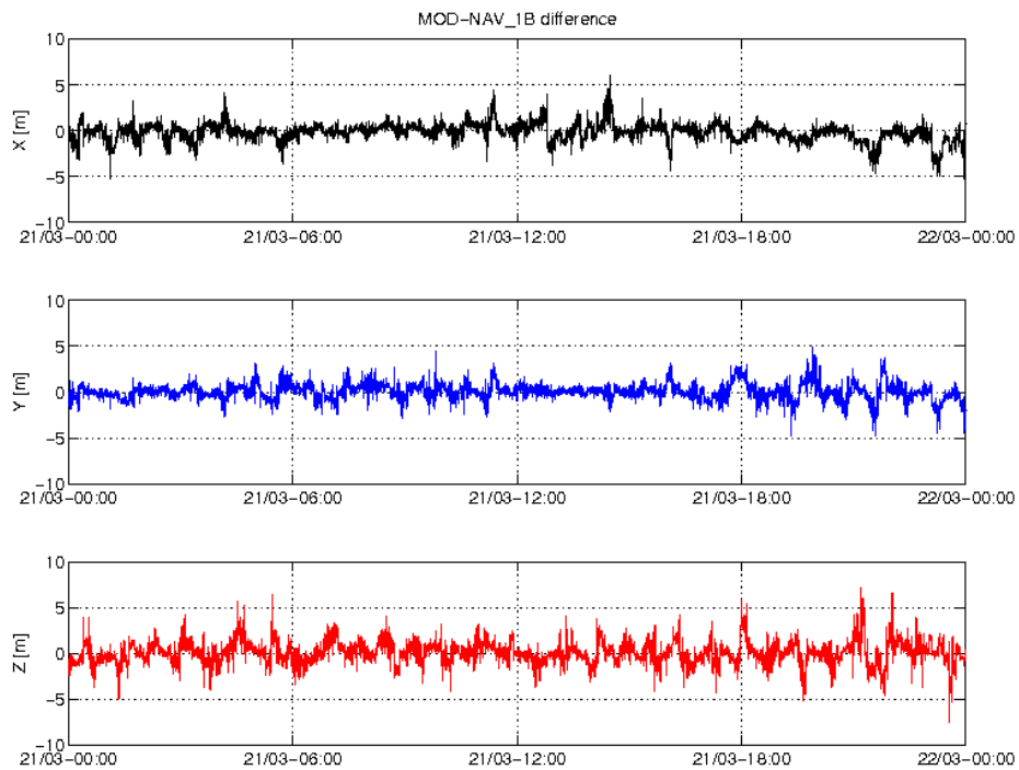
Figure 4: Difference MOD-GPSNAV, S/C B, 21/03. From top to bottom: X, Y and Z-axis
