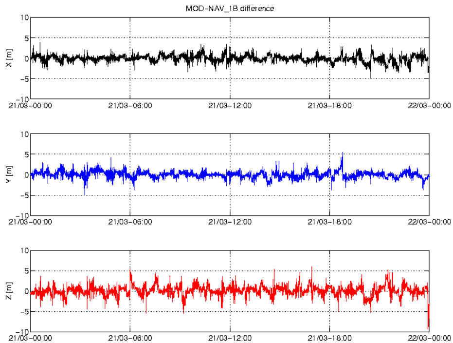
Figure 5: Difference MOD-GPSNAV, S/C C, 21/03. From top to bottom: X, Y and Z-axis
