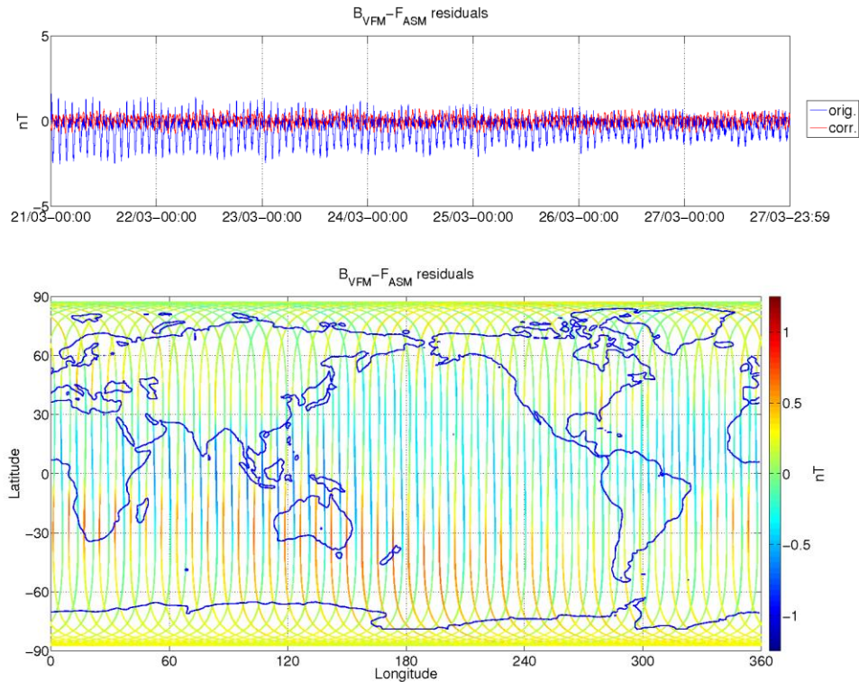
Figure 8: ASM-VFM residuals for S/C A, during monitoring period 21/03-27/03. In top figure are plotted: difference between |B_{VFM}| and F_{ASM} (without dB Sun correction) (blue colour), and the residuals with dB Sun corrections (red colour). In bottom figure residuals are presented on the world map.
