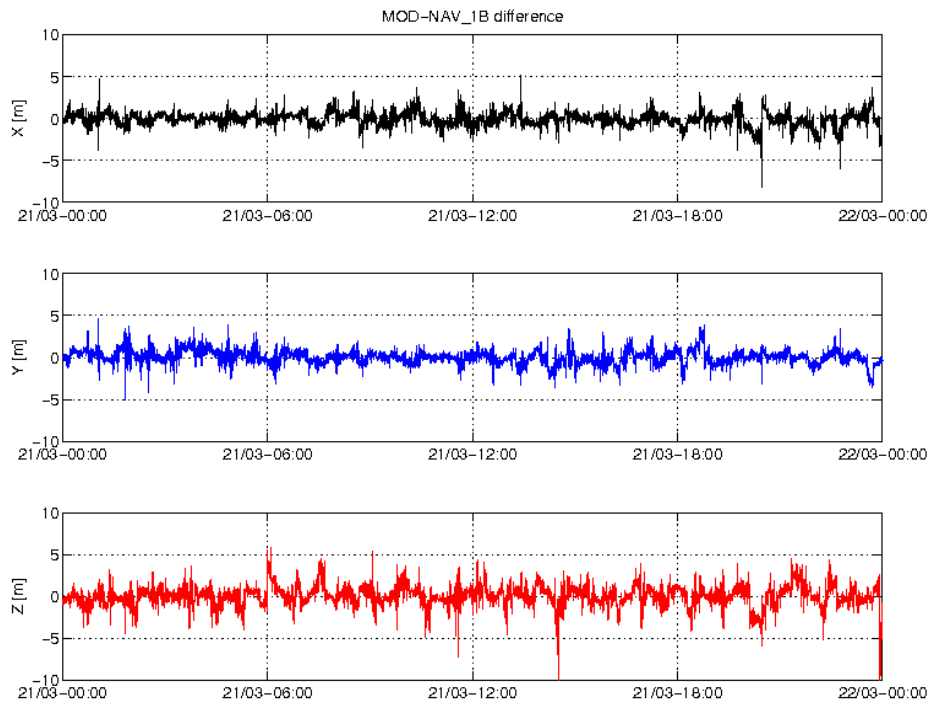
Figure 3: Difference MOD-GPSNAV, S/C A, 21/03. From top to bottom: X, Y and Z-axis
