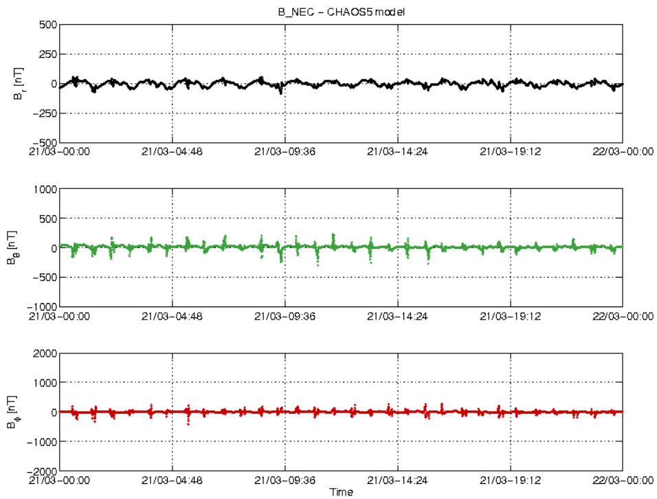
Figure 16: Swarm B day 21/03 time series of B_{NEC} - B_{Chaos} residuals.
