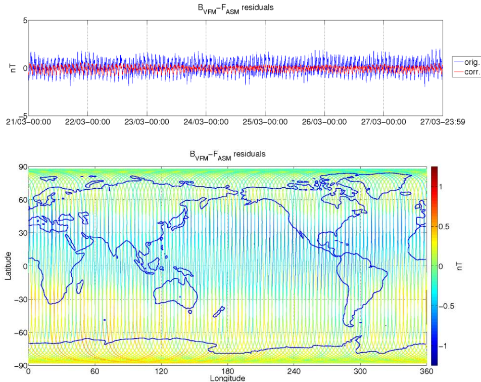
Figure 9: ASM-VFM residuals for S/C B, during monitoring period 21/03-27/03. In top figure are plotted: difference between |B\_VFM| and F\_ASM (without dB_Sun correction) (blue colour), and the residuals with dB_Sun corrections (red colour). In bottom figure residuals are presented on the world map.
