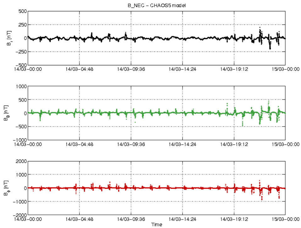
Figure 16: Swarm B day 14/03 time series of B_{NEC} - B_{Chaos} residuals.
