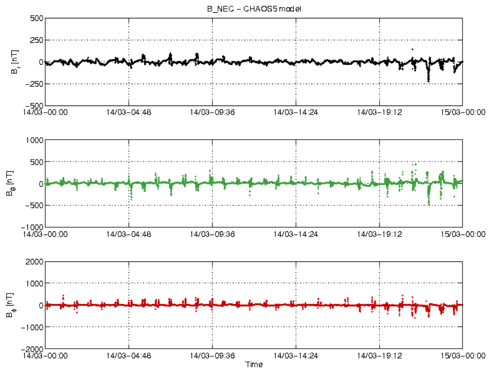
Figure 18: Swarm C day 14/03 time series of B_{NEC} - B_{Chaos} residuals.
