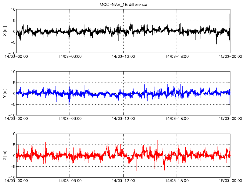
Figure 5: Difference MOD-GPSNAV, S/C C, 14/03. From top to bottom: X, Y and Z-axis
