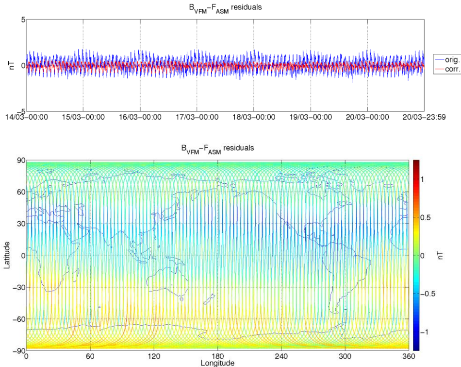
Figure 9: ASM-VFM residuals for S/C B, during monitoring period 14/03-20/03. In top figure are plotted: difference between |B_{VFM}| and F_{ASM} (without dB Sun correction) (blue colour), and the residuals with dB Sun corrections (red colour). In bottom figure residuals are presented on the world map.
