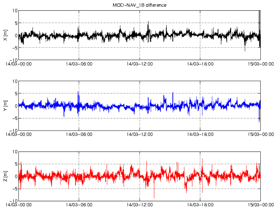
Figure 3: Difference MOD-GPSNAV, S/C A, 14/03. From top to bottom: X, Y and Z-axis
