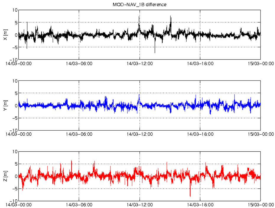
Figure 4: Difference MOD-GPSNAV, S/C B, 14/03. From top to bottom: X, Y and Z-axis
