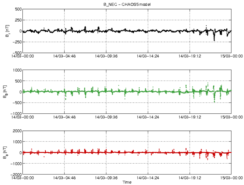
Figure 14: Swarm A day 14/03: time series of B_{NEC} - B_{Chaos} residuals.
