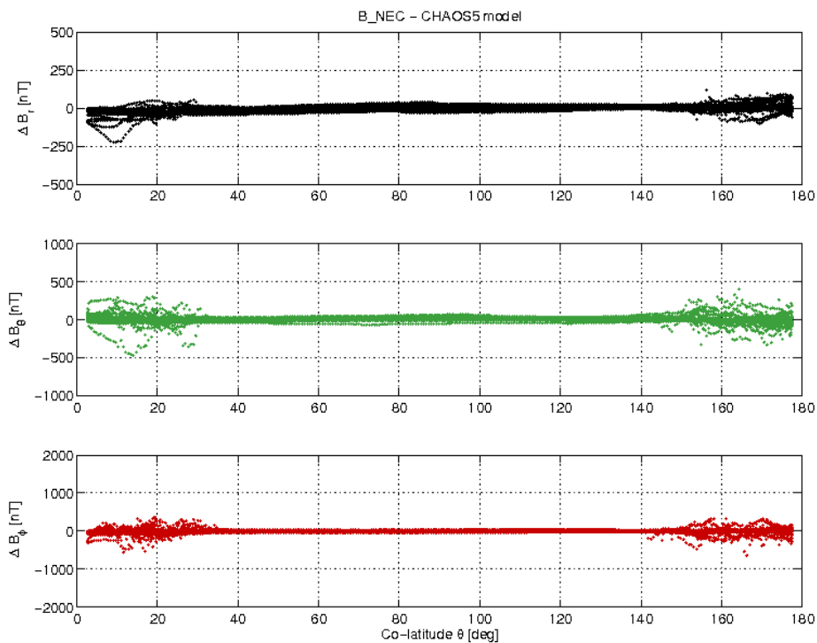
Figure 13: Swarm A day 14/03 B_{NEC} - B_{Chaos} vs colatitude.
