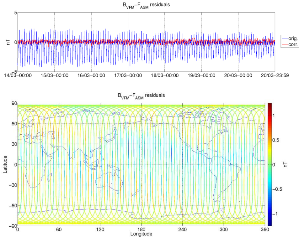
Figure 8: ASM-VFM residuals for S/C A, during monitoring period 14/03-20/03. In top figure are plotted: difference between |B_{VFM}| and F_{ASM} (without dB Sun correction) (blue colour), and the residuals with dB Sun corrections (red colour). In bottom figure residuals are presented on the world map.
