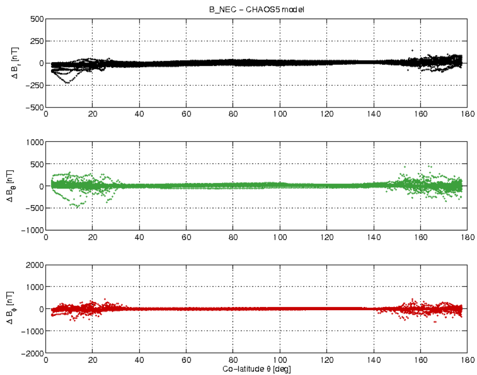
Figure 17: Swarm C day 14/03 B_{NEC} - B_{Chaos} difference vs colatitude.
