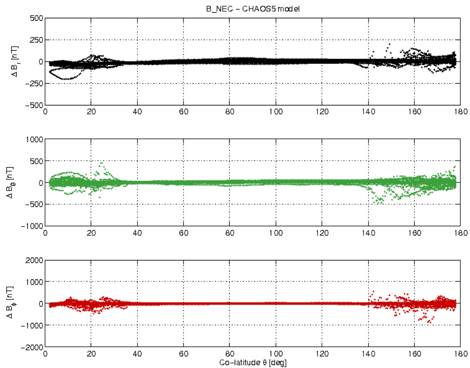
Figure 15: Swarm B day 14/03 B_{NEC} - B_{Chaos} difference vs colatitude.
