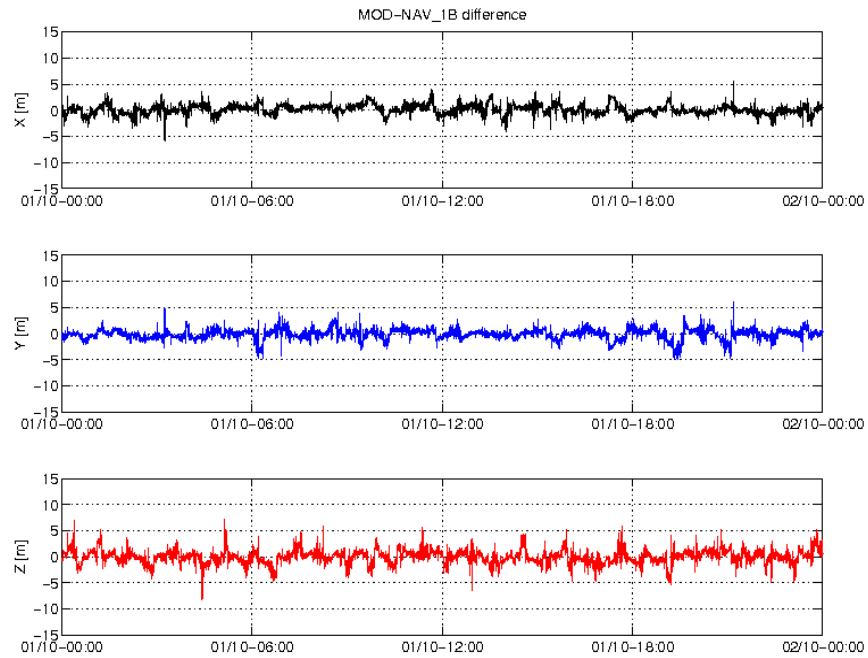
Figure 2: Difference MOD-GPSNAV, S/C A, 01/10. From top to bottom: X, Y and Z axis
