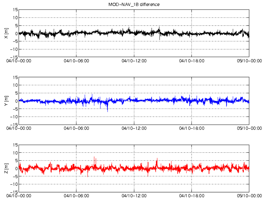
Figure 9: Difference MOD-GPSNAV, S/C C, 04/10. From top to bottom: X, Y and Z axis
