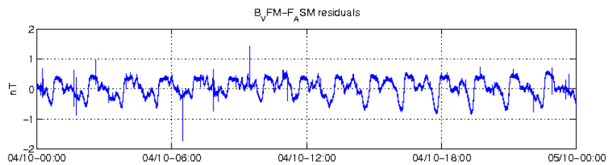
Figure 13: ASM-VFM residuals for S/C A, 04/10.
