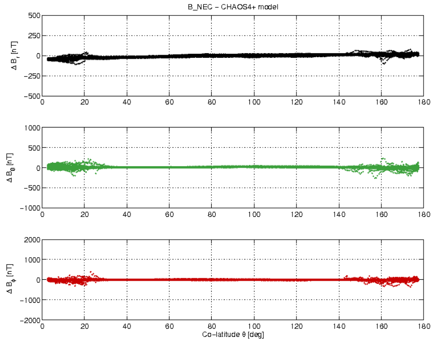
Figure 23: Swarm C day 28/09 B_NEC - B_Chao difference vs colatitude.
