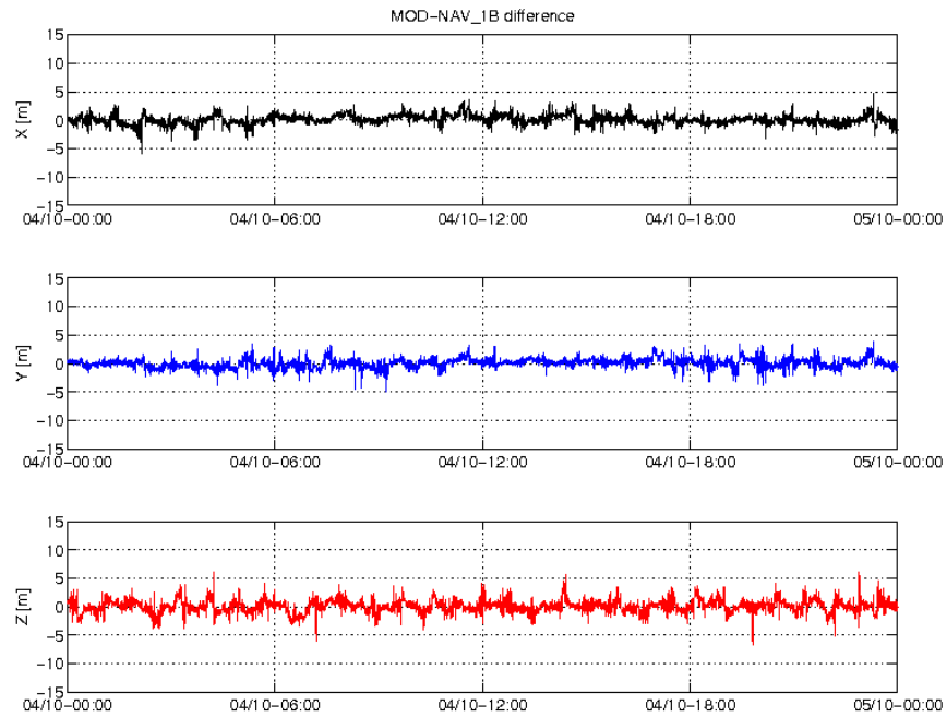
Figure 3: Difference MOD-GPSNAV, S/C A, 04/10. From top to bottom: X, Y and Z axis
