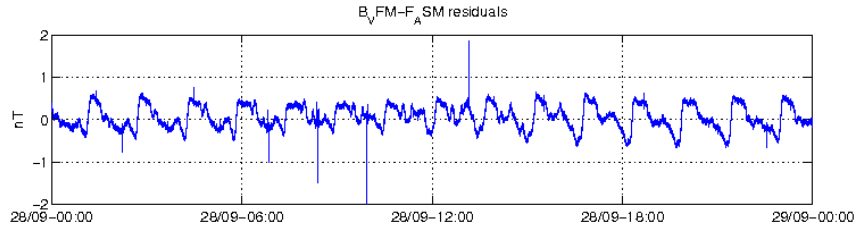
Figure 12: ASM-VFM residuals for S/C A, 28/09.
