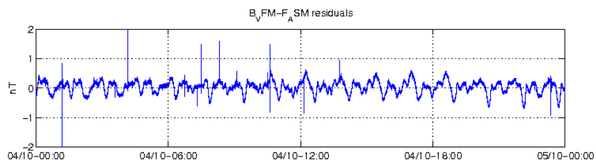
Figure 15: ASM-VFM residuals for S/C B, 04/10.
