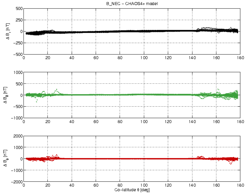
Figure 21: Swarm B day 28/09 B_NEC - B_Chaos difference vs colatitude.
