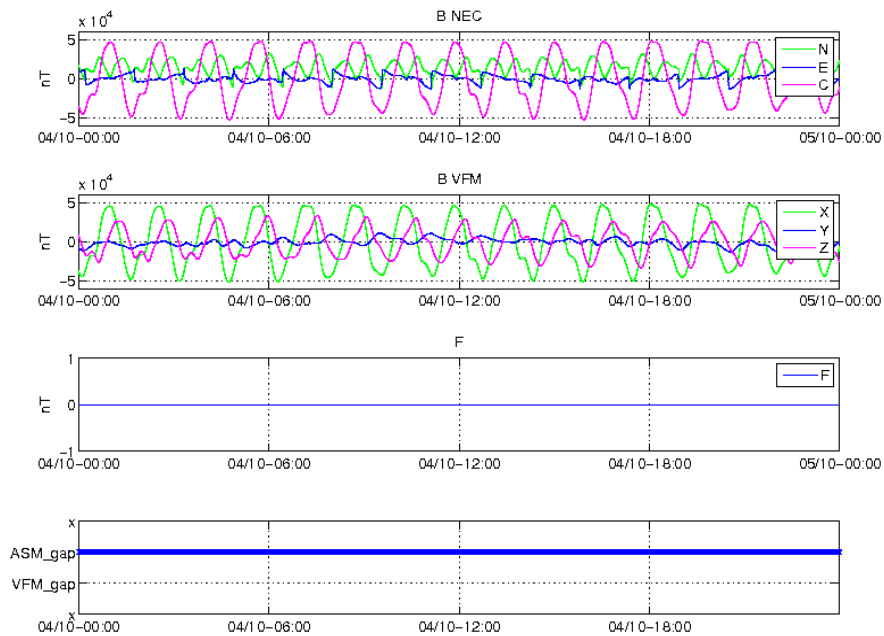
Figure 18: Time series of the geomagnetic field for 04/10, S/C C. From top to bottom: magnetic field components in NEC reference frame, magnetic field components in the VFM reference frame, magnetic field intensity (F) from ASM (no data here because ASM it is off) and location of gaps.
