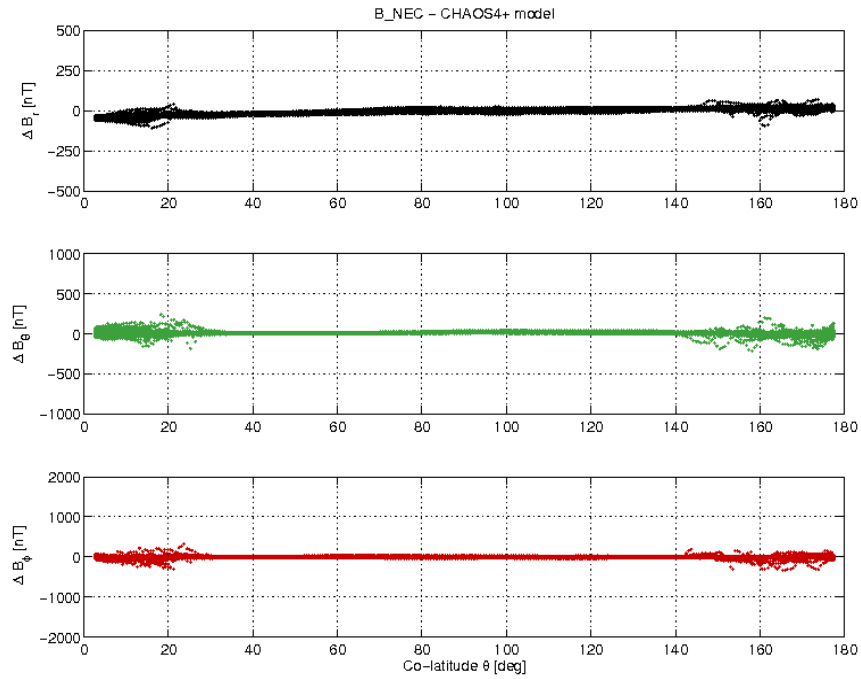
Figure 19: Swarm A day 28/09 B_NEC - B_Chaos vs colatitude.
