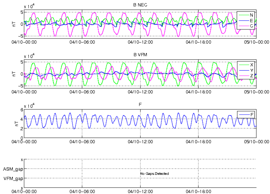
Figure 16: Time series of the geomagnetic field, for 04/10, S/C A. From top to bottom: magnetic field components in NEC reference frame, magnetic field components in the VFM reference frame, magnetic field intensity (F) from ASM, and location of gaps (if any).
