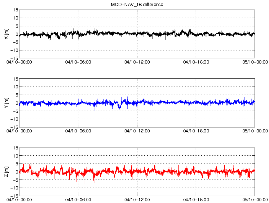
Figure 6: Difference MOD-GPSNAV, S/C B, 04/10. From top to bottom: X, Y and Z axis
