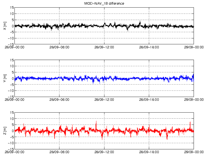
Figure 4: Difference MOD-GPSNAV, S/C B, 28/09. From top to bottom: X, Y and Z axis
