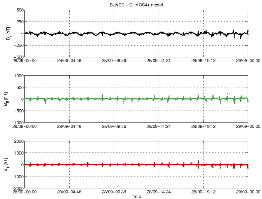
Figure 20: Swarm A day 28/09: time series of B_NEC – B_Chaos residuals.
