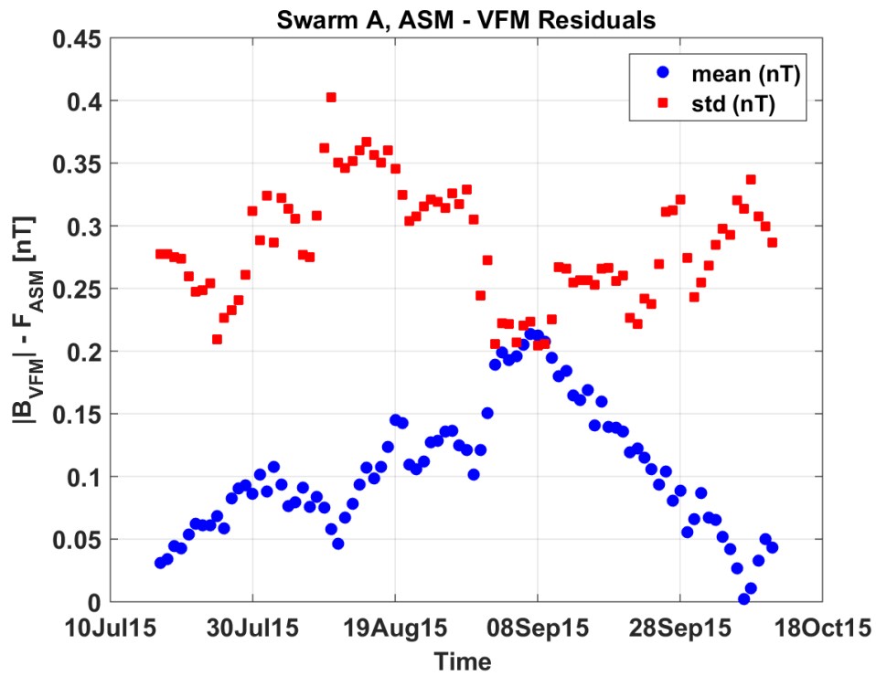
Figure 10: Daily mean and standard deviation values of ASM-VFM residuals (defined as dF=|B_{VFM}|-F_{ASM} ) for S/C Alpha.
