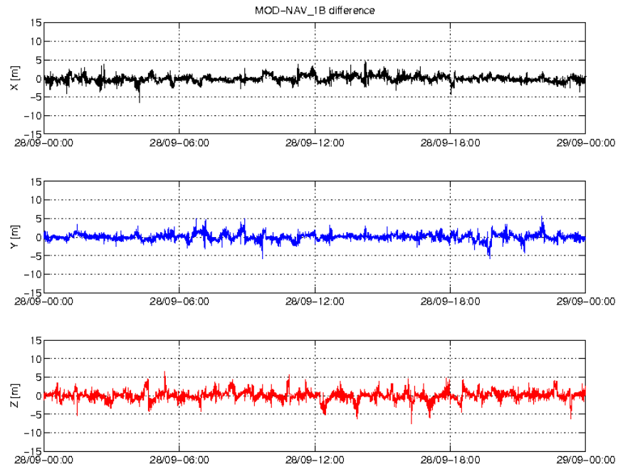
Figure 7: Difference MOD-GPSNAV, S/C C, 28/09. From top to bottom: X, Y and Z axis
