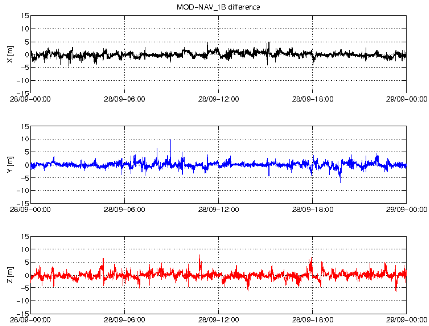
Figure 1: Difference MOD-GPSNAV, S/C A, 28/09. From top to bottom: X, Y and Z axis
