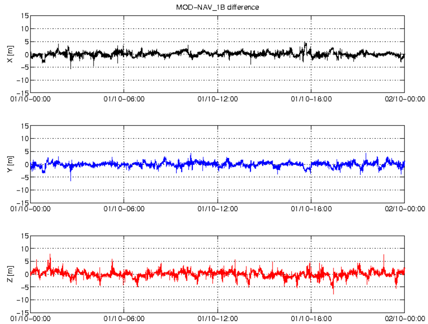
Figure 5: Difference MOD-GPSNAV, S/C B, 01/10. From top to bottom: X, Y and Z axis
