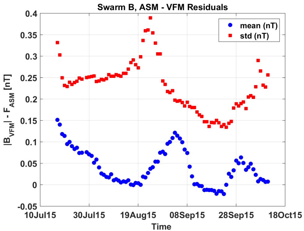
Figure 11: Daily mean and standard deviation values of ASM-VFM residuals (defined as dF=|B_{VFM}|-F_{ASM} ) for S/C Alpha.
