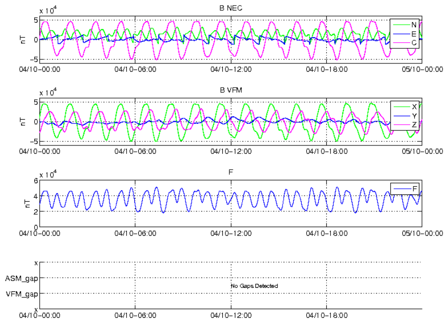
Figure 17: Time series of the geomagnetic field for 04/10, S/C B. From top to bottom: magnetic field components in NEC reference frame, magnetic field components in the VFM reference frame, magnetic field intensity (F) from ASM, and location of gaps (if any).
