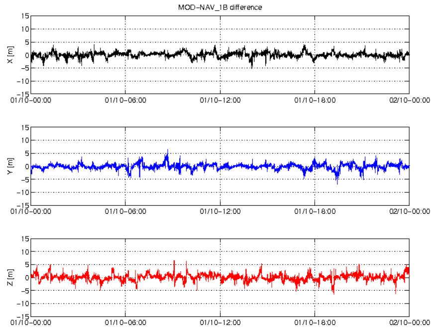
Figure 8: Difference MOD-GPSNAV, S/C C, 01/10. From top to bottom: X, Y and Z axis
