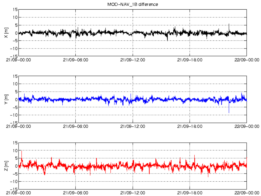
Figure 4: Difference MOD-GPSNAV, S/C B, 21/09. From top to bottom: X, Y and Z axis
