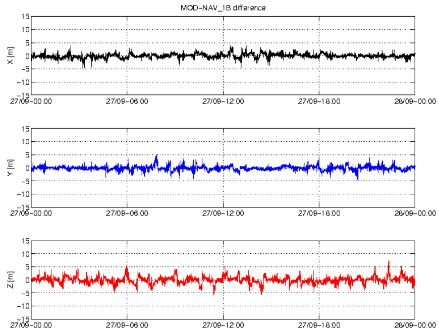
Figure 9: Difference MOD-GPSNAV, S/C C, 27/09. From top to bottom: X, Y and Z axis
