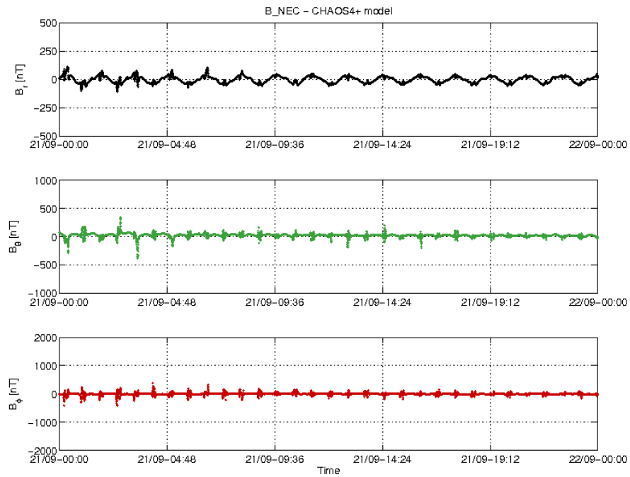
Figure 22: Swarm B day 21/09 time series of B_NEC – B_ChaoS4+ residuals.
