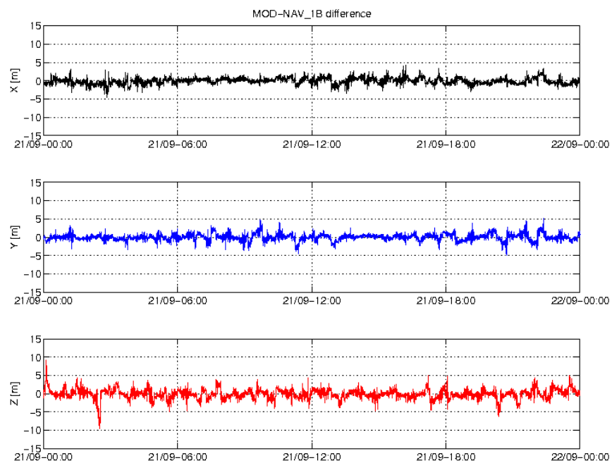
Figure 7: Difference MOD-GPSNAV, S/C C, 21/09. From top to bottom: X, Y and Z axis
