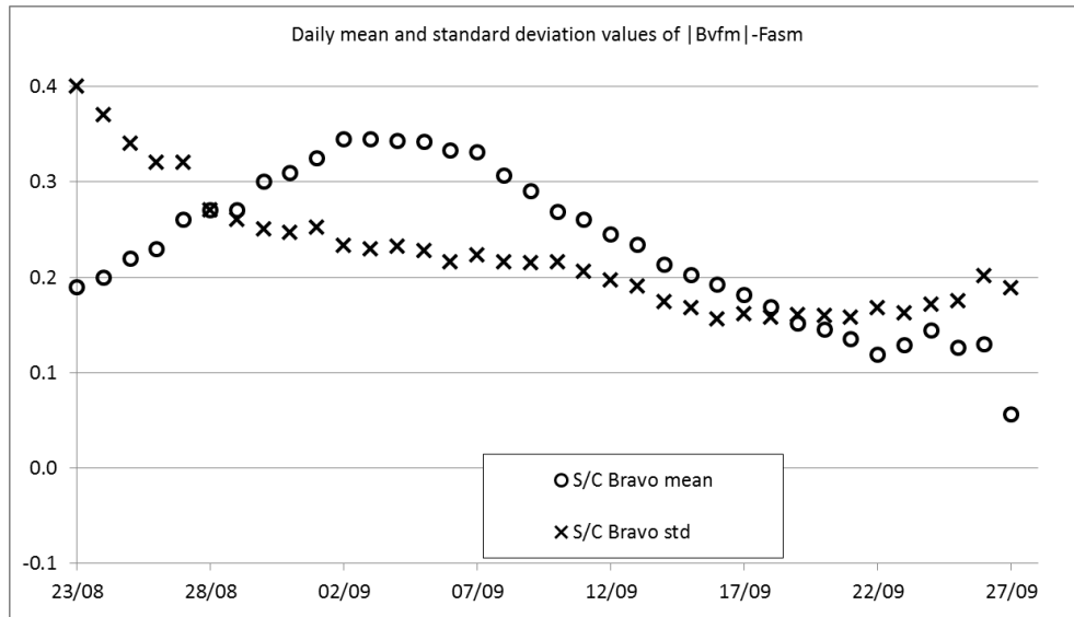
Figure 11: Daily mean and standard deviation values of ASM-VFM residuals (defined as dF=|B_{VFM}|-F_{ASM} ) for S/C Bravo.
