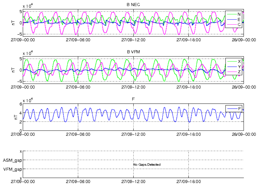
Figure 16: Time series of the geomagnetic field, for 27/09, S/C A. From top to bottom: magnetic field components in NEC reference frame, magnetic field components in the VFM reference frame, magnetic field intensity (F) from ASM, and location of gaps (if any).
