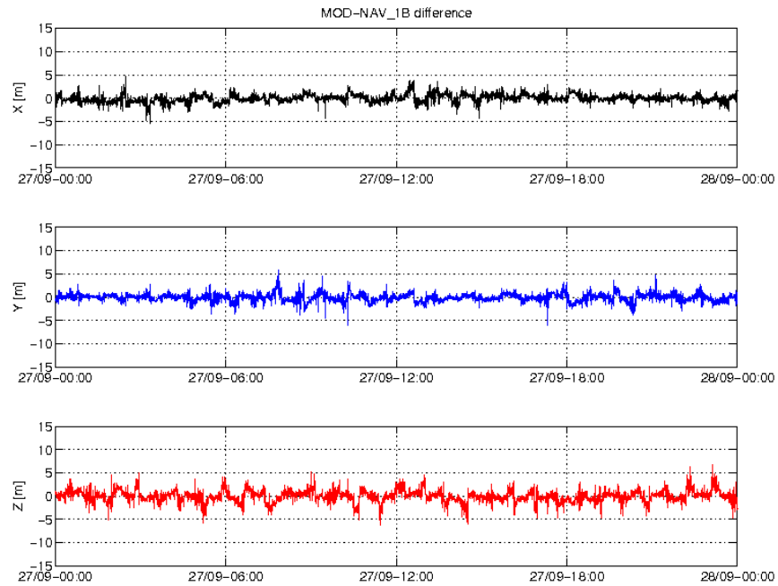
Figure 3: Difference MOD-GPSNAV, S/C A, 27/09. From top to bottom: X, Y and Z axis
