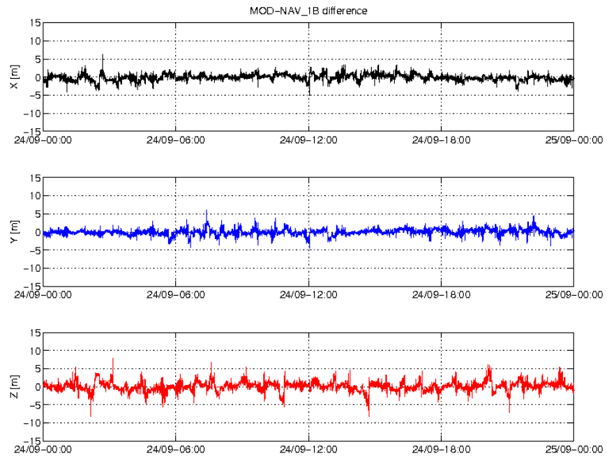
Figure 2: Difference MOD-GPSNAV, S/C A, 24/09. From top to bottom: X, Y and Z axis
