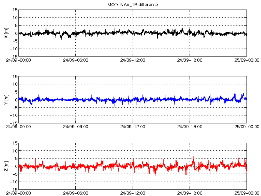
Figure 5: Difference MOD-GPSNAV, S/C B, 24/09. From top to bottom: X, Y and Z axis
