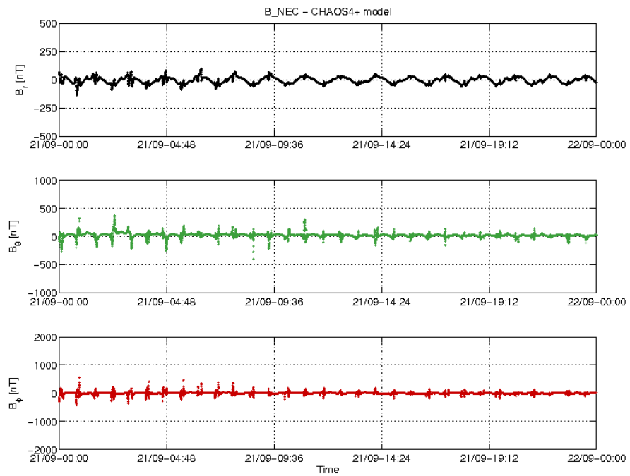
Figure 20: Swarm A day 21/09: time series of B_NEC – B_Chaos residuals.
