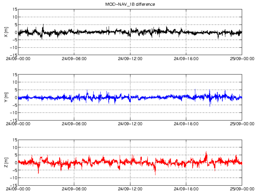
Figure 8: Difference MOD-GPSNAV, S/C C, 24/09. From top to bottom: X, Y and Z axis
