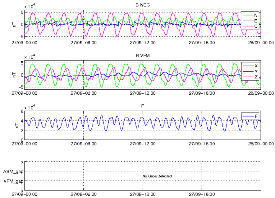
Figure 17: Time series of the geomagnetic field for 27/09, S/C B. From top to bottom: magnetic field components in NEC reference frame, magnetic field components in the VFM reference frame, magnetic field intensity (F) from ASM, and location of gaps (if any).
