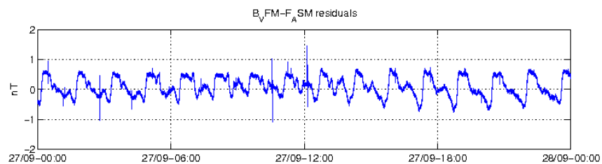
Figure 13: ASM-VFM residuals for S/C A, 27/09.
