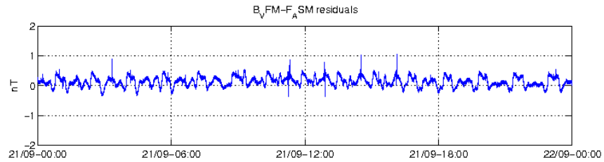
Figure 14: ASM-VFM residuals for S/C B, 21/09.
