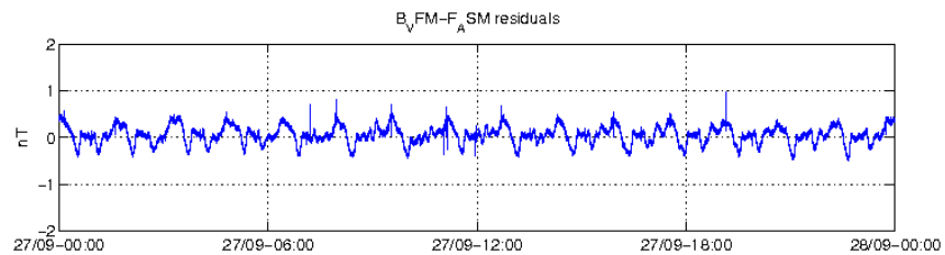
Figure 15: ASM-VFM residuals for S/C B, 27/09.
