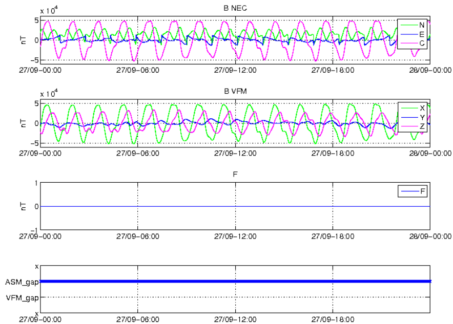
Figure 18: Time series of the geomagnetic field for 27/09, S/C C. From top to bottom: magnetic field components in NEC reference frame, magnetic field components in the VFM reference frame, magnetic field intensity (F) from ASM (no data here because ASM it is off) and location of gaps.
