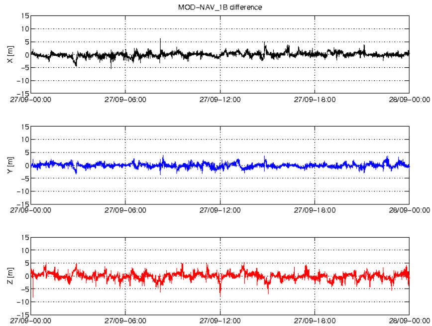
Figure 6: Difference MOD-GPSNAV, S/C B, 27/09. From top to bottom: X, Y and Z axis
