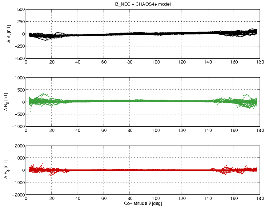
Figure 19: Swarm A day 21/09 B_NEC - B_Chaos vs colatitude.
