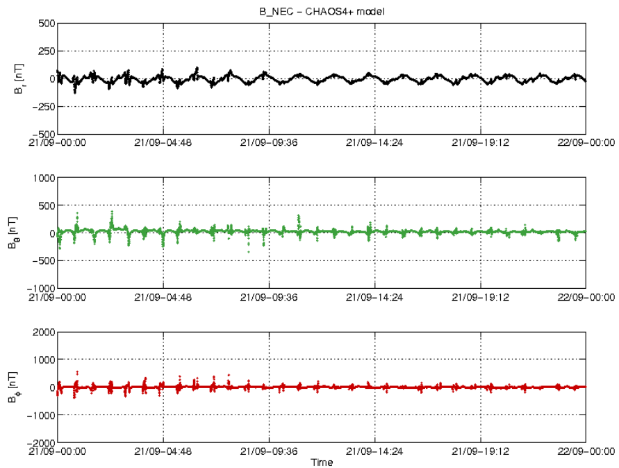
Figure 24: Swarm C day 21/09 time series of B_NEC – B_ChaoS4+ residuals.
