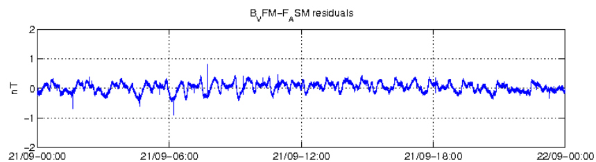
Figure 12: ASM-VFM residuals for S/C A, 21/09.
