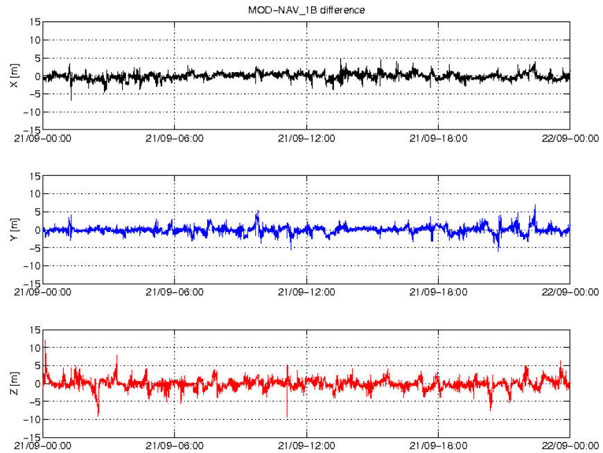
Figure 1: Difference MOD-GPSNAV, S/C A, 21/09. From top to bottom: X, Y and Z axis
