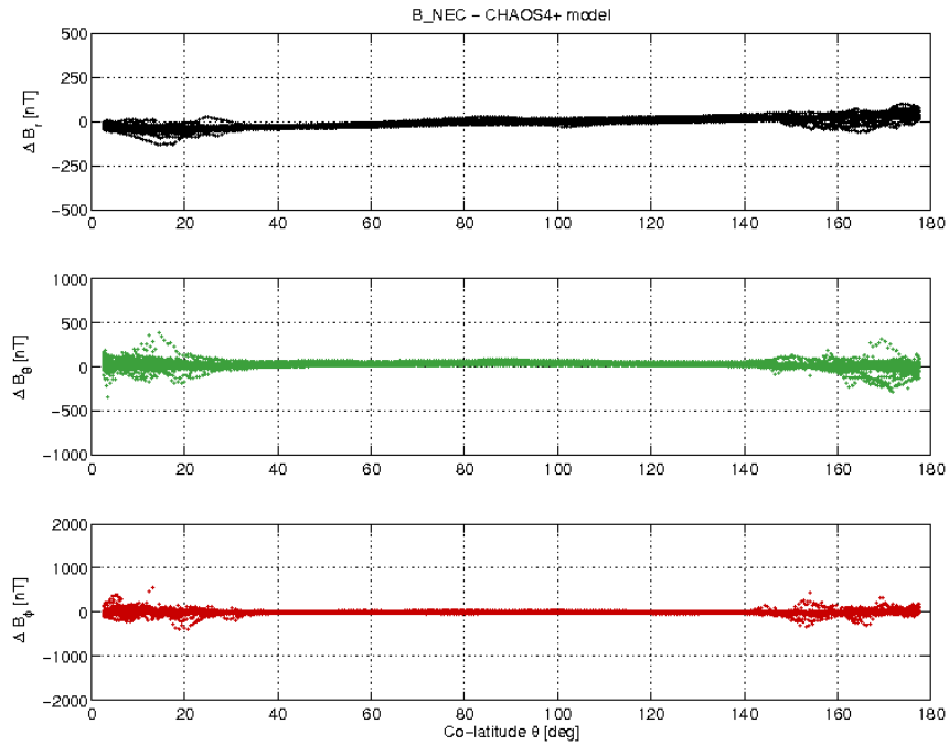
Figure 23: Swarm C day 21/09 B_NEC - B_ChaoS4+ difference vs colatitude.
