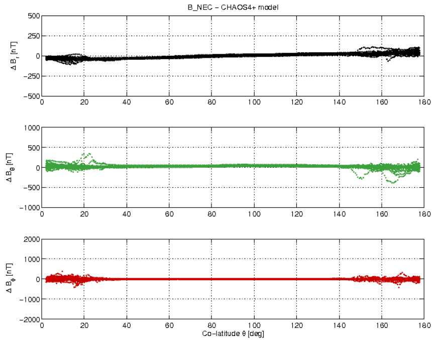
Figure 21: Swarm B day 21/09 B_NEC - B_ChaoS4+ difference vs colatitude.
