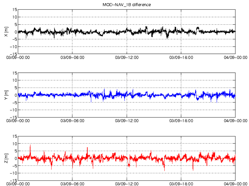
Figure 2: Difference MOD-GPSNAV, S/C A, 03/09. From top to bottom: X, Y and Z axis
