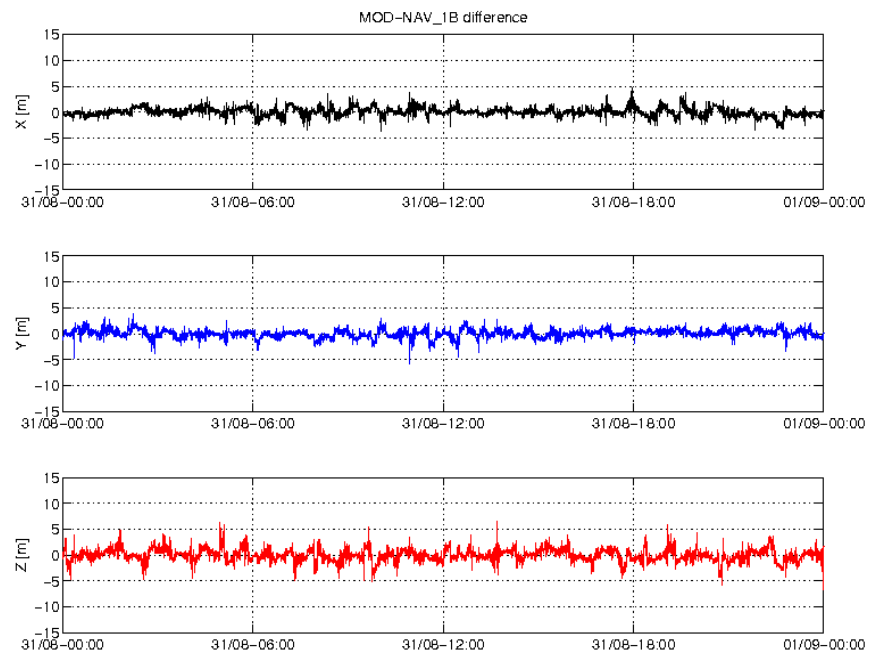
Figure 4: Difference MOD-GPSNAV, S/C B, 31/08. From top to bottom: X, Y and Z axis
