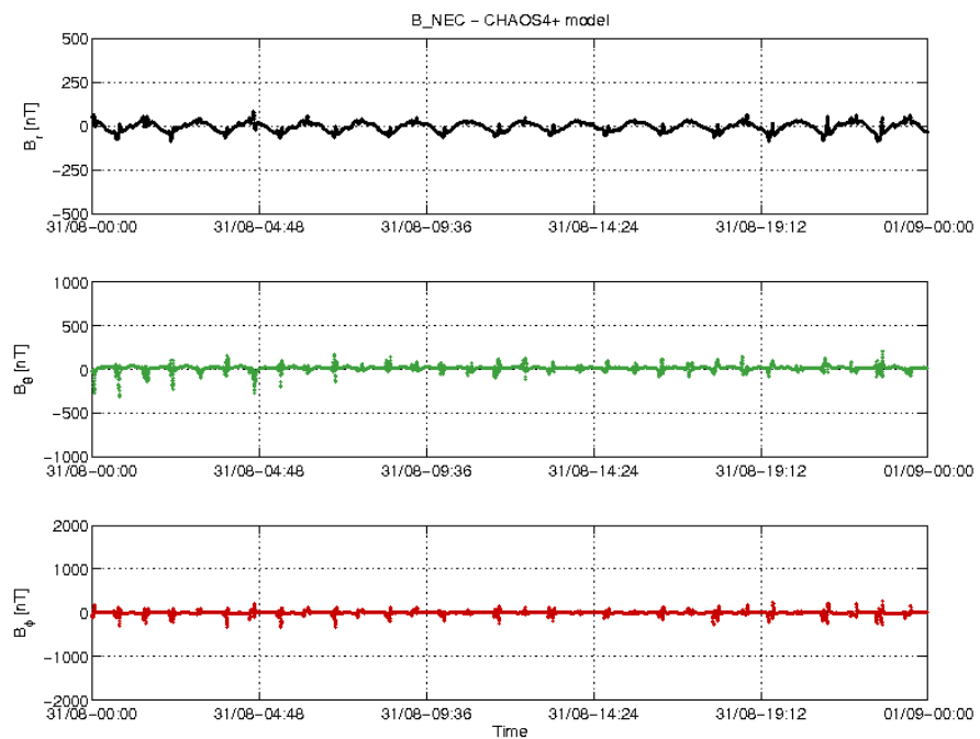
Figure 20: Swarm A day 31/08: time series of B_NEC – B_Chaos residuals.
