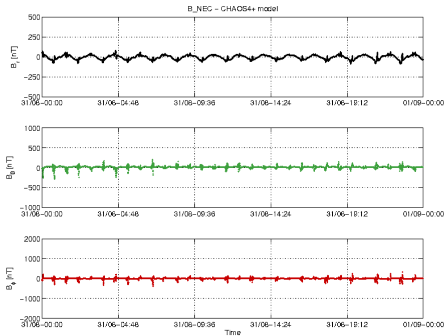
Figure 24: Swarm C day 31/08 time series of B_NEC – B_Chao residuals.
