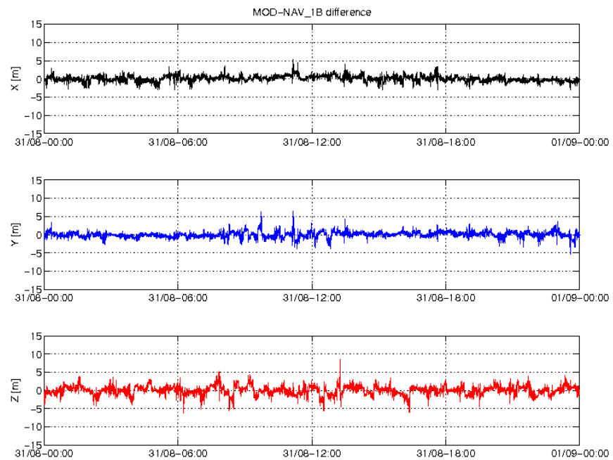
Figure 1: Difference MOD-GPSNAV, S/C A, 31/08. From top to bottom: X, Y and Z axis
