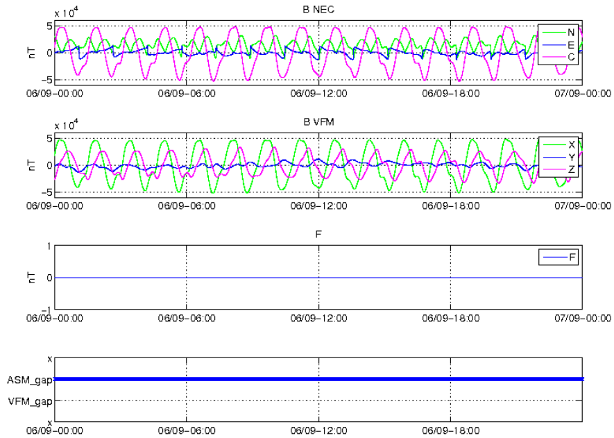
Figure 18: Time series of the geomagnetic field for 06/09, S/C C. From top to bottom: magnetic field components in NEC reference frame, magnetic field components in the VFM reference frame, magnetic field intensity (F) from ASM (no data here because ASM it is off) and location of gaps.
