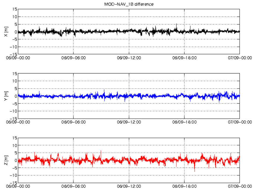
Figure 9: Difference MOD-GPSNAV, S/C C, 06/09. From top to bottom: X, Y and Z axis
