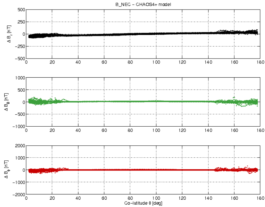
Figure 21: Swarm B day 31/08 B_NEC - B_ChaoS4+ difference vs colatitude.
