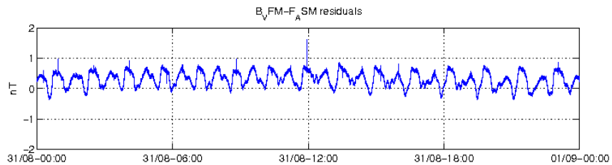
Figure 14: ASM-VFM residuals for S/C B, 31/08.
