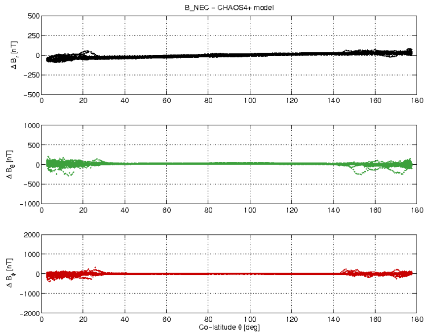
Figure 23: Swarm C day 31/08 B_NEC - B_Chao difference vs colatitude.
