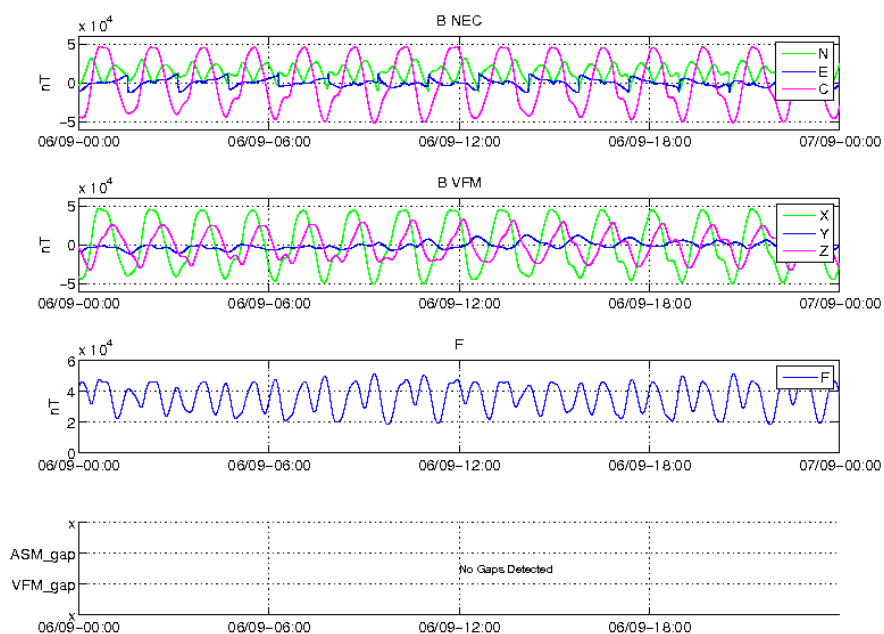
Figure 17: Time series of the geomagnetic field for 06/09, S/C B. From top to bottom: magnetic field components in NEC reference frame, magnetic field components in the VFM reference frame, magnetic field intensity (F) from ASM, and location of gaps (if any).
