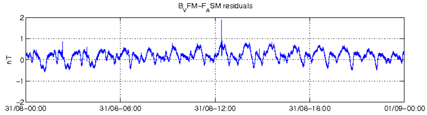
Figure 12: ASM-VFM residuals for S/C A, 31/08.
