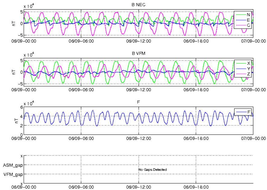
Figure 16: Time series of the geomagnetic field, for 06/09, S/C A. From top to bottom: magnetic field components in NEC reference frame, magnetic field components in the VFM reference frame, magnetic field intensity (F) from ASM, and location of gaps (if any).
