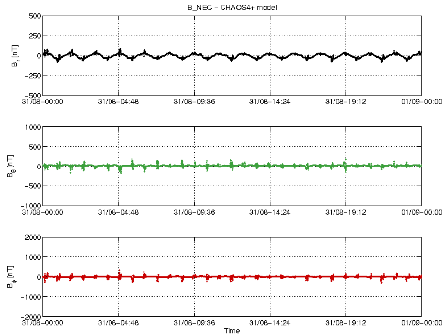
Figure 22: Swarm B day 31/08 time series of B_NEC – B_ChaoS4+ residuals.
