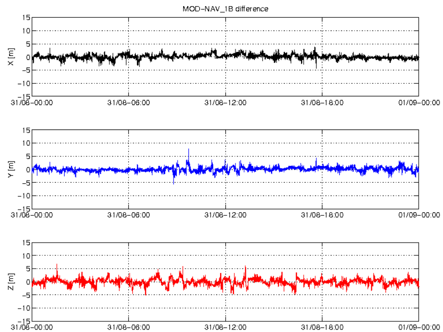
Figure 7: Difference MOD-GPSNAV, S/C C, 31/08. From top to bottom: X, Y and Z axis
