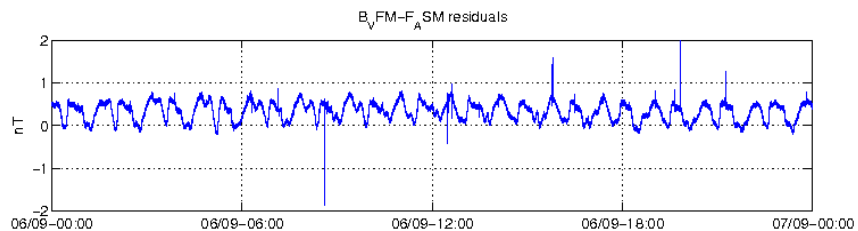
Figure 15: ASM-VFM residuals for S/C B, 06/09.
