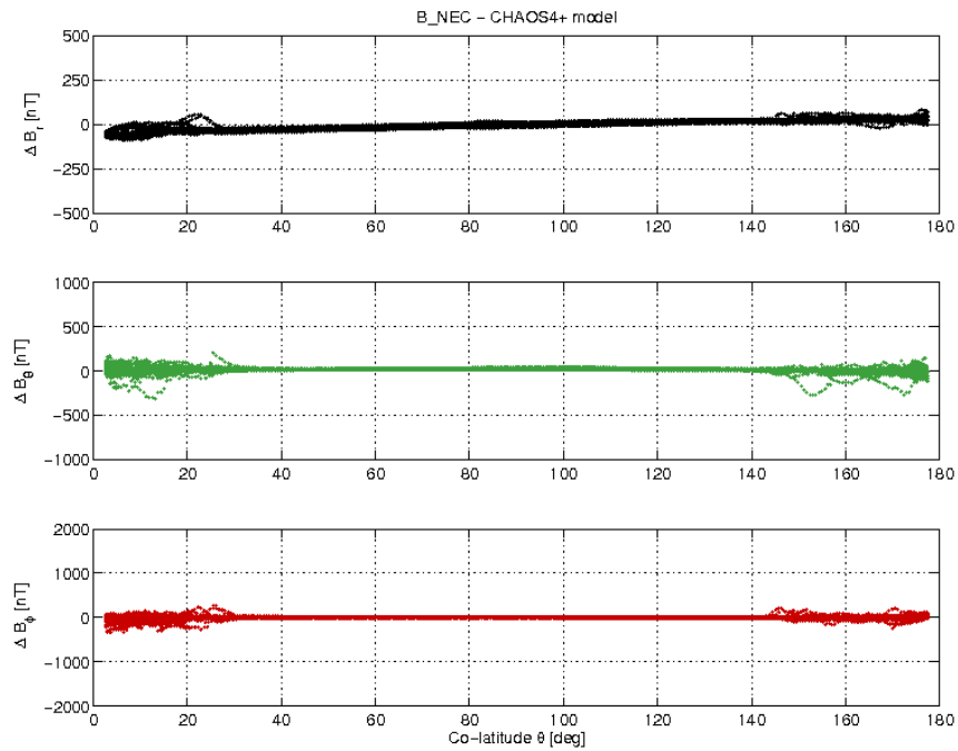
Figure 19: Swarm A day 31/08 B_NEC - B_Chaos vs colatitude.
