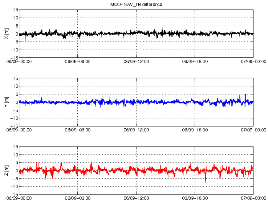
Figure 3: Difference MOD-GPSNAV, S/C A, 06/09. From top to bottom: X, Y and Z axis
