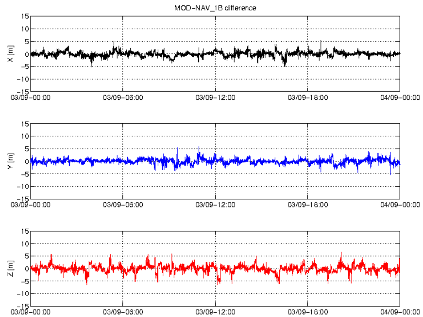
Figure 8: Difference MOD-GPSNAV, S/C C, 03/09. From top to bottom: X, Y and Z axis
