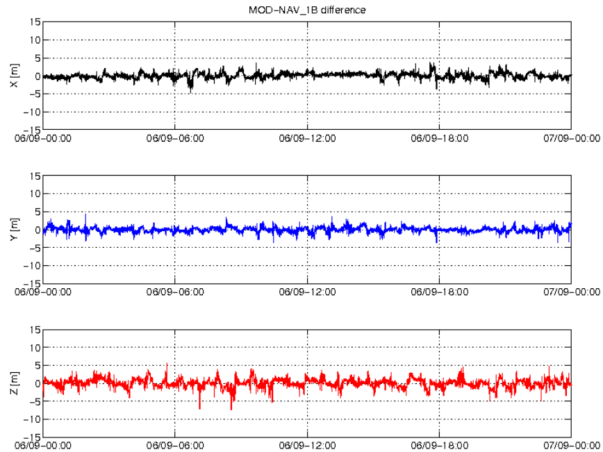
Figure 6: Difference MOD-GPSNAV, S/C B, 06/09. From top to bottom: X, Y and Z axis
