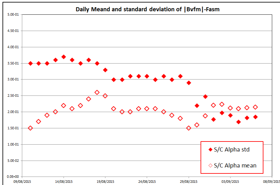
Figure 10: Daily mean and standard deviation values of ASM-VFM residuals (defined as dF=|B_{VFM}|-F_{ASM} ) for S/C Alpha.
