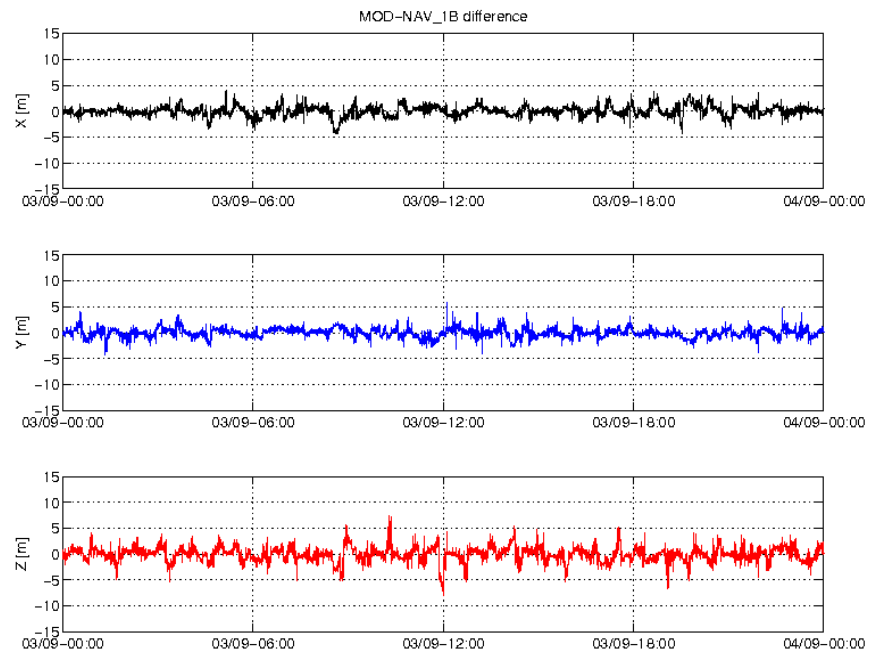
Figure 5: Difference MOD-GPSNAV, S/C B, 03/09. From top to bottom: X, Y and Z axis
