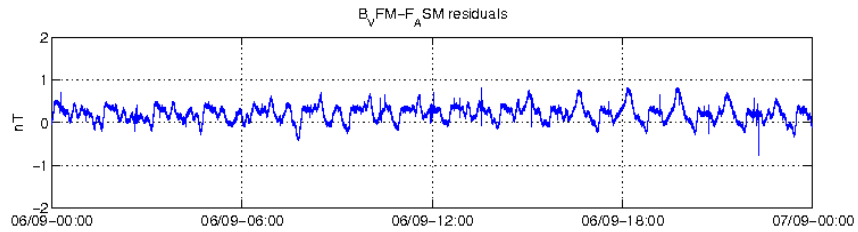
Figure 13: ASM-VFM residuals for S/C A, 06/09.
