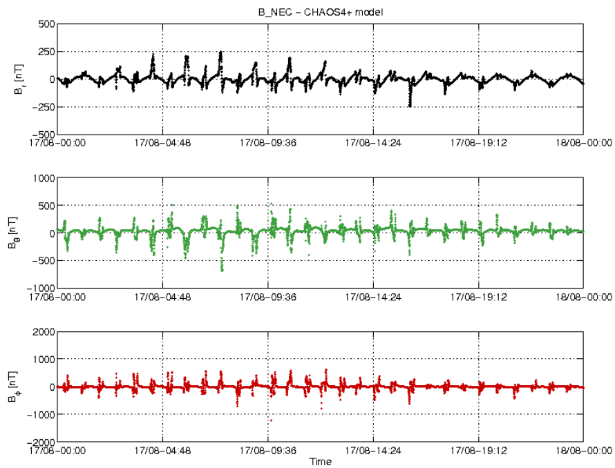
Figure 22: Swarm B day 17/08 time series of B_{NEC} - B_{Chaos} residuals.
