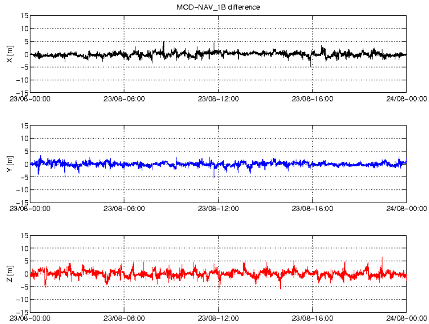
Figure 6: Difference MOD-GPSNAV, S/C B, 23/08. From top to bottom: X, Y and Z axis
