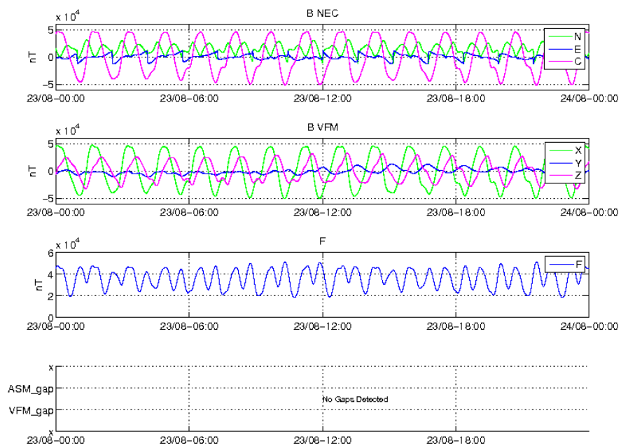
Figure 13: Time series of the geomagnetic field for 23/08, S/C B. From top to bottom: magnetic field components in NEC reference frame, magnetic field components in the VFM reference frame, magnetic field intensity (F) from ASM, and location of gaps (if any).
