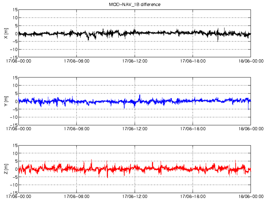
Figure 4: Difference MOD-GPSNAV, S/C B, 17/08. From top to bottom: X, Y and Z axis
