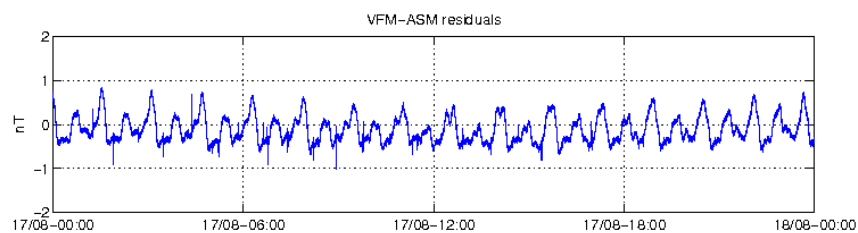
Figure 17: ASM-VFM residuals for S/C B, 17/08.
