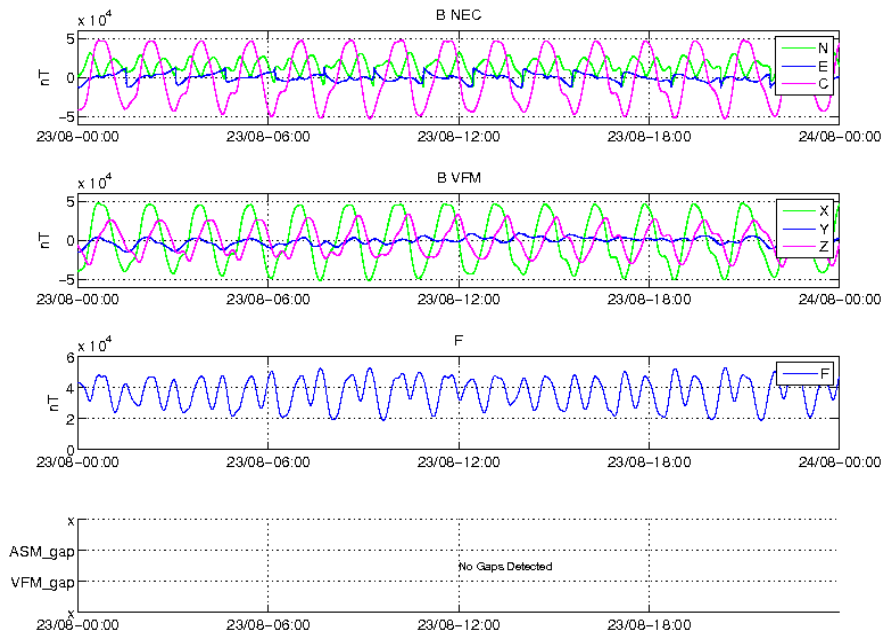
Figure 12: Time series of the geomagnetic field, for 23/08, S/C A. From top to bottom: magnetic field components in NEC reference frame, magnetic field components in the VFM reference frame, magnetic field intensity (F) from ASM, and location of gaps (if any).
