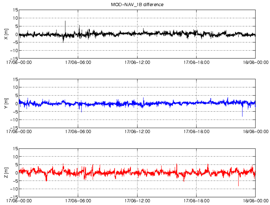
Figure 1: Difference MOD-GPSNAV, S/C A, 17/08. From top to bottom: X, Y and Z axis
