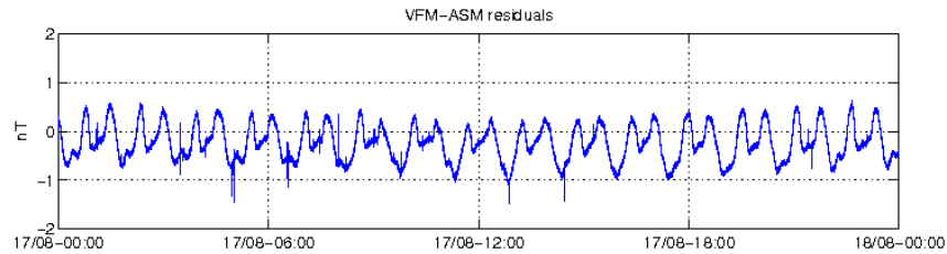
Figure 15: ASM-VFM residuals for S/C A, 17/08.
