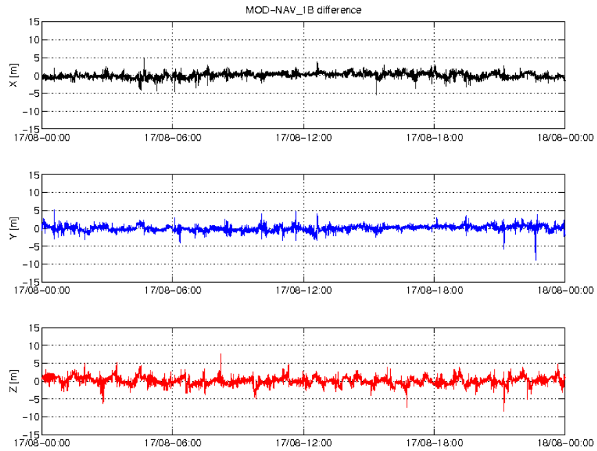
Figure 7: Difference MOD-GPSNAV, S/C C, 17/08. From top to bottom: X, Y and Z axis
