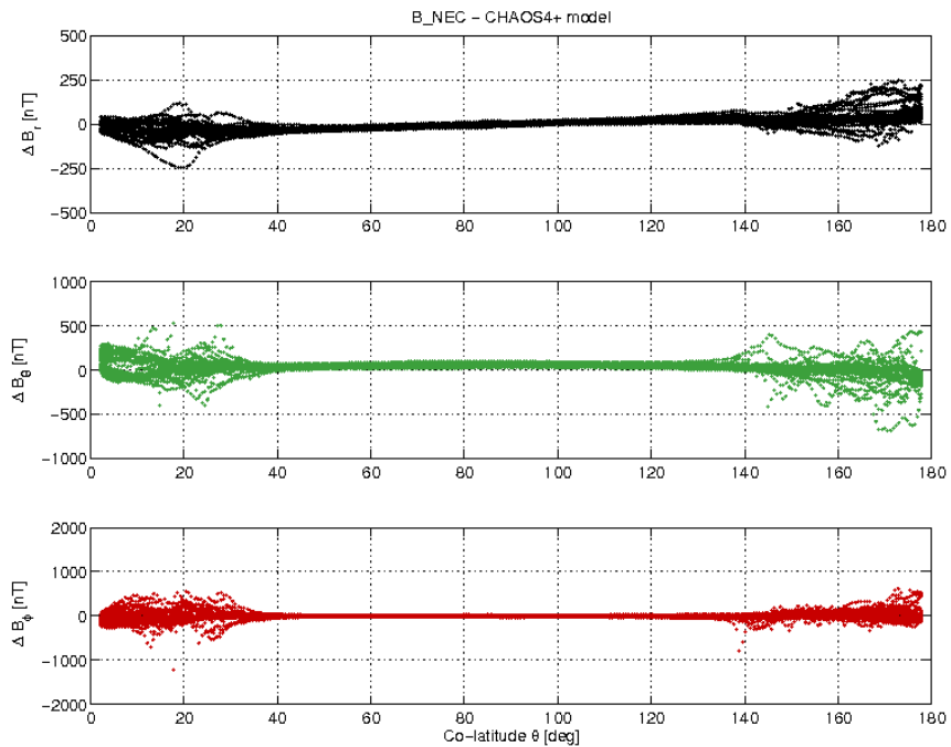
Figure 21: Swarm B day 17/08 B_NEC - B_Chao difference vs colatitude.
