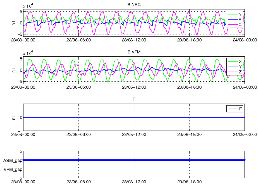
Figure 14: Time series of the geomagnetic field for 23/08, S/C C. From top to bottom: magnetic field components in NEC reference frame, magnetic field components in the VFM reference frame, magnetic field intensity (F) from ASM (no data here because ASM it is off) and location of gaps.
