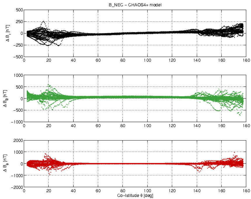
Figure 19: Swarm A day 17/08 B_{NEC} - B_{Chaos} vs colatitude.
