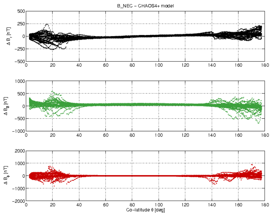
Figure 23: Swarm C day 17/08 B_{NEC} - B_{Chaos} difference vs colatitude.
