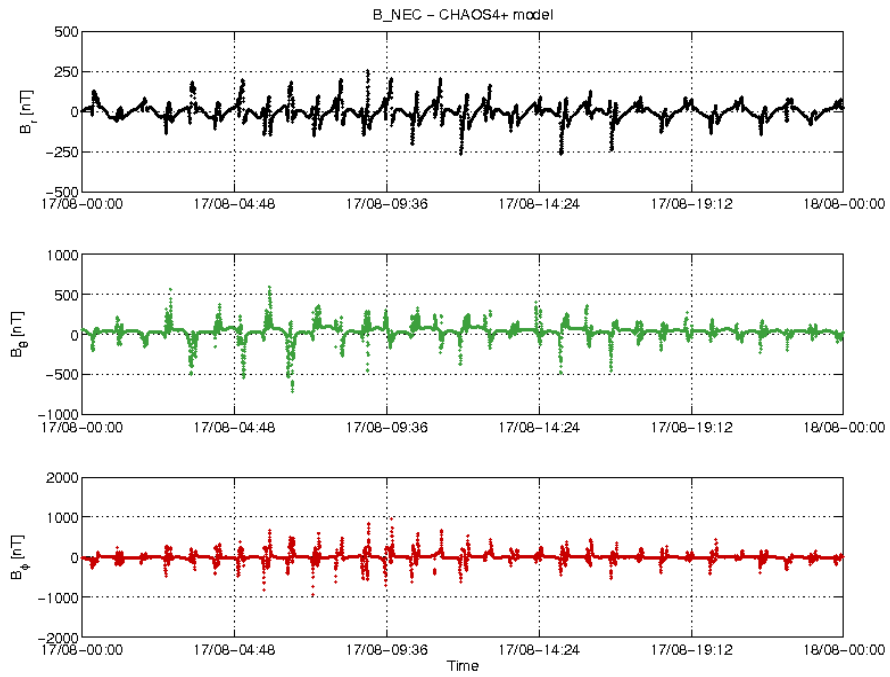
Figure 20: Swarm A day 17/08: time series of B_NEC – B_Chao residuals.
