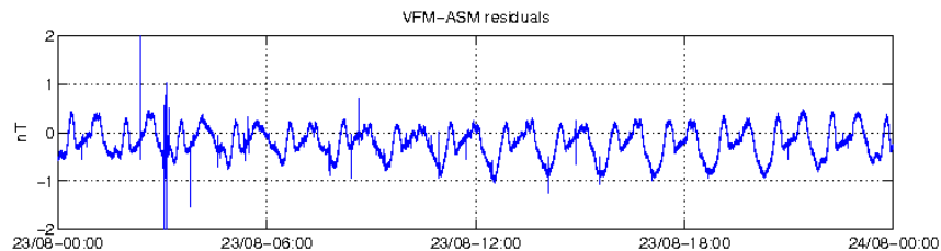
Figure 16: ASM-VFM residuals for S/C A, 23/08.
