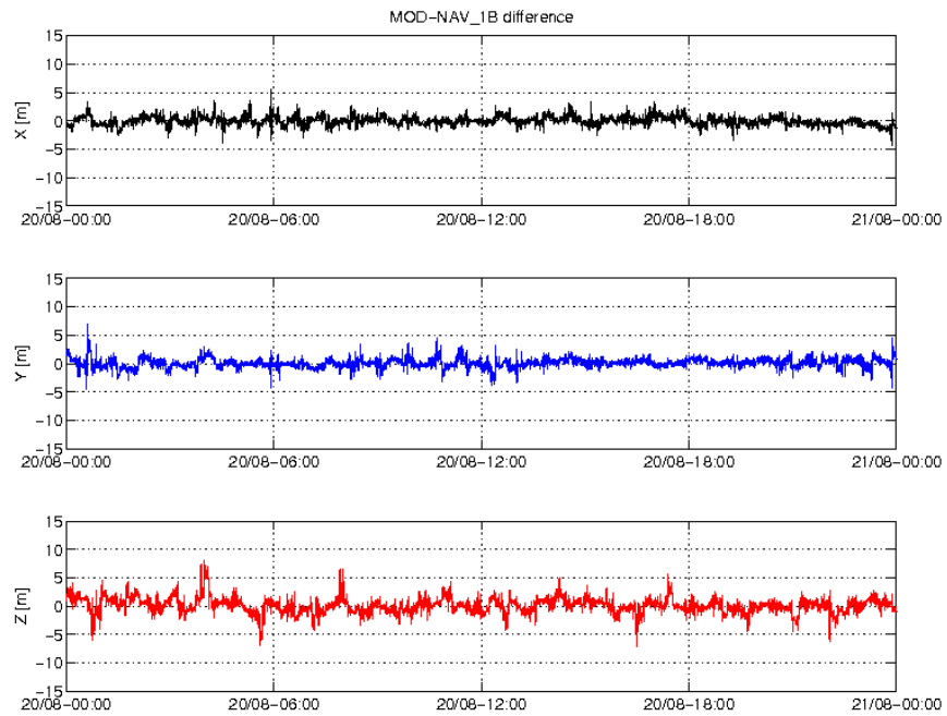
Figure 2: Difference MOD-GPSNAV, S/C A, 20/08. From top to bottom: X, Y and Z axis
