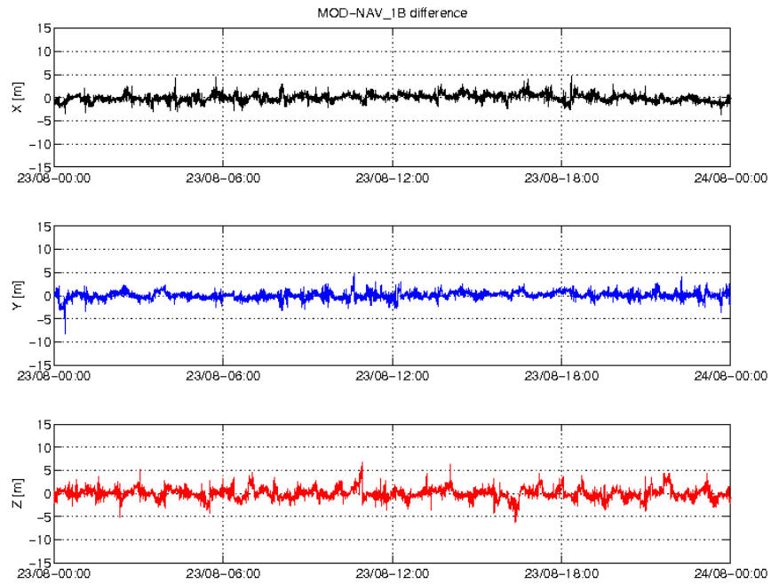
Figure 3: Difference MOD-GPSNAV, S/C A, 23/08. From top to bottom: X, Y and Z axis
