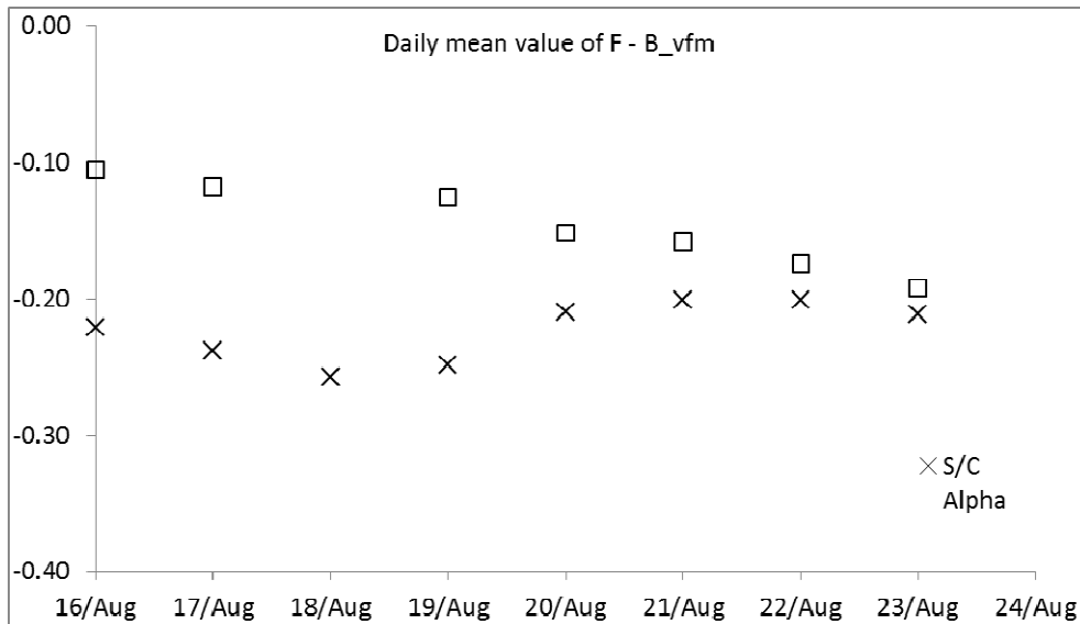
Figure 10: Daily mean values of the difference between F_{ASM} and |B_{VFM}| .
