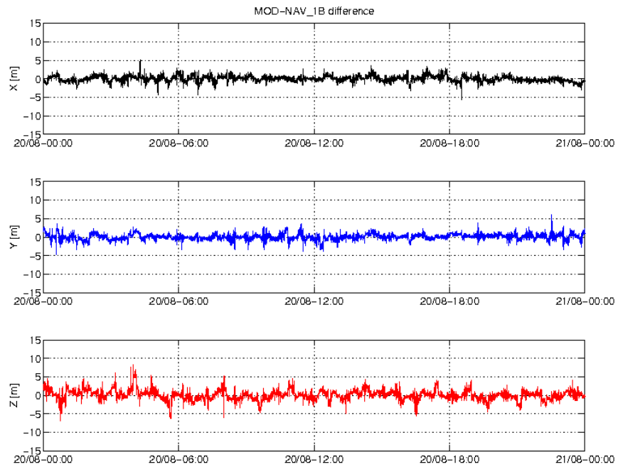
Figure 8: Difference MOD-GPSNAV, S/C C, 20/08. From top to bottom: X, Y and Z axis
