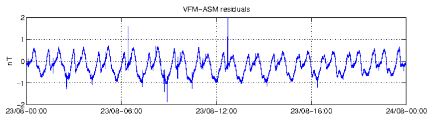
Figure 18: ASM-VFM residuals for S/C B, 23/08.
