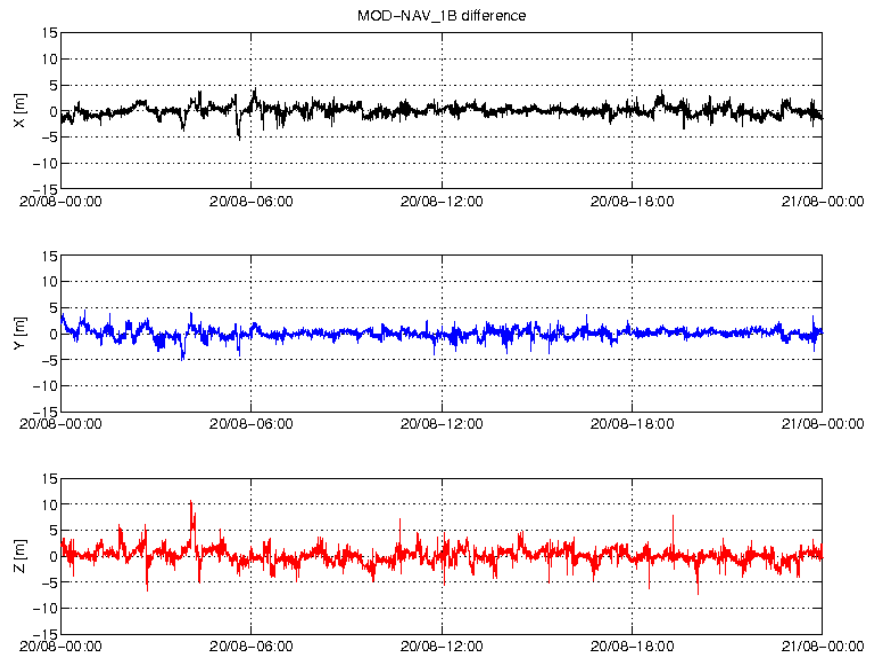
Figure 5: Difference MOD-GPSNAV, S/C B, 20/08. From top to bottom: X, Y and Z axis
