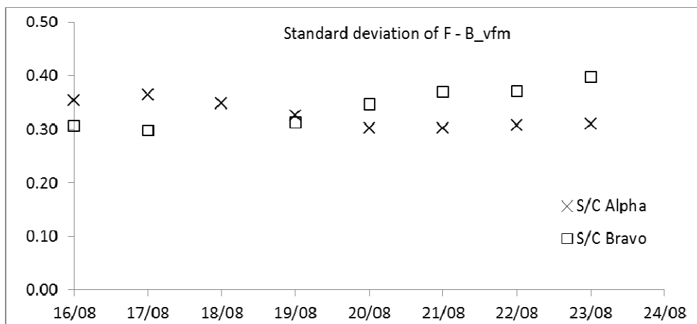
Figure 11: Daily standard deviation values of the difference between F_{ASM} and |B_{VFM}| .
