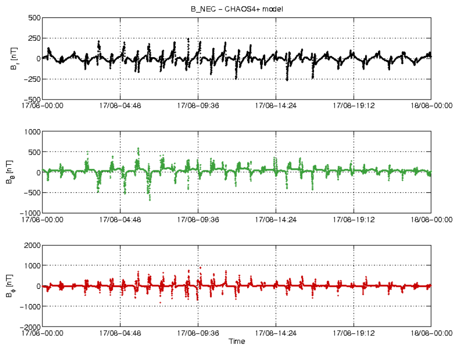
Figure 24: Swarm C day 17/08 time series of B_{NEC} - B_{Chaos} residuals.
