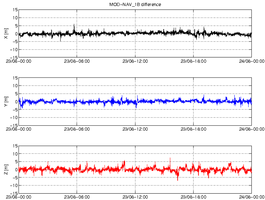
Figure 9: Difference MOD-GPSNAV, S/C C, 23/08. From top to bottom: X, Y and Z axis
