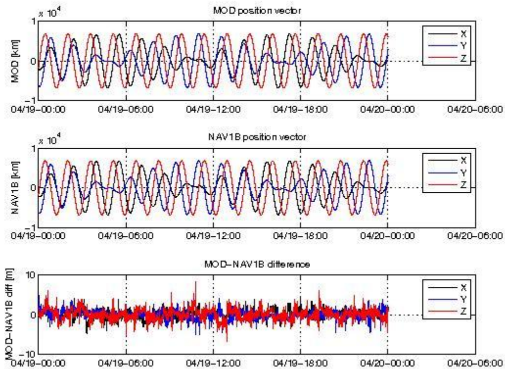
Figure 9: Difference MOD-GPSNAV, S/C C, 19/04. From top to bottom: the S/C position determined from the MOD calculation, the S/C position determined on-board, and the difference between the two.
