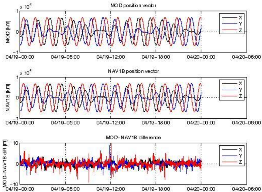
Figure 3: Difference MOD-GPSNAV, S/C A, 19/04. From top to bottom: the S/C position determined from the MOD calculation, the S/C position determined on-board, and the difference between the two. The red circled area shows a big spike in the Y and Z components.
