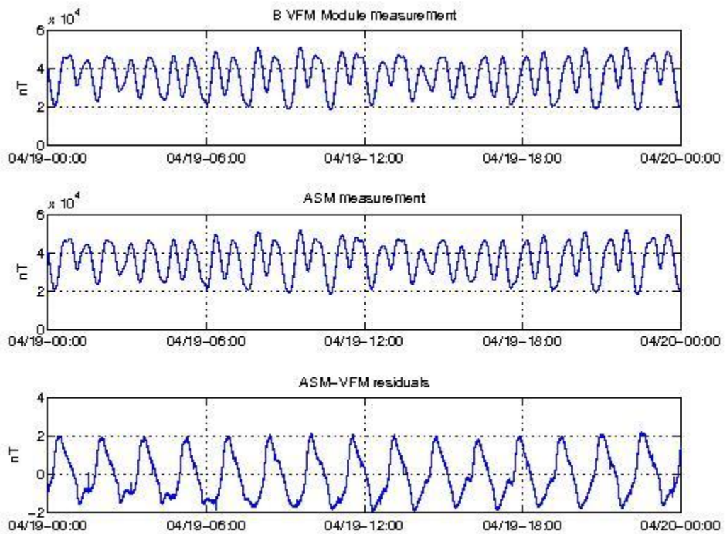
Figure 15: VFM module, ASM module and ASM-VFM residuals for S/C B, 19/04.
