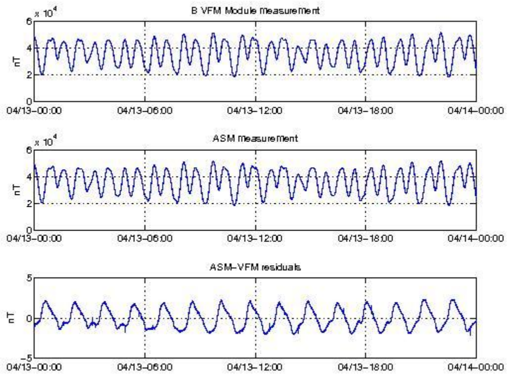
Figure 14: VFM module, ASM module and ASM-VFM residuals for S/C B, 13/04.
