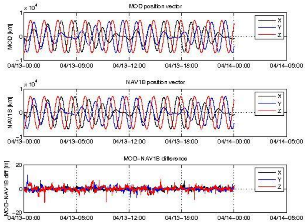
Figure 1: Difference MOD-GPSNAV, S/C A, 13/04. From top to bottom: the S/C position determined from the MOD calculation, the S/C position determined on-board, and the difference between the two.
