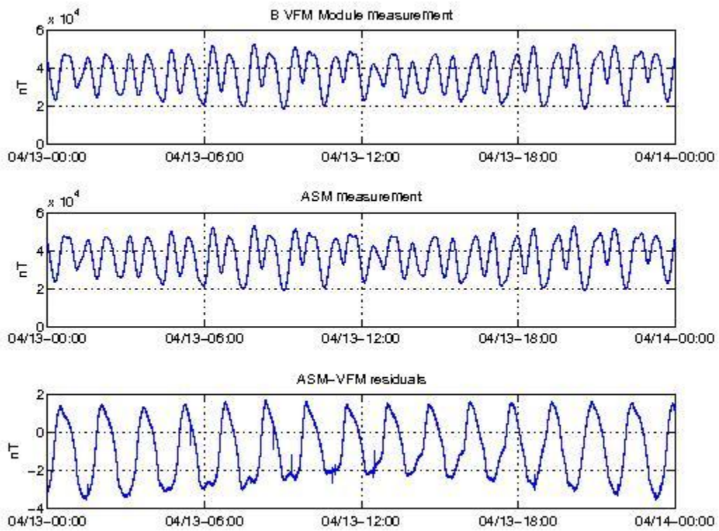
Figure 11: VFM module, ASM module and ASM-VFM residuals for S/C A, 13/04.
