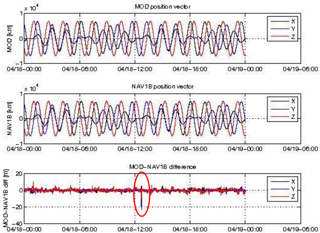
Figure 6: Difference MOD-GPSNAV, S/C B, 18/04. From top to bottom: the S/C position determined from the MOD calculation, the S/C position determined on-board, and the difference between the two. In the red circled area a spike is shown
