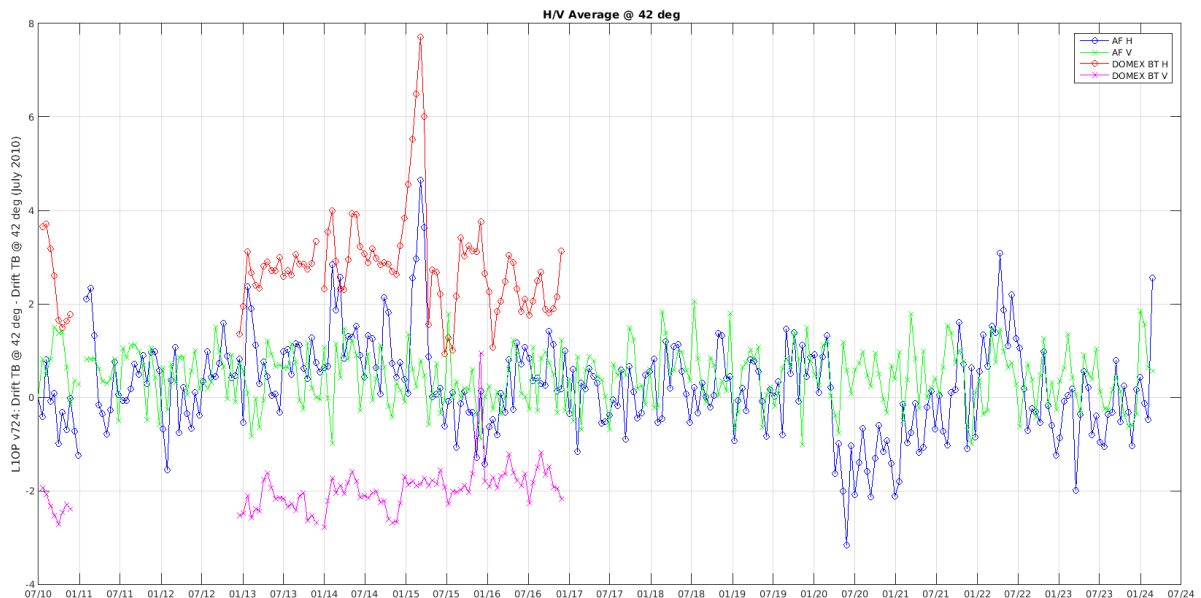
Figure 37: Dome-C H and V polarization trends in Alias Free zone (incidence angle 42°)
