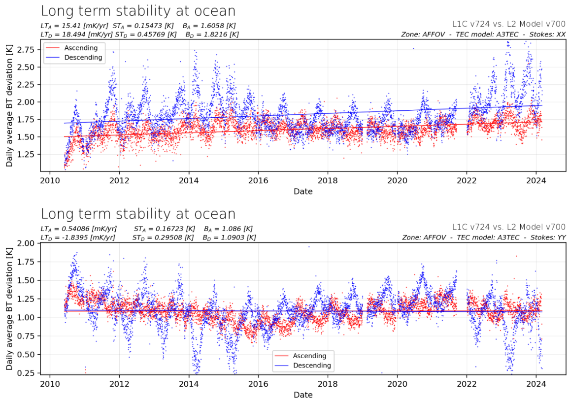
Figure 47: BT long term stability (ASC/DES), for XX and YY polarizations, and Stokes 1.
