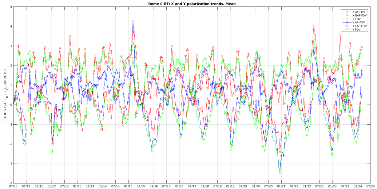
Figure 36: Dome-C X and Y polarization trends (all incidence angles).
