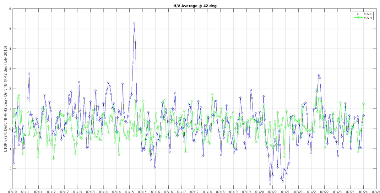
Figure 38: Dome-C H and V polarization trends in Extended Alias Free zone (incidence angle 42°)
