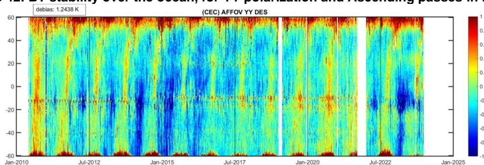
Figure 43: BT stability over the ocean, for YY polarization and Descending passes in Kelvin.
