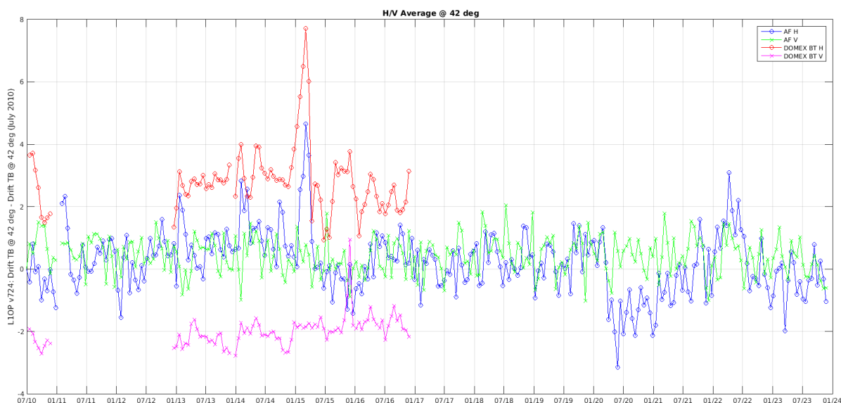
Figure 37: Dome-C H and V polarization trends in Alias Free zone (incidence angle 42°)
