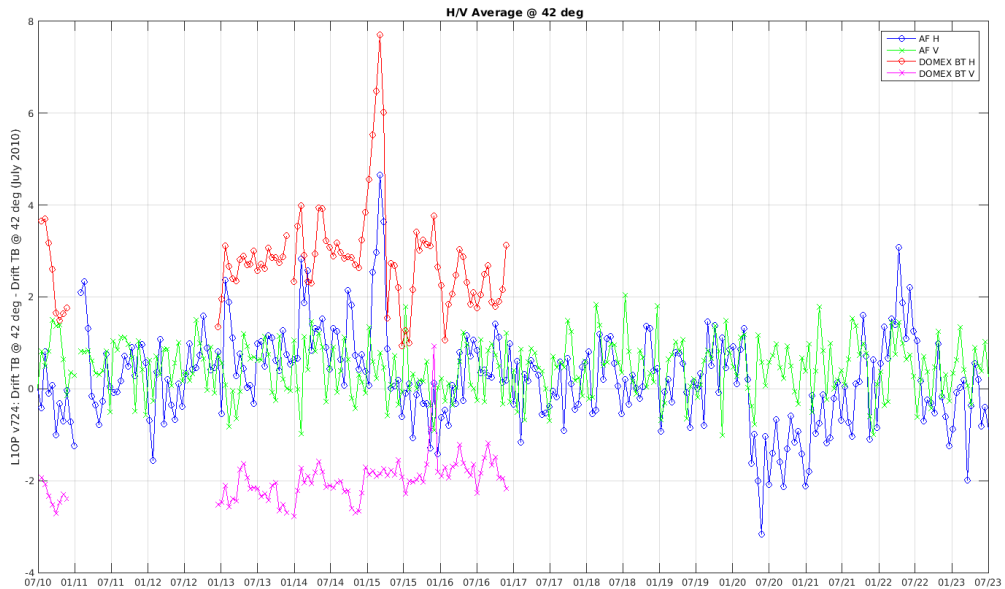
Figure 37: Dome-C H and V polarization trends in Alias Free zone (incidence angle 42°)
