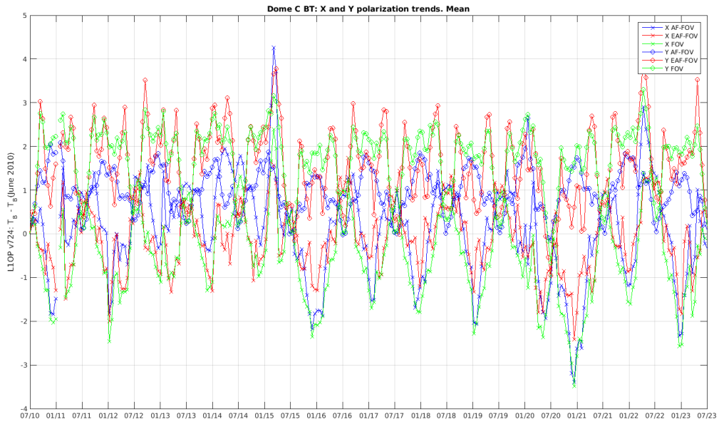
Figure 36: Dome-C X and Y polarization trends (all incidence angles).
