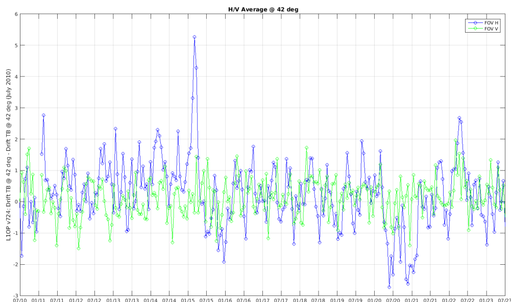
Figure 38: Dome-C H and V polarization trends in Extended Alias Free zone (incidence angle 42°)
