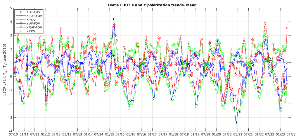
Figure 36: Dome-C X and Y polarization trends (all incidence angles).
