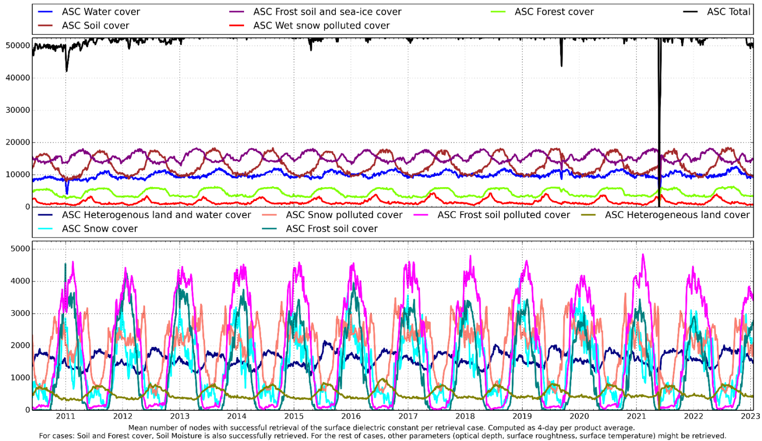
Figure 63: L2SM v700 Mean Retrievals Absolute - ASC
