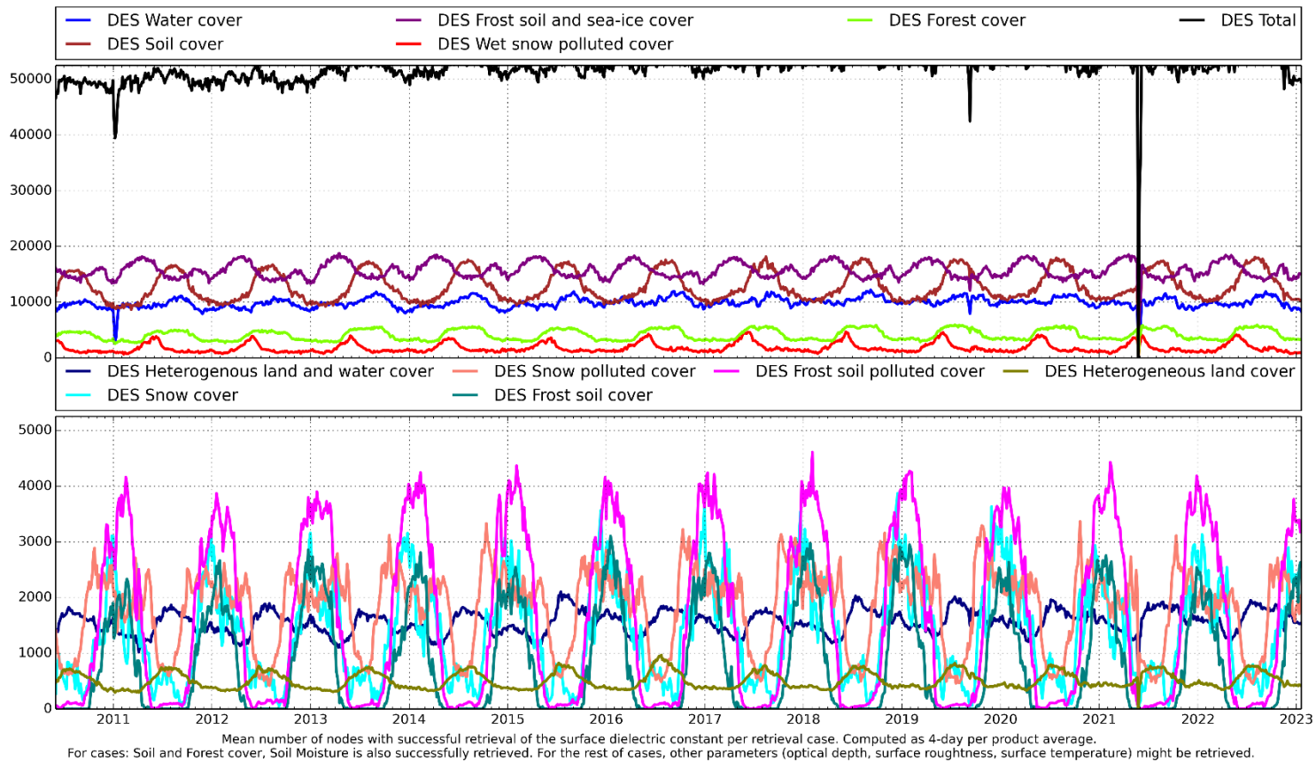
Figure 64: L2SM v700 Mean Retrievals Absolute - DES
