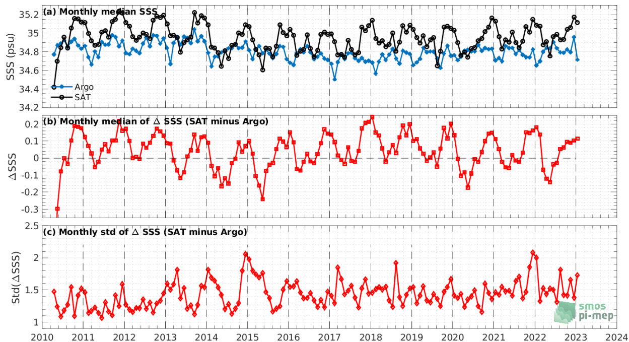
Figure 69 - Time series of the monthly median SSS (top), median of \Delta SSS (Satellite -
