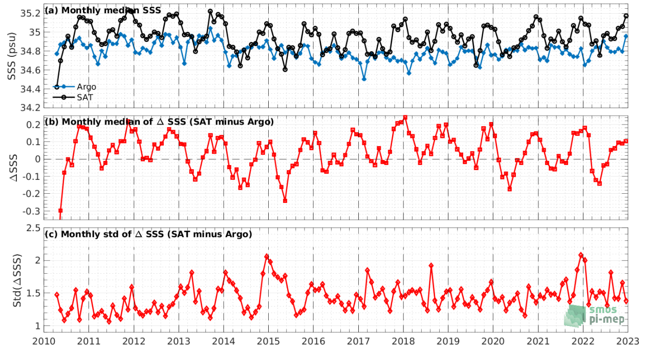
Figure 69 - Time series of the monthly median SSS (top), median of \Delta SSS (Satellite - Argo) and Std of \Delta SSS (Satellite - Argo) over the Global Ocean Pi-MEP region considering only descending orbits from all match-ups collected by the Pi-MEP.
