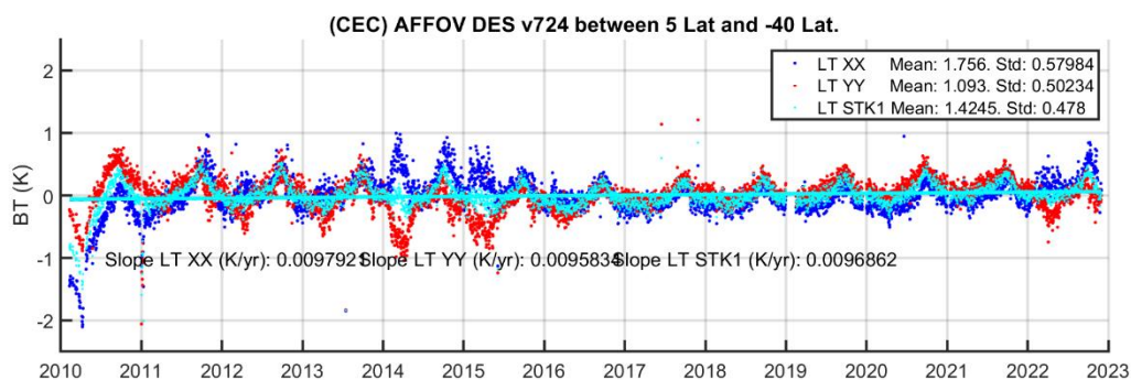
Figure 47: BT long term stability (ASC/DES), for XX and YY polarizations, and Stokes 1.
