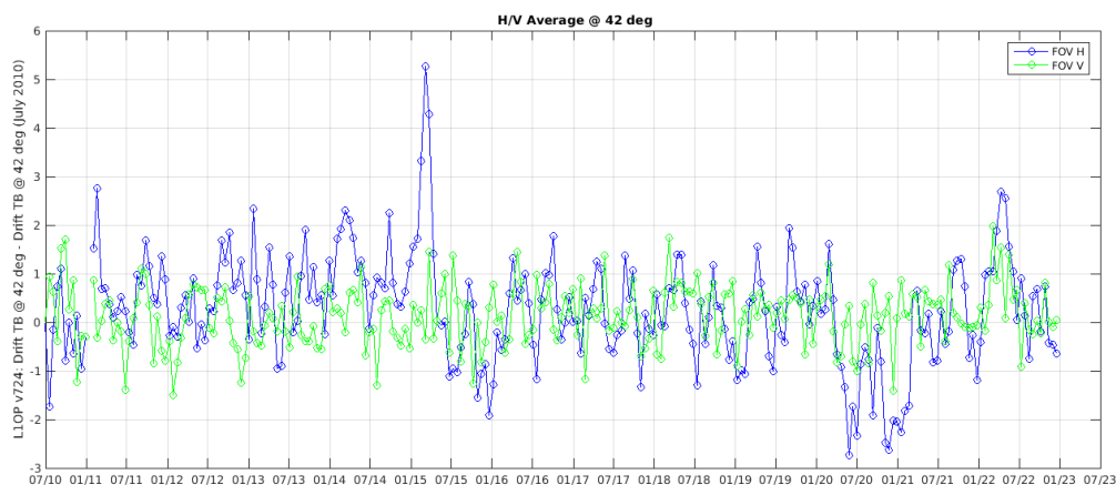
Figure 38: Dome-C H and V polarization trends in Extended Alias Free zone (incidence angle 42°)
