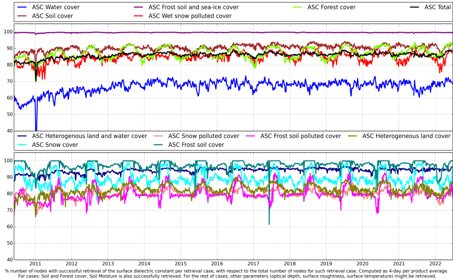
Figure 65: L2SM v700 Mean Retrievals Relative - ASC
