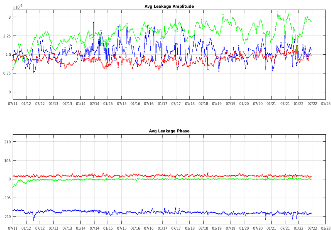
Figure 8 Leakage factor evolution in amplitude and phase of NIR AB (blue), NIR BC (green) and NIR CA (red) since the beginning of the mission
