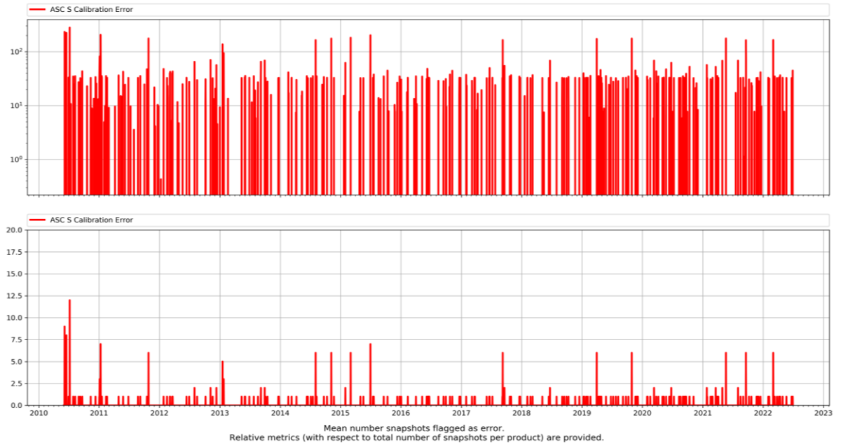
Figure 54: L1C V724 Calibration Errors Ascending Orbits
