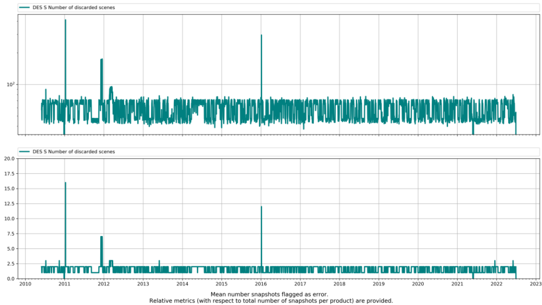
Figure 59: L1C V724 Discarded Scenes Descending Orbits
