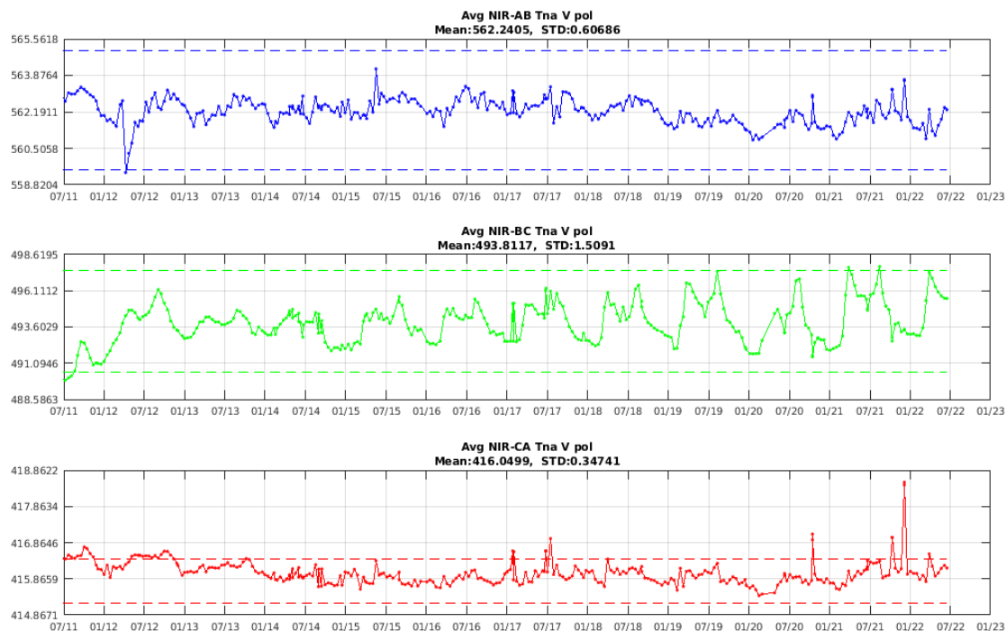
Figure 2 Tna evolution of NIR AB (blue), NIR BC (green) and NIR CA (red) in the V-channel since the beginning of the mission. Thresholds in dashed lines
