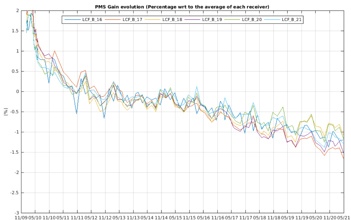
Figure 16 Evolution of the \Delta PMS Gain of the LICEFS in CMN B3
