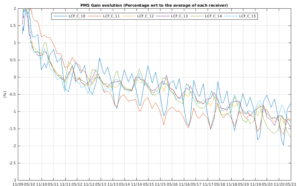
Figure 19 Evolution of the \Delta PMS Gain of the LICEFS in CMN C2
