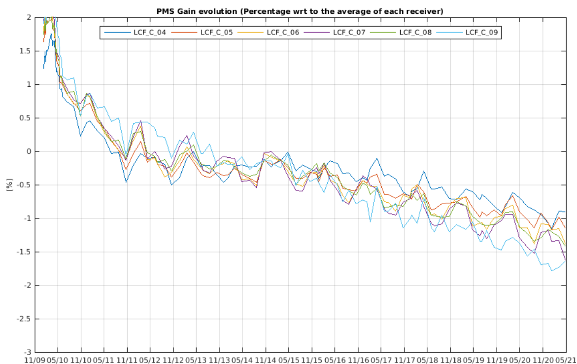
Figure 18 Evolution of the \Delta PMS Gain of the LICEFS in CMN C1
