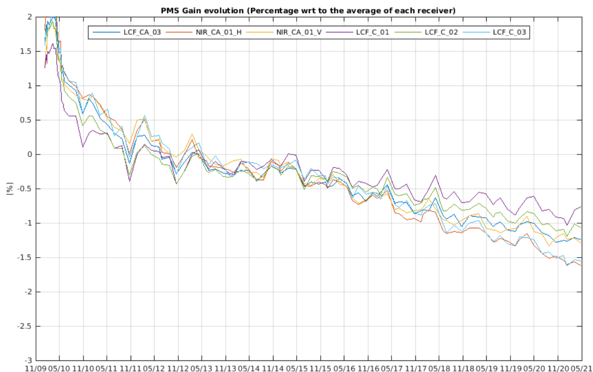
Figure 17 Evolution of the \Delta PMS Gain of the LICEFS in CMN H3
