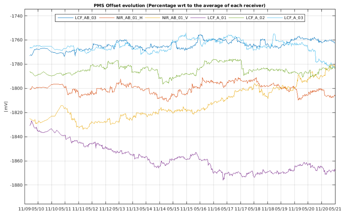
Figure 21 Evolution of the \Delta PMS Offset of the LICEFS in CMN H1
