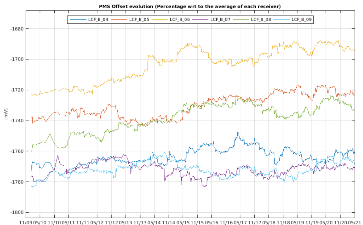
Figure 26 Evolution of the \Delta PMS Offset of the LICEFS in CMN B1
