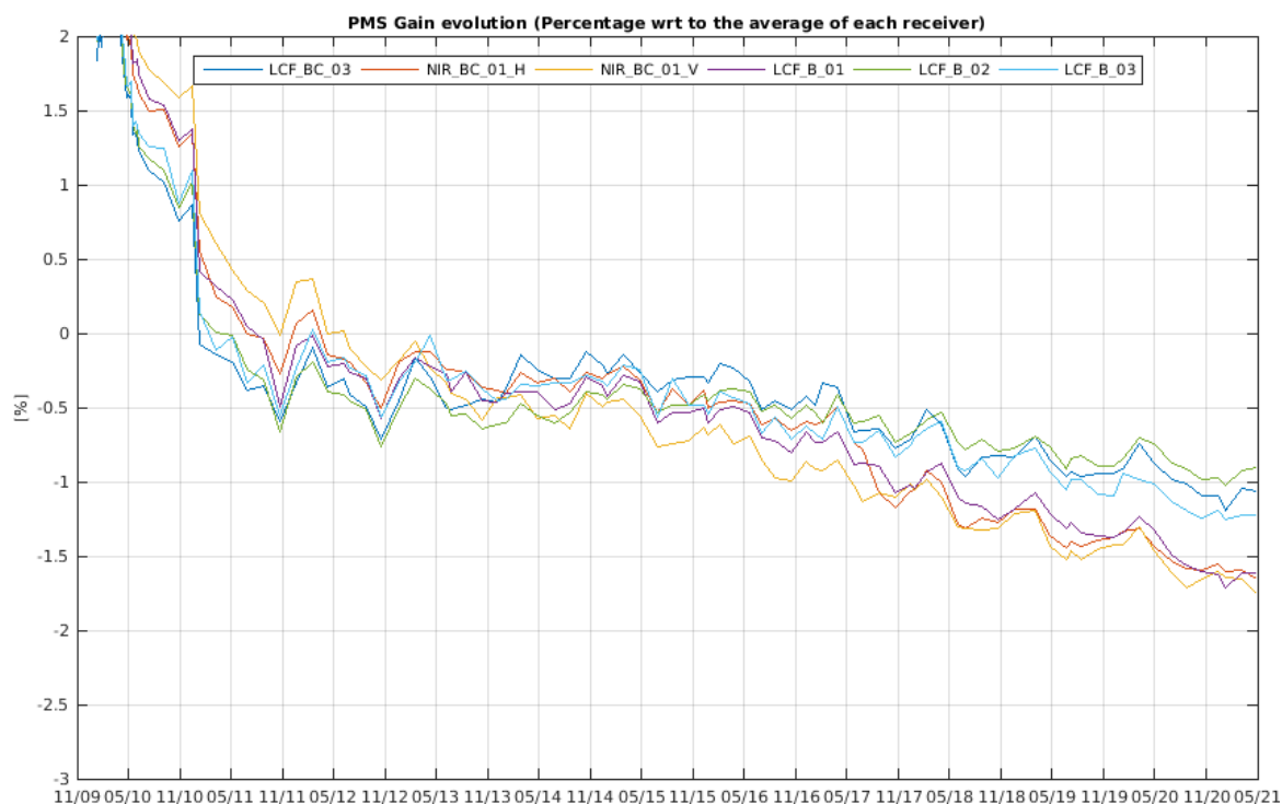
Figure 13 Evolution of the \Delta PMS Gain of the LICEFS in CMN H2
