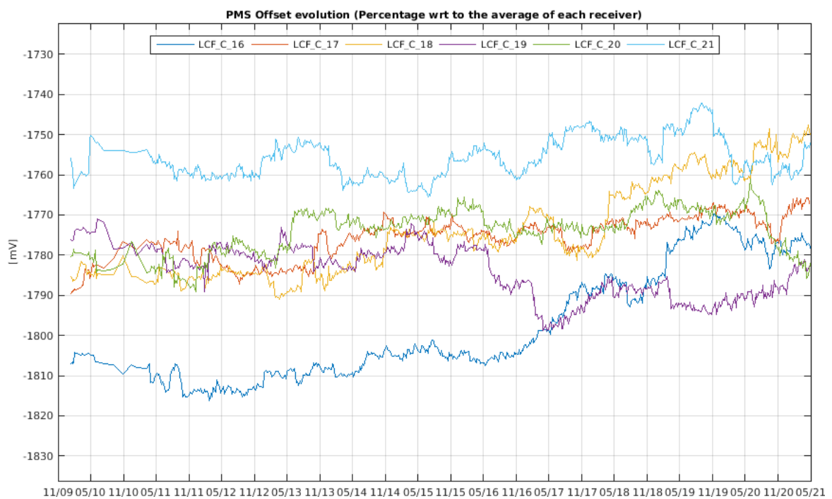
Figure 32 Evolution of the \Delta PMS Offset of the LICEFS in CMN C3
