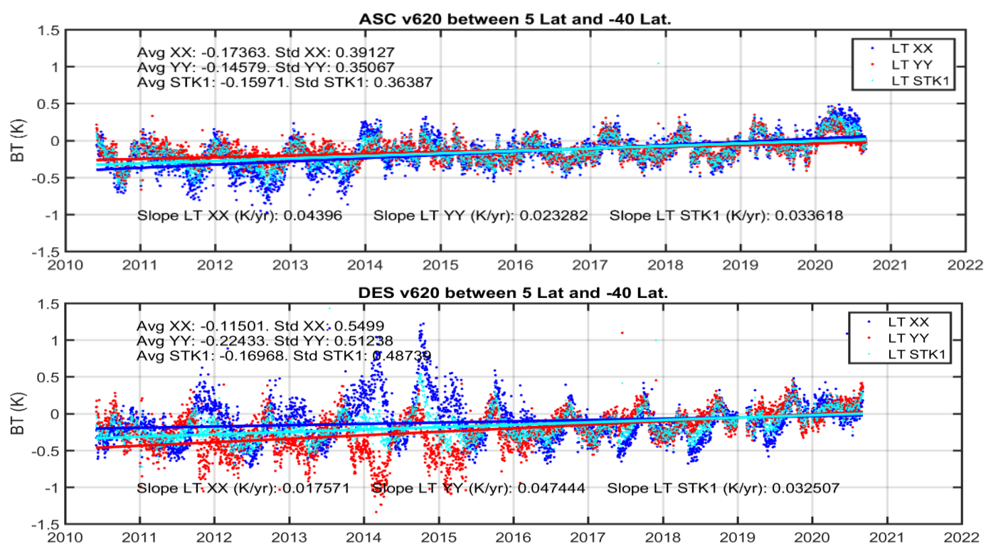
Figure 47: BT long term stability (ASC/DES), for XX and YY polarizations, and Stokes 1.
