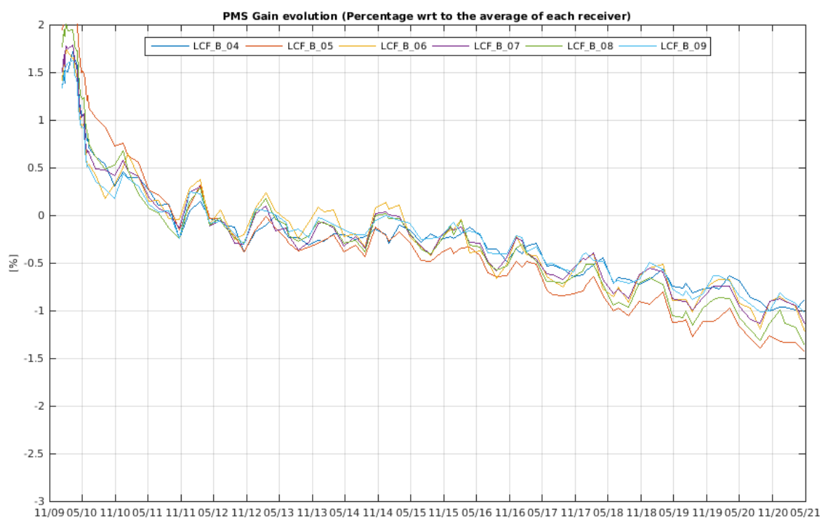
Figure 14 Evolution of the \Delta PMS Gain of the LICEFS in CMN B1
