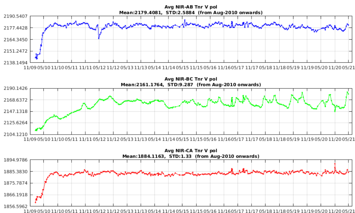
Figure 4 Tnr evolution of NIR AB (blue), NIR BC (green) and NIR CA (red) in the V-channel since the beginning of the mission.
