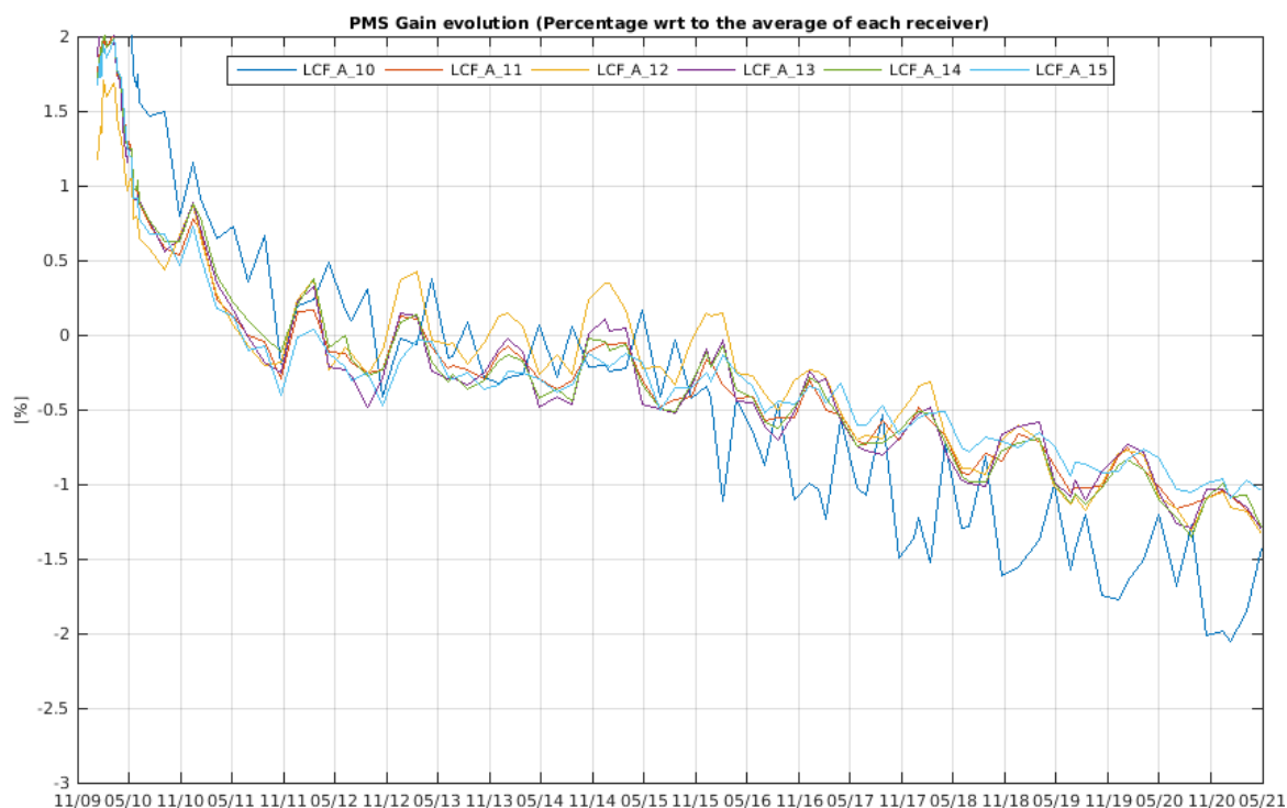
Figure 11 Evolution of the \Delta PMS Gain of the LICEFS in CMN A2
