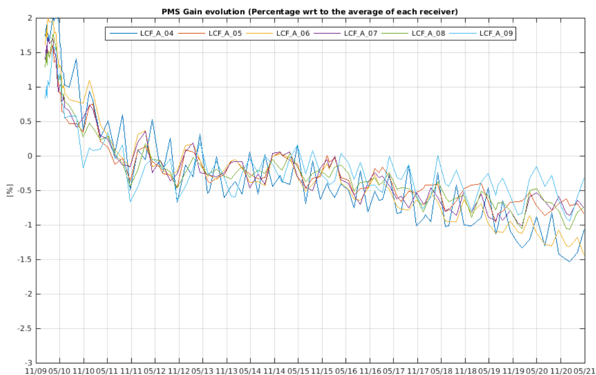
Figure 10 Evolution of the \Delta PMS Gain of the LICEFS in CMN A1
