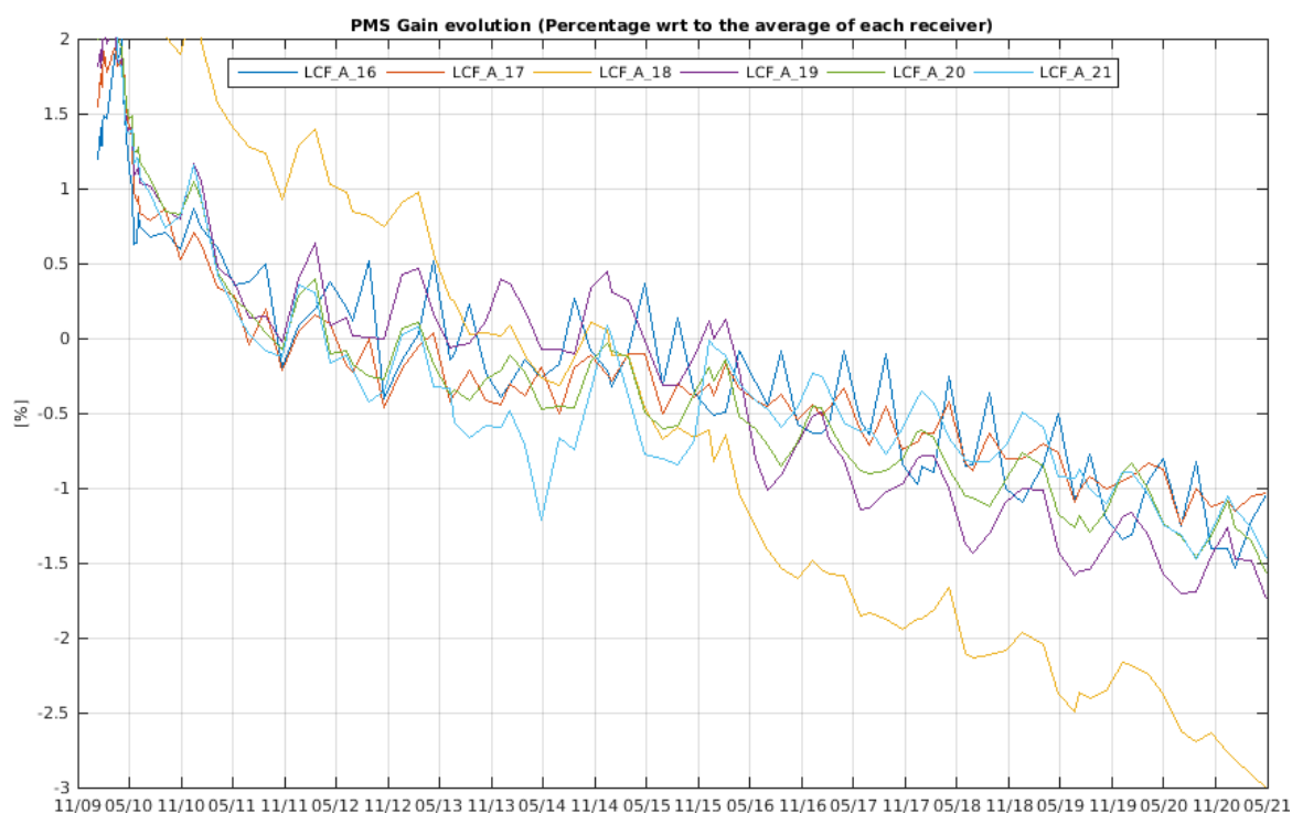
Figure 12 Evolution of the \Delta PMS Gain of the LICEFS in CMN A3
