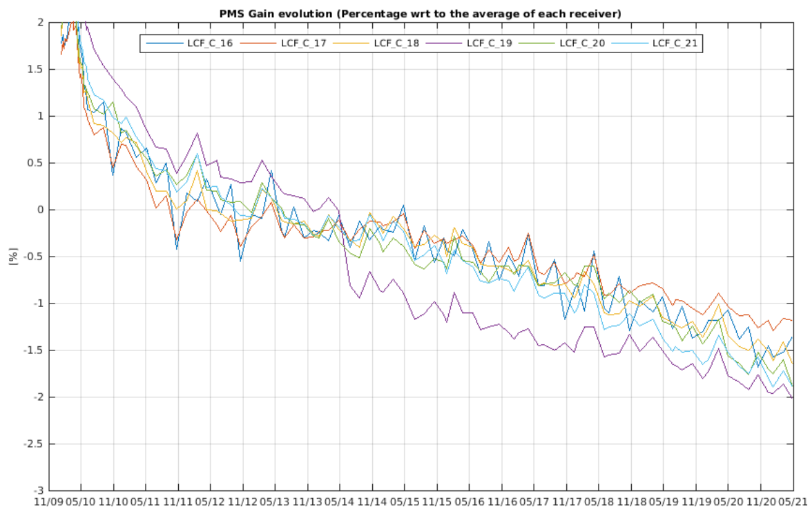
Figure 20 Evolution of the \Delta PMS Gain of the LICEFS in CMN C3
