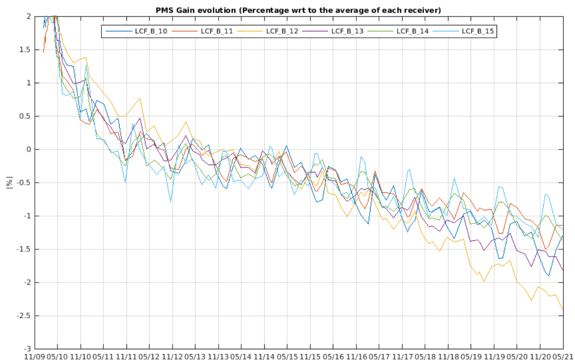
Figure 15 Evolution of the \Delta PMS Gain of the LICEFS in CMN B2
