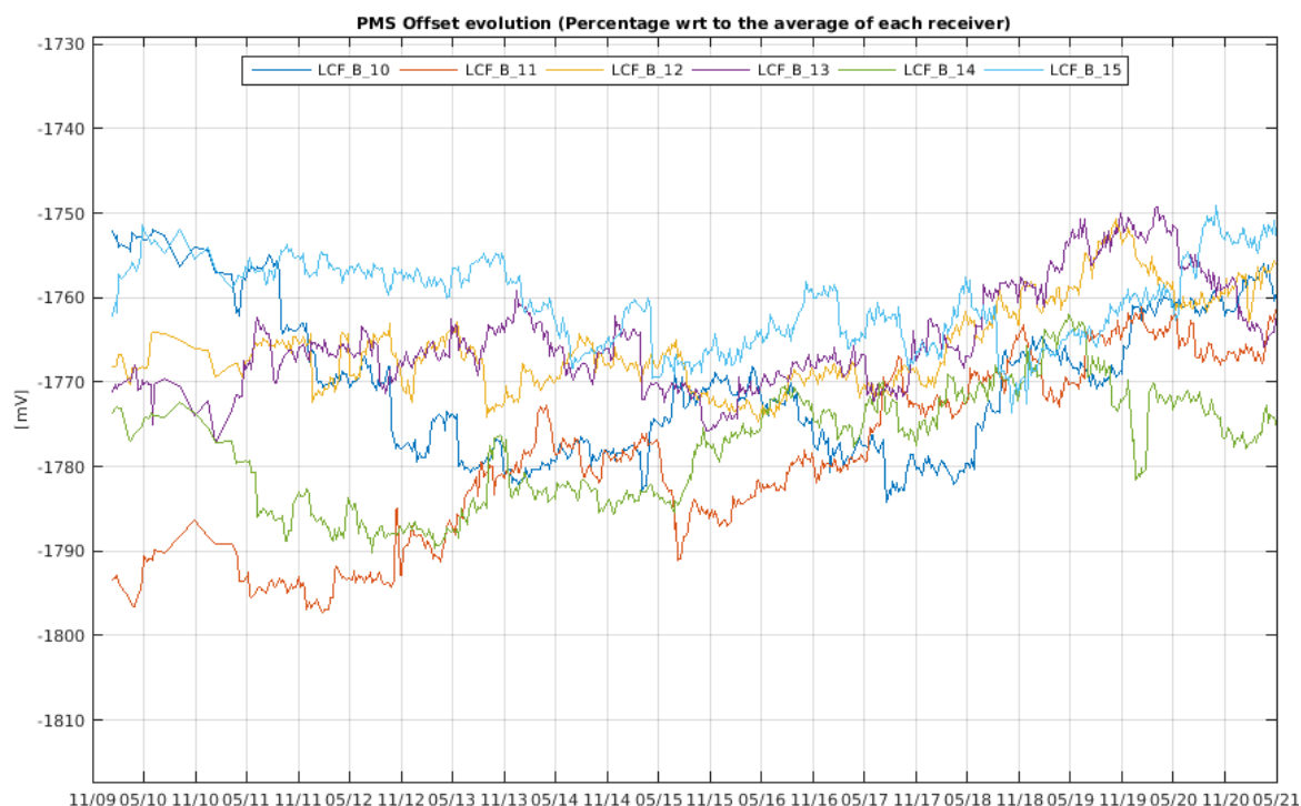
Figure 27 Evolution of the \Delta PMS Offset of the LICEFS in CMN B2
