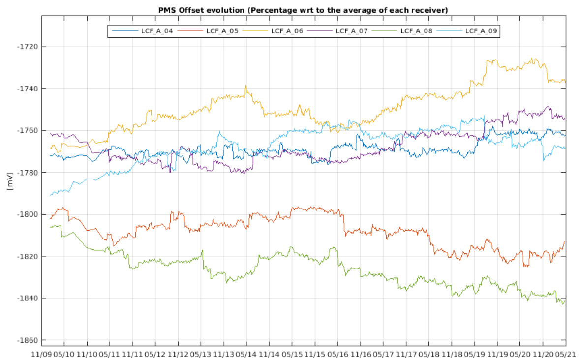
Figure 22 Evolution of the \Delta PMS Offset of the LICEFS in CMN A1
