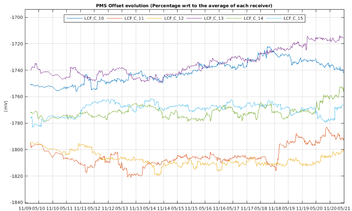
Figure 31 Evolution of the \Delta PMS Offset of the LICEFS in CMN C2
