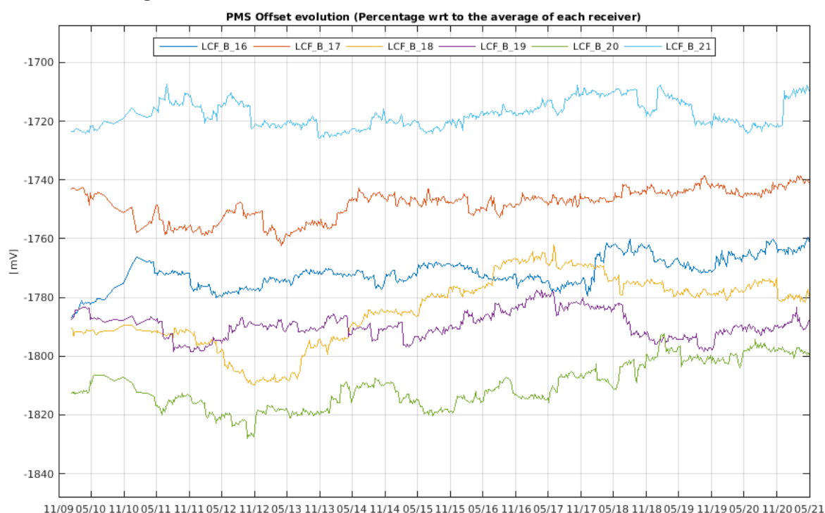
Figure 28 Evolution of the \Delta PMS Offset of the LICEFS in CMN B3
