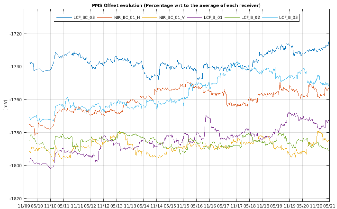
Figure 25 Evolution of the \Delta PMS Offset of the LICEFS in CMN H2
