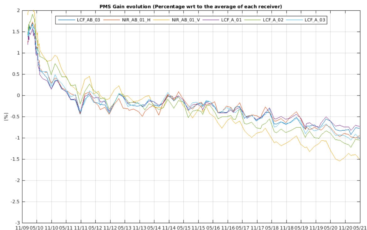
Figure 9 Evolution of the \Delta PMS Gain of the LICEFS in CMN H1
