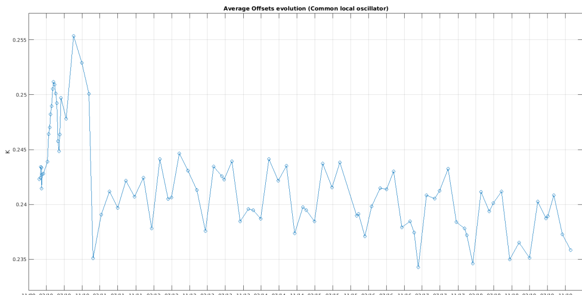
Figure 34 Evolution of the average of the Correlator offsets for the baselines which share local oscillator
