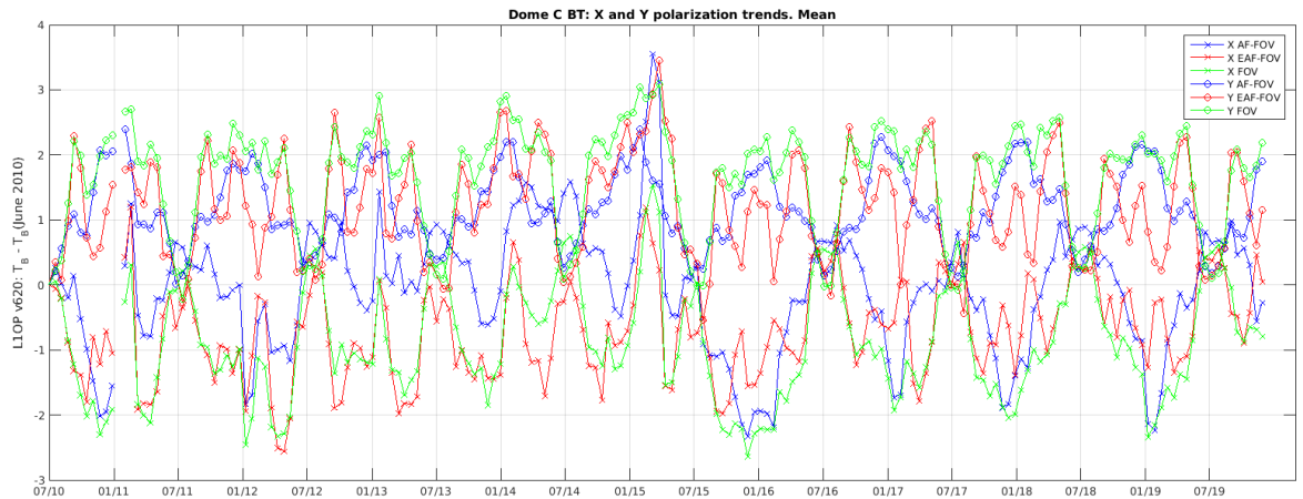
Figure 36: Dome-C X and Y polarization trends (all incidence angles)
