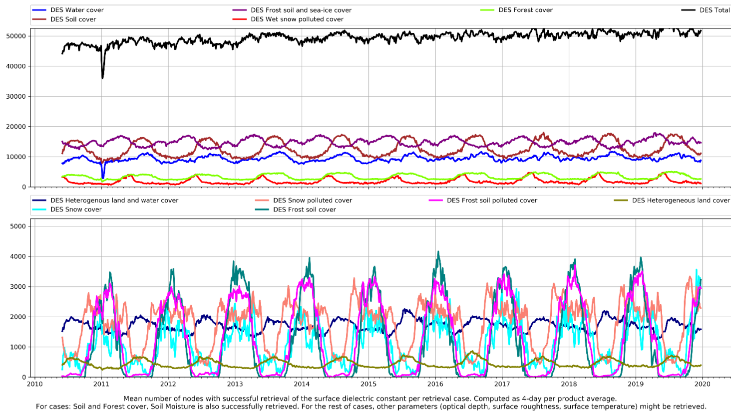
Figure 52: L2SM v650 Mean Retrievals Absolute - DES
