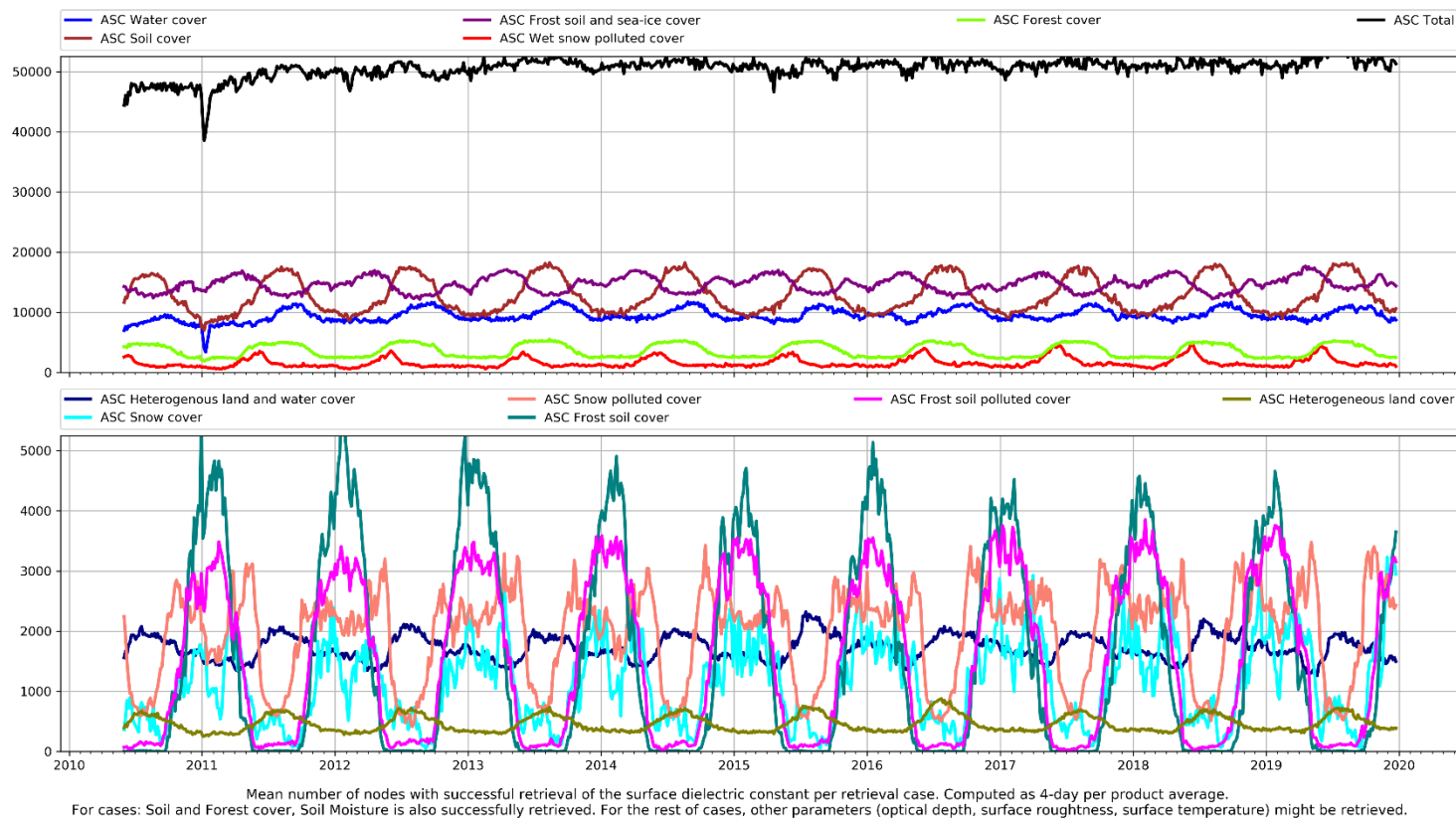
Figure 51: L2SM v650 Mean Retrievals Absolute - ASC
