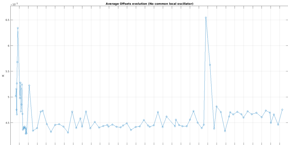
Figure 35 Evolution of the average of the Correlator offsets for the baselines which do not share local oscillator
