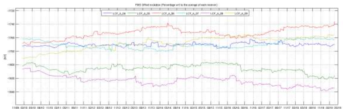
Figure 21 Evolution of the \Delta PMS Offset of the LICEFS in CMN H1
