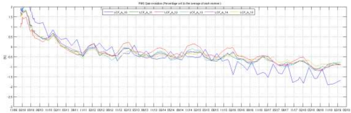
Figure 11 Evolution of the \Delta PMS Gain of the LICEFS in CMN A2
