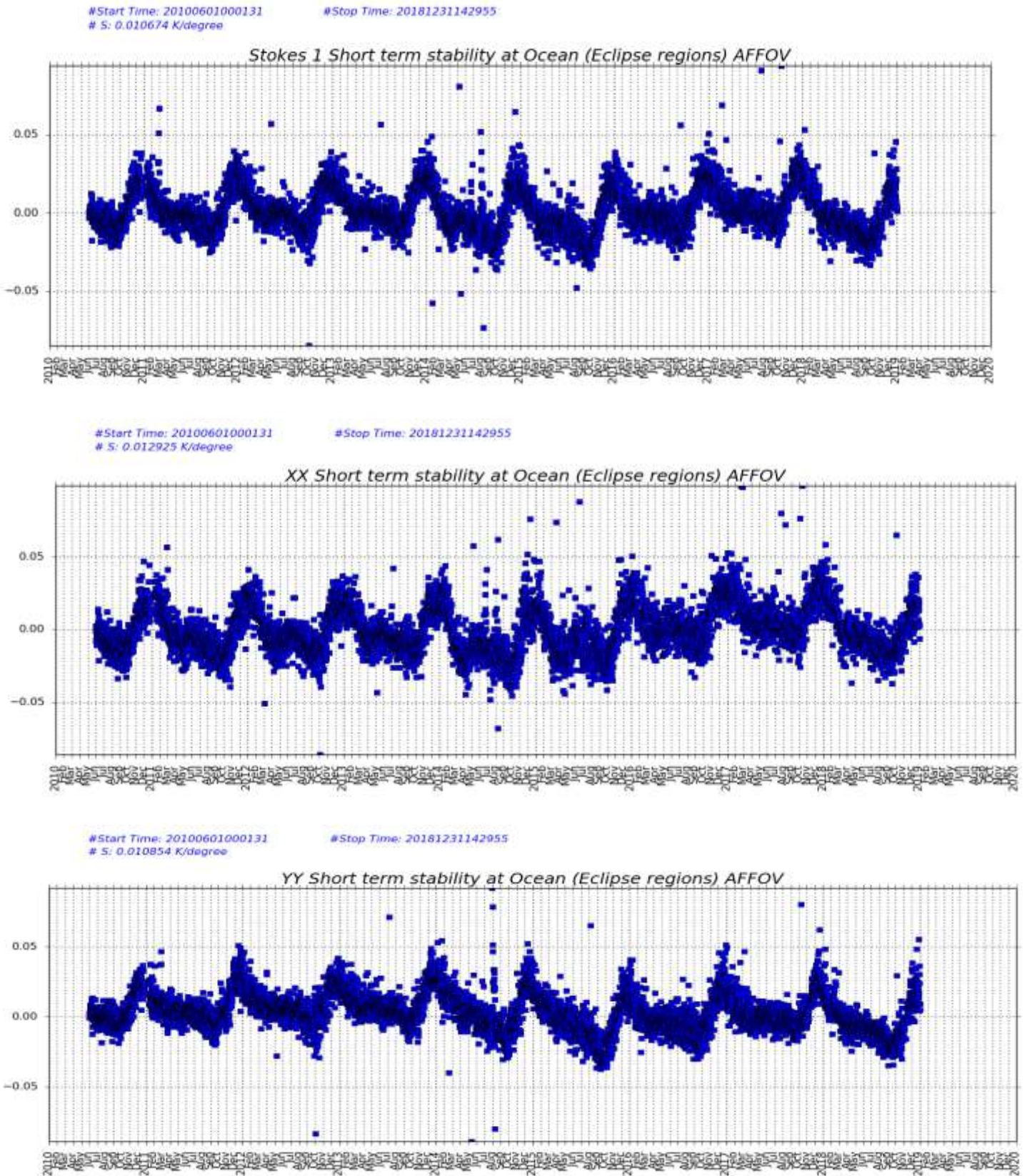
Figure 45: BT short term stability at Eclipse regions, for Stokes 1, XX and YY polarizations
