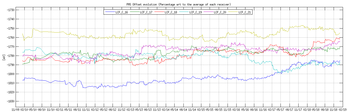
Figure 32 Evolution of the \Delta PMS Offset of the LICEFS in CMN C3
