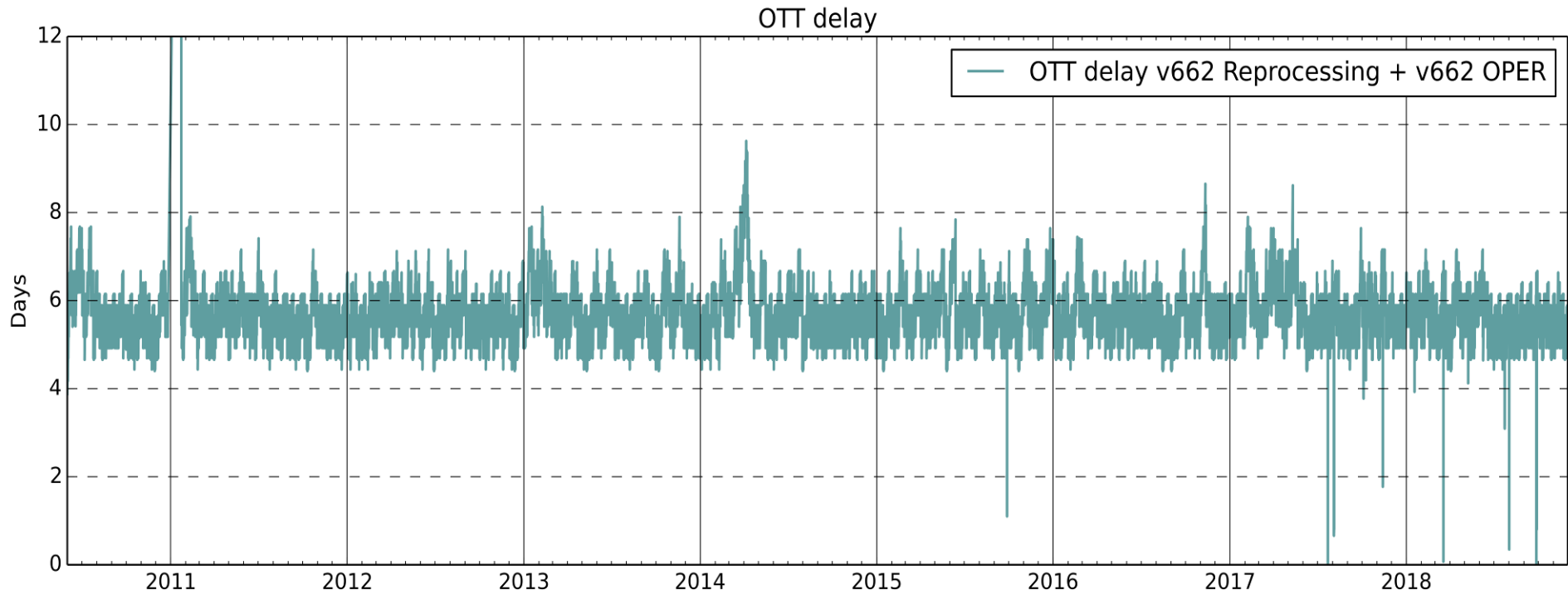
Figure 48: OTT delay per semi-orbit (Delta time between each L2OS product start time and the OTT correction validity start time file).
