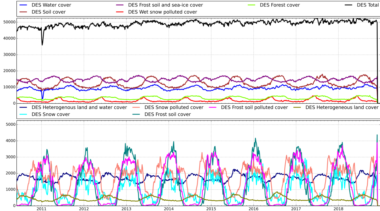
Mean number of nodes with successful retrieval of the surface dielectric constant per retrieval case. Computed as 4-day per product average. For cases: Soil and Forest cover, Soil Moisture is also successfully retrieved. For the rest of cases, other parameters (optical depth, surface roughness, surface temperature) might be retrieved.
