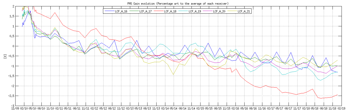
Figure 12 Evolution of the \Delta PMS Gain of the LICEFS in CMN A3
