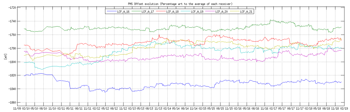
Figure 24 Evolution of the \Delta PMS Offset of the LICEFS in CMN A3
