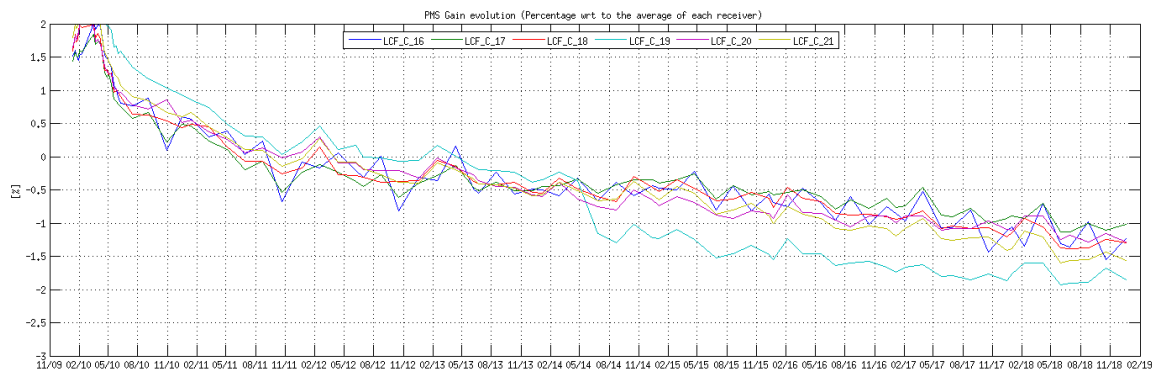
Figure 20 Evolution of the \Delta PMS Offset of the LICEFS in CMN C3
