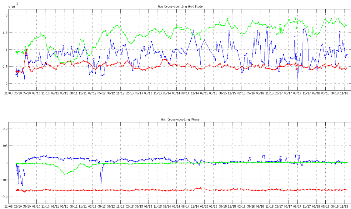
Figure 7 Cross-coupling evolution in amplitude and phase of NIR AB (blue), NIR BC (green) and NIR CA (red) since the beginning of the mission
