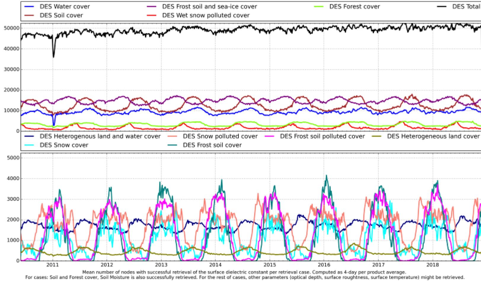
Figure 52: L2SM v650 Mean Retrievals Absolute - DES
