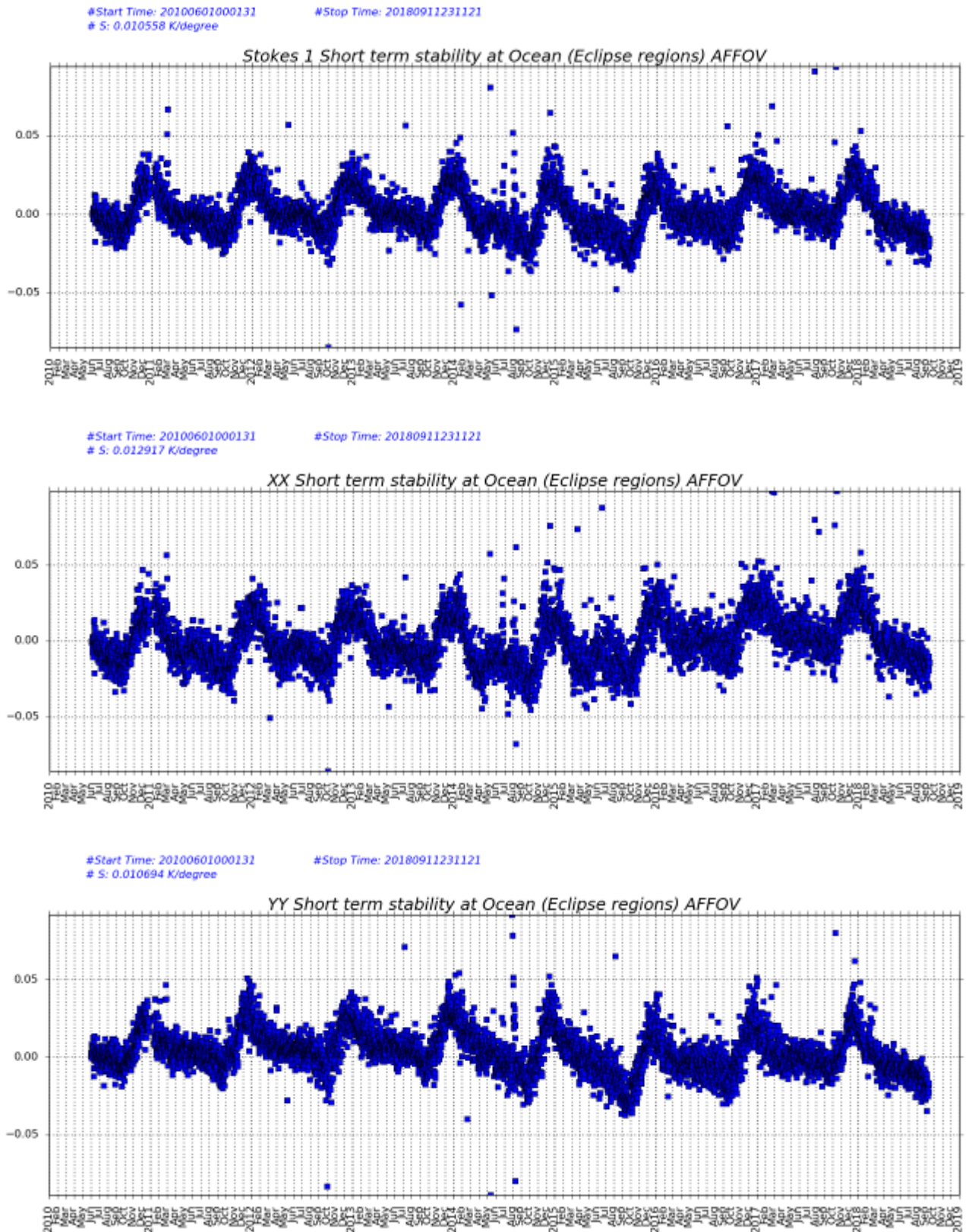
Figure 45: BT short term stability at Eclipse regions, for Stokes 1, XX and YY polarizations
