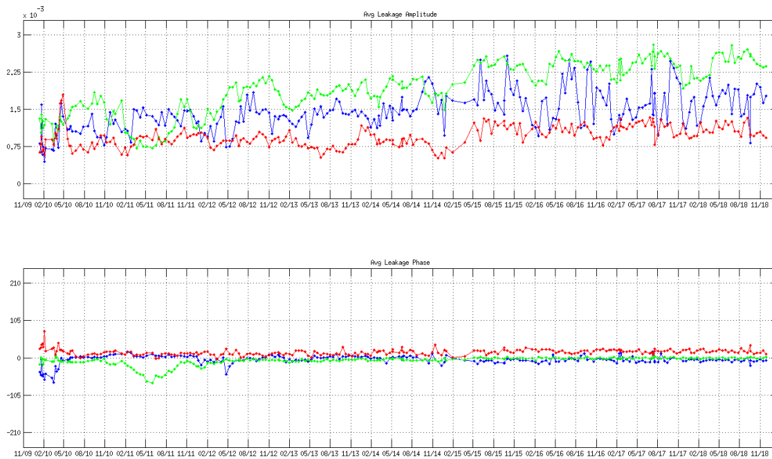
Figure 8 Leakage factor evolution in amplitude and phase of NIR AB (blue), NIR BC (green) and NIR CA (red) since the beginning of the mission
