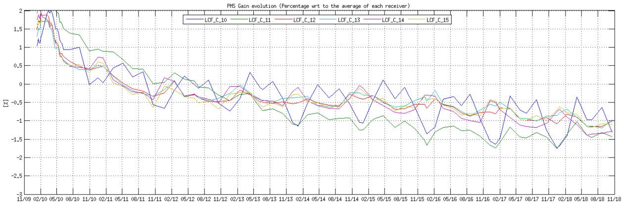
Figure 19 Evolution of the \Delta PMS Gain of the LICEFS in CMN C2
