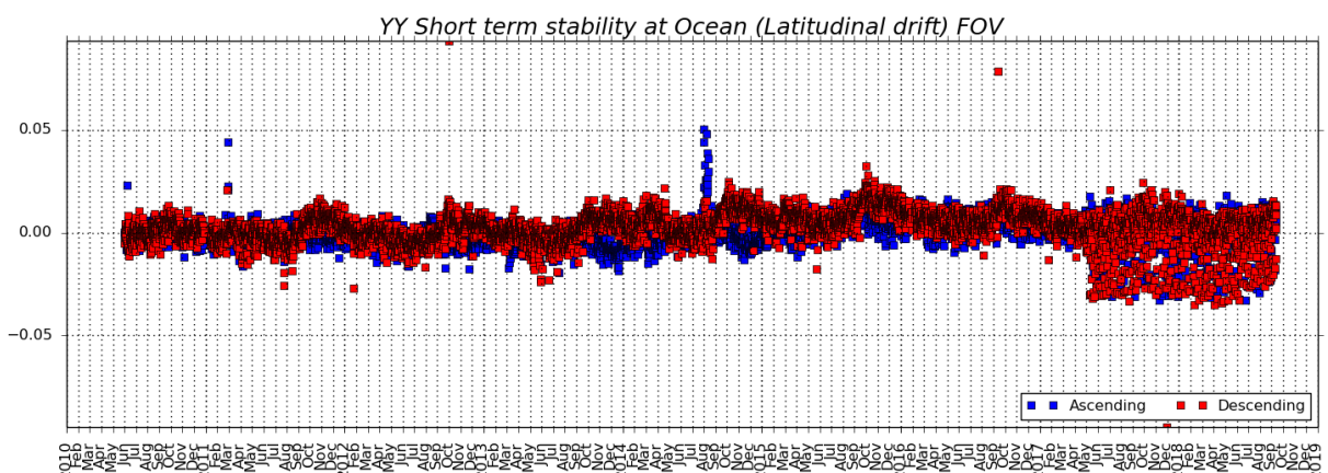
Figure 46: BT short term stability (Latitudinal drift) for Stokes 1, XX and YY polarizations.
