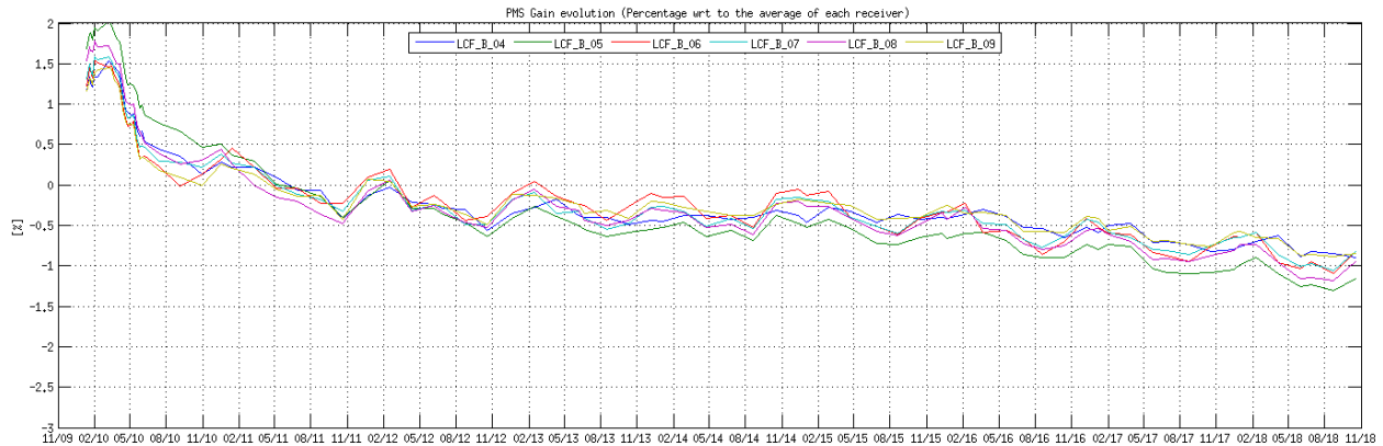
Figure 14 Evolution of the \Delta PMS Gain of the LICEFS in CMN B1
