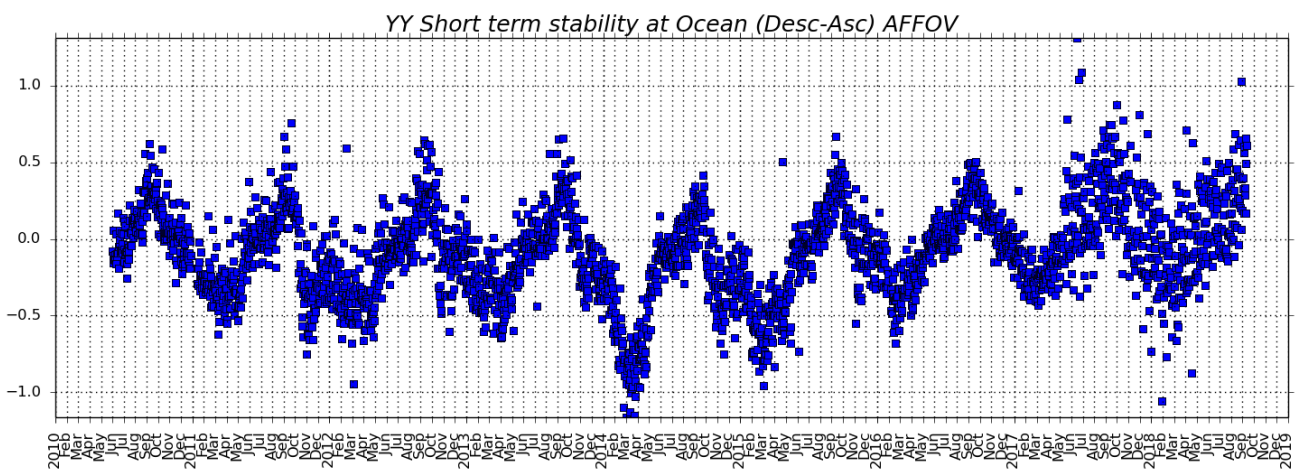
Figure 44: BT short-term stability trends (ASC-DES) for Stokes I, XX and YY polarizations
