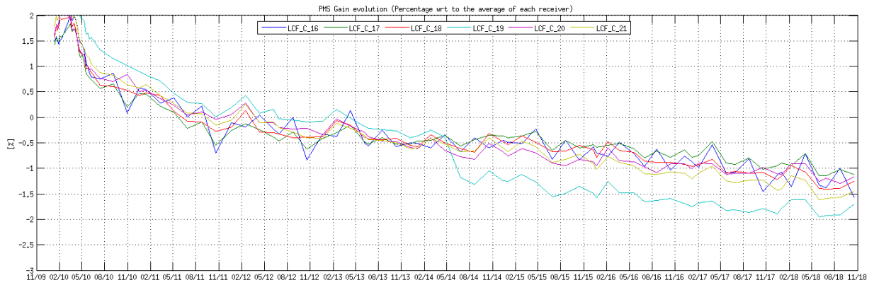
Figure 20 Evolution of the \Delta PMS Gain of the LICEFS in CMN C3
