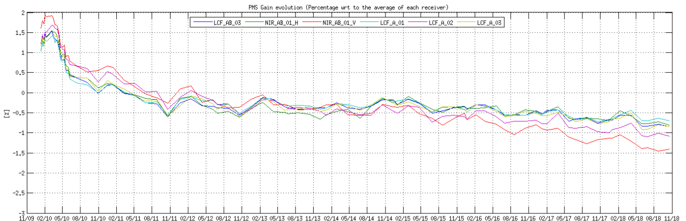
Figure 9 Evolution of the \Delta PMS Gain of the LICEFS in CMN H1
