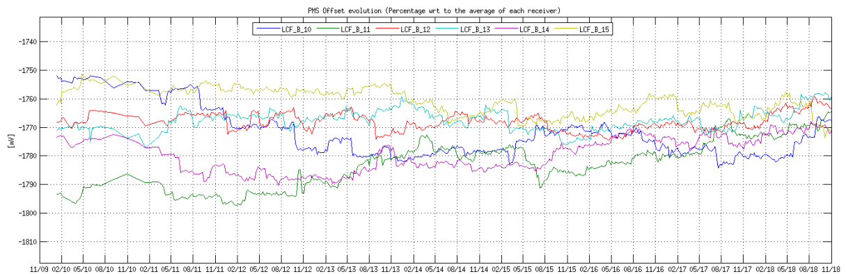
Figure 27 Evolution of the \Delta PMS Offset of the LICEFS in CMN B2
