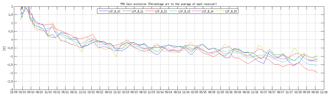
Figure 15 Evolution of the \Delta PMS Gain of the LICEFS in CMN B2
