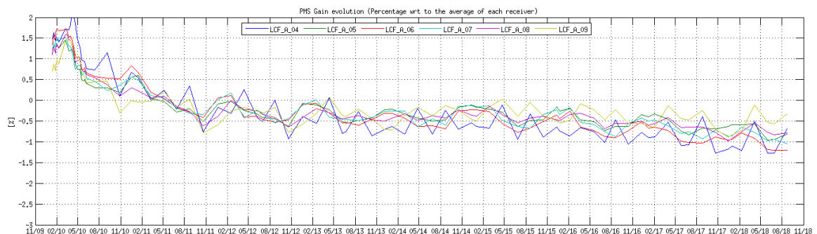
Figure 10 Evolution of the \Delta PMS Gain of the LICEFS in CMN A1
