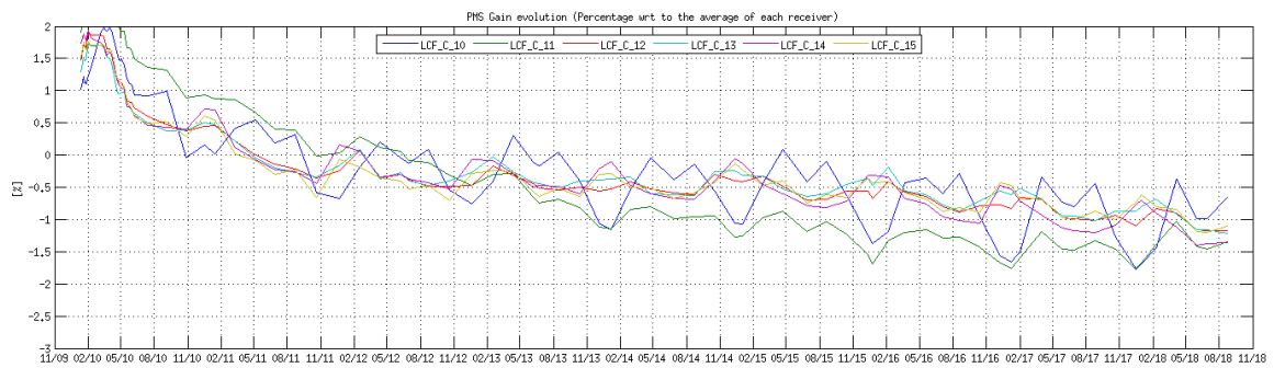
Figure 19 Evolution of the \Delta PMS Gain of the LICEFS in CMN C2
