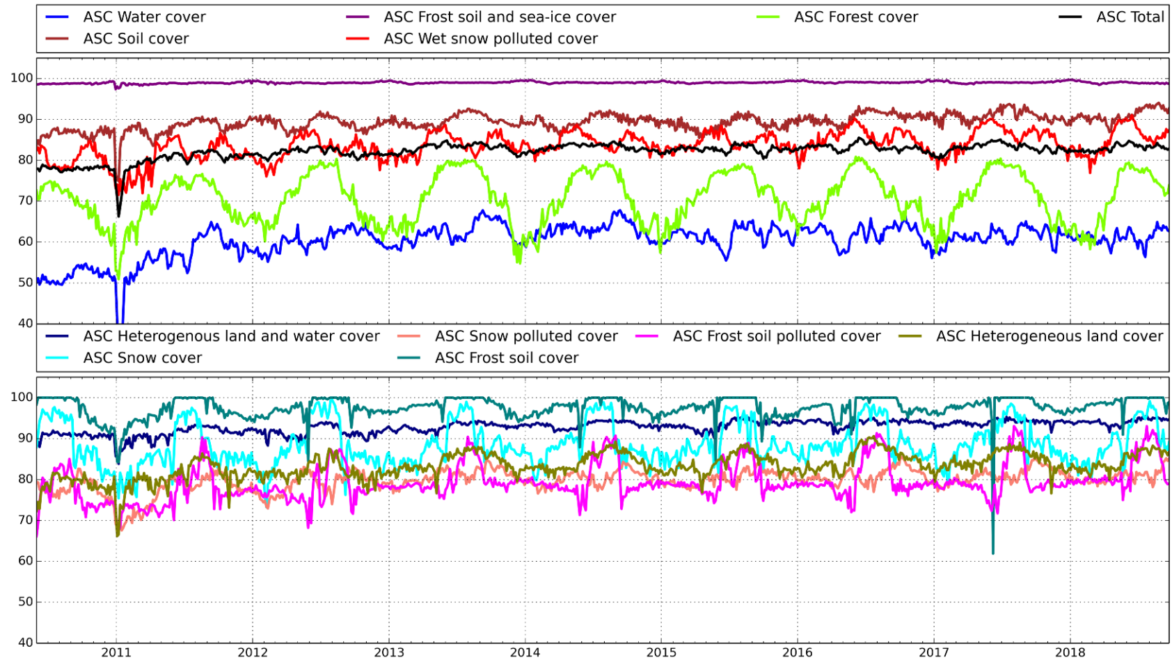
% number of nodes with successful retrieval of the surface dielectric constant per retrieval case, with respect to the total number of nodes for such retrieval case. Computed as 4-day per product average. For cases: Soil and Forest cover, Soil Moisture is also successfully retrieved. For the rest of cases, other parameters (optical depth, surface roughness, surface temperature) might be retrieved.
