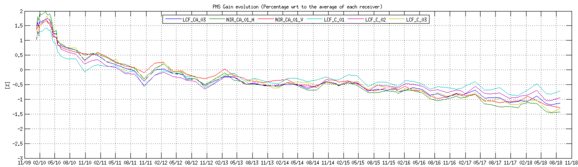
Figure 17 Evolution of the \Delta PMS Gain of the LICEFS in CMN H3
