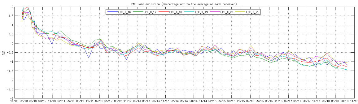
Figure 16 Evolution of the \Delta PMS Gain of the LICEFS in CMN B3
