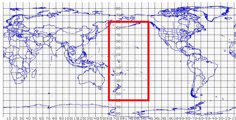
Figure 39: Open ocean region used for the Hovmoller computation.
