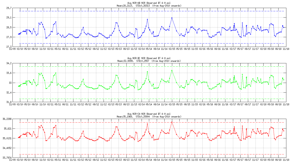
Figure 5 NIR Observed BT evolution of NIR AB (blue), NIR BC (green) and NIR CA (red) in the H-channel since the beginning of the mission. Thresholds in dashed lines
