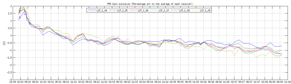
Figure 18 Evolution of the \Delta PMS Gain of the LICEFS in CMN C1
