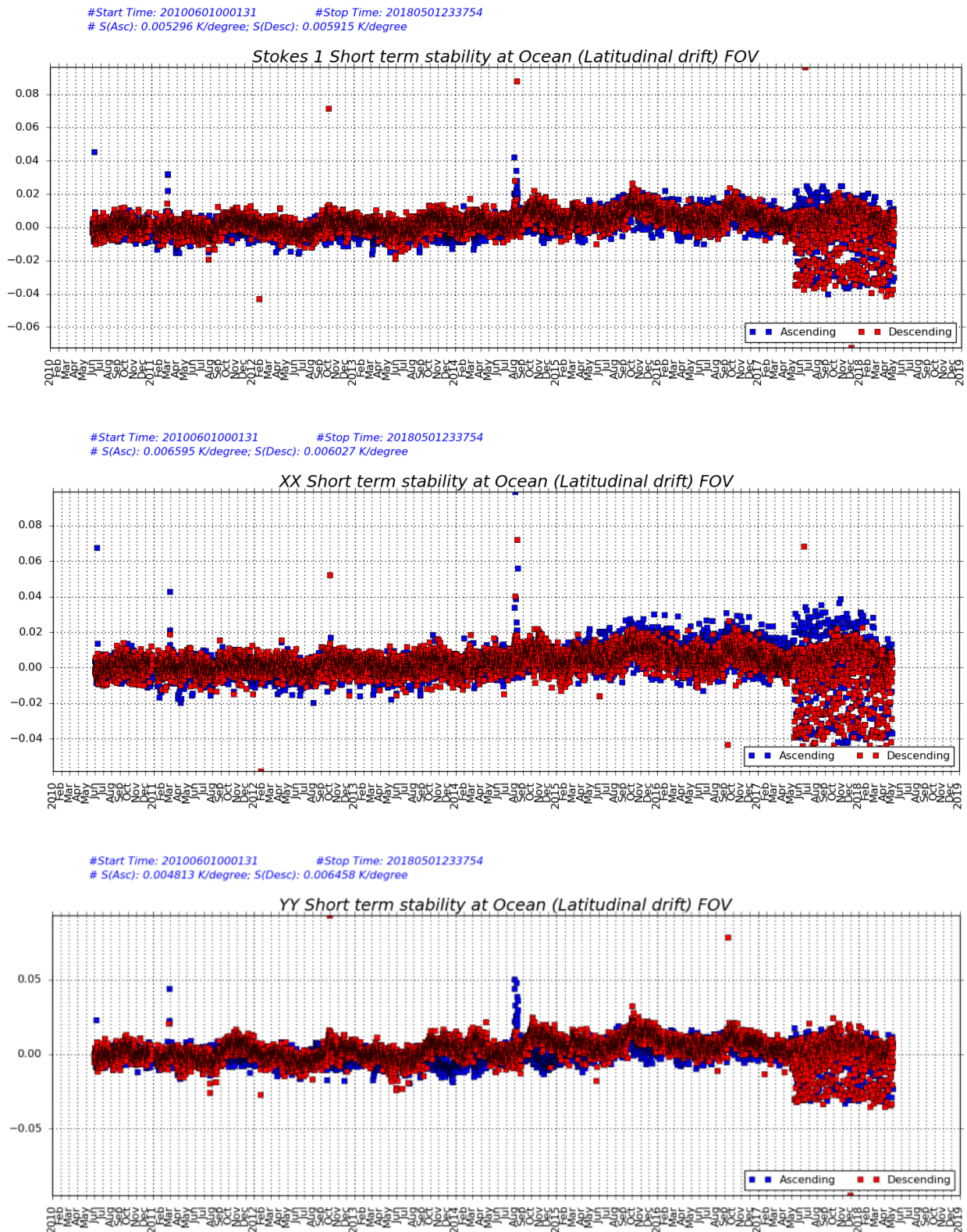
Figure 46: BT short term stability (Latitudinal drift) for Stokes 1, XX and YY polarizations.
