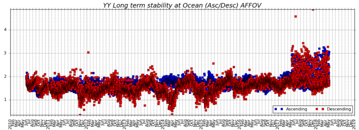
Figure 47: BT long term stability (ASC/DES), for XX and YY polarizations.
