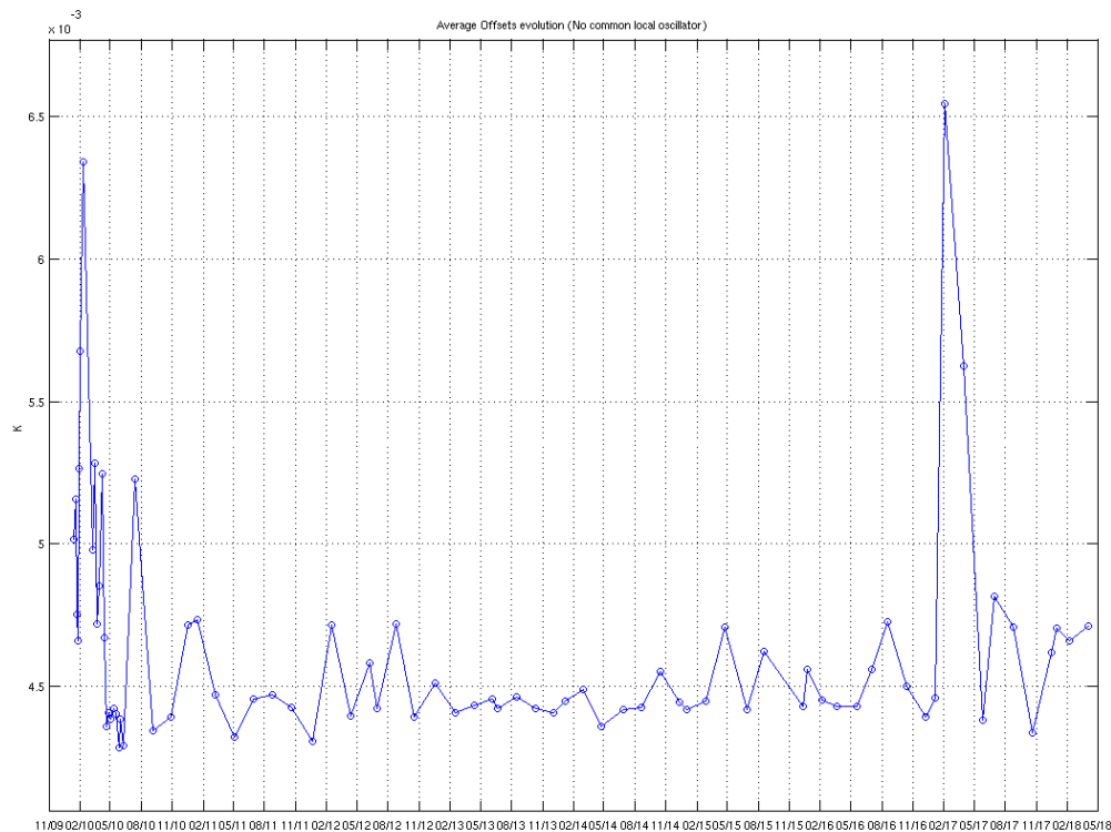
Figure 35 Evolution of the average of the Correlator offsets for the baselines which do not share local oscillator
