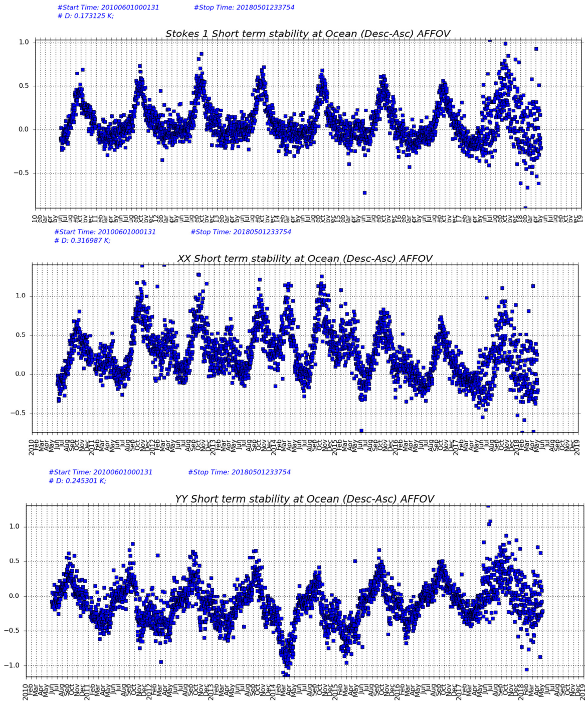
Figure 44: BT short-term stability trends (ASC-DES) for Stokes 1, XX and YY polarizations
