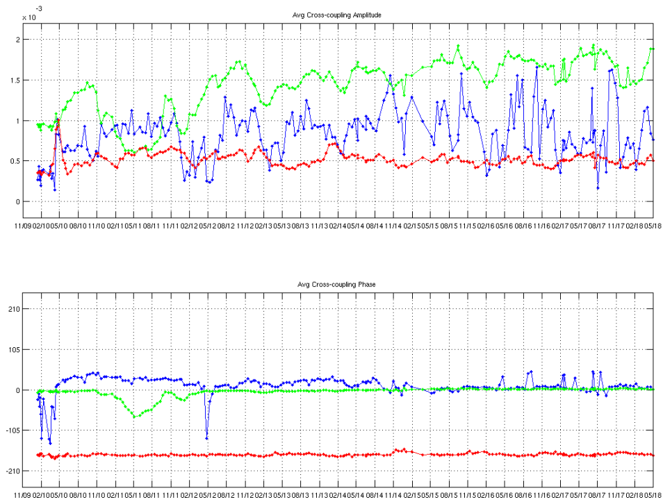
Figure 8 Leakage factor evolution in amplitude and phase of NIR AB (blue), NIR BC (green) and NIR CA (red) since the beginning of the mission
