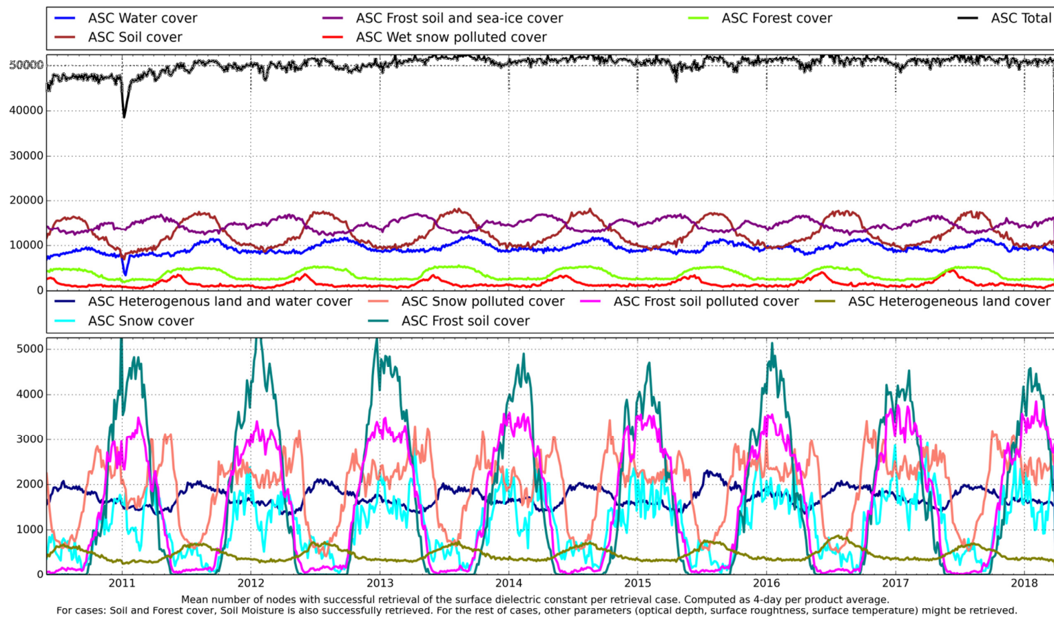
Figure 51: L2SM v650 Mean Retrievals Absolute - ASC
