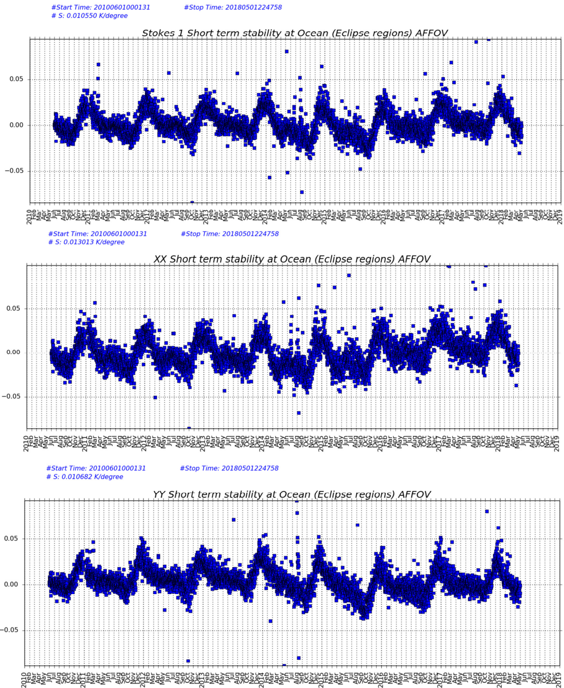
Figure 45: BT short term stability at Eclipse regions, for Stokes 1, XX and YY polarizations
