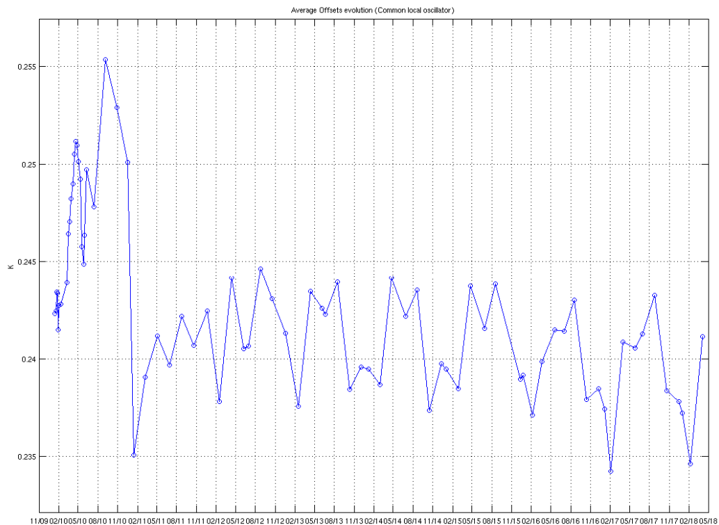
Figure 34 Evolution of the average of the Correlator offsets for the baselines which share local oscillator
