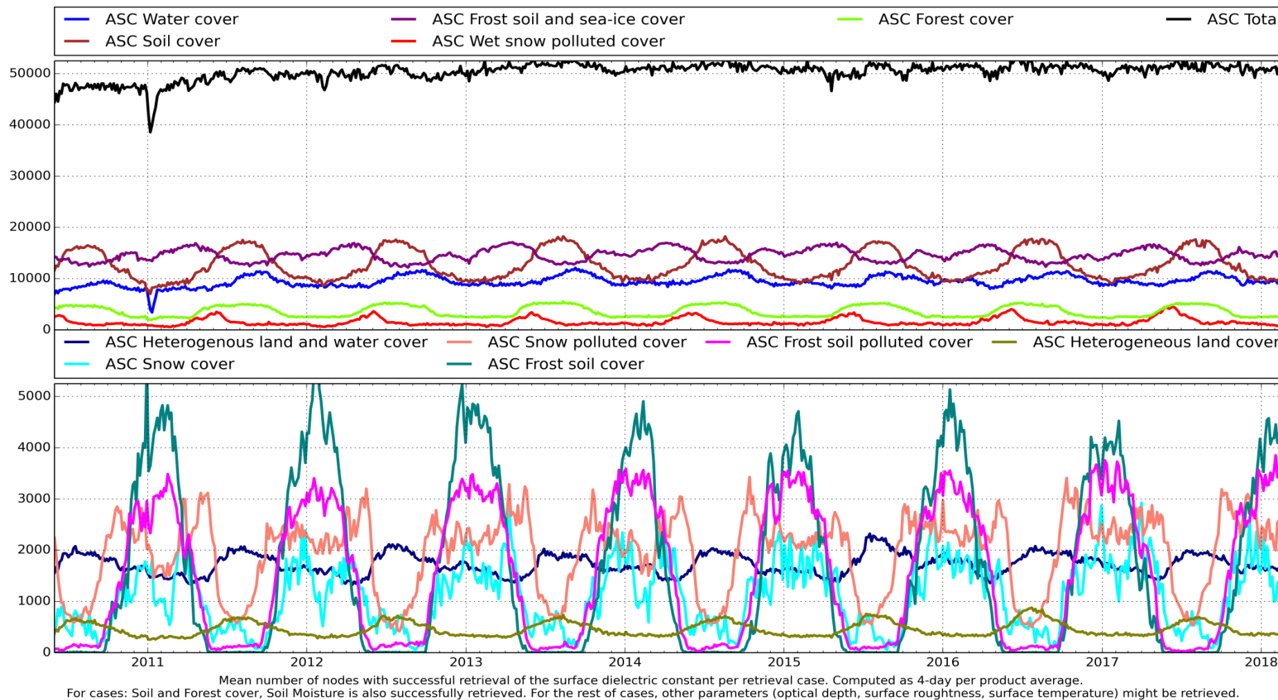
Figure 51: L2SM v650 Mean Retrievals Absolute - ASC
