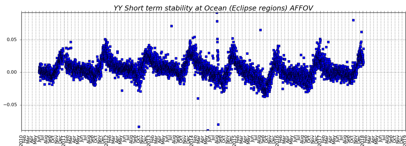
Figure 45: BT short term stability at Eclipse regions, for Stokes 1, XX and YY polarizations
