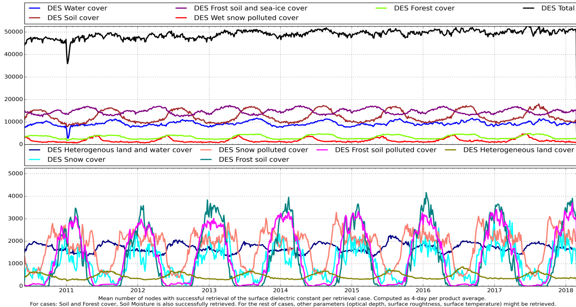
Figure 52: L2SM v650 Mean Retrievals Absolute - DES
