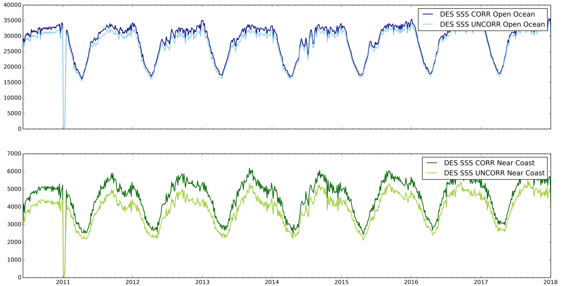
Figure 41: DES Open Ocean and Near Coast L2OS Good Quality Retrievals
