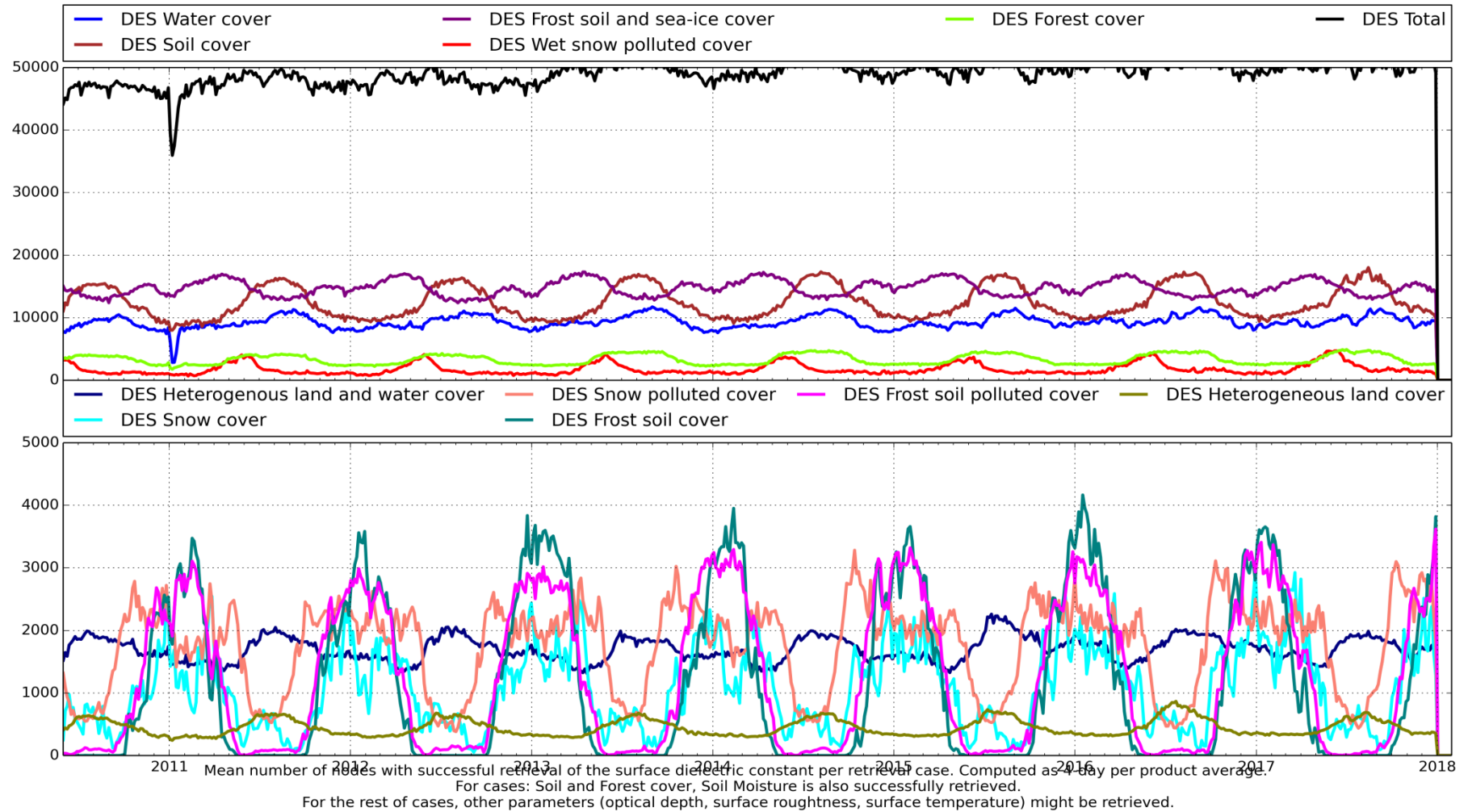
Figure 43: L2SM v650 Mean Retrievals Absolute - DES
