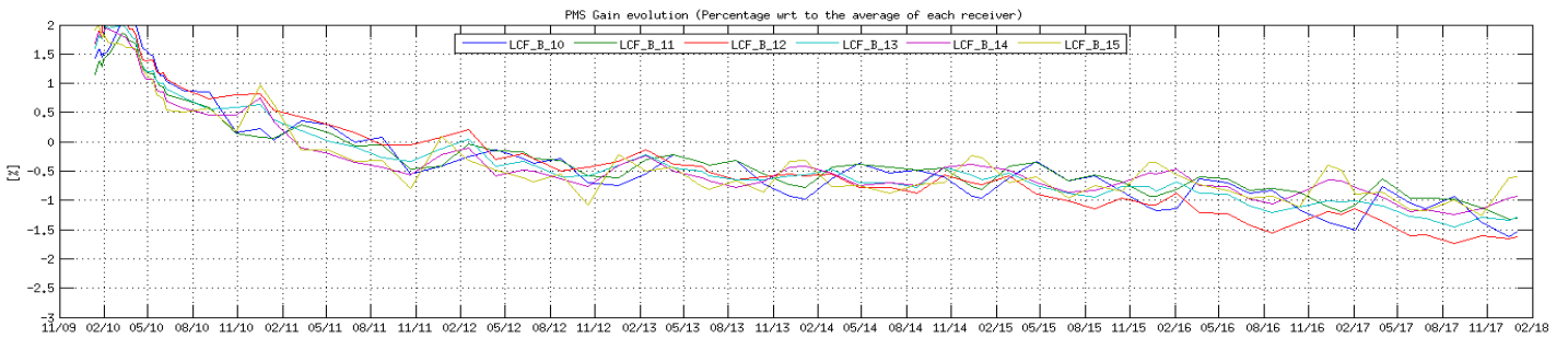
Figure 15 Evolution of the \Delta PMS Gain of the LICEFS in CMN B2
