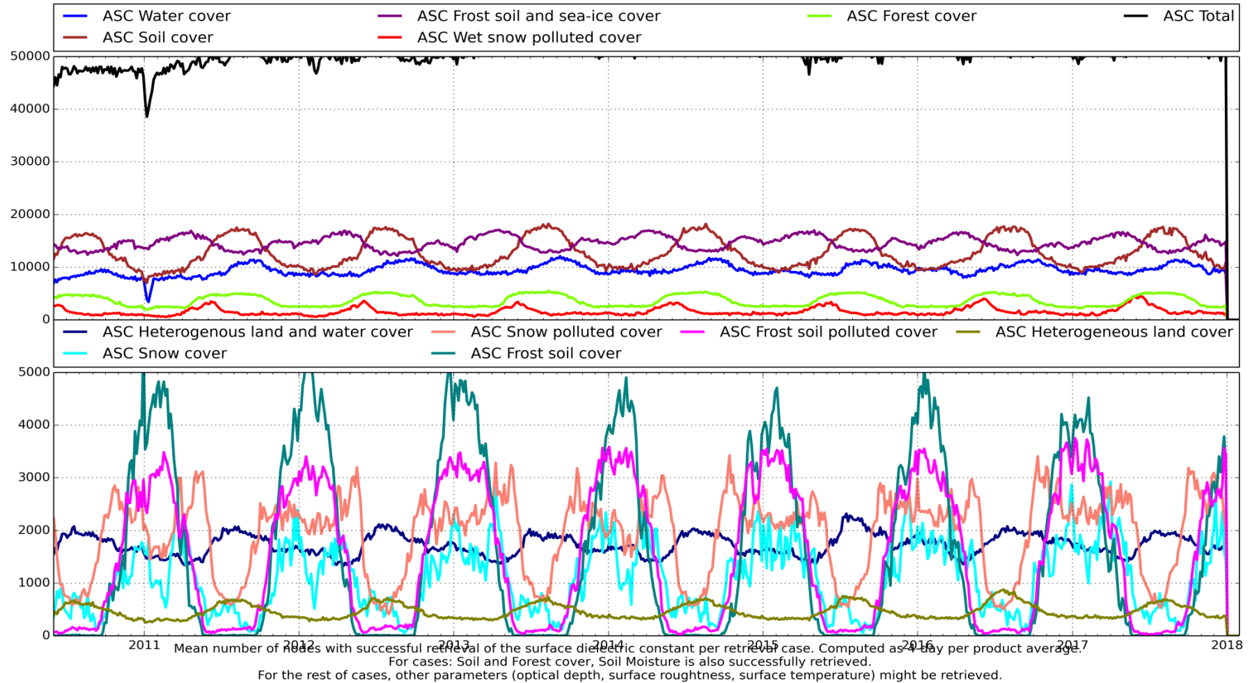
Figure 42: L2SM v650 Mean Retrievals Absolute - ASC
