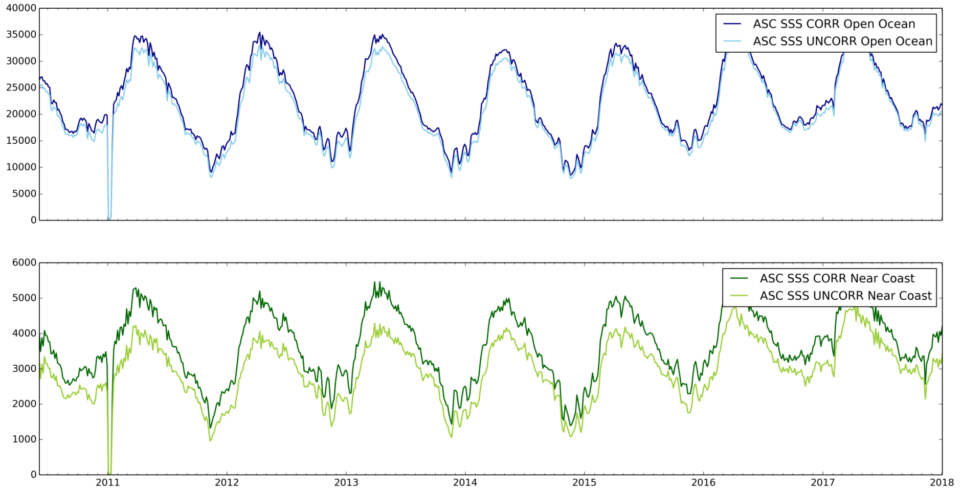
Figure 40: ASC Open Ocean and Near Coast L2OS Good Quality Retrievals
