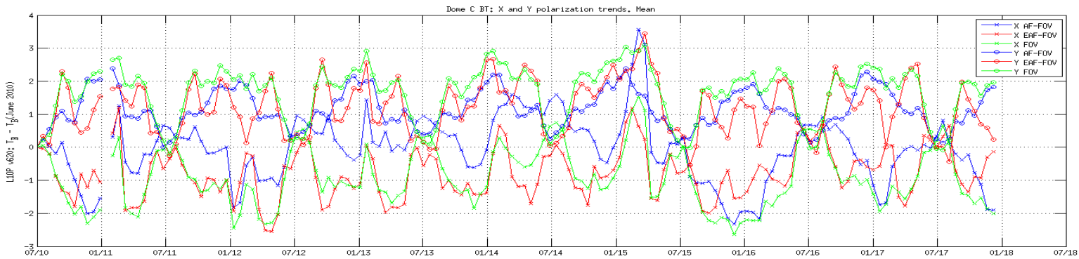
Figure 36: Dome-C X and Y polarization trends (all incidence angles)
