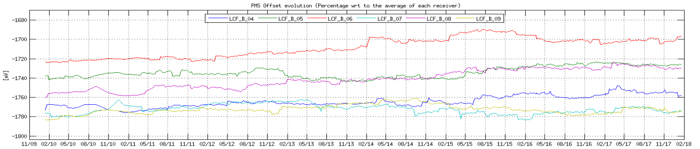
Figure 26 Evolution of the \Delta PMS Offset of the LICEFS in CMN B1
