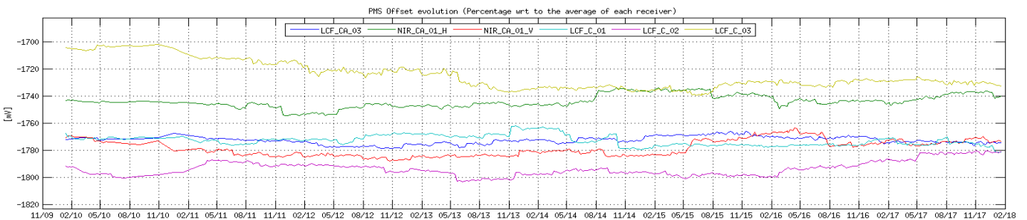
Figure 29 Evolution of the \Delta PMS Offset of the LICEFS in CMN H3
