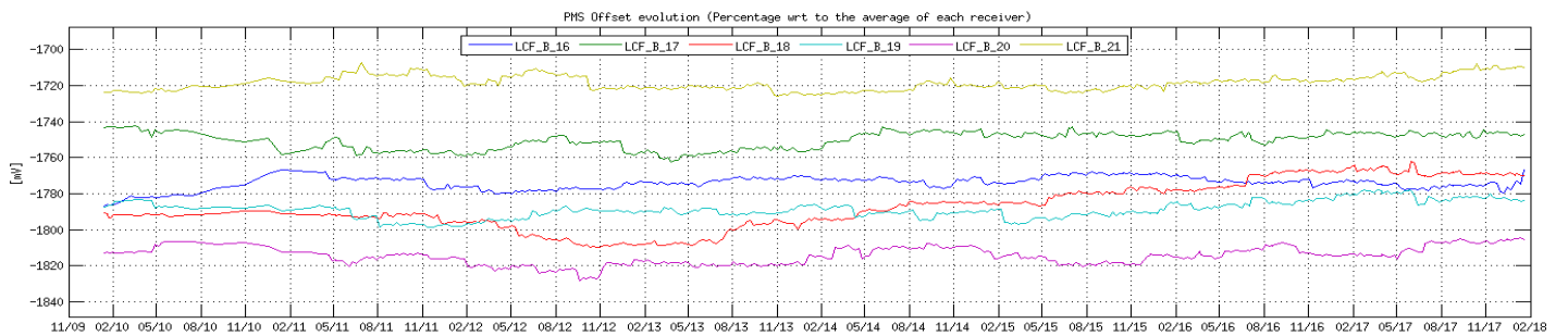
Figure 28 Evolution of the \Delta PMS Offset of the LICEFS in CMN B3
