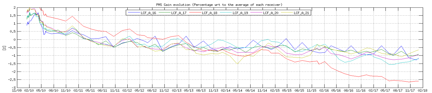
Figure 12 Evolution of the \Delta PMS Gain of the LICEFS in CMN A3
