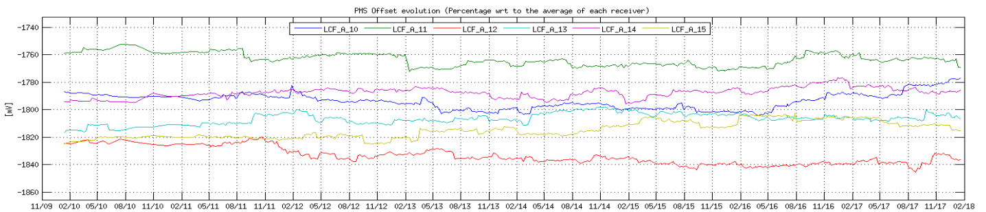
Figure 23 Evolution of the \Delta PMS Offset of the LICEFS in CMN A2
