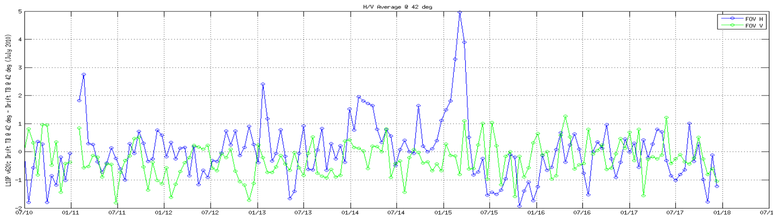
Figure 38: Dome-C H and V polarization trends in Extended Alias Free zone (incidence angle 42°)
