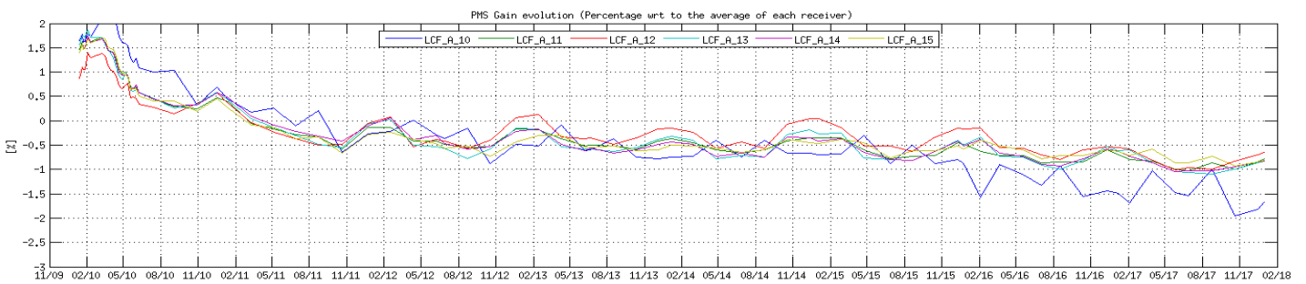
Figure 11 Evolution of the \Delta PMS Gain of the LICEFS in CMN A2
