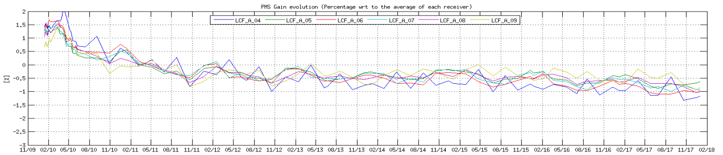
Figure 10 Evolution of the \Delta PMS Gain of the LICEFS in CMN A1
