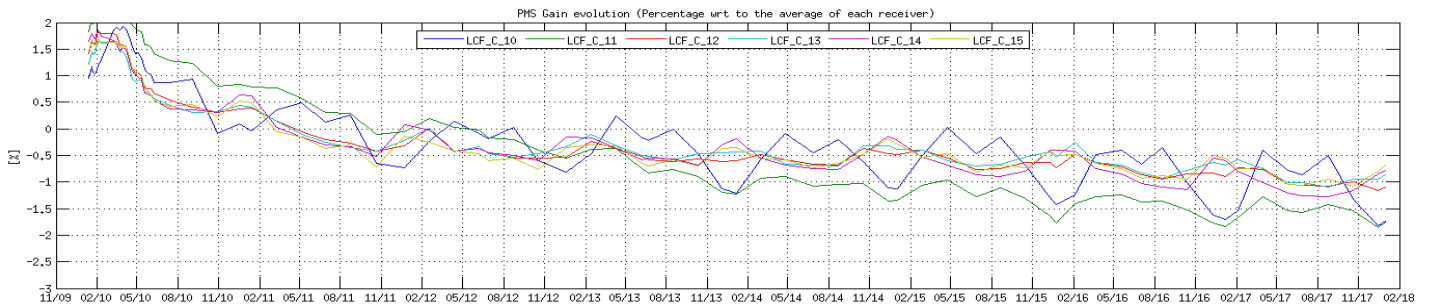
Figure 19 Evolution of the \Delta PMS Gain of the LICEFS in CMN C2
