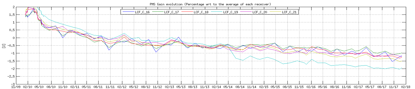
Figure 20 Evolution of the \Delta PMS Gain of the LICEFS in CMN C3
