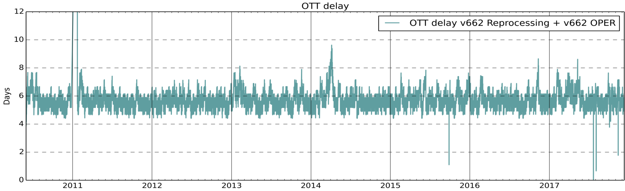
Figure 39: OTT delay per semi-orbit (Delta time between each L2OS product start time and the OTT correction validity start time file).
