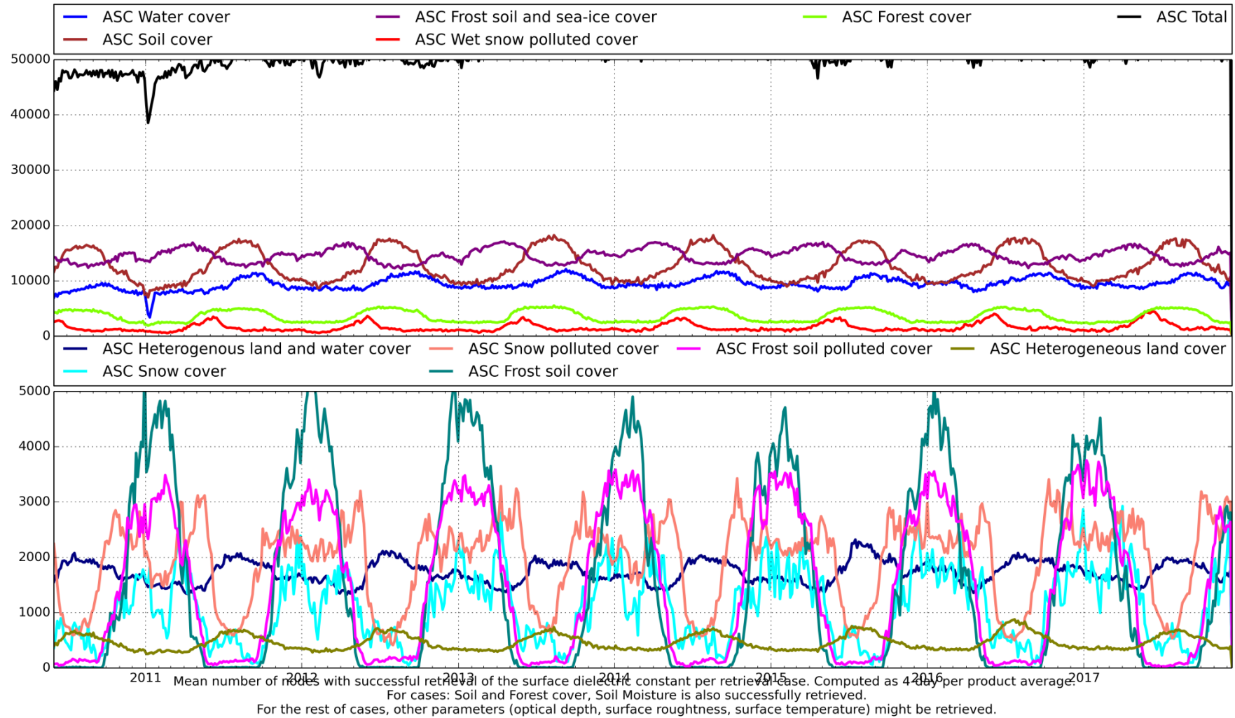
Figure 41: L2SM v650 Mean Retrievals Absolute - ASC
