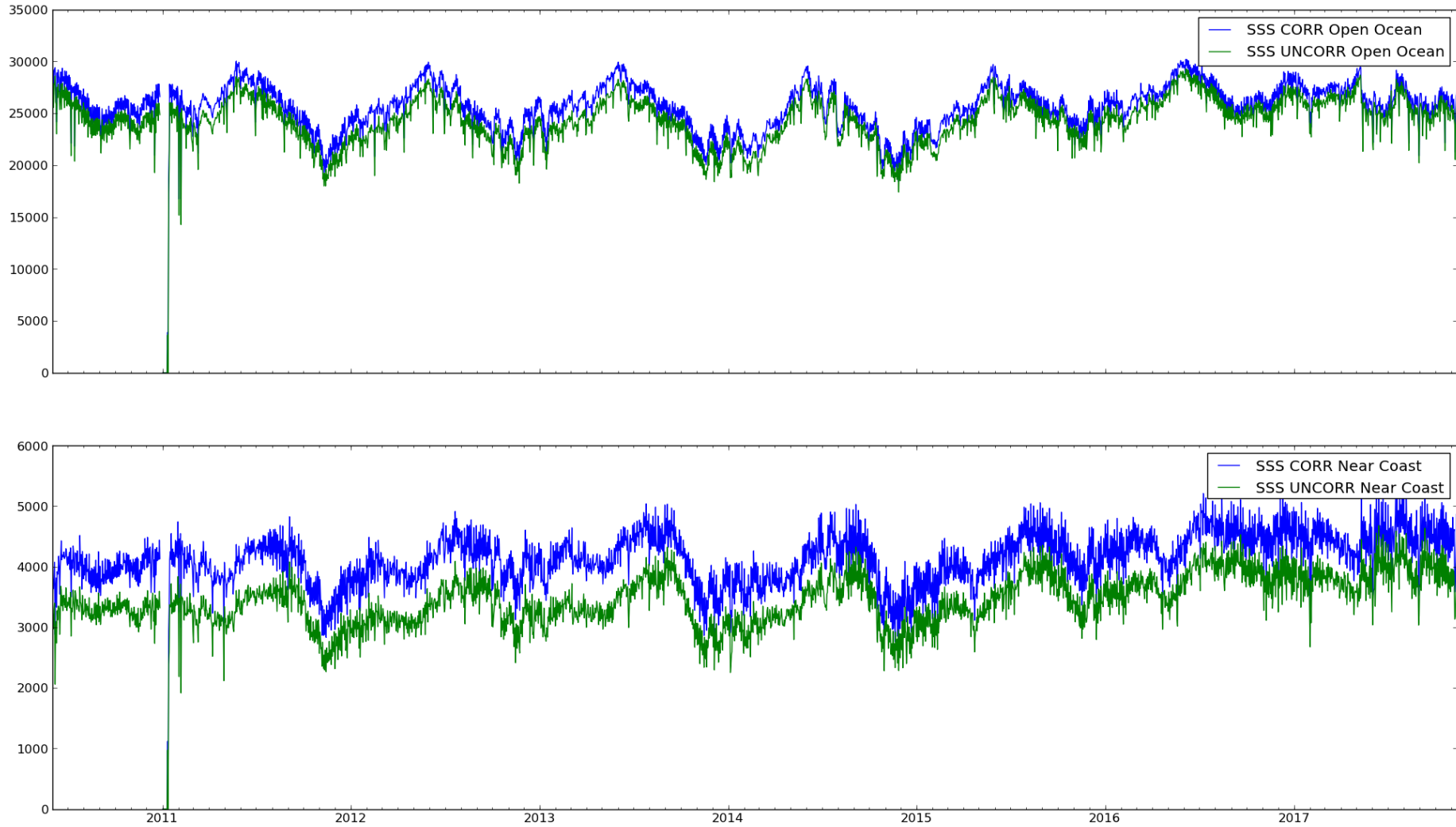
Figure 40: Open Ocean and Near Coast L2OS Good Quality Retrievals
