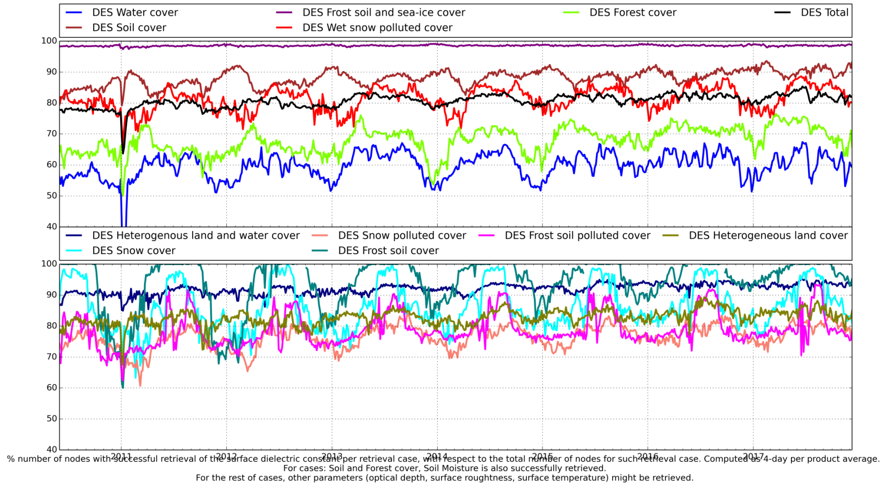
Figure 44: L2SM v650 Mean Retrievals Relative - DES
