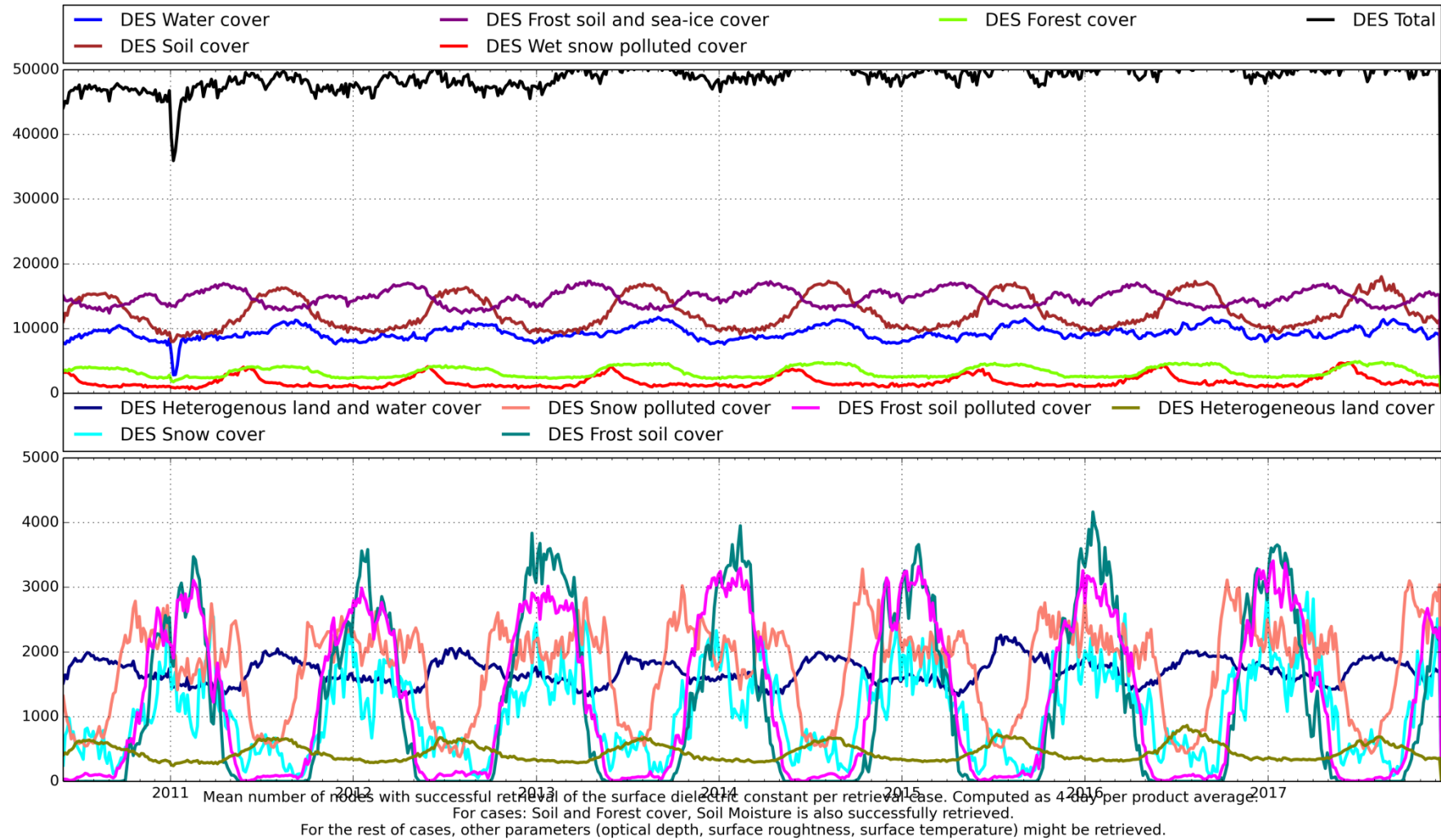
Figure 42: L2SM v650 Mean Retrievals Absolute - DES
