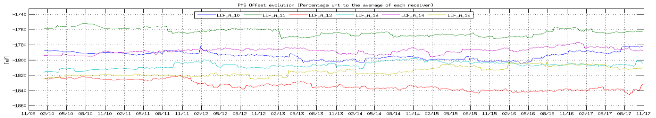
Figure 24 Evolution of the \Delta PMS Offset of the LICEFS in CMN A3
