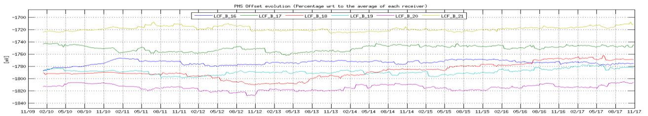
Figure 29 Evolution of the \Delta PMS Offset of the LICEFS in CMN H3
