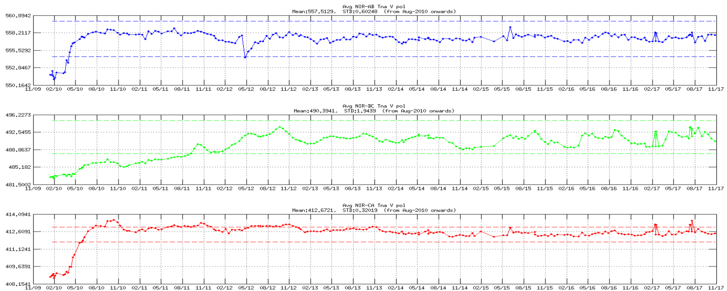
Figure 2 Tna evolution of NIR AB (blue), NIR BC (green) and NIR CA (red) in the V-channel since the beginning of the mission. Thresholds in dashed lines
