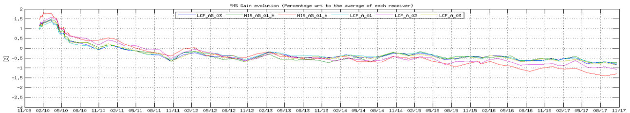
Figure 10 Evolution of the \Delta PMS Gain of the LICEFS in CMN A1
