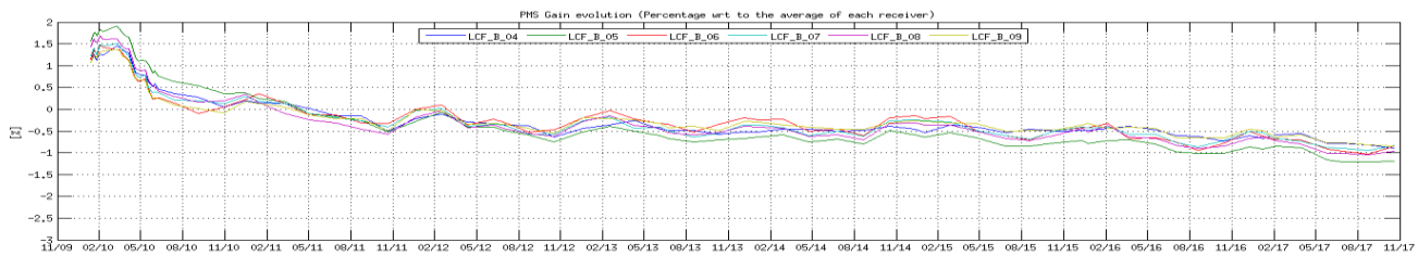
Figure 15 Evolution of the \Delta PMS Gain of the LICEFS in CMN B2
