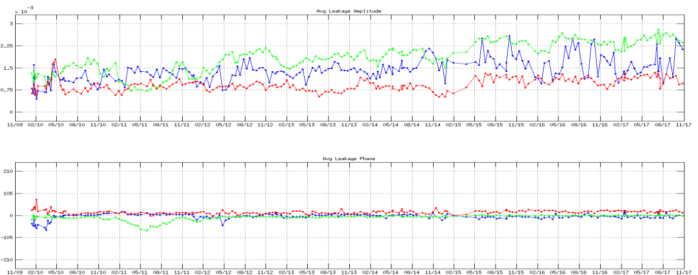
Figure 8 Leakage factor evolution in amplitude and phase of NIR AB (blue), NIR BC (green) and NIR CA (red) since the beginning of the mission
