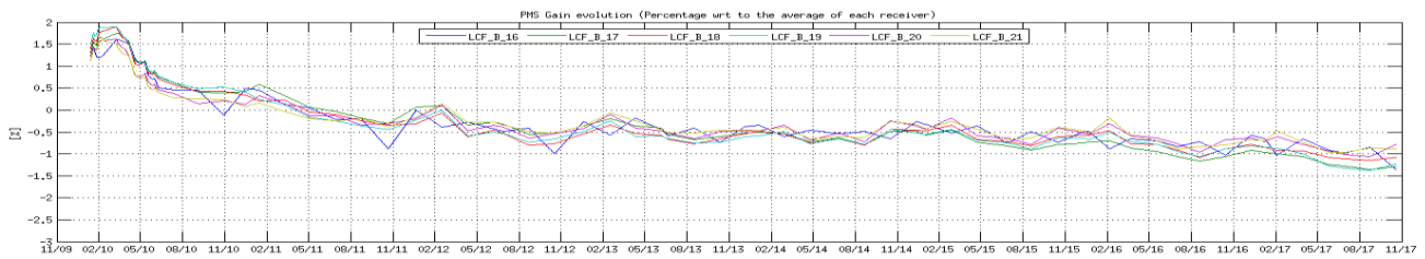
Figure 16 Evolution of the \Delta PMS Gain of the LICEFS in CMN B3
