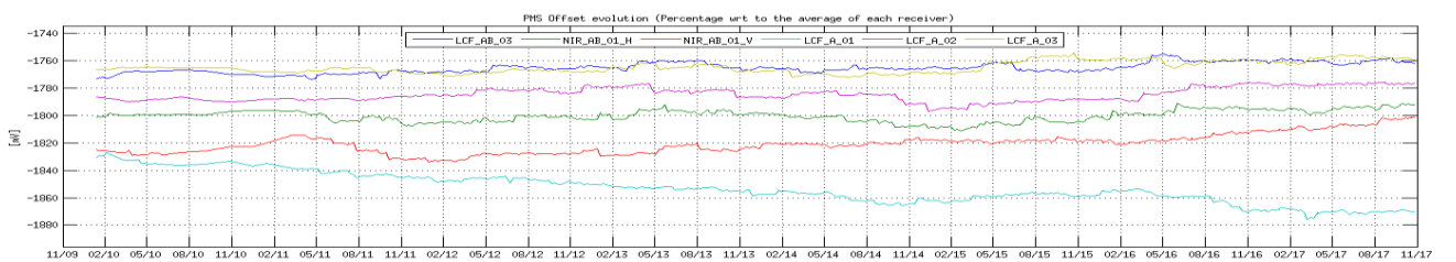
Figure 21 Evolution of the \Delta PMS Offset of the LICEFS in CMN H1
