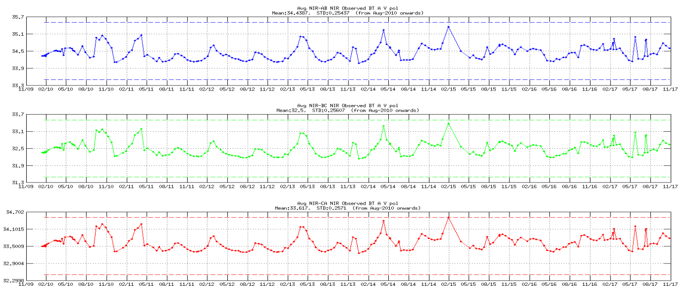
Figure 6 NIR Observed BT evolution of NIR AB (blue), NIR BC (green) and NIR CA (red) in the V-channel since the beginning of the mission. Thresholds in dashed lines
