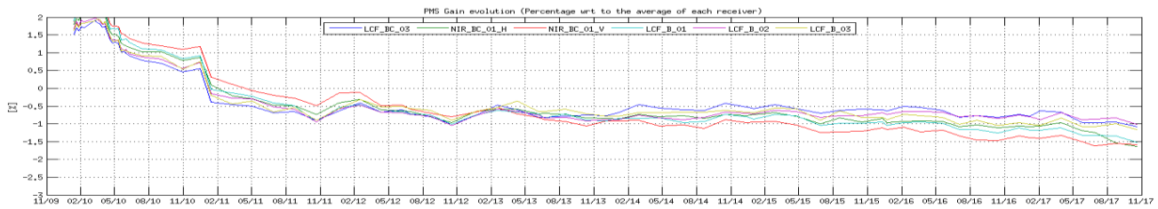
Figure 14 Evolution of the \Delta PMS Gain of the LICEFS in CMN B1
