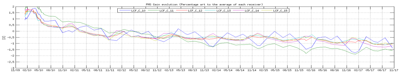
Figure 20 Evolution of the \Delta PMS Gain of the LICEFS in CMN C3
