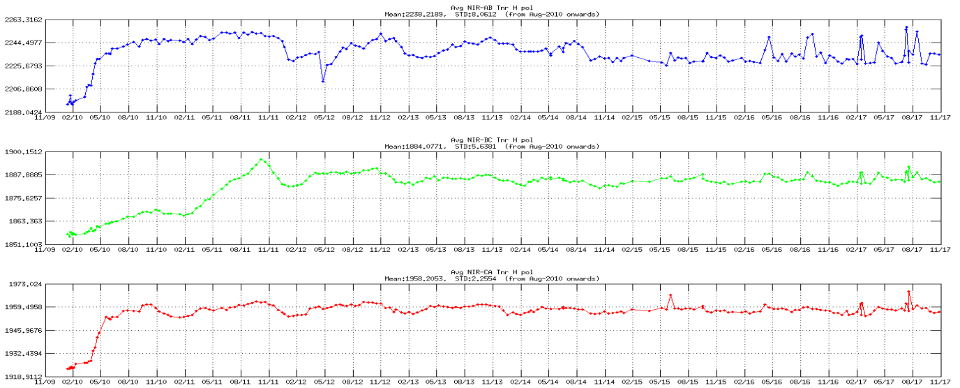
Figure 3 Tnr evolution of NIR AB (blue), NIR BC (green) and NIR CA (red) in the H-channel since the beginning of the mission.
