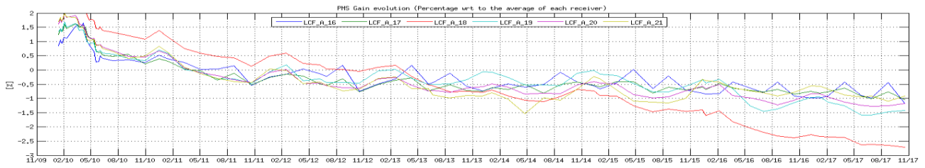
Figure 13 Evolution of the \Delta PMS Gain of the LICEFS in CMN H2
