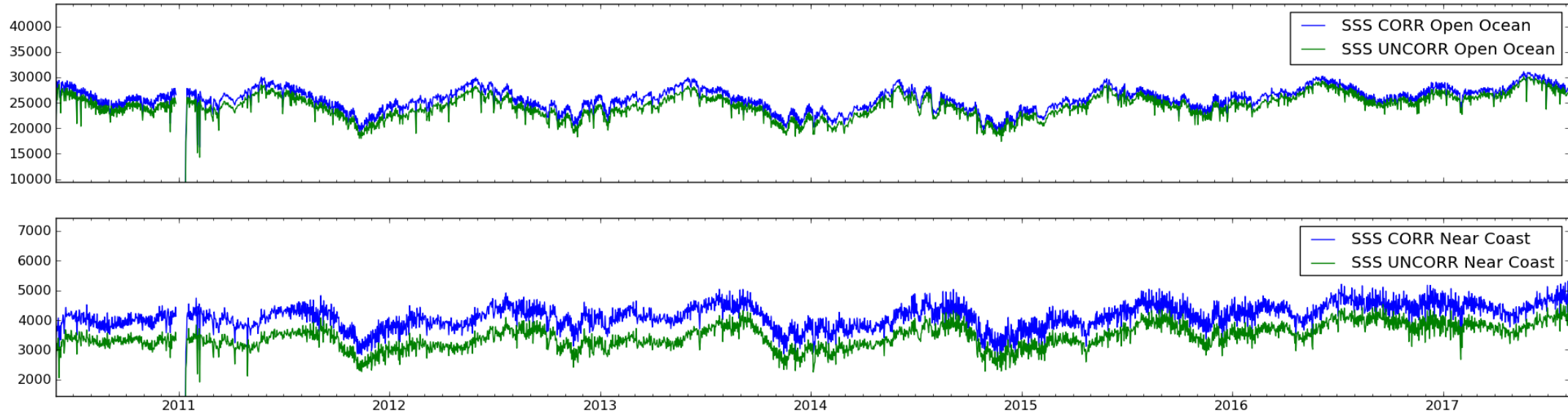
Figure 40: Open Ocean and Near Coast L2OS Good Quality Retrievals
