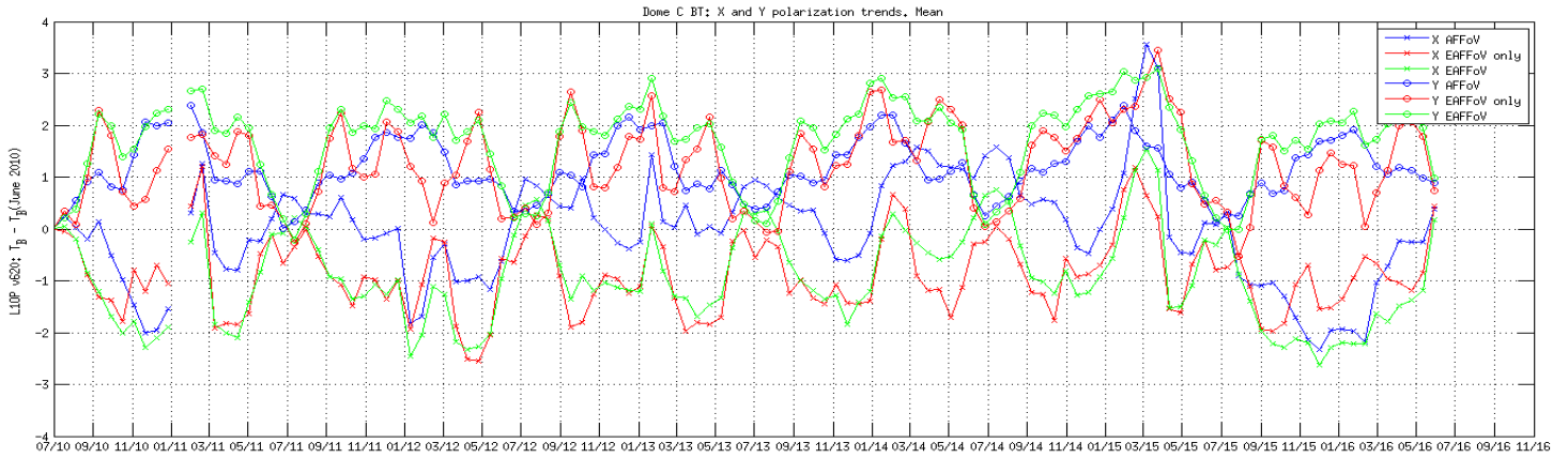
Figure 36: Dome-C X and Y polarization trends (all incidence angles)
