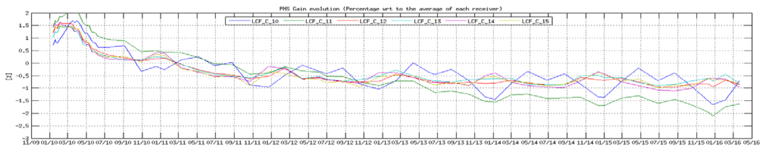
Figure 19 Evolution of the \Delta PMS Gain of the LICEFS in CMN C2
