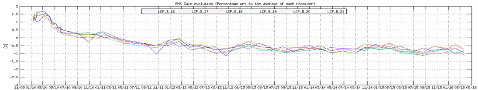
Figure 16 Evolution of the \Delta PMS Gain of the LICEFS in CMN B3
