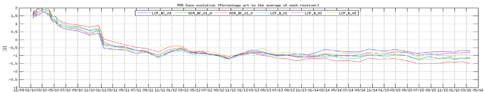
Figure 13 Evolution of the \Delta PMS Gain of the LICEFS in CMN H2
