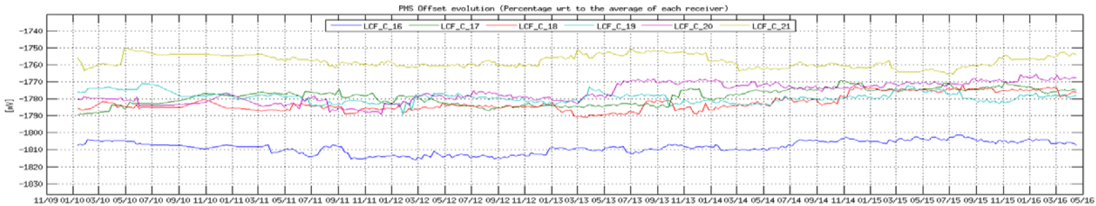
Figure 32 Evolution of the \Delta PMS Offset of the LICEFS in CMN C3
