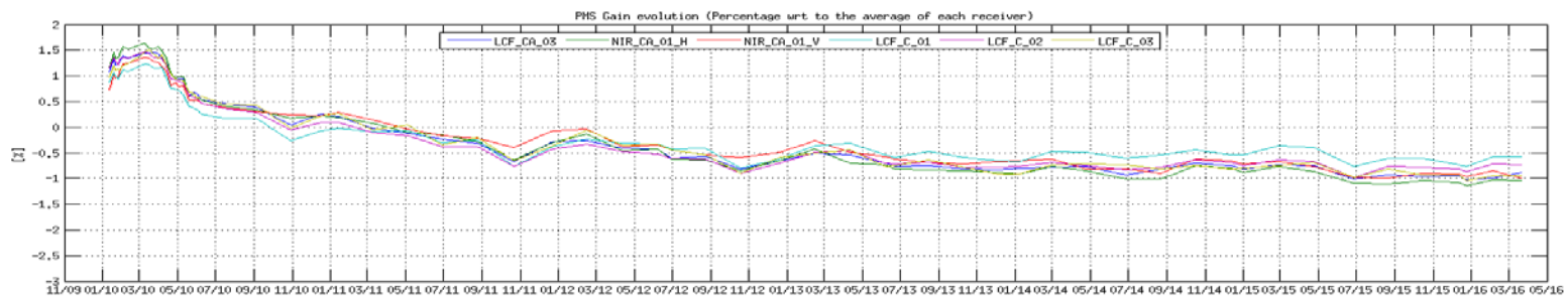
Figure 17 Evolution of the \Delta PMS Gain of the LICEFS in CMN H3
