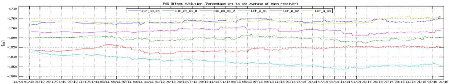
Figure 21 Evolution of the \Delta PMS Offset of the LICEFS in CMN H1
