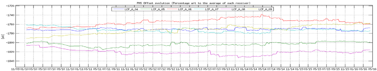
Figure 22 Evolution of the \Delta PMS Offset of the LICEFS in CMN A1
