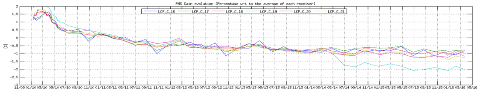
Figure 20 Evolution of the \Delta PMS Gain of the LICEFS in CMN C3
