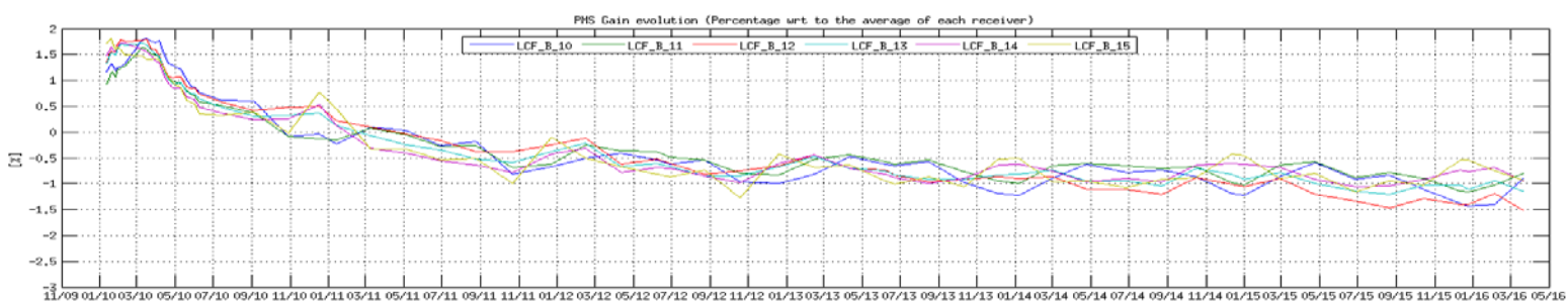
Figure 15 Evolution of the \Delta PMS Gain of the LICEFS in CMN B2
