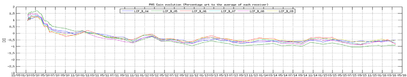
Figure 14 Evolution of the \Delta PMS Gain of the LICEFS in CMN B1
