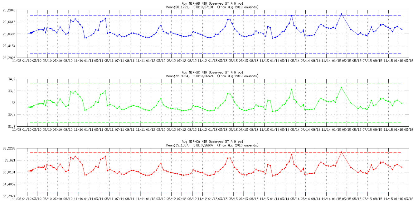
Figure 5 NIR Observed BT evolution of NIR AB (blue), NIR BC (green) and NIR CA (red) in the H-channel since the beginning of the mission. Thresholds in dashed lines
