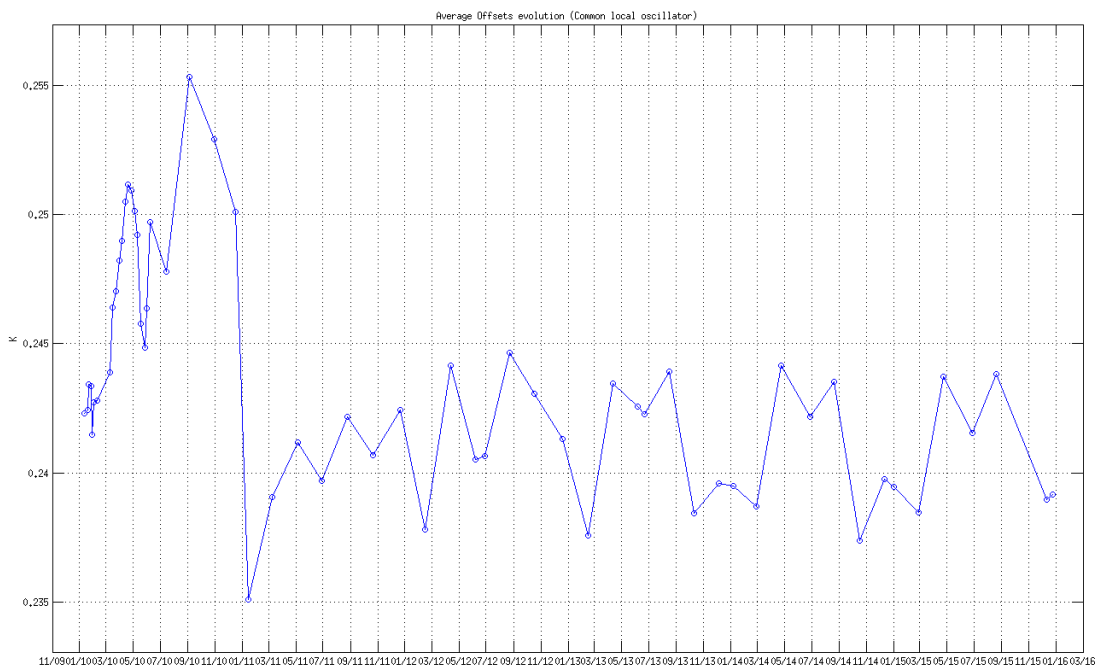
Figure 34 Evolution of the average of the Correlator offsets for the baselines which share local oscillator
