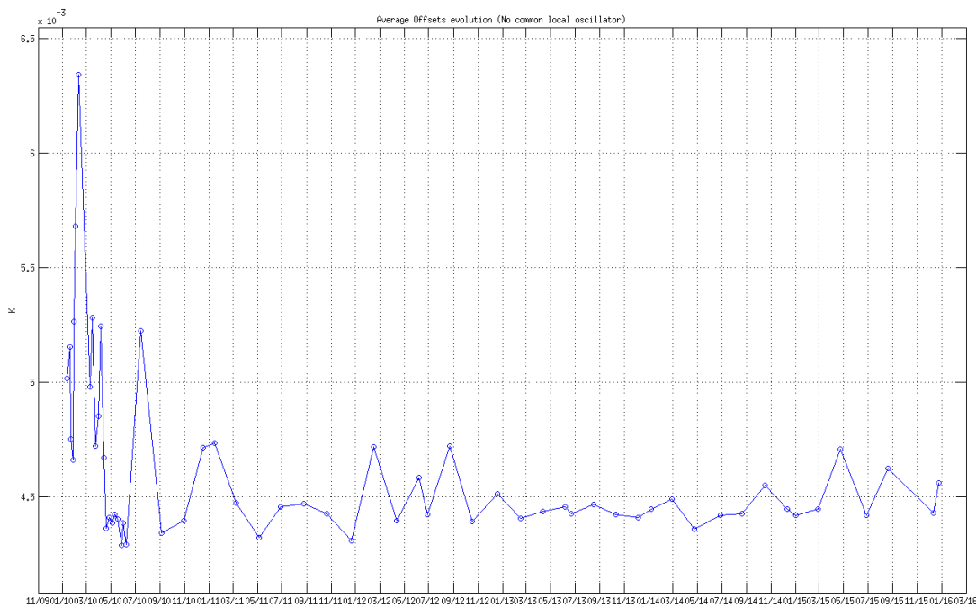
Figure 35 Evolution of the average of the Correlator offsets for the baselines which do not share local oscillator
