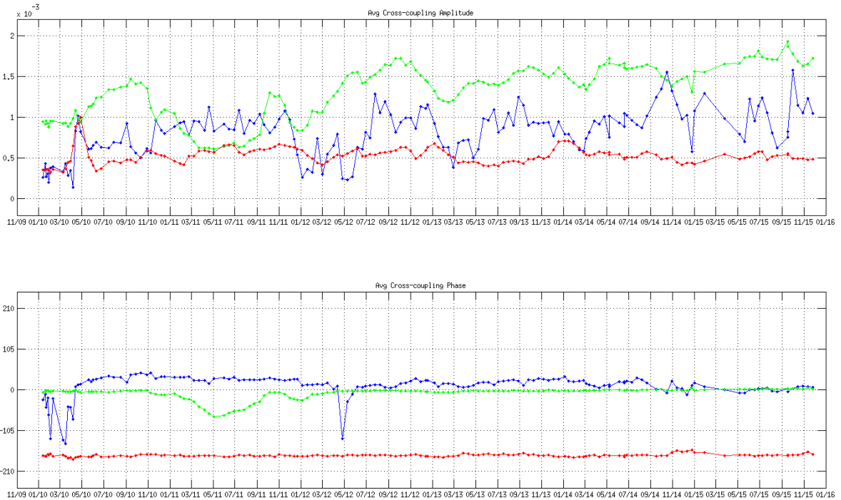
Figure 6 Leakage factor evolution in amplitude and phase of NIR AB (blue), NIR BC (green) and NIR CA (red) since the beginning of the mission
