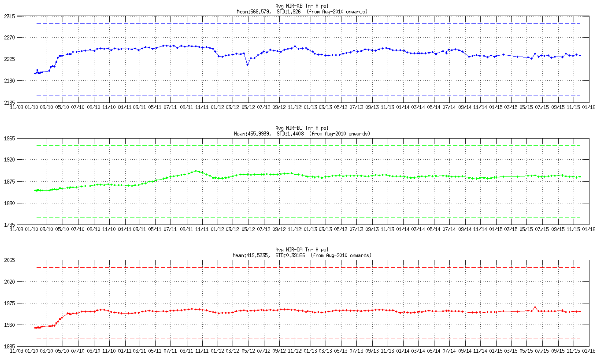
Figure 3 Tnr evolution of NIR AB (blue), NIR BC (green) and NIR CA (red) in the H-channel since the beginning of the mission. Thresholds in dashed lines
