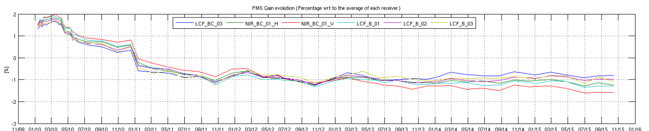
Figure 11 Evolution of the \Delta PMS Gain of the LICEFS in CMN H2
