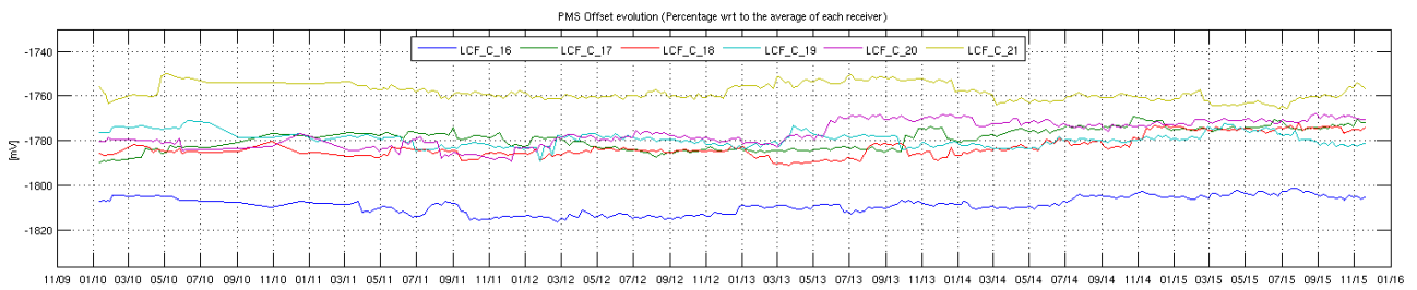
Figure 30 Evolution of the \Delta PMS Offset of the LICEFS in CMN C3
