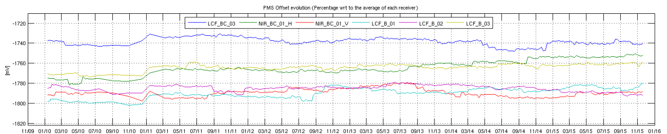
Figure 23 Evolution of the \Delta PMS Offset of the LICEFS in CMN H2
