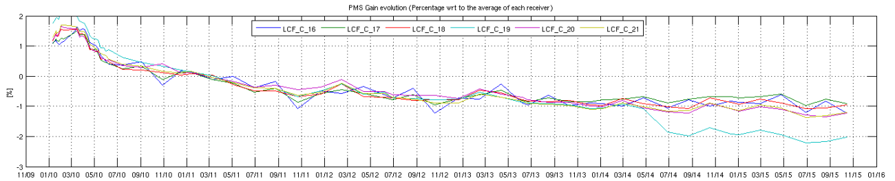
Figure 18 Evolution of the \Delta PMS Gain of the LICEFS in CMN C3
