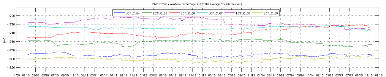
Figure 28 Evolution of the \Delta PMS Offset of the LICEFS in CMN C1
