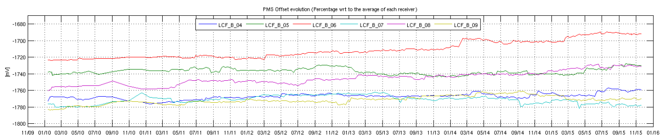
Figure 24 Evolution of the \Delta PMS Offset of the LICEFS in CMN B1
