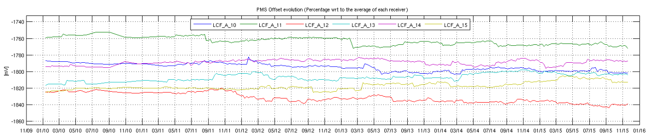
Figure 21 Evolution of the \Delta PMS Offset of the LICEFS in CMN A2
