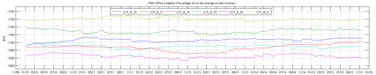
Figure 26 Evolution of the \Delta PMS Offset of the LICEFS in CMN B3
