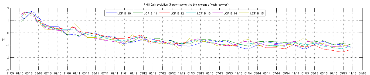
Figure 13 Evolution of the \Delta PMS Gain of the LICEFS in CMN B2
