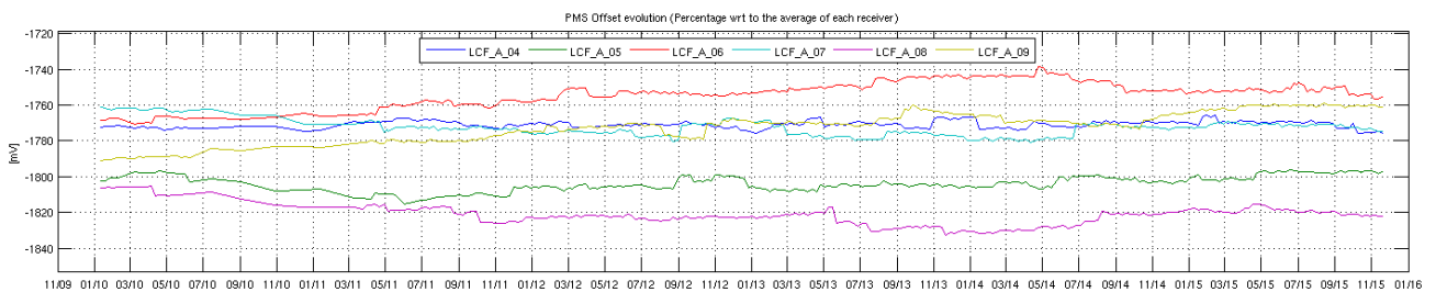
Figure 20 Evolution of the \Delta PMS Offset of the LICEFS in CMN A1
