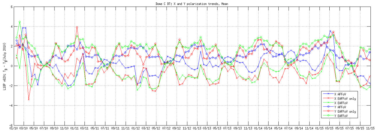
Figure 35: Dome-C H and V polarization trends in Alias Free zone (incidence angle 42°)
