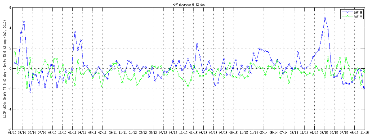
Figure 36: Dome-C H and V polarization trends in Extended Alias Free zone (incidence angle 42°)
