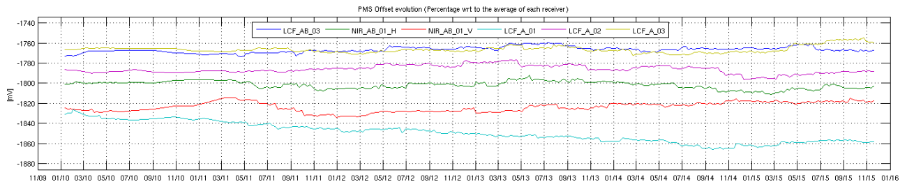
Figure 19 Evolution of the \Delta PMS Offset of the LICEFS in CMN H1
