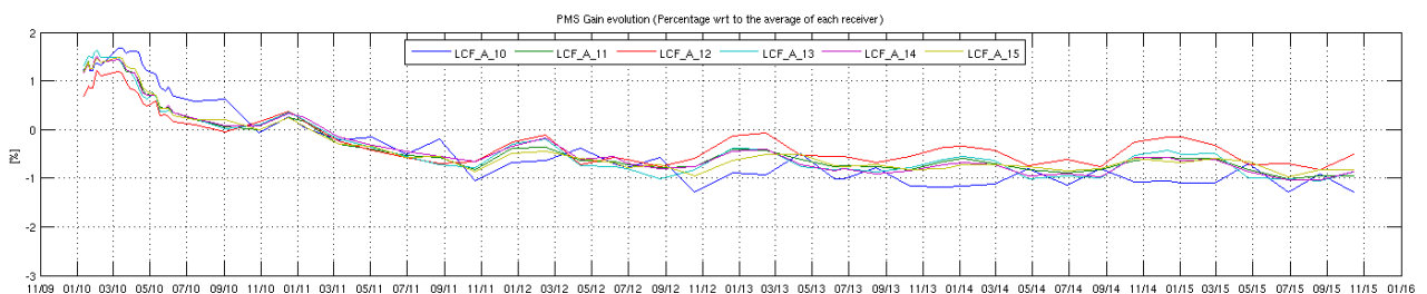
Figure 9 Evolution of the \Delta PMS Gain of the LICEFS in CMN A2
