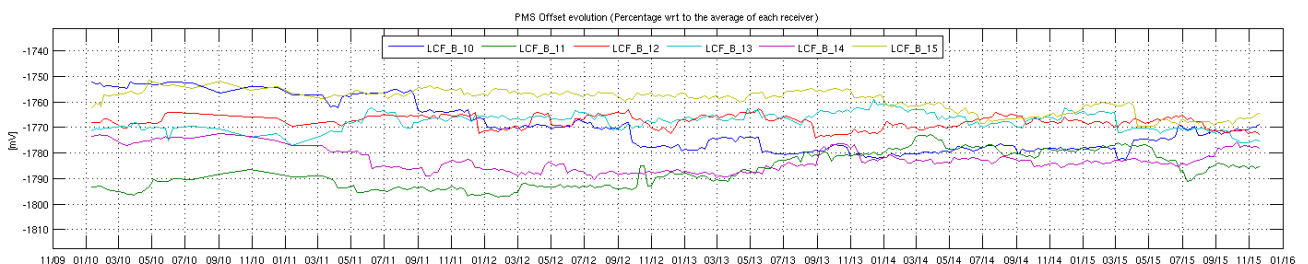
Figure 25 Evolution of the \Delta PMS Offset of the LICEFS in CMN B2
