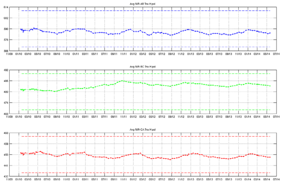
Figure 1 Tna evolution of NIR AB (blue), NIR BC (green) and NIR CA (red) in the H-channel since the beginning of the mission. Thresholds in dashed lines
