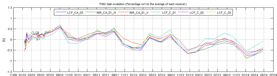
Figure 16 Evolution of the \Delta PMS Gain of the LICEFS in CMN C1
