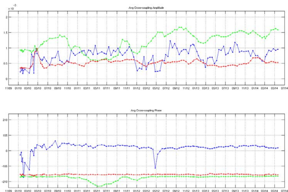
Figure 6 Leakage factor evolution in amplitude and phase of NIR AB (blue), NIR BC (green) and NIR CA (red) since the beginning of the mission
