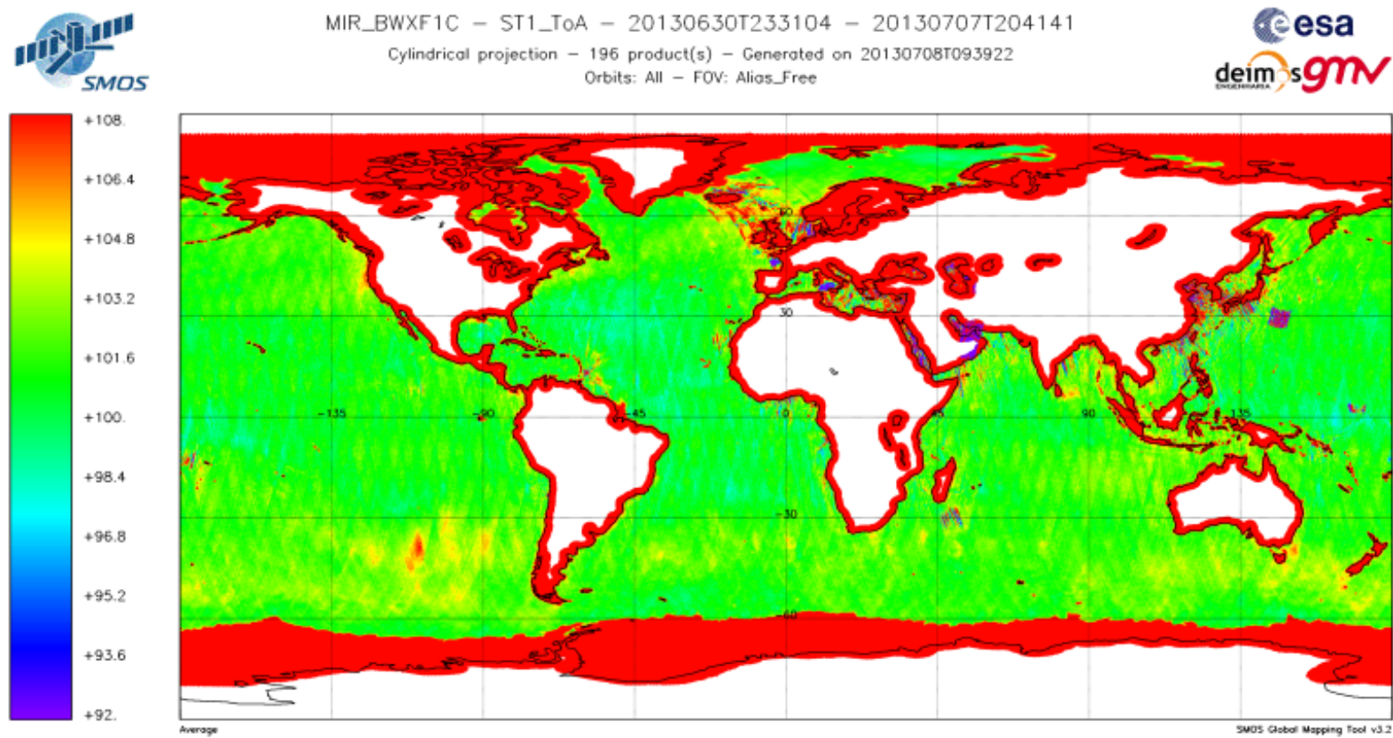
Figure 49 1st Stokes evolution over sea during the reporting period (week 27)
