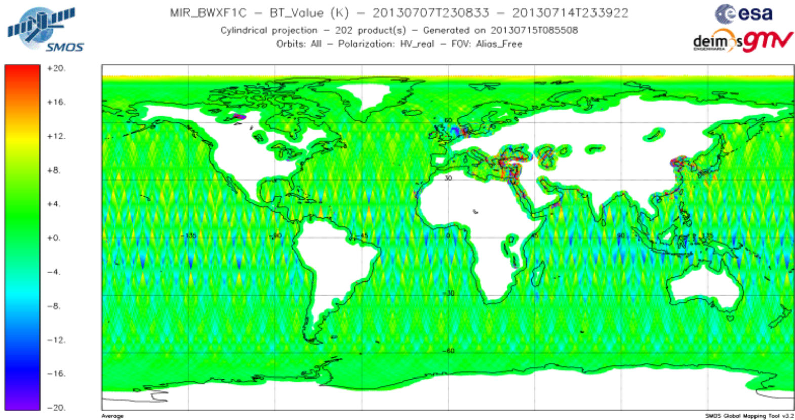
Figure 55 Real Part of the XY Brightness temperature evolution over sea during the reporting period (week 28)
