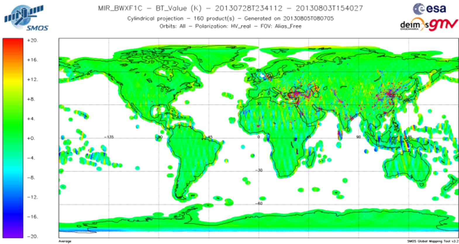
Figure 43 Real Part of the XY Brightness temperature evolution over land during the reporting period (week 31)
