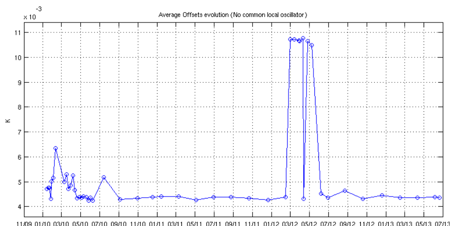
Figure 33 Evolution of the average of the Correlator offsets for the baselines which do not share local oscillator
