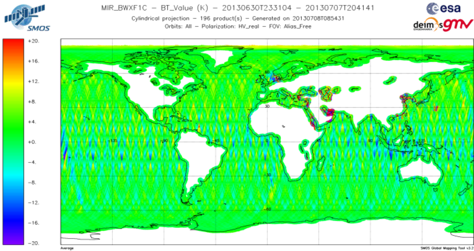
Figure 54 Real Part of the XY Brightness temperature evolution over sea during the reporting period (week 27)
