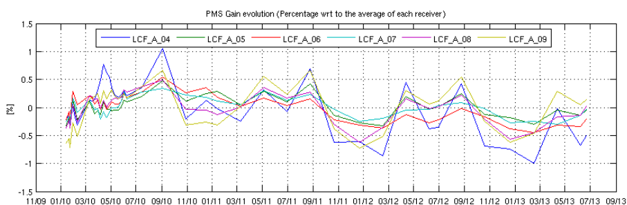
Figure 8 Evolution of the \Delta PMS Gain of the LICEFS in CMN A1
