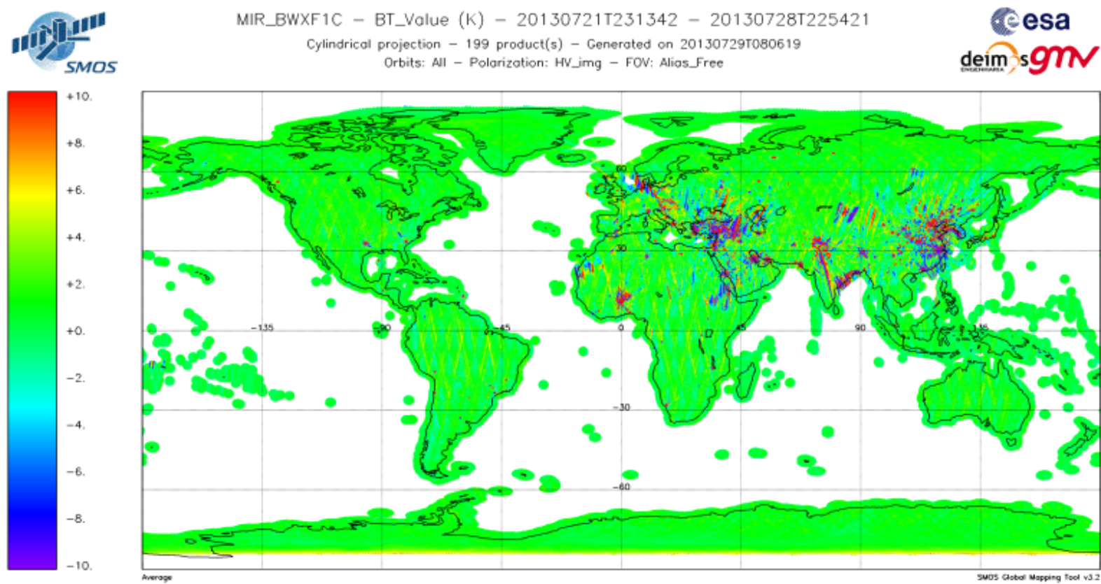
Figure 47 Imaginary Part of the XY Brightness temperature evolution over land during the reporting period (week 30)
