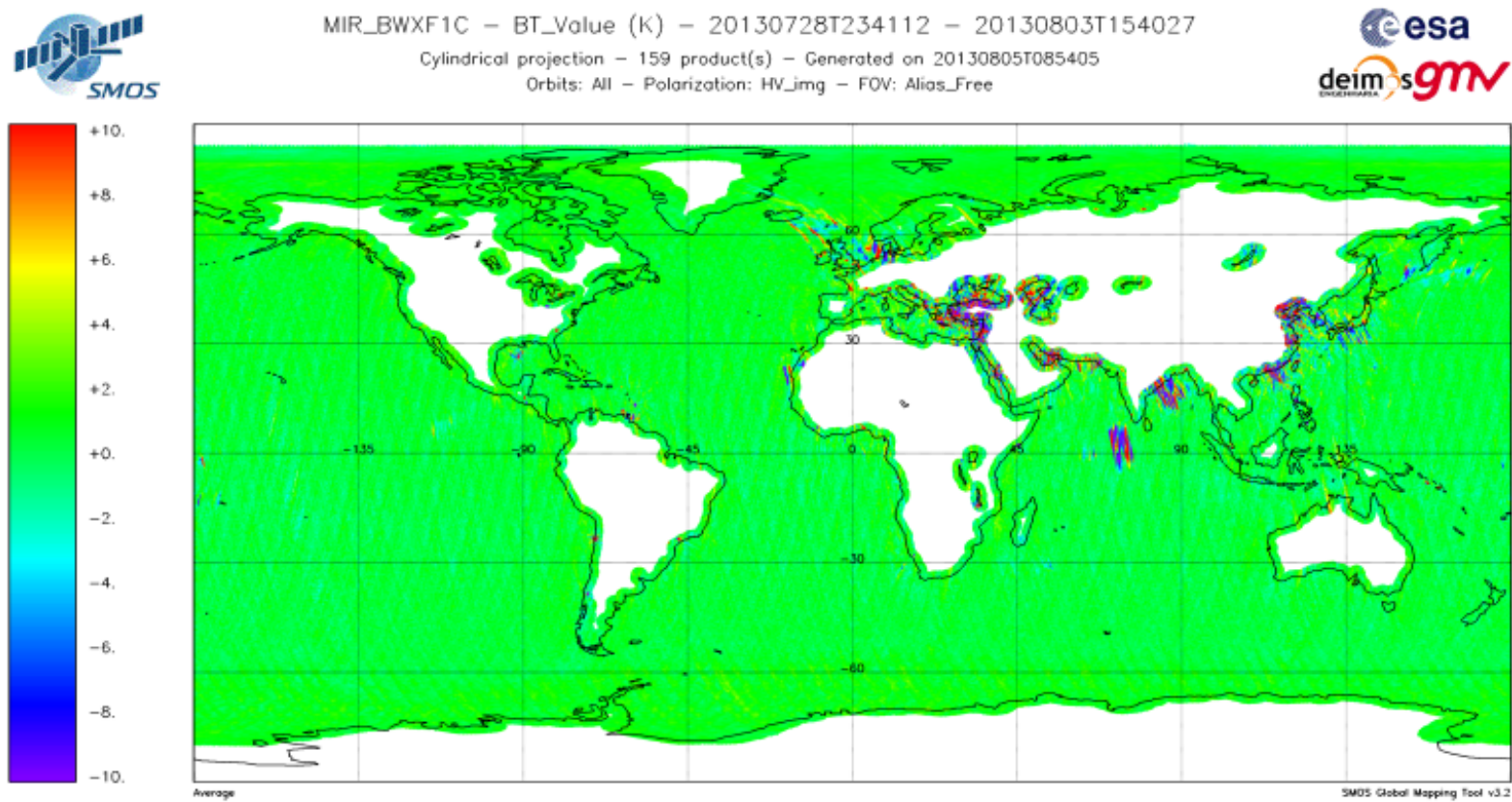
Figure 63 Imaginary Part of the XY Brightness temperature evolution over sea during the reporting period (week 31)
