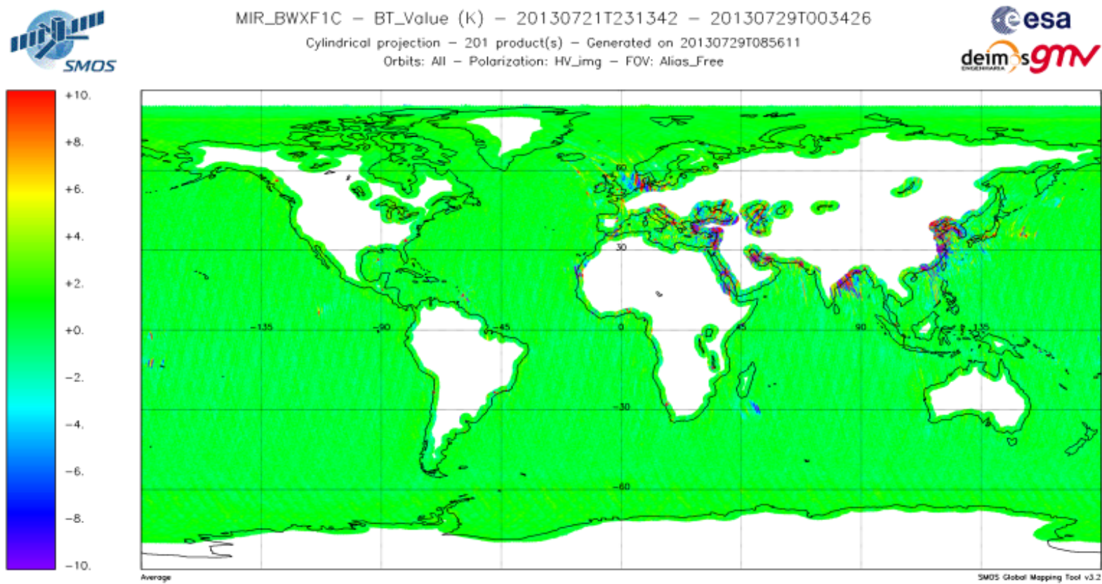
Figure 62 Imaginary Part of the XY Brightness temperature evolution over sea during the reporting period (week 30)
