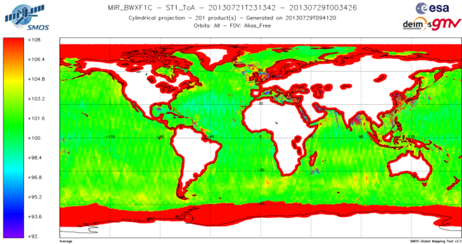
Figure 52 1st Stokes evolution over sea during the reporting period (week 30)
