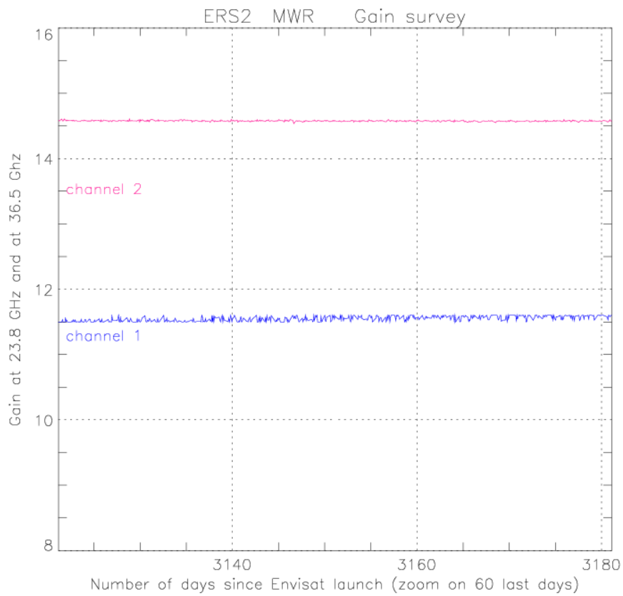
Figure 3: Time evolution of the gain since June, 1996.
