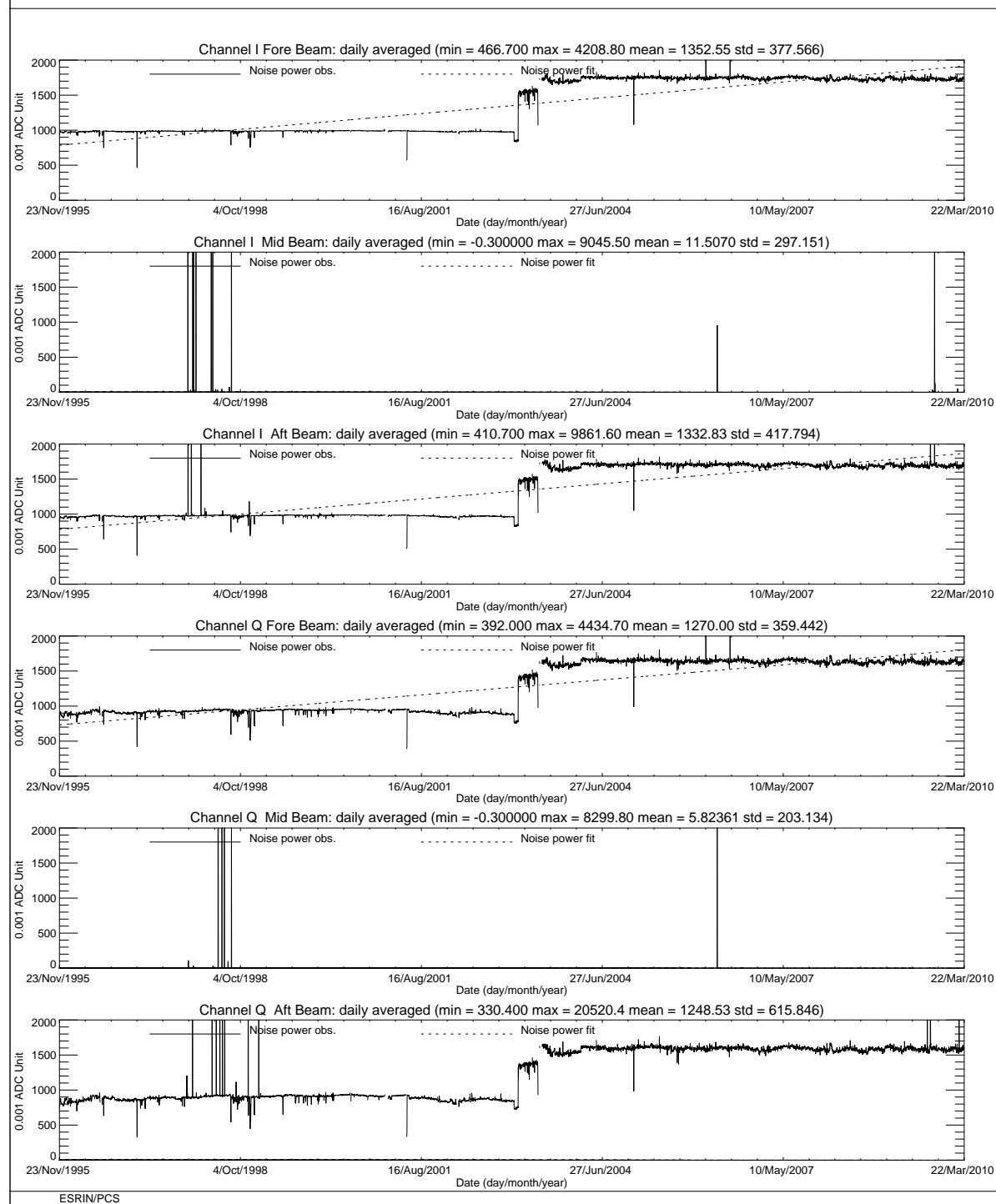
FIGURE 7 ERS-2 Scatterometer: noise power I and Q channel since the beginning of the mission.
