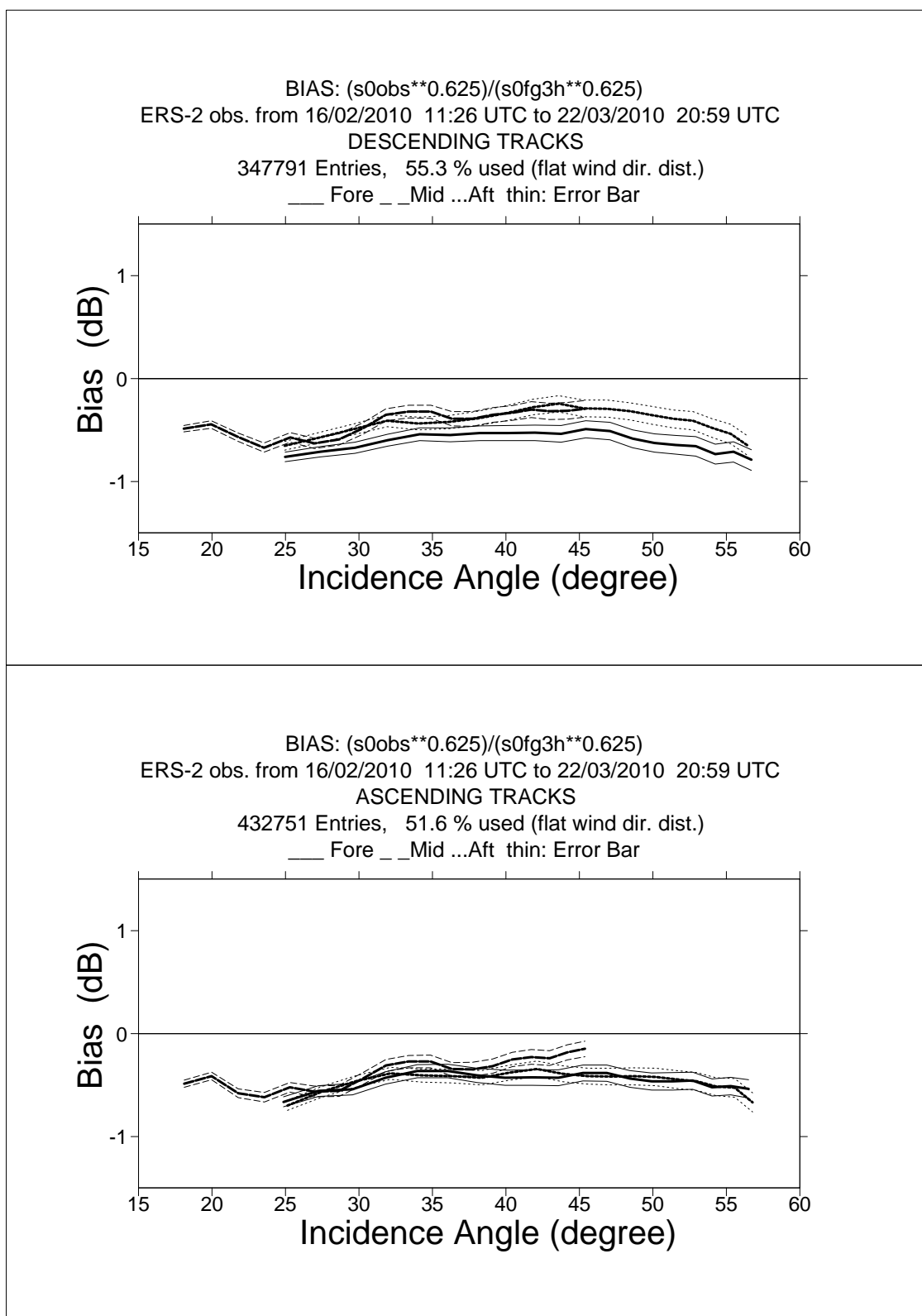
FIGURE 1 ERS-2 Scatterometer Ocean Calibration cycle 155. Ratio of \langle \sigma_0^{0.625} \rangle / \langle \text{CMOD4}(\text{First Guess})^{0.625} \rangle converted in dB for the fore beam (solid line), mid beam (dashed line) an aft beam (dotted line), as a function of incidence angle for descending and ascending tracks. The thin lines indicate the error bars on the estimated mean. First-guess winds are based on the in time closest (+3h, +6h, +9h, or +12h) T511 forecast field, and are bilinearly interpolated in space.
