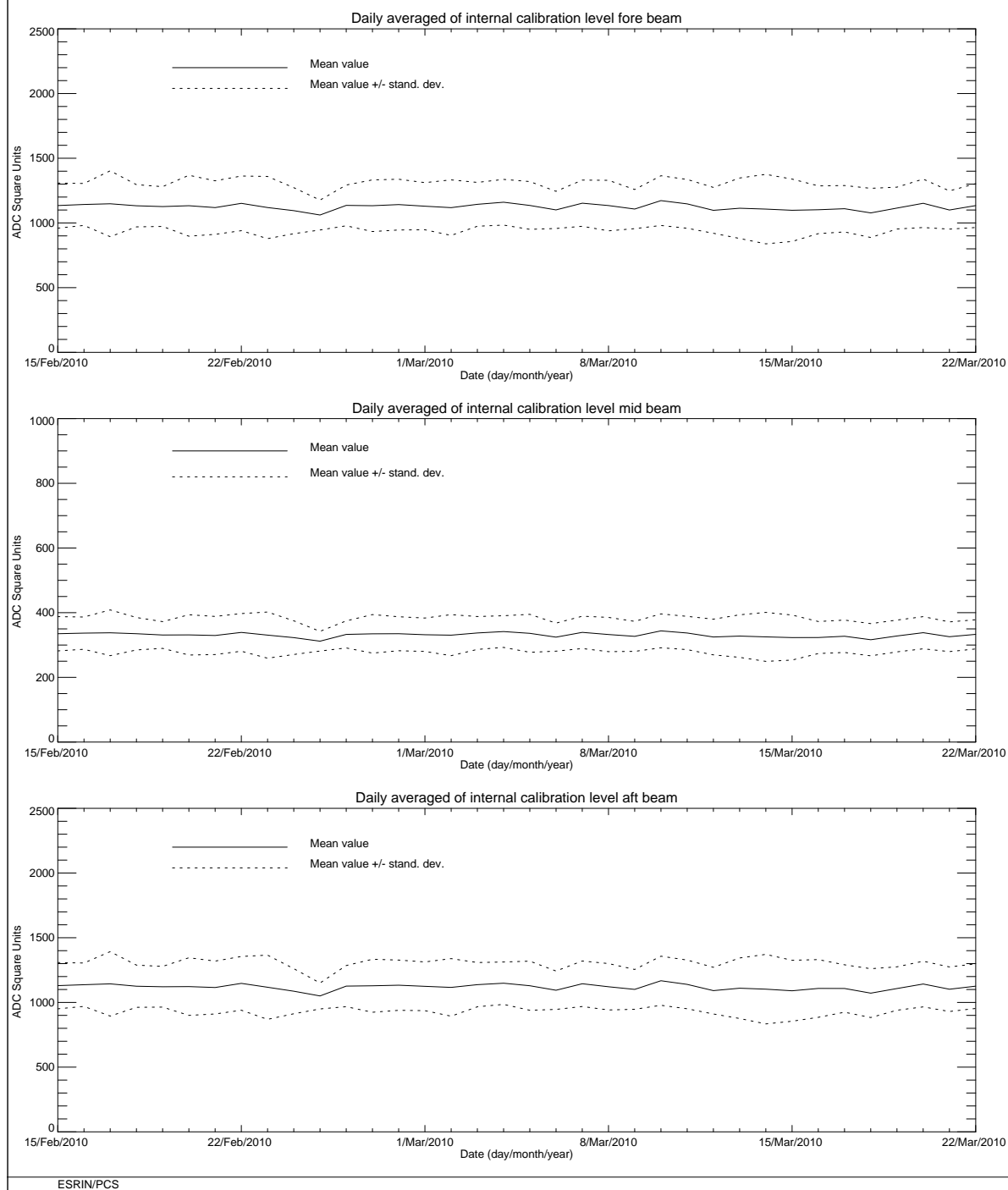
FIGURE 10 ERS-2 Scatterometer: power of internal calibration level cycle 155.
