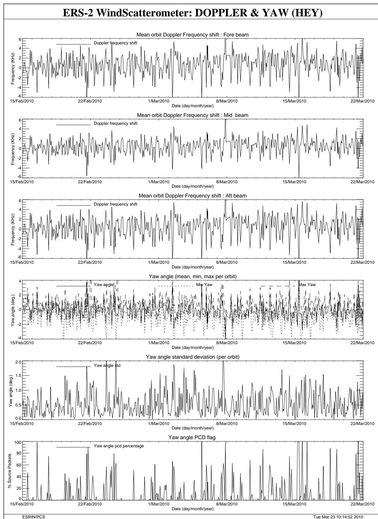
FIGURE 31 Doppler frequency shift and Yaw error angle evolution cycle 155.
