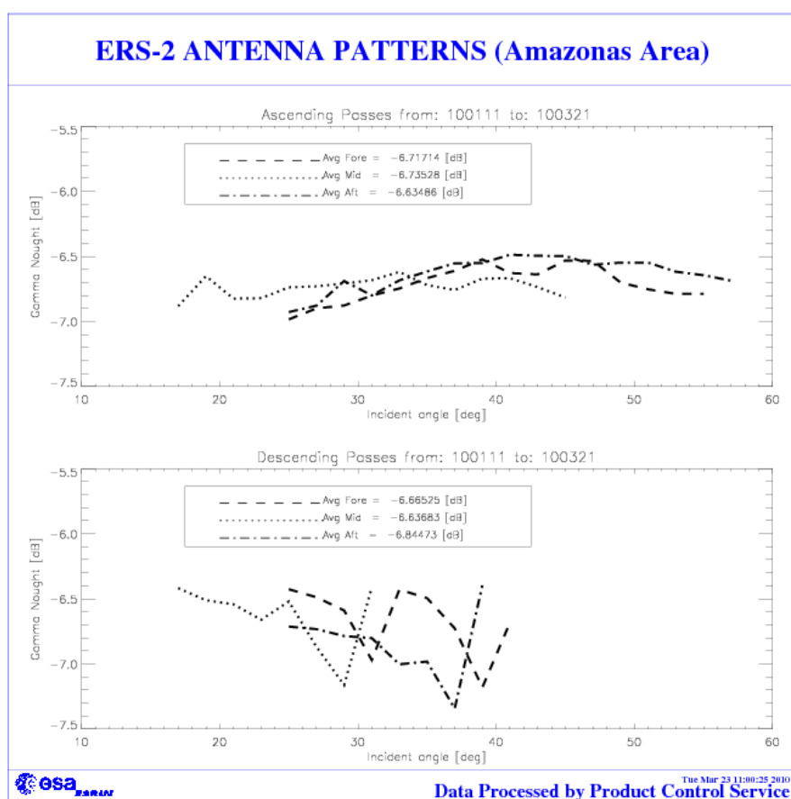
FIGURE 2 ERS-2 Scatterometer antenna pattern as function of the incidence angle: cycle 154 and 155.
