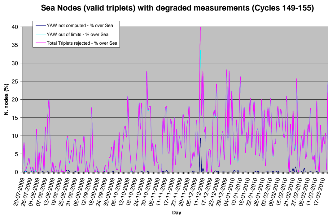
FIGURE 33 Statistics of degraded sigma nought triplets over Sea.
