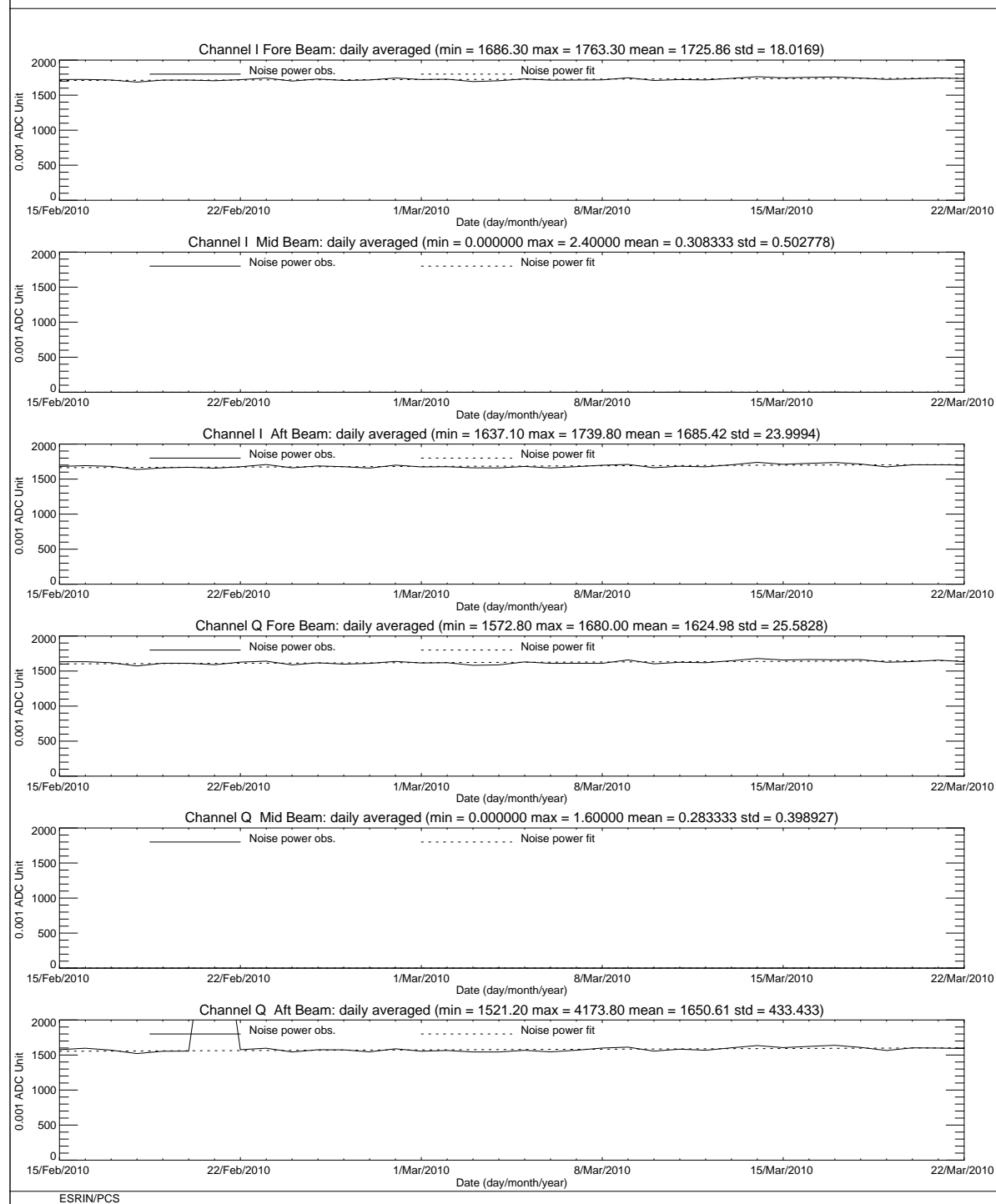
FIGURE 8 ERS-2 Scatterometer: noise power I and Q channel for cycle 155.
