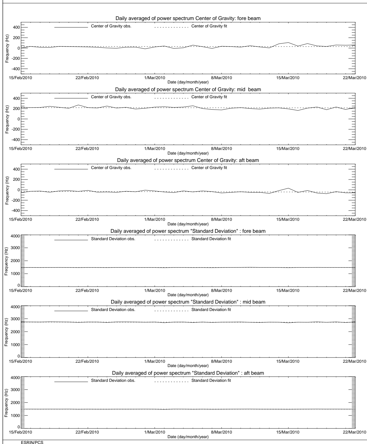
FIGURE 6 ERS-2 Scatterometer: Centre of Gravity and standard deviation of received power spectrum for cycle 155.
