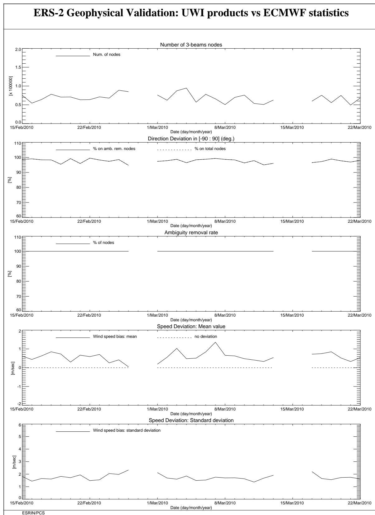
FIGURE 13 ERS-2 Scatterometer: wind products performance for cycle 155.
