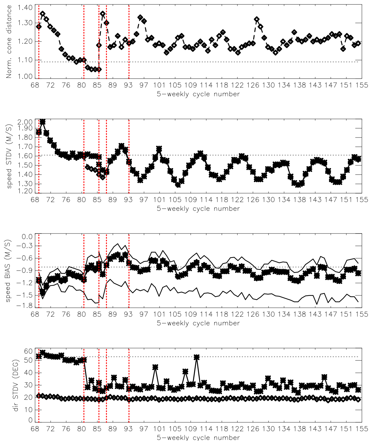
FIGURE 14 Evolution of the performance of the ERS-2 Scatterometer averaged over 5-weekly cycles from 12 December 2001 (cycle 69) to 15 February 2010 (end cycle 154) for the UWI product (solid, star) and de-aliased winds based on CMOD4 (dashed, diamond). Results are based on data that passed the UWI QC flags. For cycle 85 two values are plotted; the first value for the global set, the second one for the regional set. Dotted lines represent values for cycle 59 (5 December 2000 to 17 January 2001), i.e. the last stable cycle of the nominal period. From top to bottom panel are shown the normalized distance to the one (CMOD4 only) the standard deviation of the wind speed compared to FG winds, the corresponding bias (for UWI winds the extreme inter-node averages are shown as well), and the standard deviation of wind direction compared to FG.
