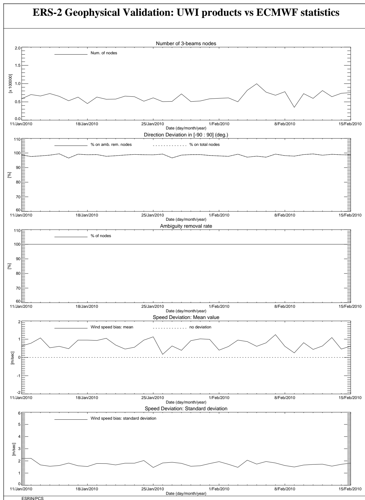
FIGURE 13 ERS-2 Scatterometer: wind products performance for cycle 154.
