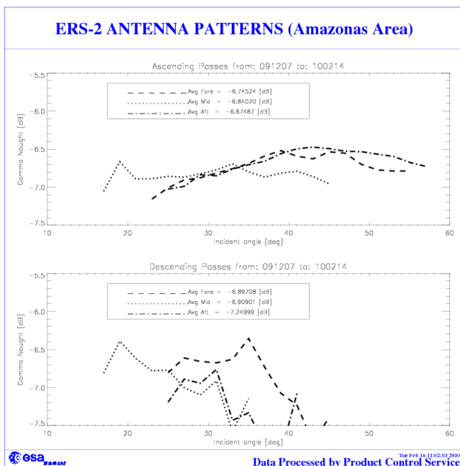
FIGURE 2 ERS-2 Scatterometer antenna pattern as function of the incidence angle: cycle 153 and 154.
