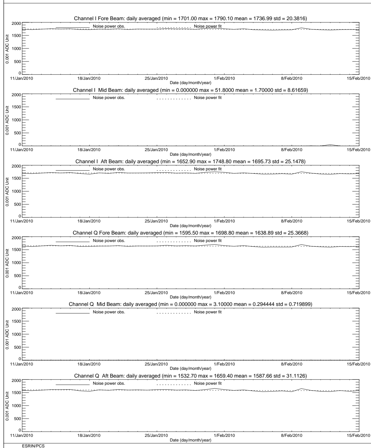
FIGURE 8 ERS-2 Scatterometer: noise power I and Q channel for cycle 154.
