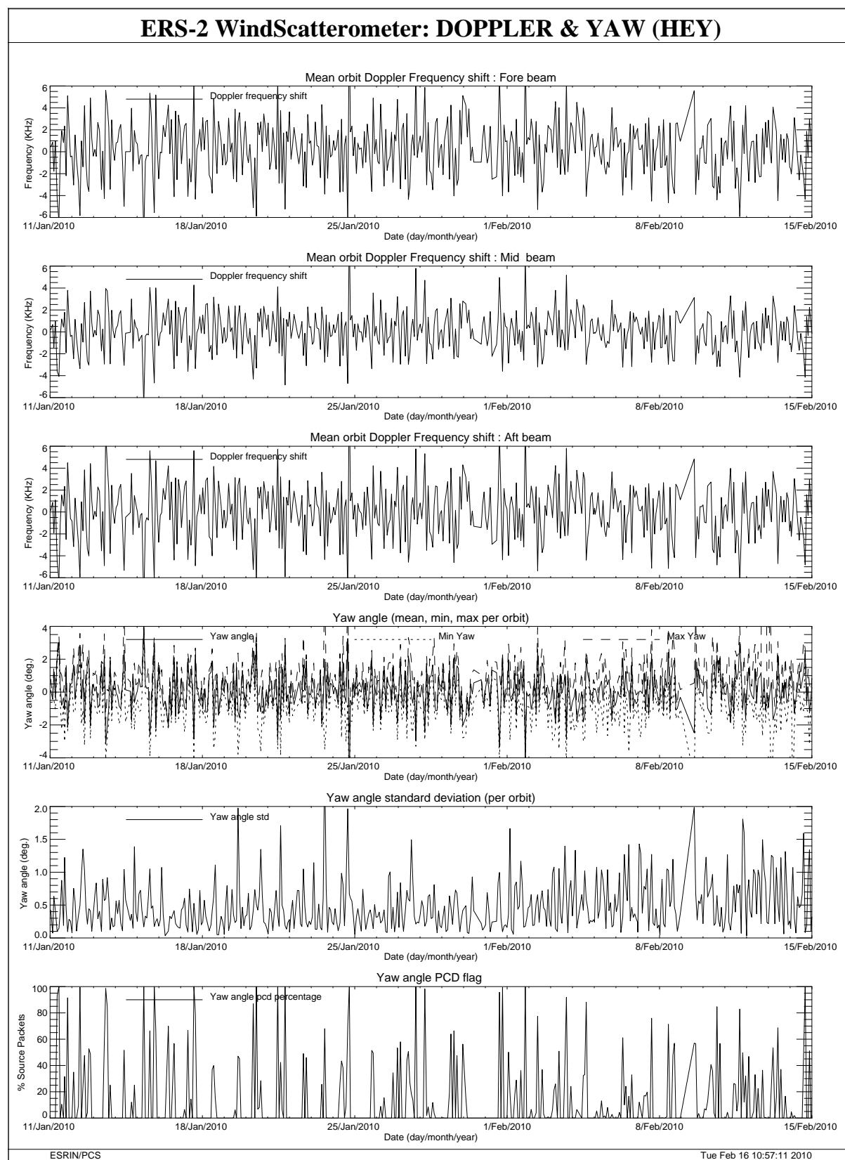
FIGURE 31 Doppler frequency shift and Yaw error angle evolution cycle 154.
