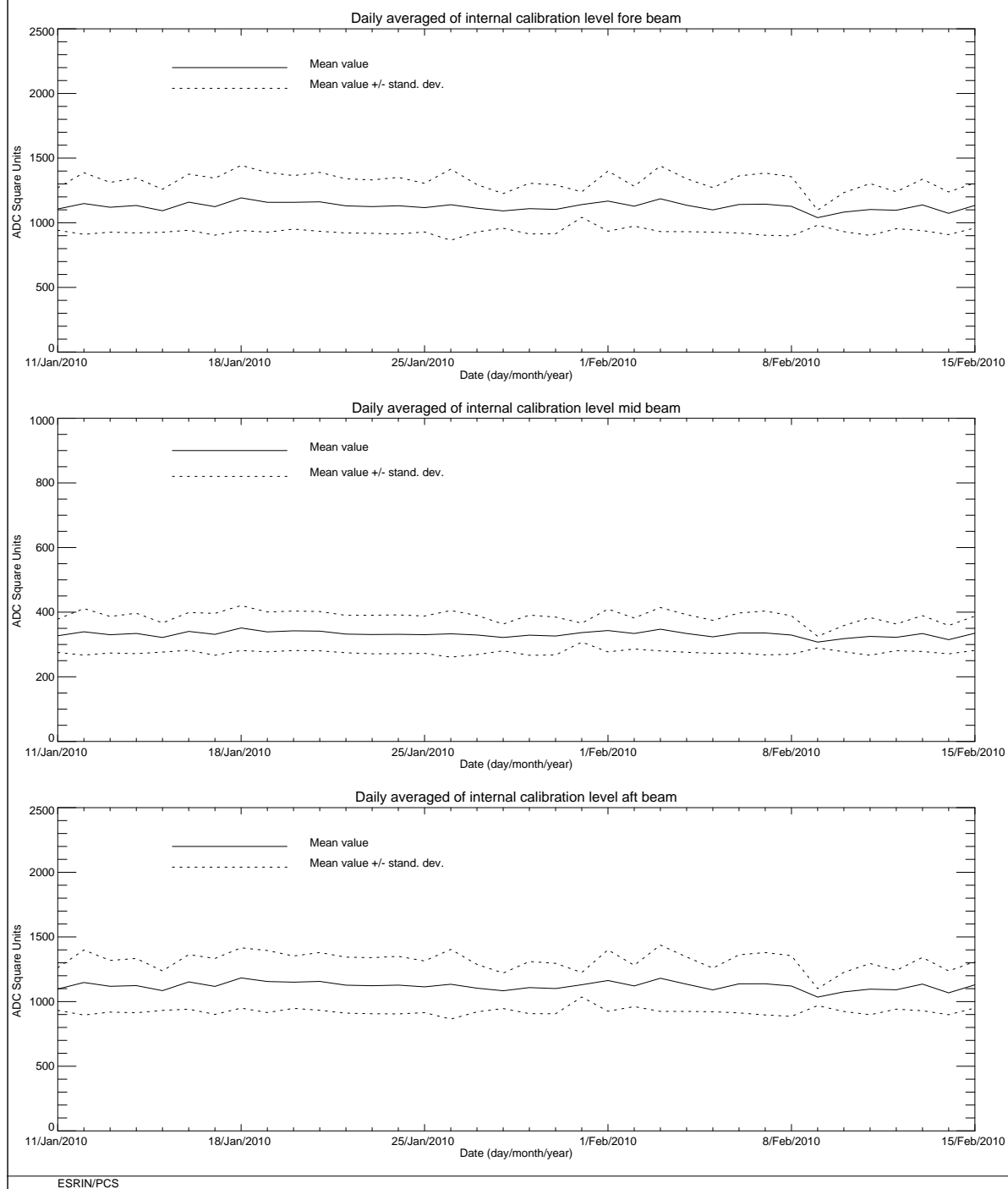
FIGURE 10 ERS-2 Scatterometer: power of internal calibration level cycle 154.
