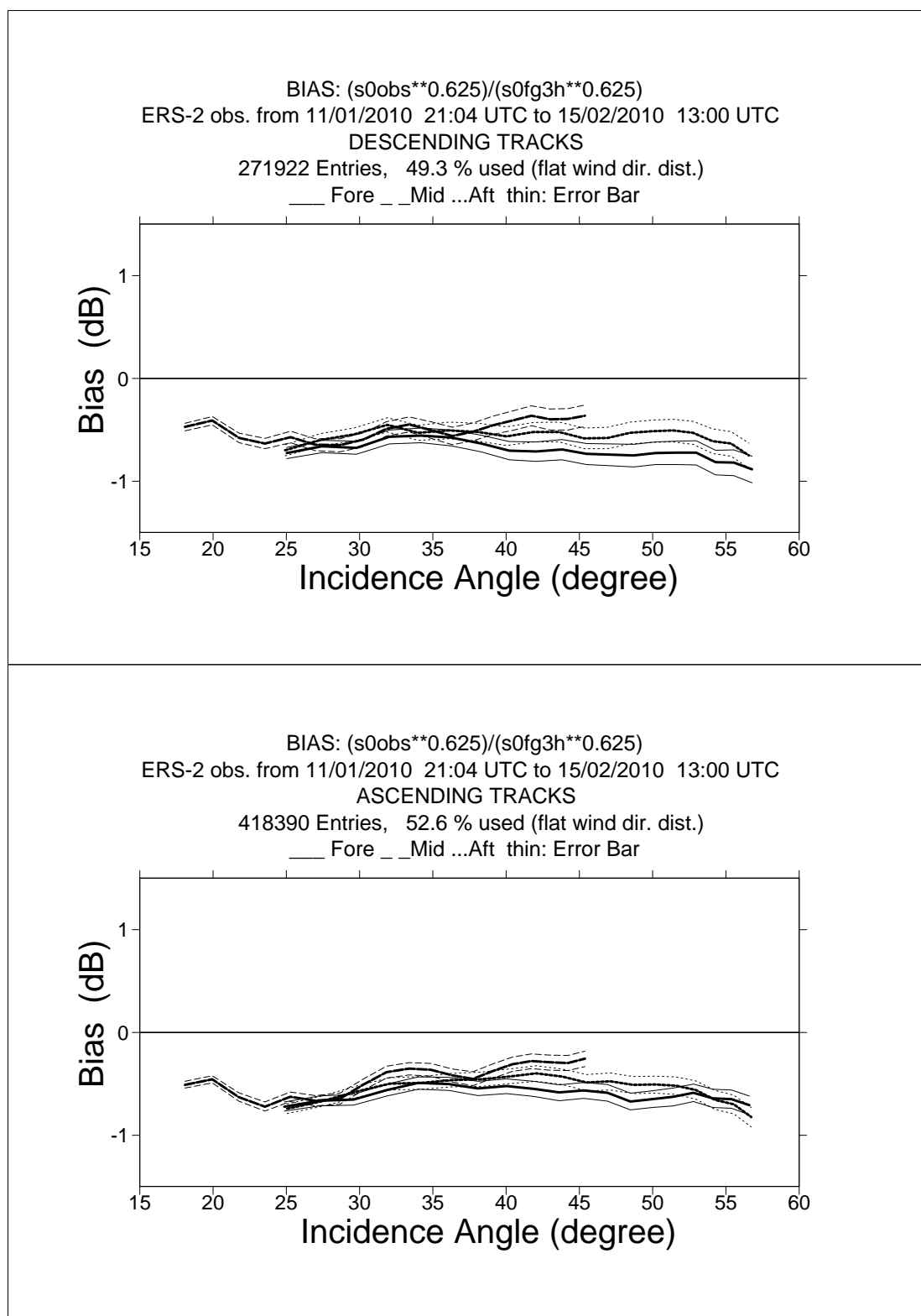
FIGURE 1 ERS-2 Scatterometer Ocean Calibration cycle 154. Ratio of \langle \sigma_0^{0.625} \rangle / \langle \text{CMOD4}(\text{First Guess})^{0.625} \rangle converted in dB for the fore beam (solid line), mid beam (dashed line) and aft beam (dotted line), as a function of incidence angle for descending and ascending tracks. The thin lines indicate the error bars on the estimated mean. First-guess winds are based on the in time closest (+3h, +6h, +9h, or +12h) T511 forecast field, and are bilinearly interpolated in space.
