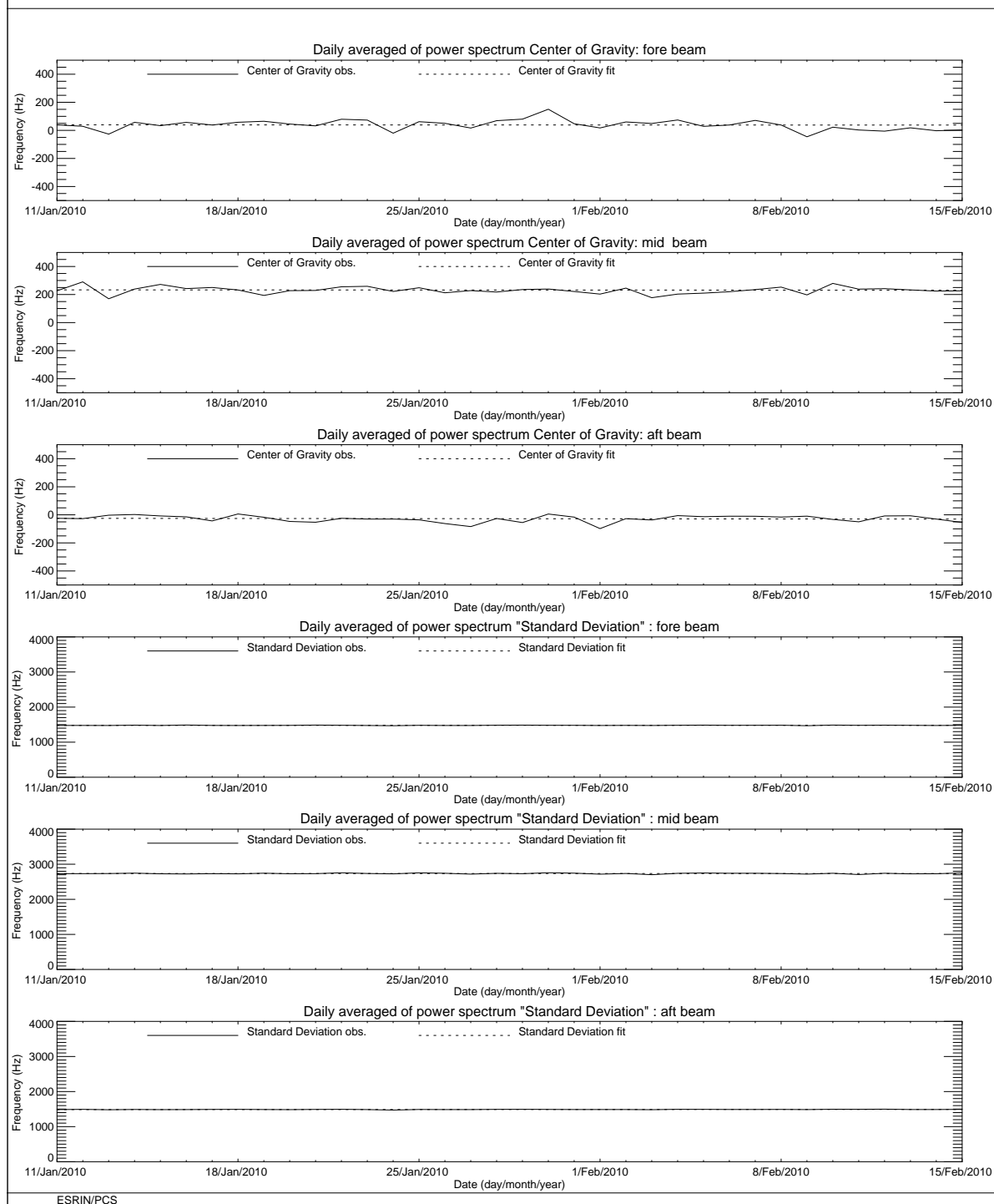
FIGURE 6 ERS-2 Scatterometer: Centre of Gravity and standard deviation of received power spectrum for cycle 154.
