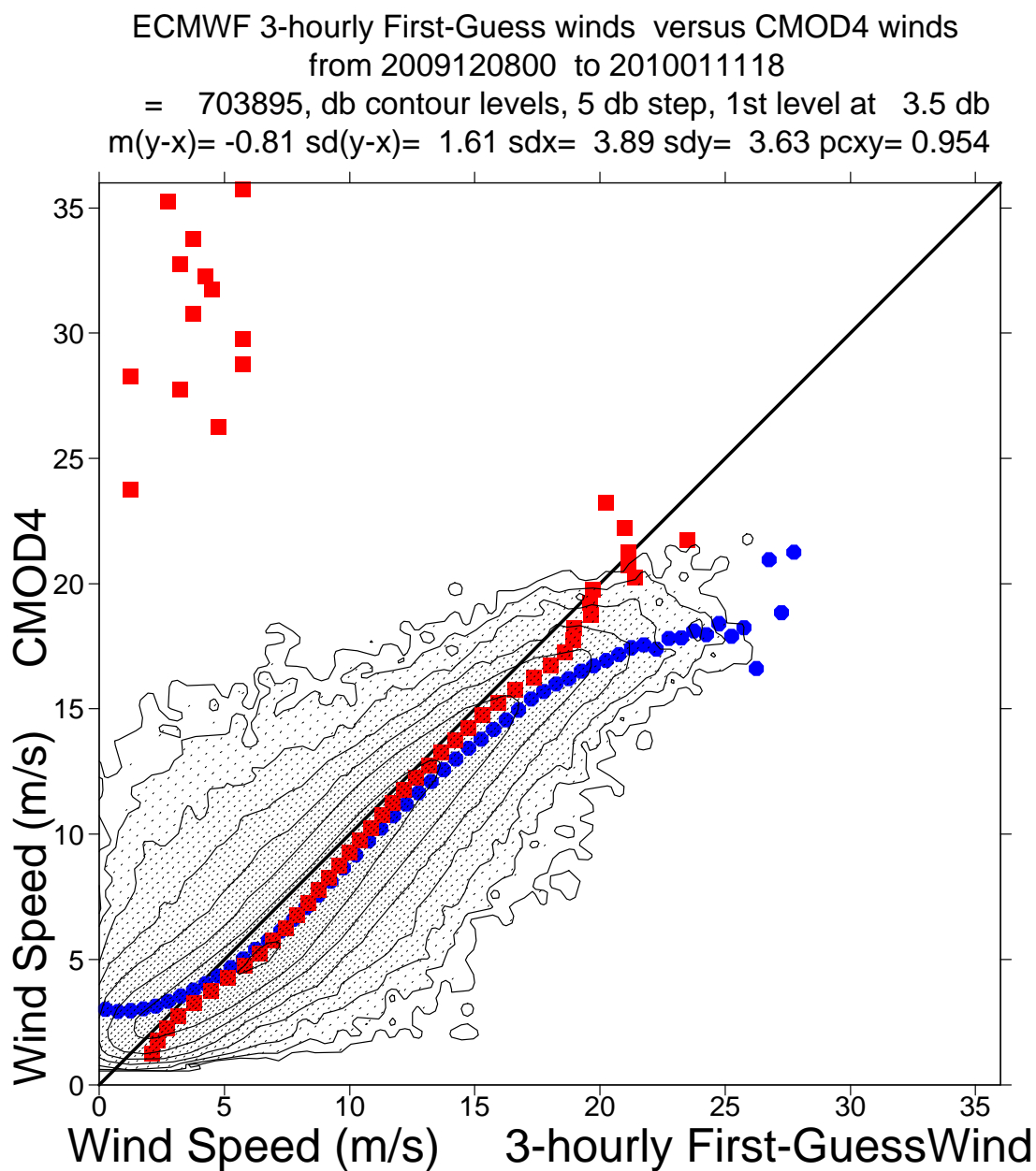
FIGURE 26 Same as Fig. 24, but for de-aliased CMOD4 winds.
