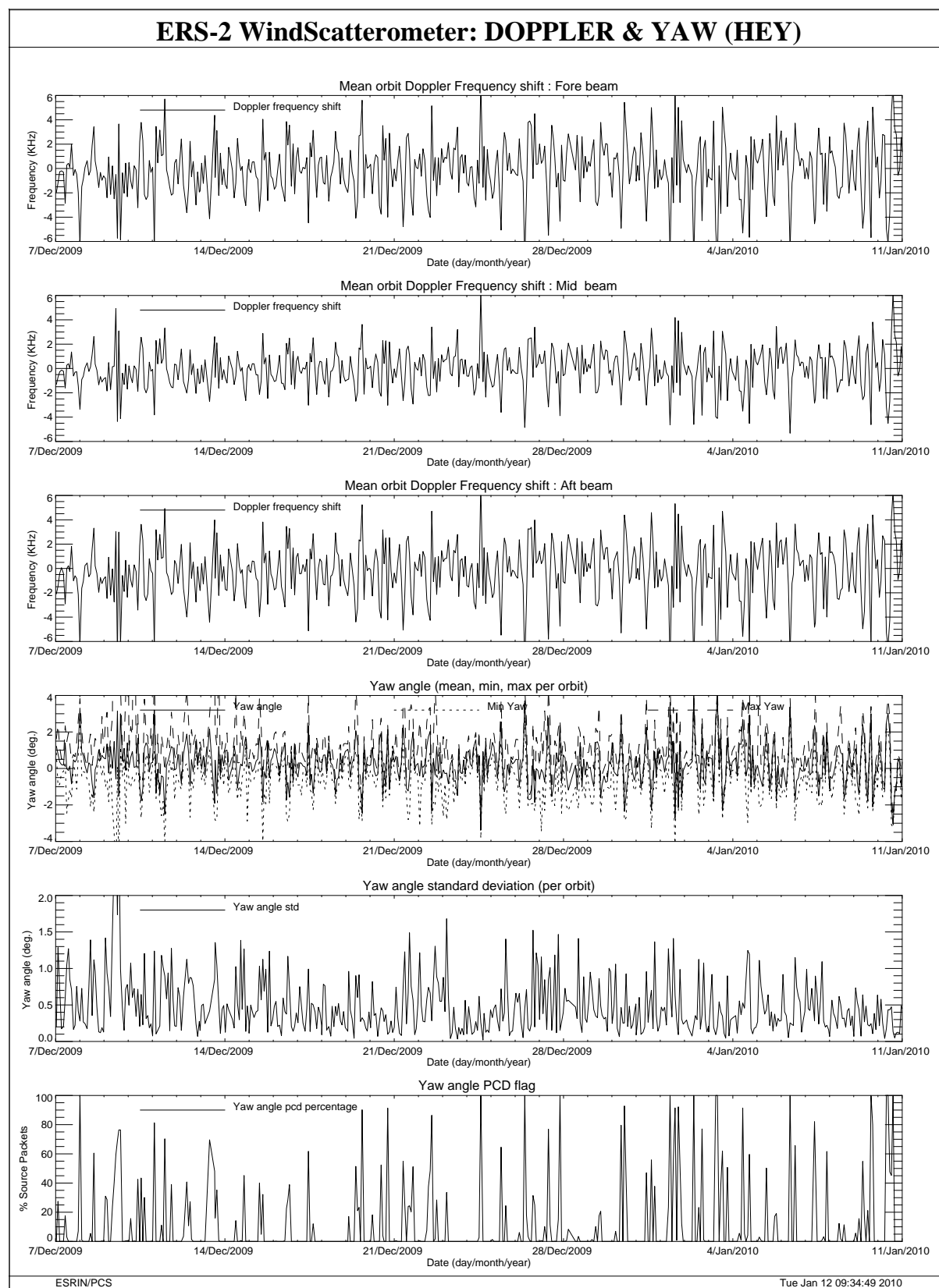
FIGURE 31 Doppler frequency shift and Yaw error angle evolution cycle 153.
