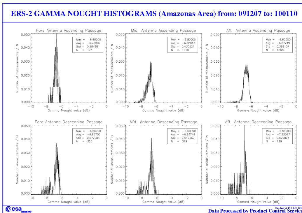
FIGURE 3 Gamma nought histograms over the Brazilian Rain Forest: cycle 153.
