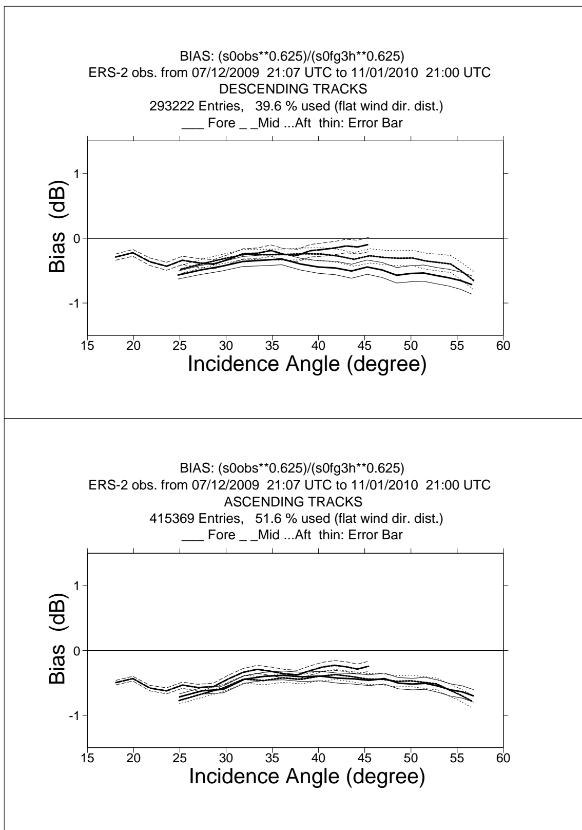
FIGURE 1 ERS-2 Scatterometer Ocean Calibration cycle 153. Ratio of \langle \sigma_0^{0.625} \rangle / \langle \text{CMOD4}(\text{First Guess})^{0.625} \rangle converted in dB for the fore beam (solid line), mid beam (dashed line) and aft beam (dotted line), as a function of incidence angle for descending and ascending tracks. The thin lines indicate the error bars on the estimated mean. First-guess winds are based on the in time closest (+3h, +6h, +9h, or +12h) T511 forecast field, and are bilinearly interpolated in space.
