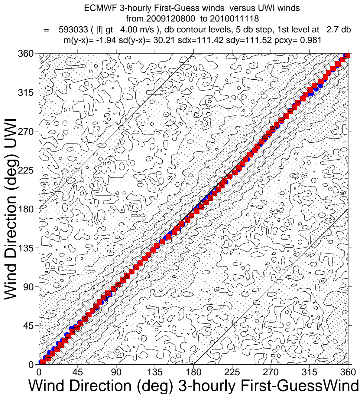
FIGURE 25 Same as Fig. 24, but for wind direction. Only wind speeds higher than 4m/s are taken into account.
