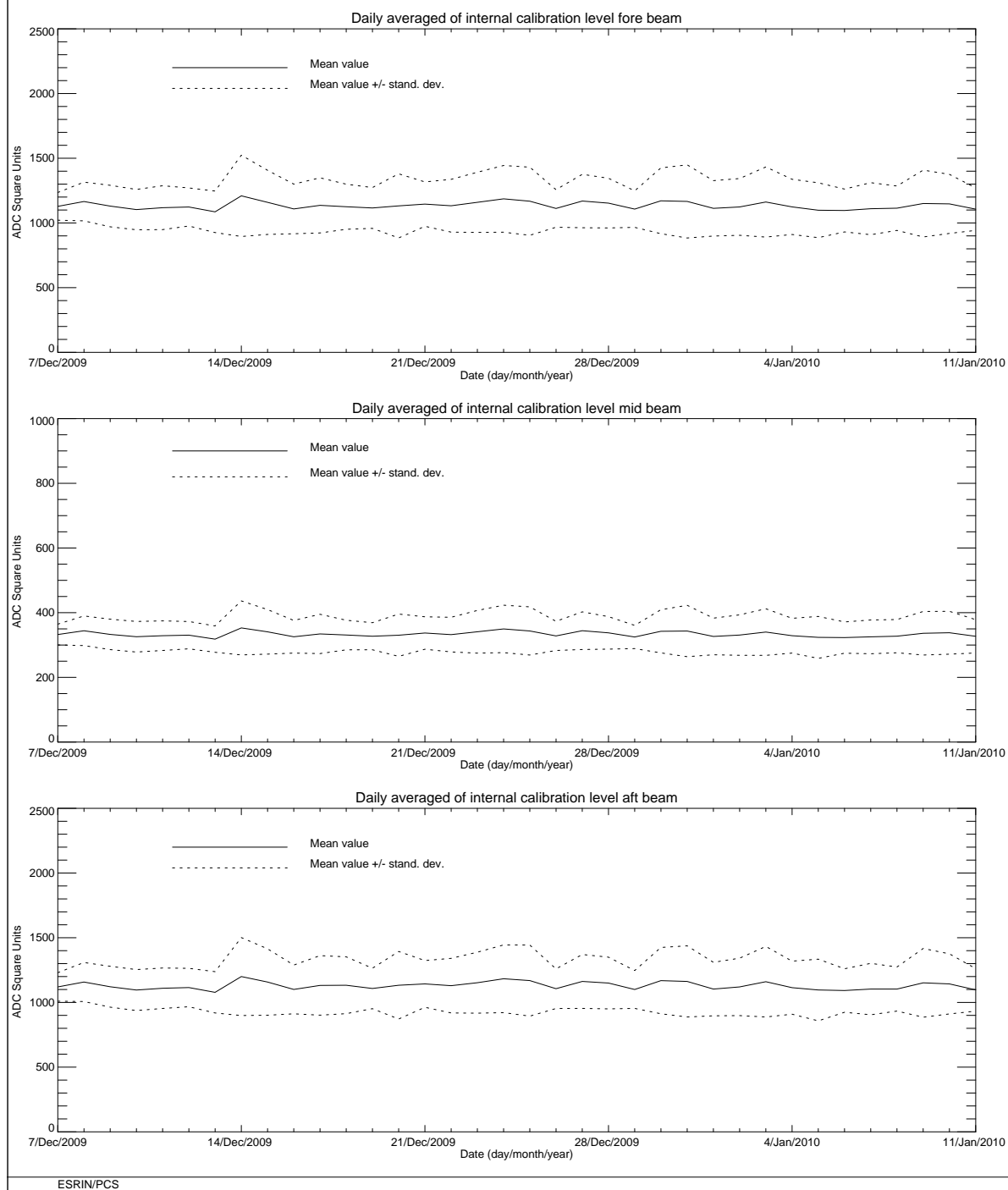
FIGURE 10 ERS-2 Scatterometer: power of internal calibration level cycle 153.
