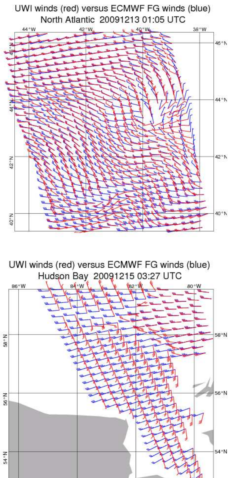
FIGURE 23 Comparison of UWI winds (in red) with ECMWF FG winds (in blue) for a case on 13 December 2009 (top panel) in the North Atlantic and a case on 15 December 2009 (lower panel) in the Hudson Bay.
