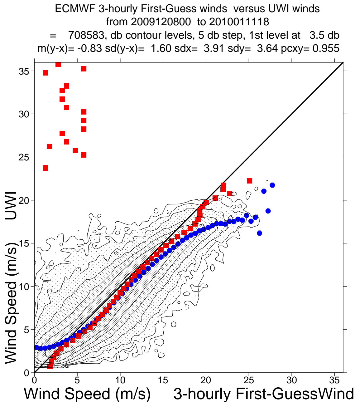
FIGURE 24 Two-dimensional histogram of first guess and UWI wind speeds, for the data kept by the UWI flags, and QC based on the ECMWF ice and land and sea-ice mask. Circles denote the mean values in the y-direction and squares those in the x-direction.
