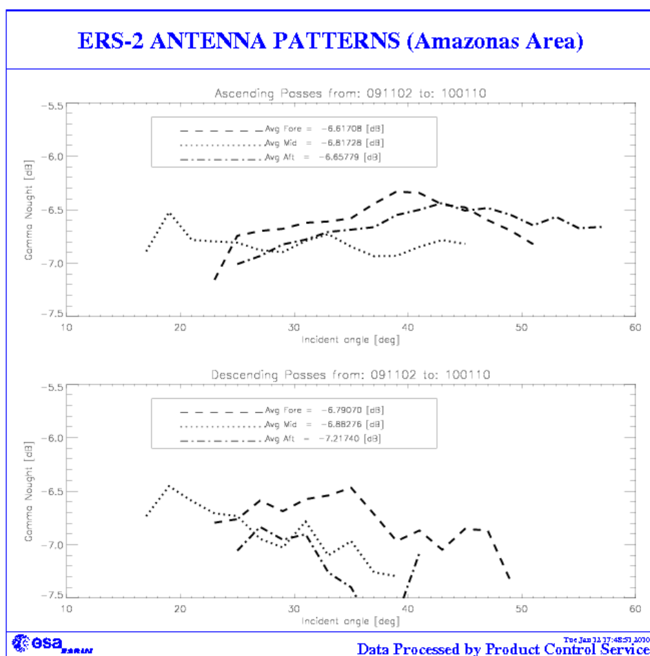
FIGURE 2 ERS-2 Scatterometer antenna pattern as function of the incidence angle: cycle 152 and 153.
