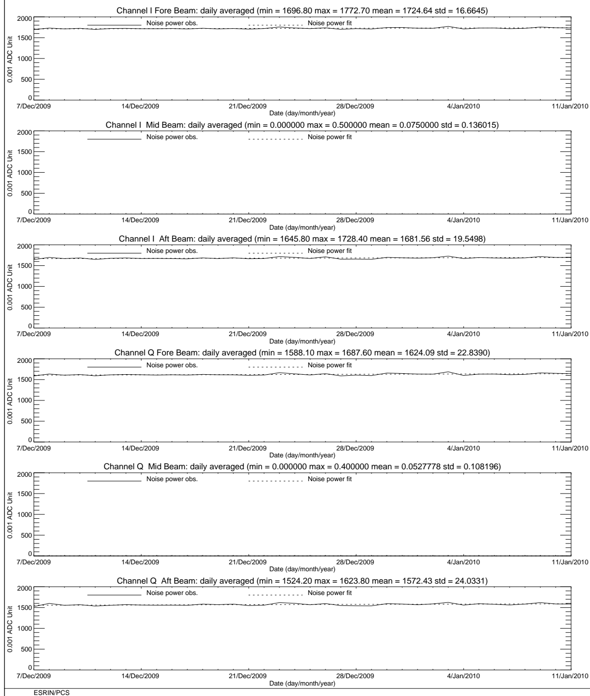
FIGURE 8 ERS-2 Scatterometer: noise power I and Q channel for cycle 153.
