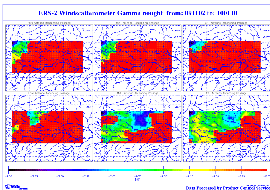
FIGURE 4 : ERS-2 Scatterometer: gamma nought over the Brazilian rain forest cycles 152 and 153.
