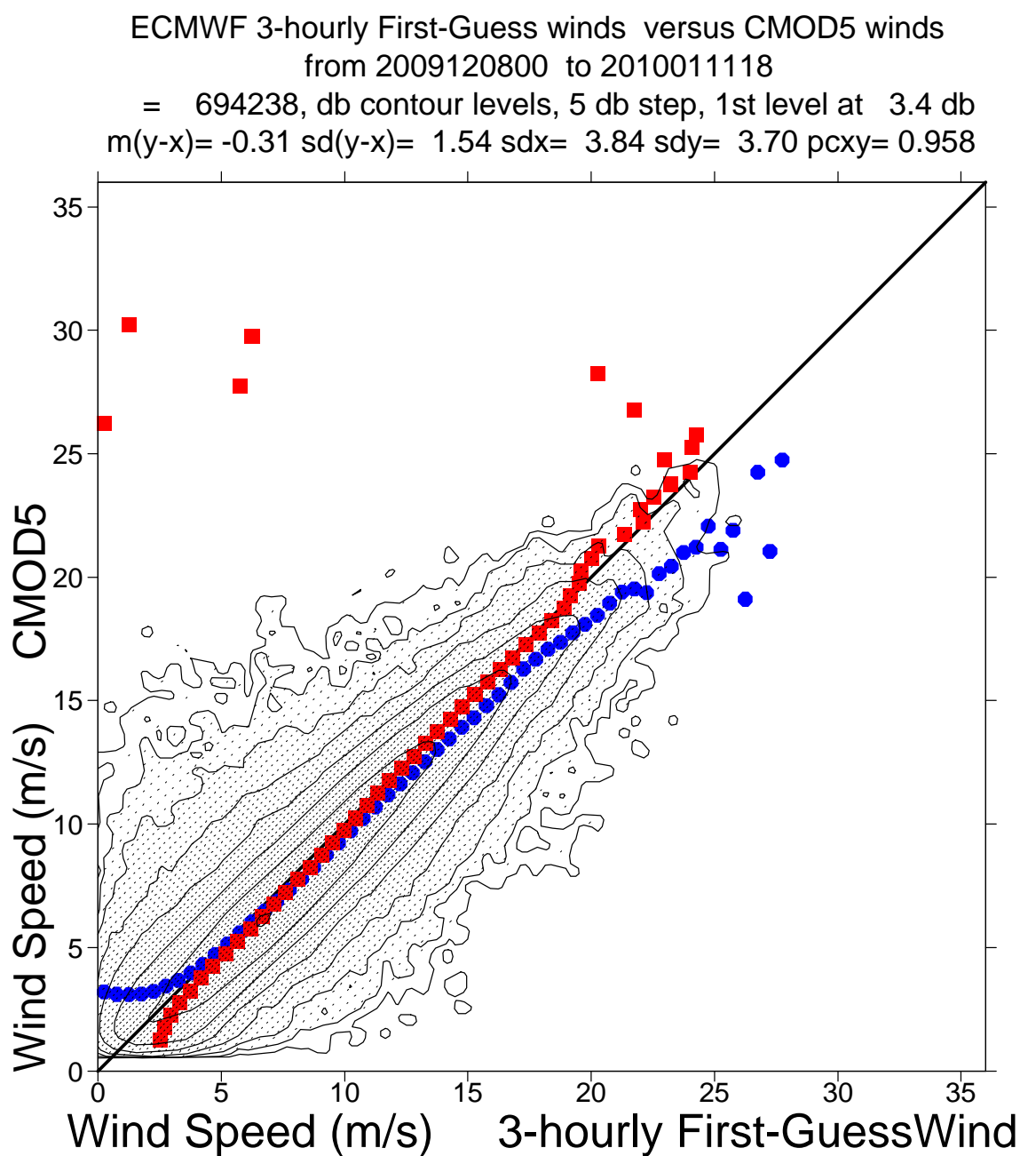
FIGURE 27 Same as Fig. 24, but for de-aliased CMOD5 winds.
