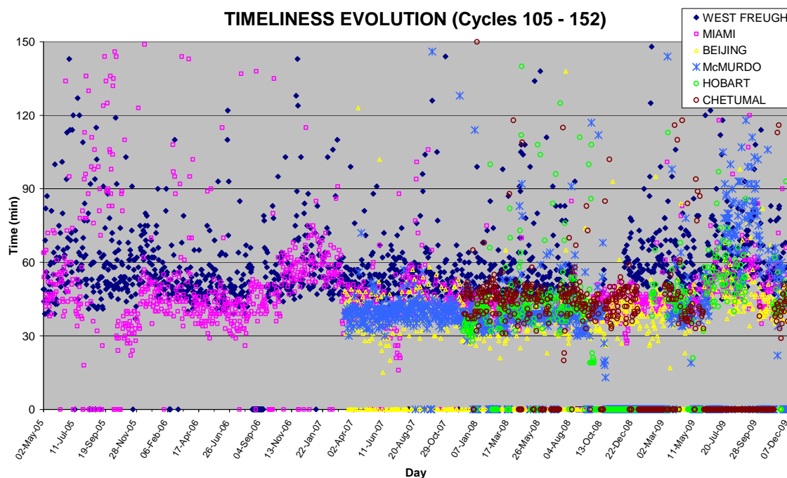
FIGURE 30 : Timeliness evolution from 19 th April 2005 to 7 th December 2009 for West Freugh, Miami, Beijing, McMurdo, Hobart and Chetumal ground stations.
