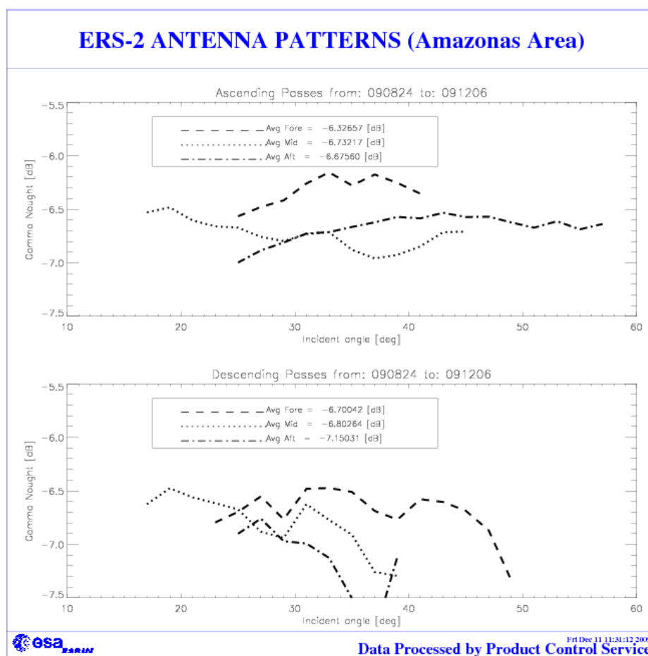
FIGURE 2 ERS-2 Scatterometer antenna pattern as function of the incidence angle: cycle 150, 151 and 152.
