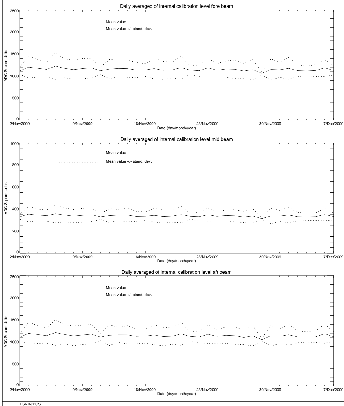
FIGURE 10 ERS-2 Scatterometer: power of internal calibration level cycle 152.
