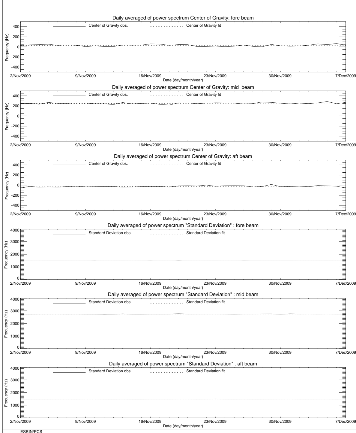
FIGURE 6 ERS-2 Scatterometer: Centre of Gravity and standard deviation of received power spectrum for cycle 152.
