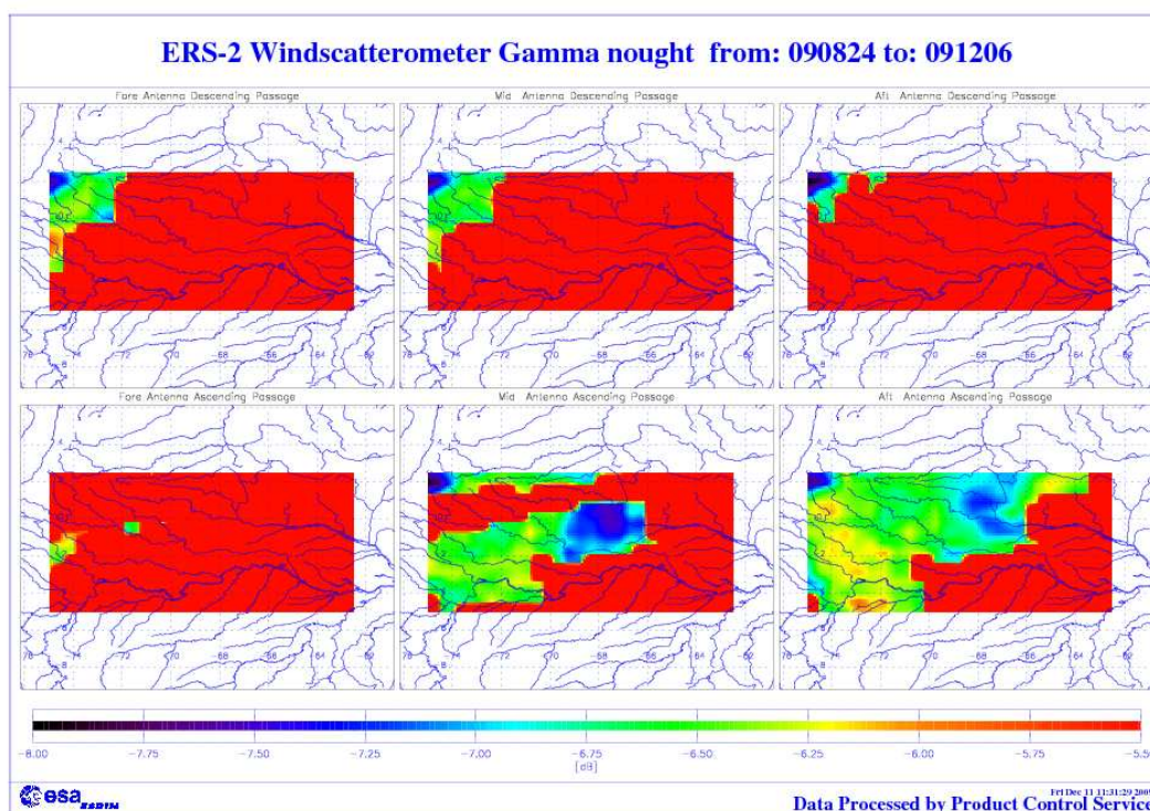
FIGURE 4 : ERS-2 Scatterometer: gamma nought over the Brazilian rain forest cycles 150, 151 and 152.
