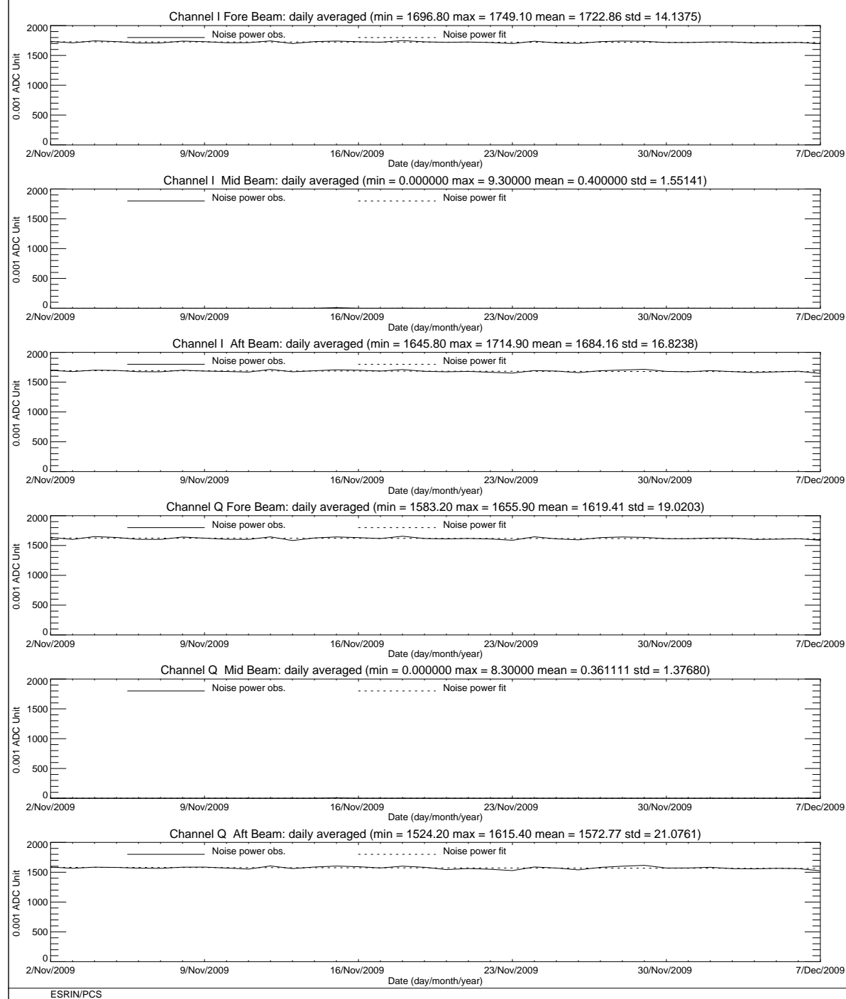
FIGURE 8 ERS-2 Scatterometer: noise power I and Q channel for cycle 152.
