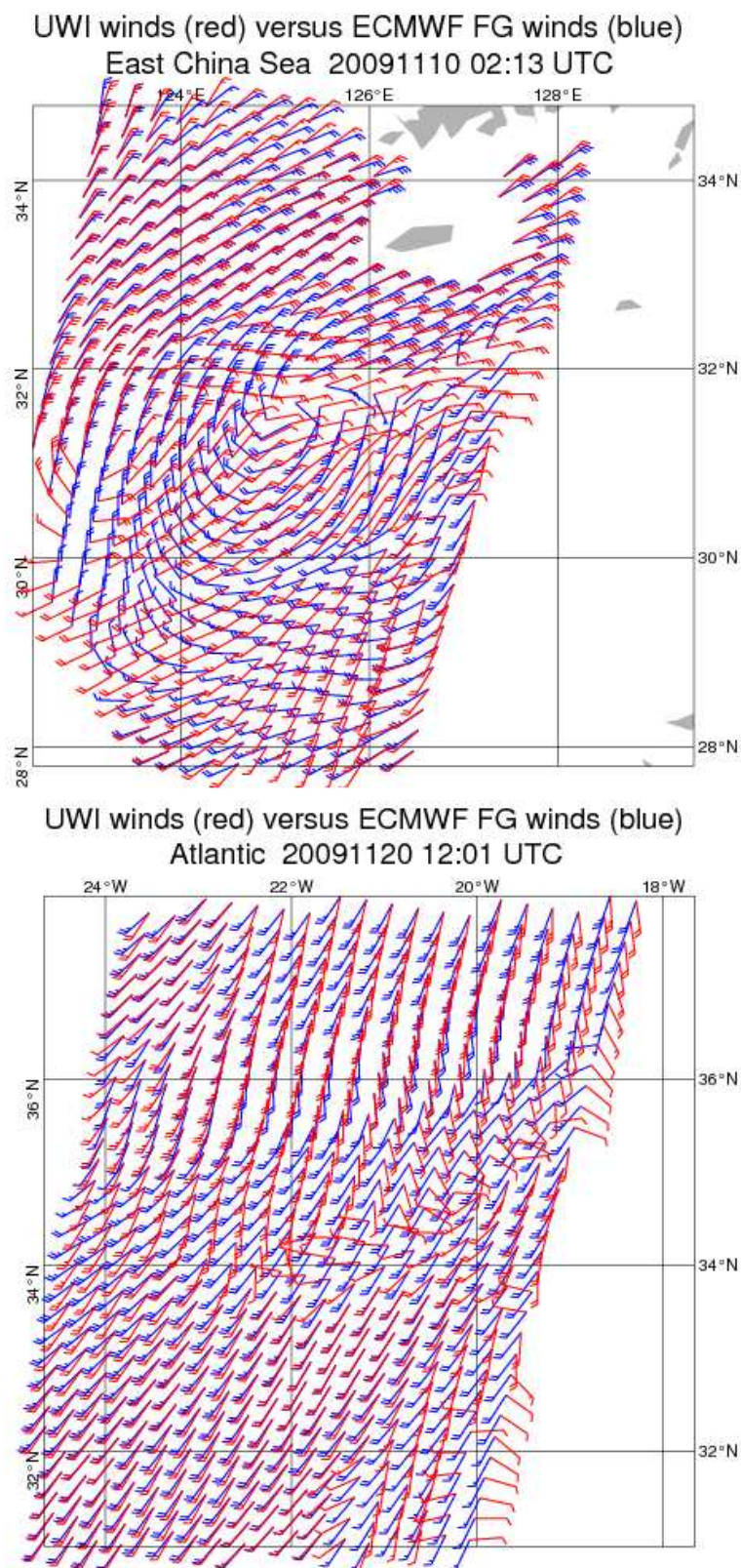
FIGURE 23 Comparison of UWI winds (in red) with ECMWF FG winds (in blue) for a case on 10 November 2009 (top panel) in the East Chinese Sea and a case on 20 November 2009 (lower panel) in the Atlantic.
