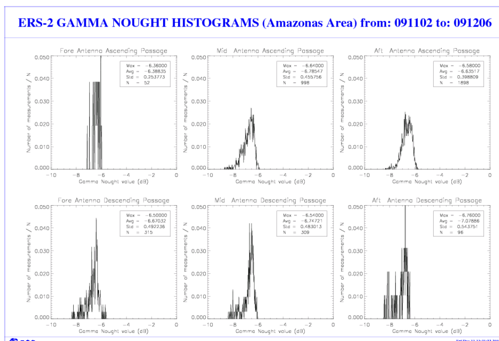
FIGURE 3 Gamma nought histograms over the Brazilian Rain Forest: cycle 152.
