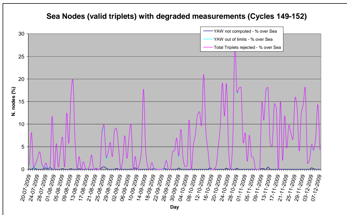
FIGURE 34 Statistics of degraded sigma nought triplets over Sea.
