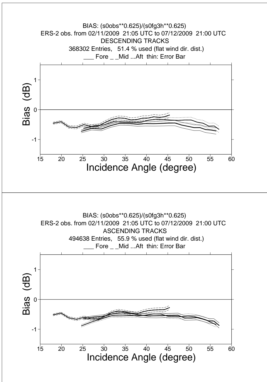
FIGURE 1 ERS-2 Scatterometer Ocean Calibration cycle 152. Ratio of \langle \sigma_0^{0.625} \rangle / \langle \text{CMOD4}(\text{First Guess})^{0.625} \rangle converted in dB for the fore beam (solid line), mid beam (dashed line) and aft beam (dotted line), as a function of incidence angle for descending and ascending tracks. The thin lines indicate the error bars on the estimated mean. First-guess winds are based on the in time closest (+3h, +6h, +9h, or +12h) T511 forecast field, and are bilinearly interpolated in space.
