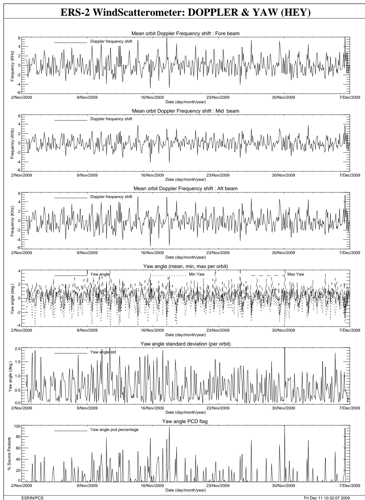
FIGURE 32 Doppler frequency shift and Yaw error angle evolution cycle 152.
