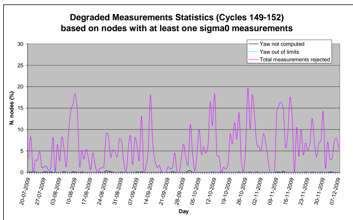
FIGURE 33 Statistics of sigma nought degraded measurements.
