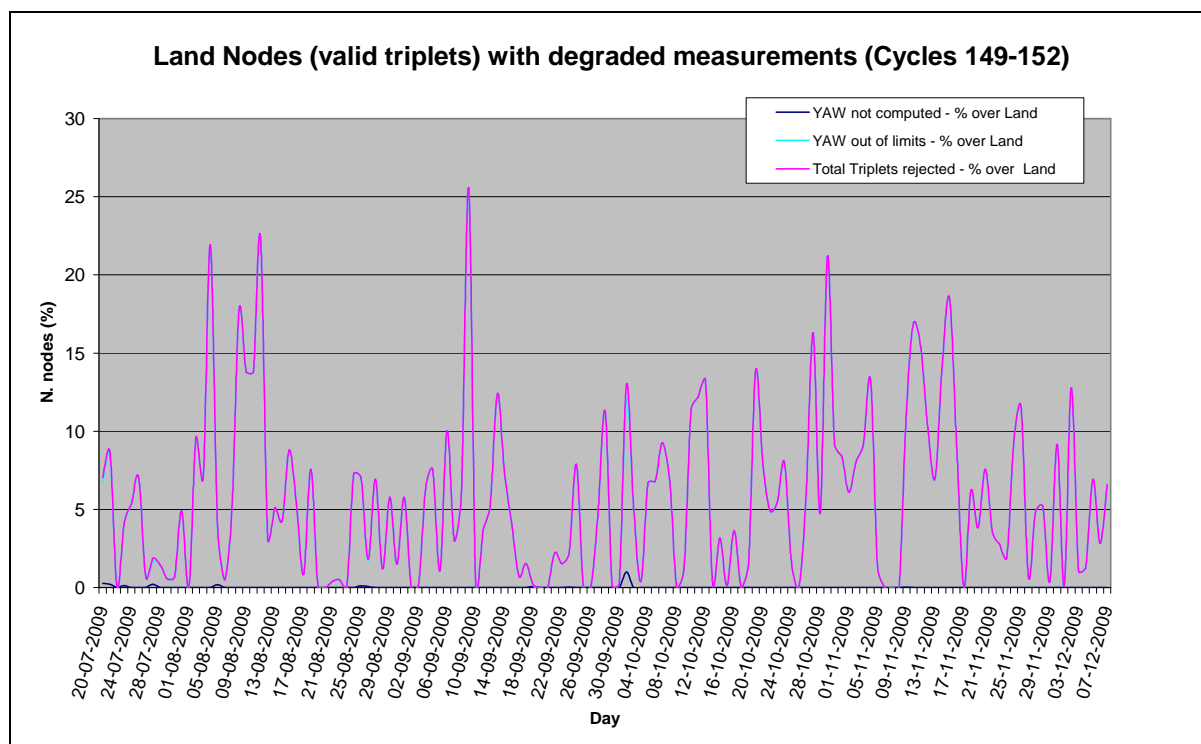
FIGURE 35 Statistics of degraded sigma nought triplets over Land.
