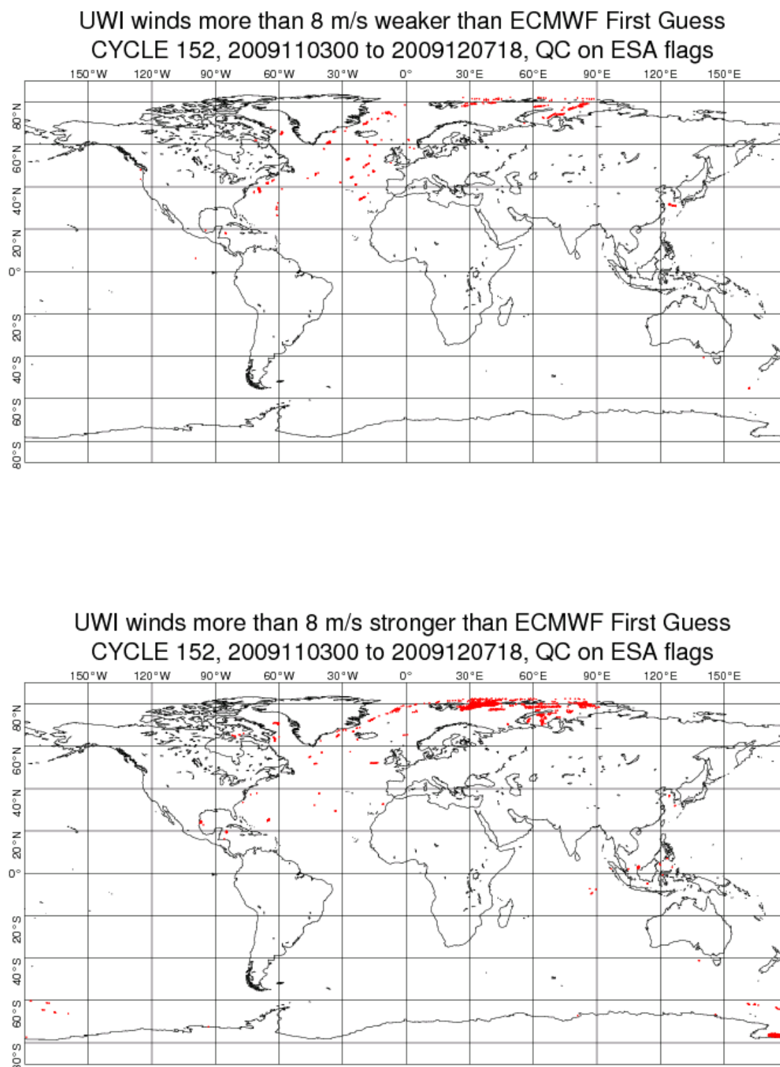
FIGURE 22 Locations of data during cycle 152 for which UWI winds are more than 8 m/s weaker (top panel) respectively stronger (lower panel) than FGAT, and on which QC on UWI flags and the ECMWF land/sea-ice mask was applied.
