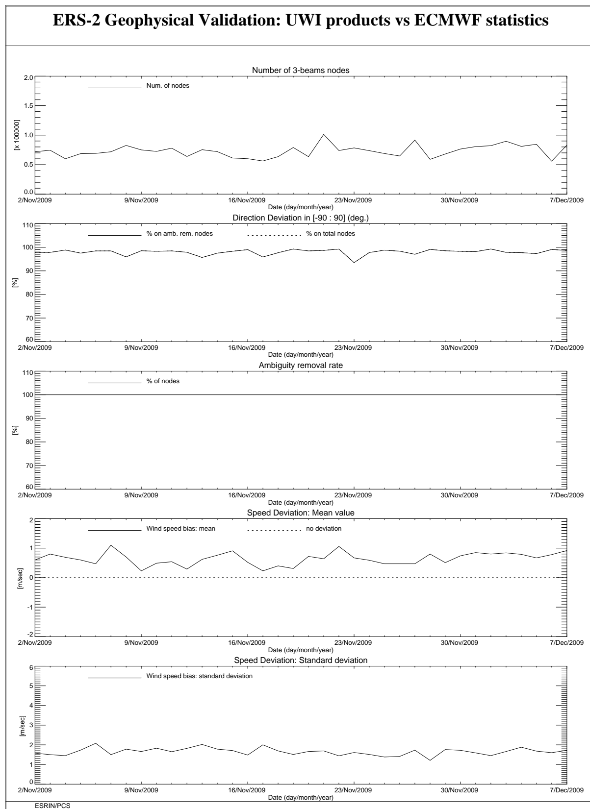
FIGURE 13 ERS-2 Scatterometer: wind products performance for cycle 152.
