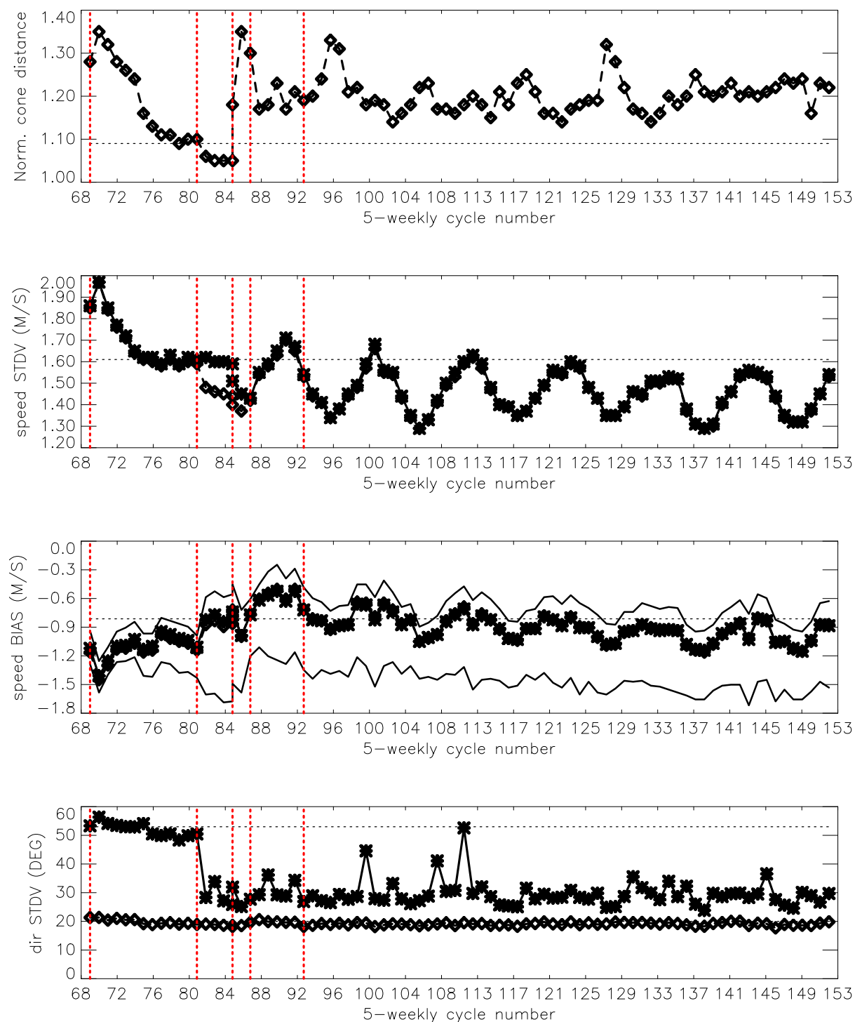
FIGURE 14 Evolution of the performance of the ERS-2 Scatterometer averaged over 5-weekly cycles from 12 December 2001 (cycle 69) to 7 December 2009 (end cycle 152) for the UWI product (solid, star) and de-aliased winds based on CMOD4 (dashed, diamond). Results are based on data that passed the UWI QC flags. For cycle 85 two values are plotted; the first value for the global set, the second one for the regional set. Dotted lines represent values for cycle 59 (5 December 2000 to 17 January 2001), i.e. the last stable cycle of the nominal period. From top to bottom panel are shown the normalized distance to the one (CMOD4 only) the standard deviation of the wind speed compared to FG winds, the corresponding bias (for UWI winds the extreme inter-node averages are shown as well), and the standard deviation of wind direction compared to FG.
