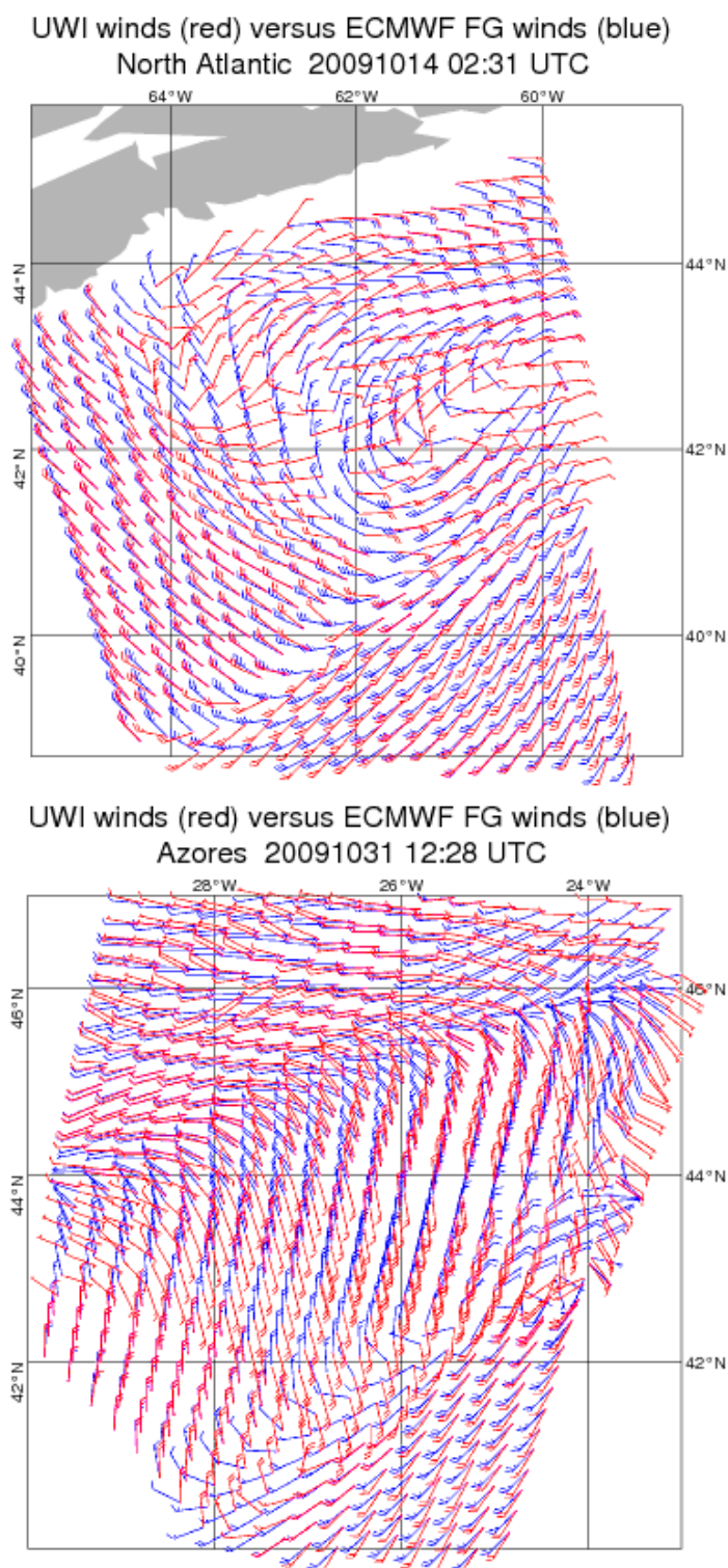
FIGURE 23 Comparison between Comparison of UWI winds (in red) with ECMWF FG winds (in blue) for a case on 14 October 2009 (top panel) in the Atlantic and a case on 31 October 2009 (lower panel) near The Azores.
