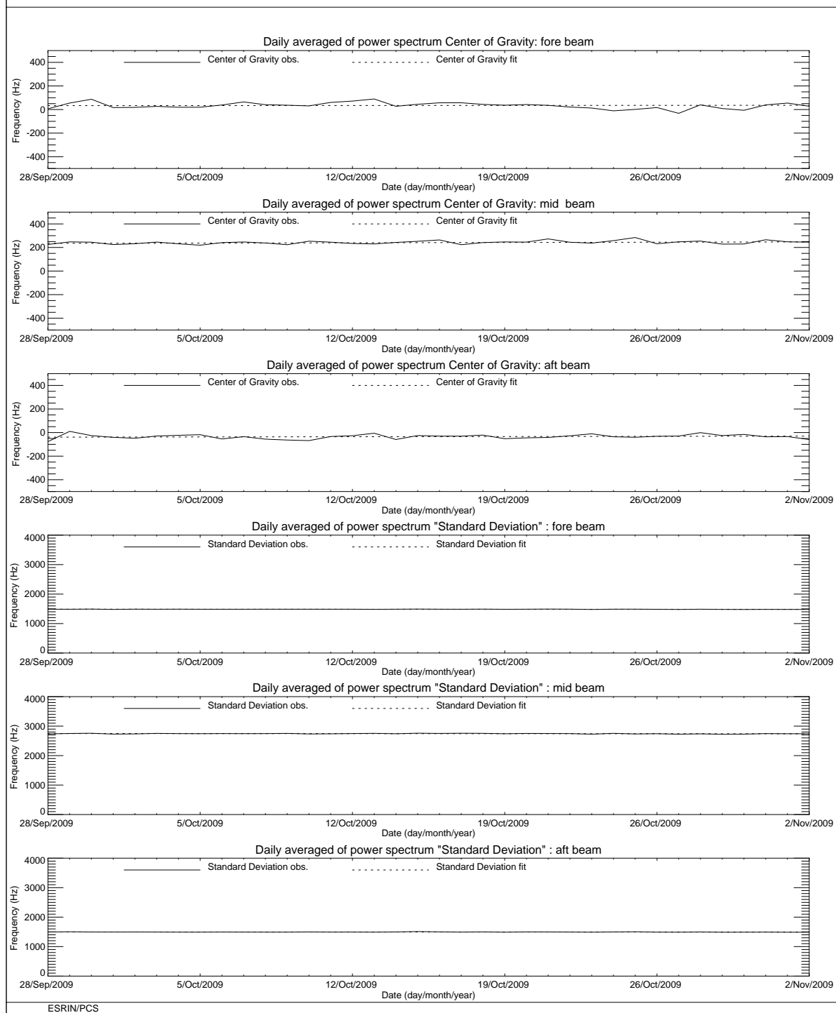
FIGURE 6 ERS-2 Scatterometer: Centre of Gravity and standard deviation of received power spectrum for cycle 151.
