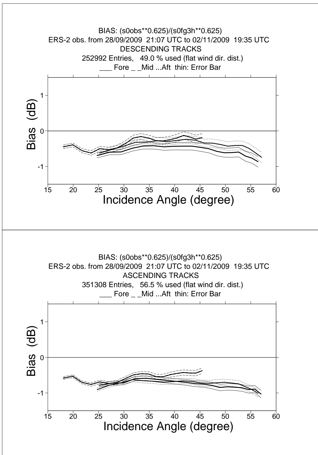
FIGURE 1 ERS-2 Scatterometer Ocean Calibration cycle 151. Ratio of \langle \sigma_0^{0.625} \rangle / \langle \text{CMOD4(First Guess)}^{0.625} \rangle converted in dB for the fore beam (solid line), mid beam (dashed line) an aft beam (dotted line), as a function of incidence angle for descending and ascending tracks. The thin lines indicate the error bars on the estimated mean. First-guess winds are based on the in time closest (+3h, +6h, +9h, or +12h) T511 forecast field, and are bilinearly interpolated in space.
