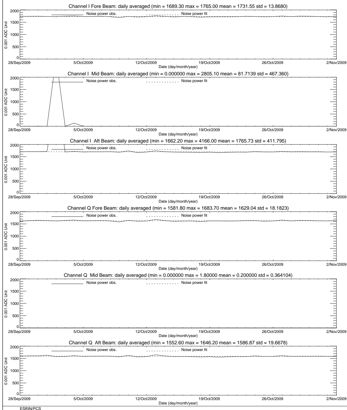
FIGURE 8 ERS-2 Scatterometer: noise power I and Q channel for cycle 151.
