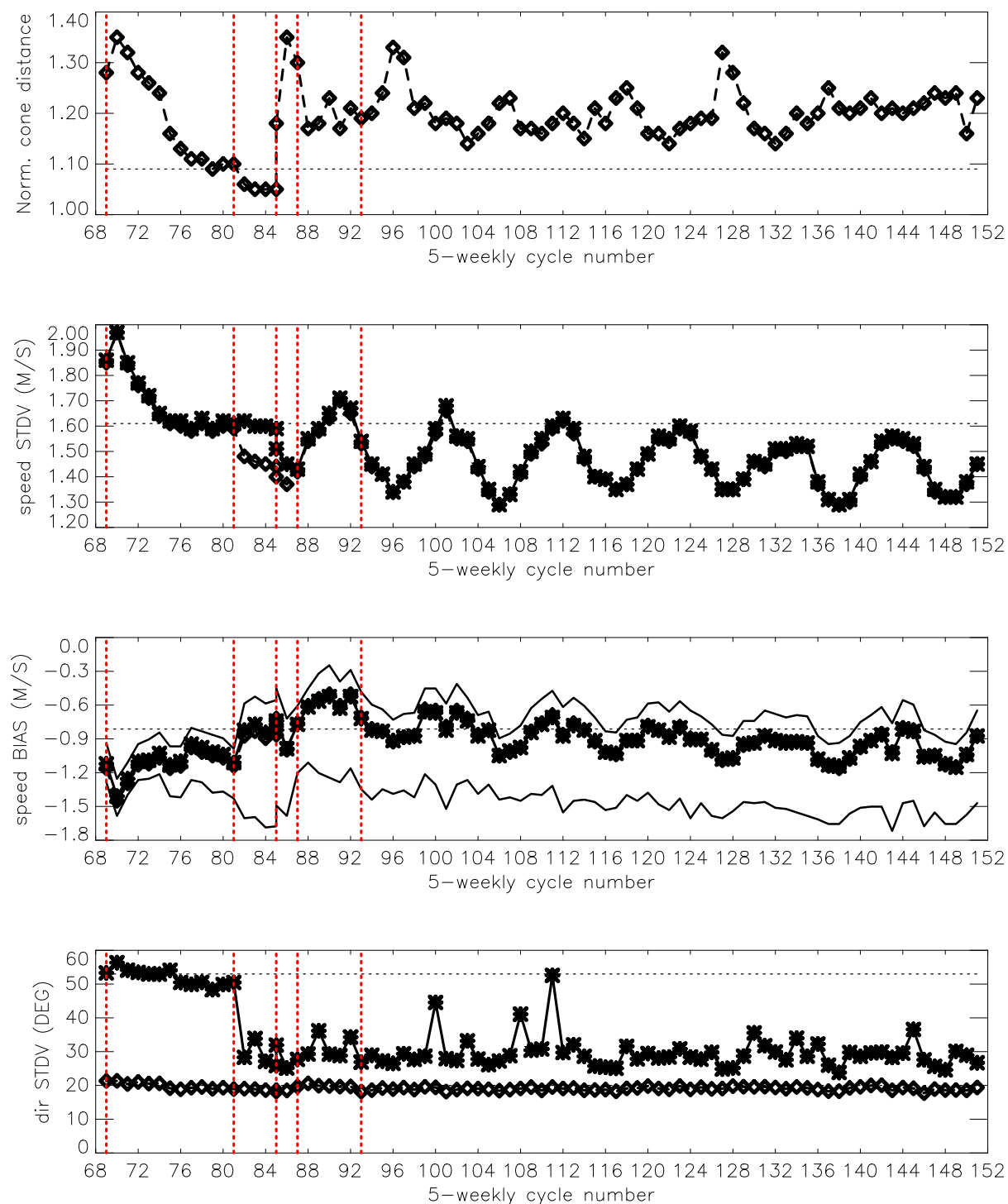
FIGURE 14 Evolution of the performance of the ERS-2 Scatterometer averaged over 5-weekly cycles from 12 December 2001 (cycle 69) to 2 November 2009 (end cycle 151) for the UWI product (solid, star) and de-aliased winds based on CMOD4 (dashed, diamond). Results are based on data that passed the UWI QC flags. For cycle 85 two values are plotted; the first value for the global set, the second one for the regional set. Dotted lines represent values for cycle 59 (5 December 2000 to 17 January 2001), i.e. the last stable cycle of the nominal period. From top to bottom panel are shown the normalized distance to the one (CMOD4 only) the standard deviation of the wind speed compared to FG winds, the corresponding bias (for UWI winds the extreme inter-node averages are shown as well), and the standard deviation of wind direction compared to FG.
