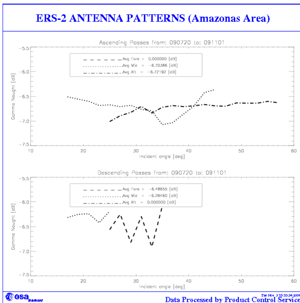
FIGURE 2 ERS-2 Scatterometer antenna pattern as function of the incidence angle: cycle 149, 150 and 151.
