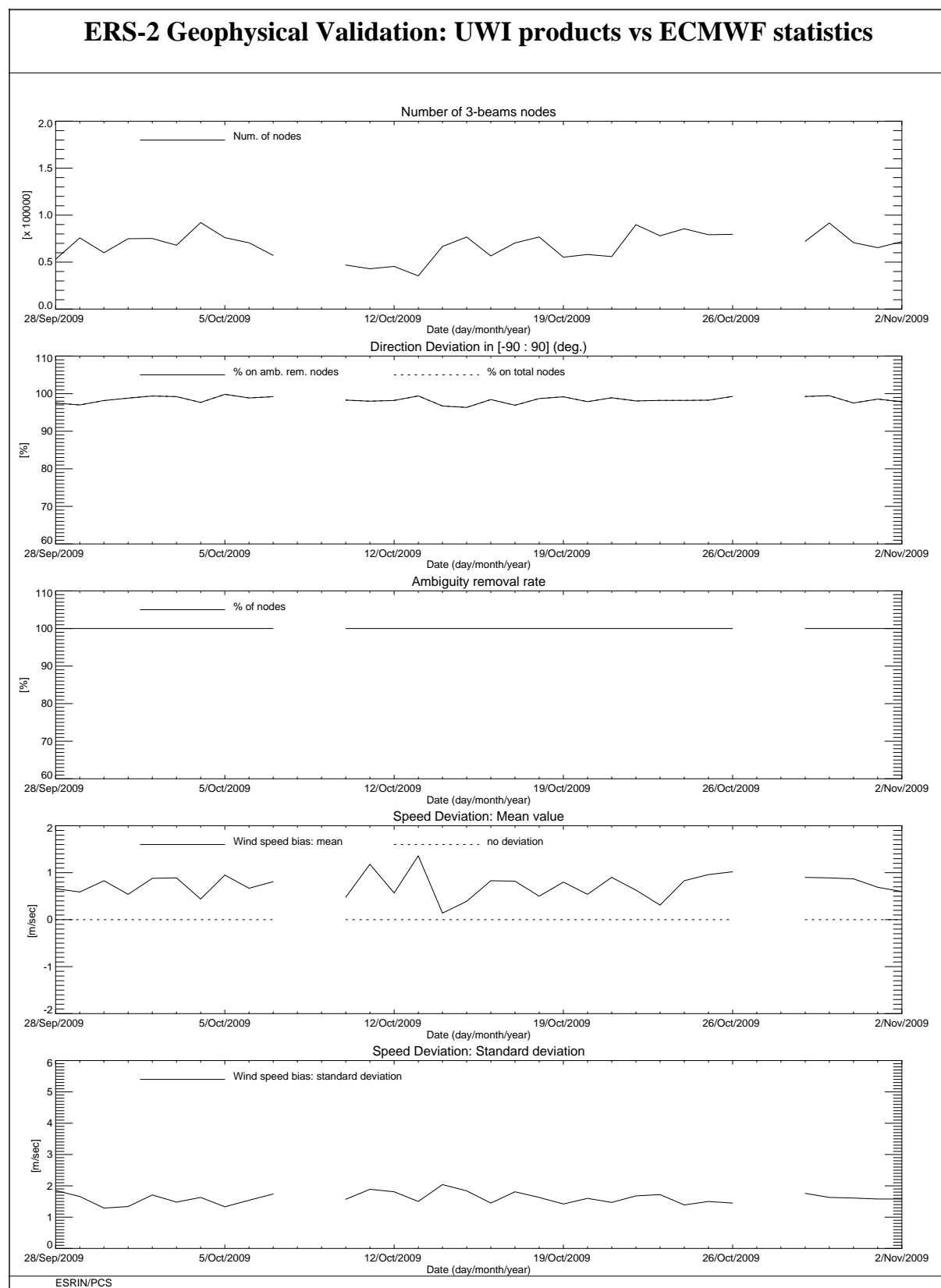
FIGURE 13 ERS-2 Scatterometer: wind products performance for cycle 151.
