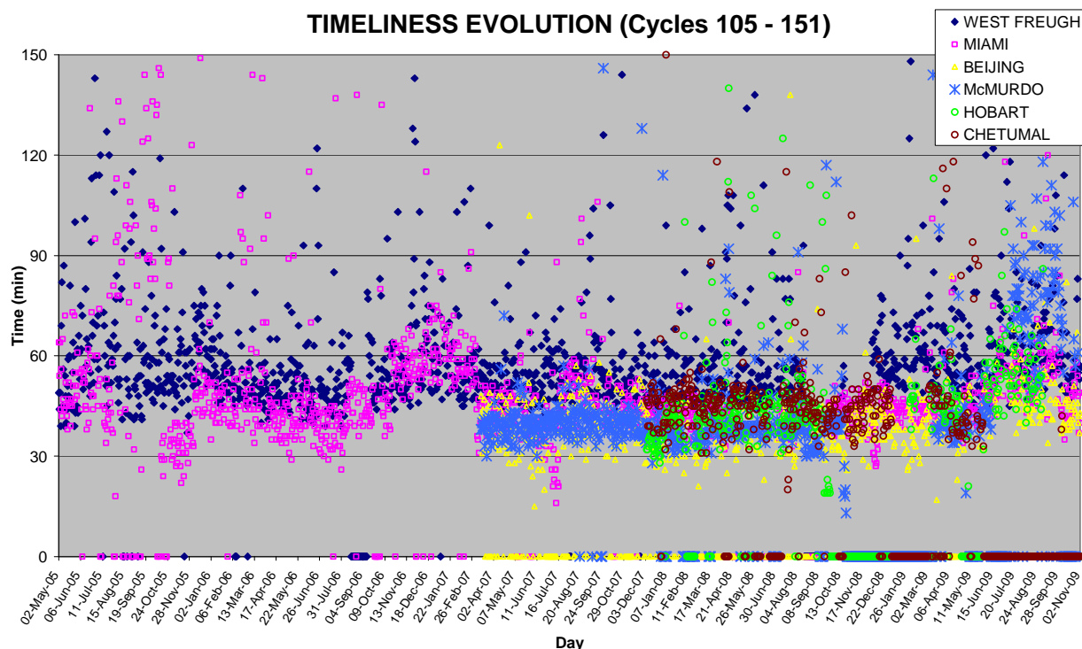
FIGURE 30 : Timeliness evolution from 19 th April 2005 to 2 nd November 2009 for West Freugh, Miami, Beijing, McMurdo, Hobart and Chetumal ground stations.
