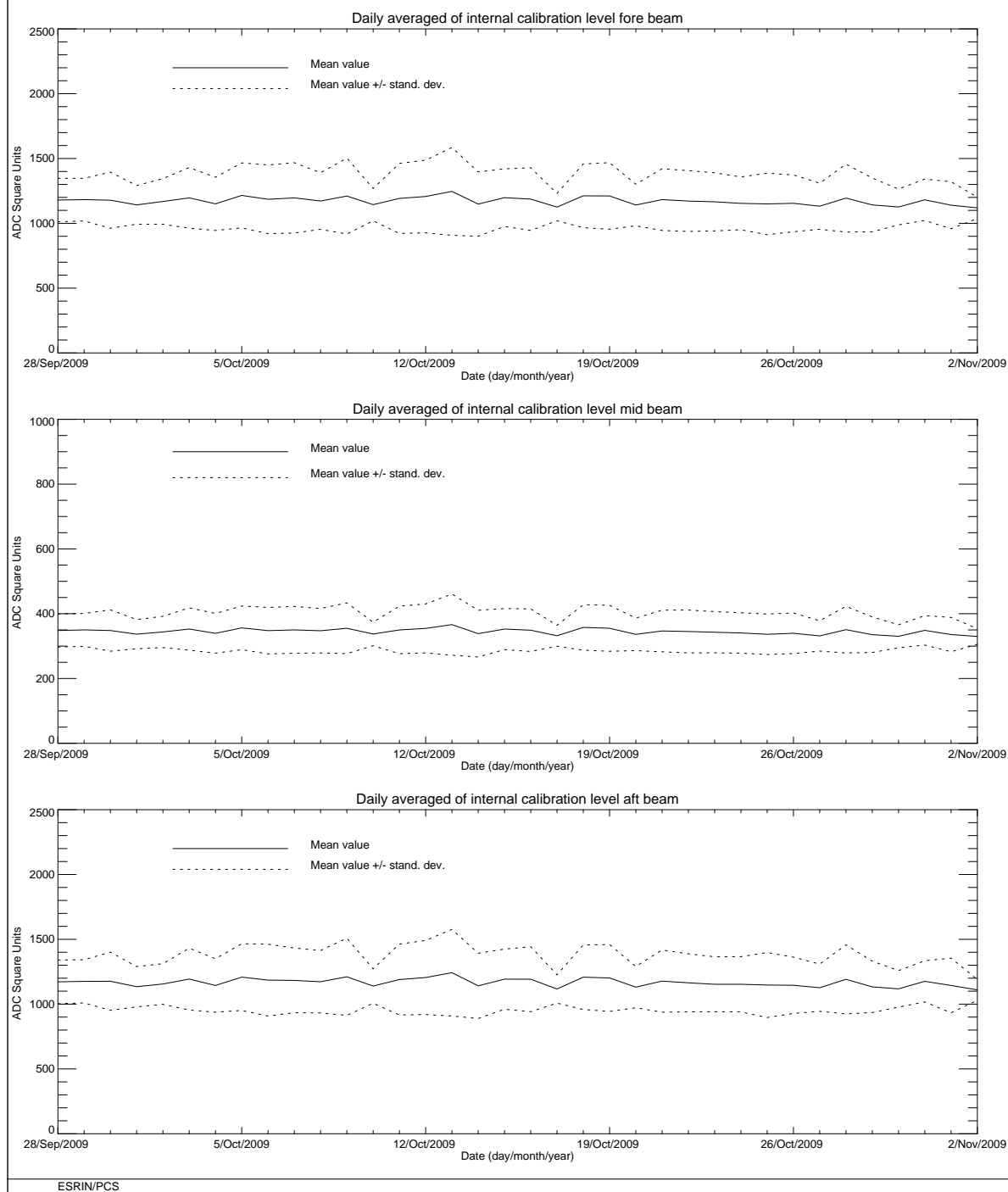
FIGURE 10 ERS-2 Scatterometer: power of internal calibration level cycle 151.
