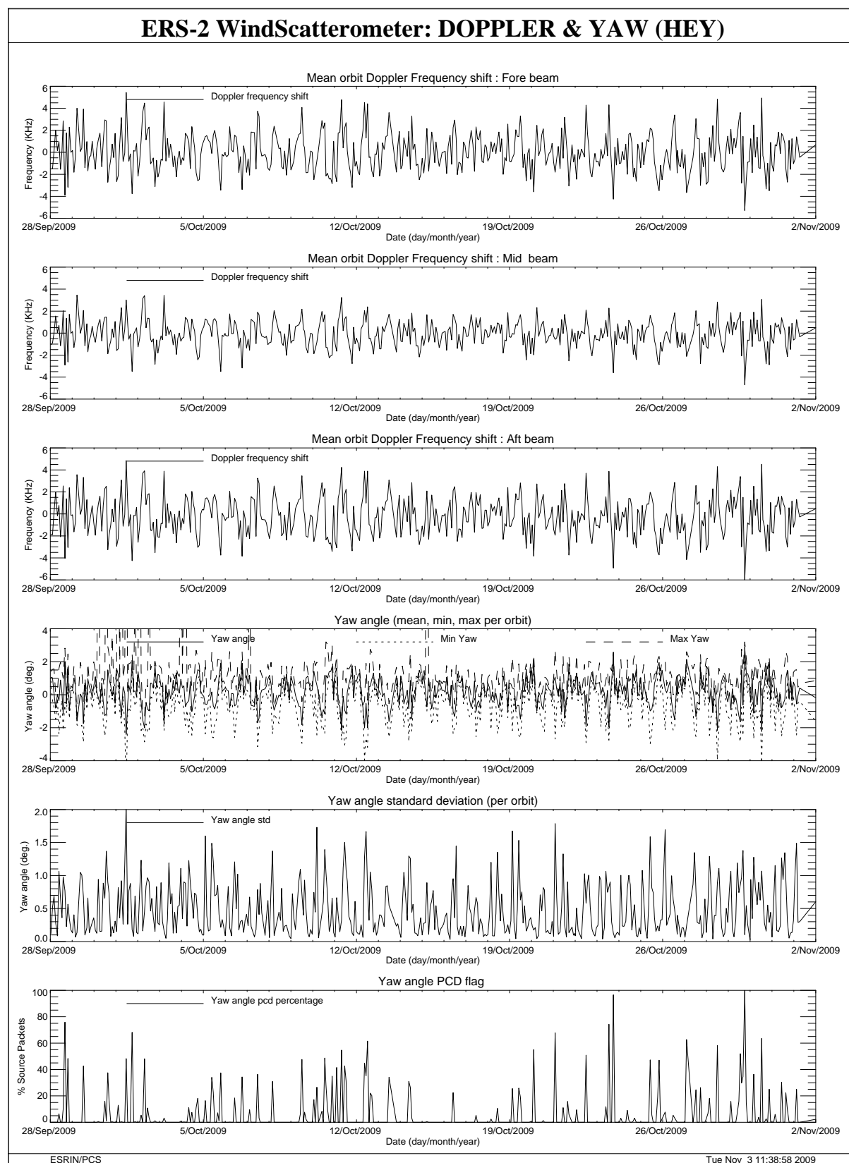
FIGURE 32 Doppler frequency shift and Yaw error angle evolution cycle 151.
