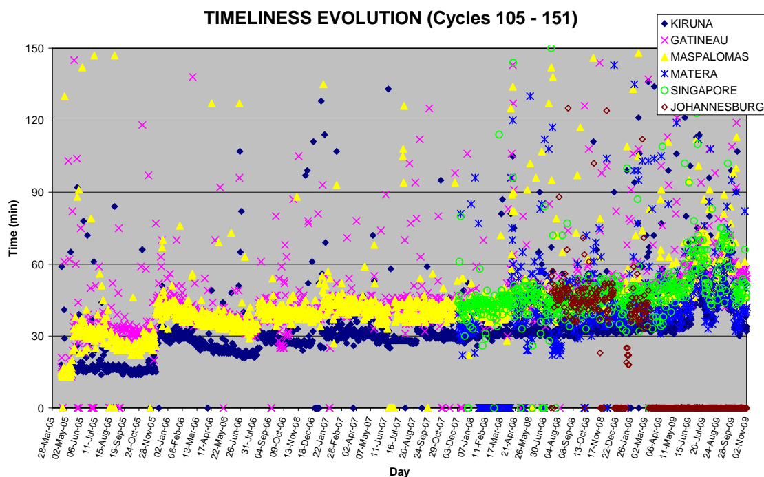
FIGURE 29 Timeliness evolution from 19 th April 2005 to 2 nd November 2009 for Kiruna, Gatineau, Maspalomas, Matera, Singapore and Johannesburg ground stations.
