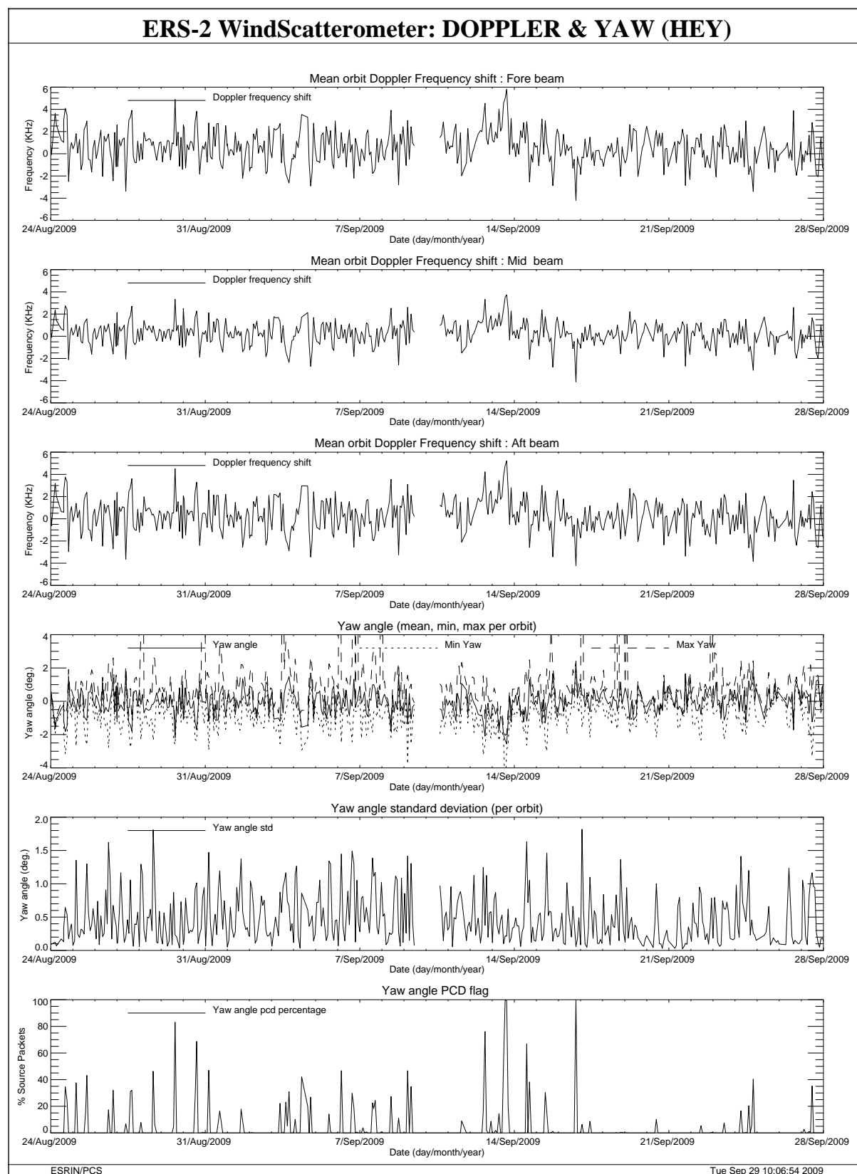
FIGURE 32 Doppler frequency shift and Yaw error angle evolution cycle 150.
