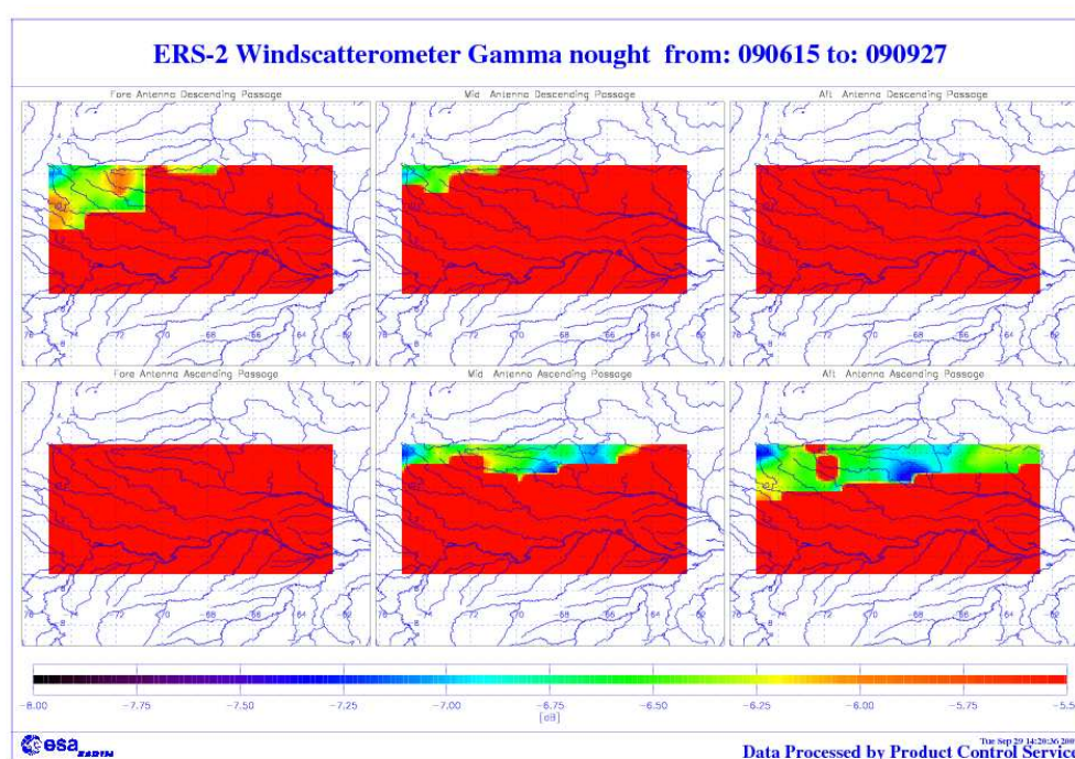
FIGURE 4 : ERS-2 Scatterometer: gamma nought over the Brazilian rain forest cycles 148, 149 and 150.
