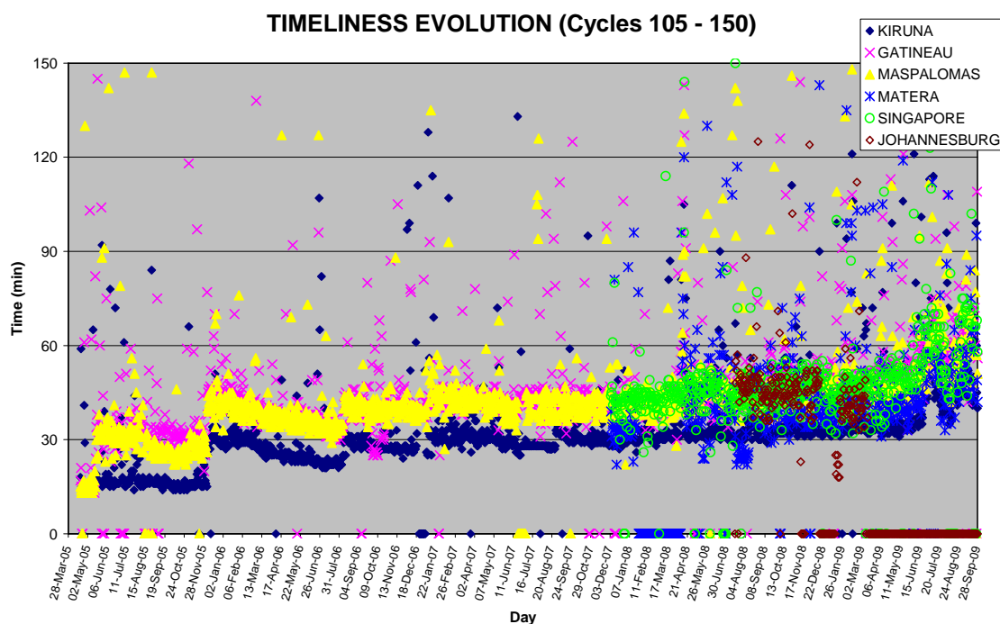
FIGURE 29 Timeliness evolution from 19 th April 2005 to 28 th September 2009 for Kiruna, Gatineau, Maspalomas, Matera, Singapore and Johannesburg ground stations.
