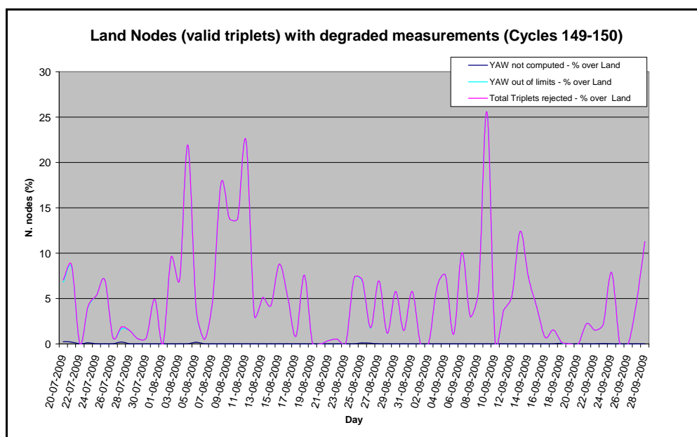
FIGURE 35 Statistics of degraded sigma nought triplets over Land.
