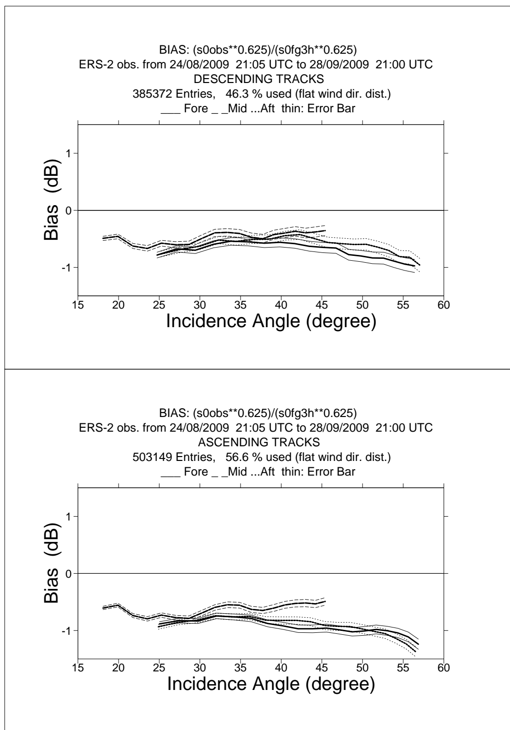
FIGURE 1 ERS-2 Scatterometer Ocean Calibration cycle 150. Ratio of \langle \sigma_0^{0.625} \rangle / \langle \text{CMOD4}(\text{First Guess})^{0.625} \rangle converted in dB for the fore beam (solid line), mid beam (dashed line) an aft beam (dotted line), as a function of incidence angle for descending and ascending tracks. The thin lines indicate the error bars on the estimated mean. First-guess winds are based on the in time closest (+3h, +6h, +9h, or +12h) T511 forecast field, and are bilinearly interpolated in space.
