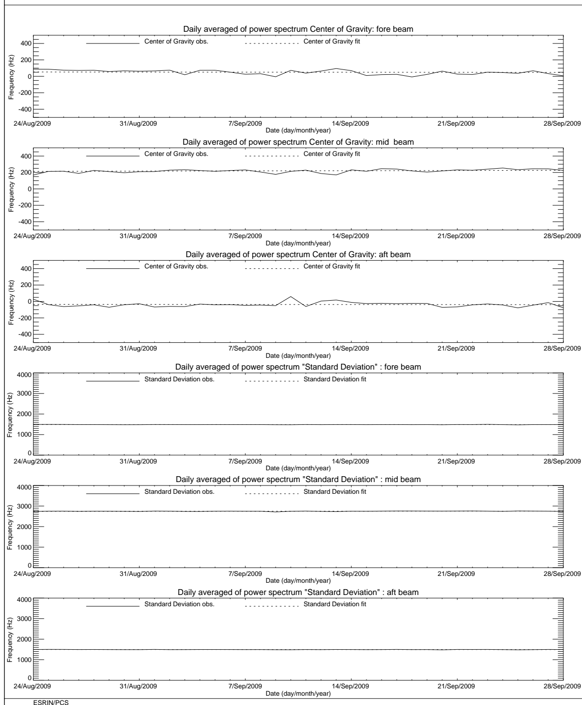
FIGURE 6 ERS-2 Scatterometer: Centre of Gravity and standard deviation of received power spectrum for cycle 150.
