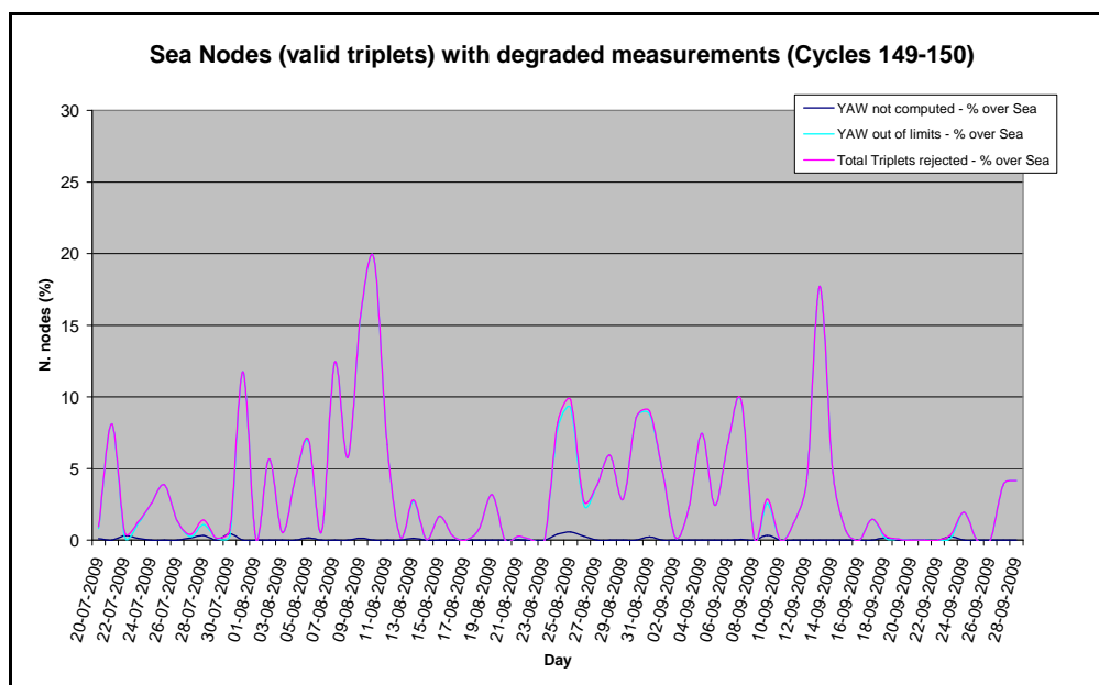
FIGURE 34 Statistics of degraded sigma nought triplets over Sea.
