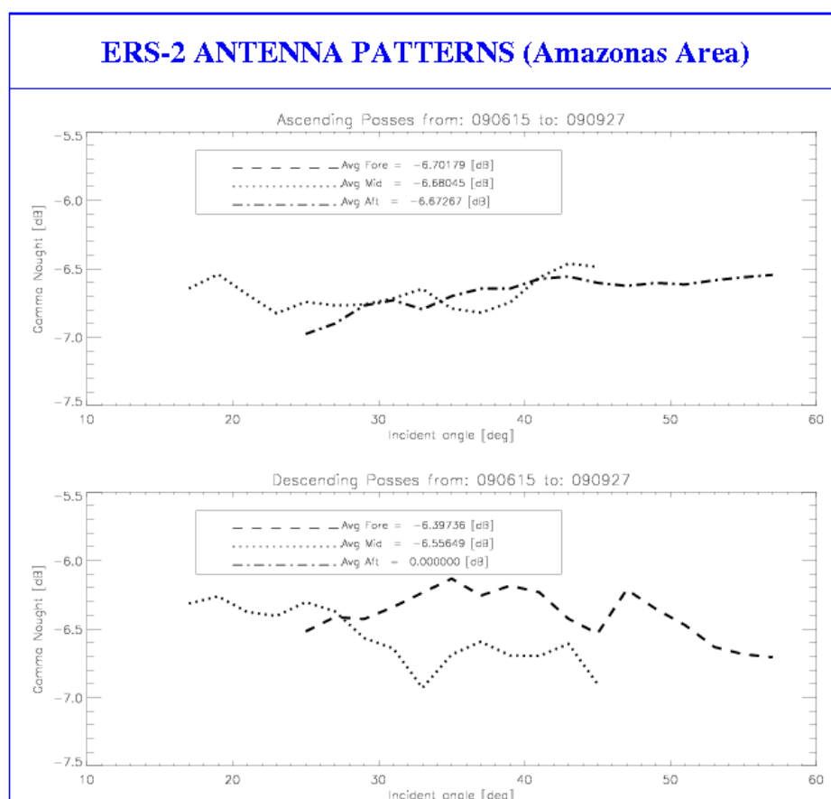
FIGURE 2 ERS-2 Scatterometer antenna pattern as function of the incidence angle: cycle 148, 149 and 150.
