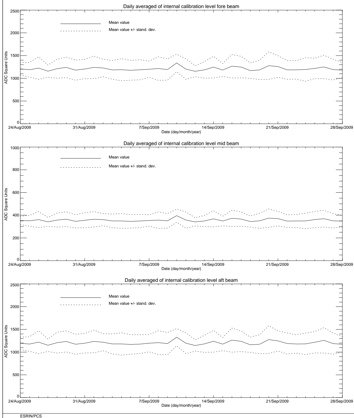
FIGURE 10 ERS-2 Scatterometer: power of internal calibration level cycle 150.
