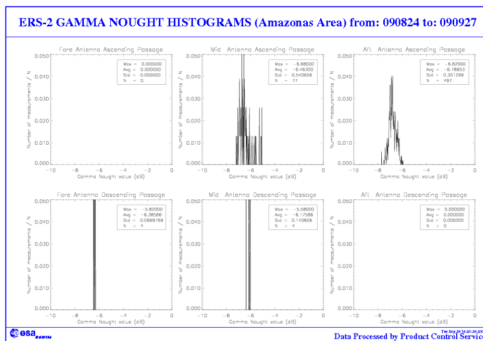
FIGURE 3 Gamma nought histograms over the Brazilian Rain Forest: cycle 150.
