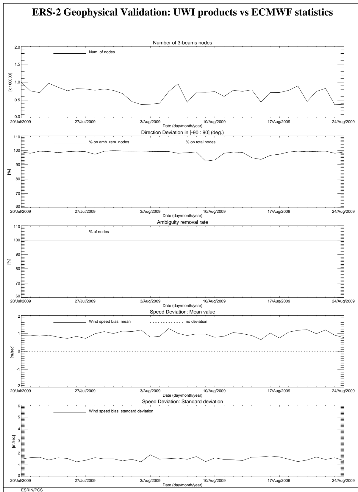
FIGURE 13 ERS-2 Scatterometer: wind products performance for cycle 149.
