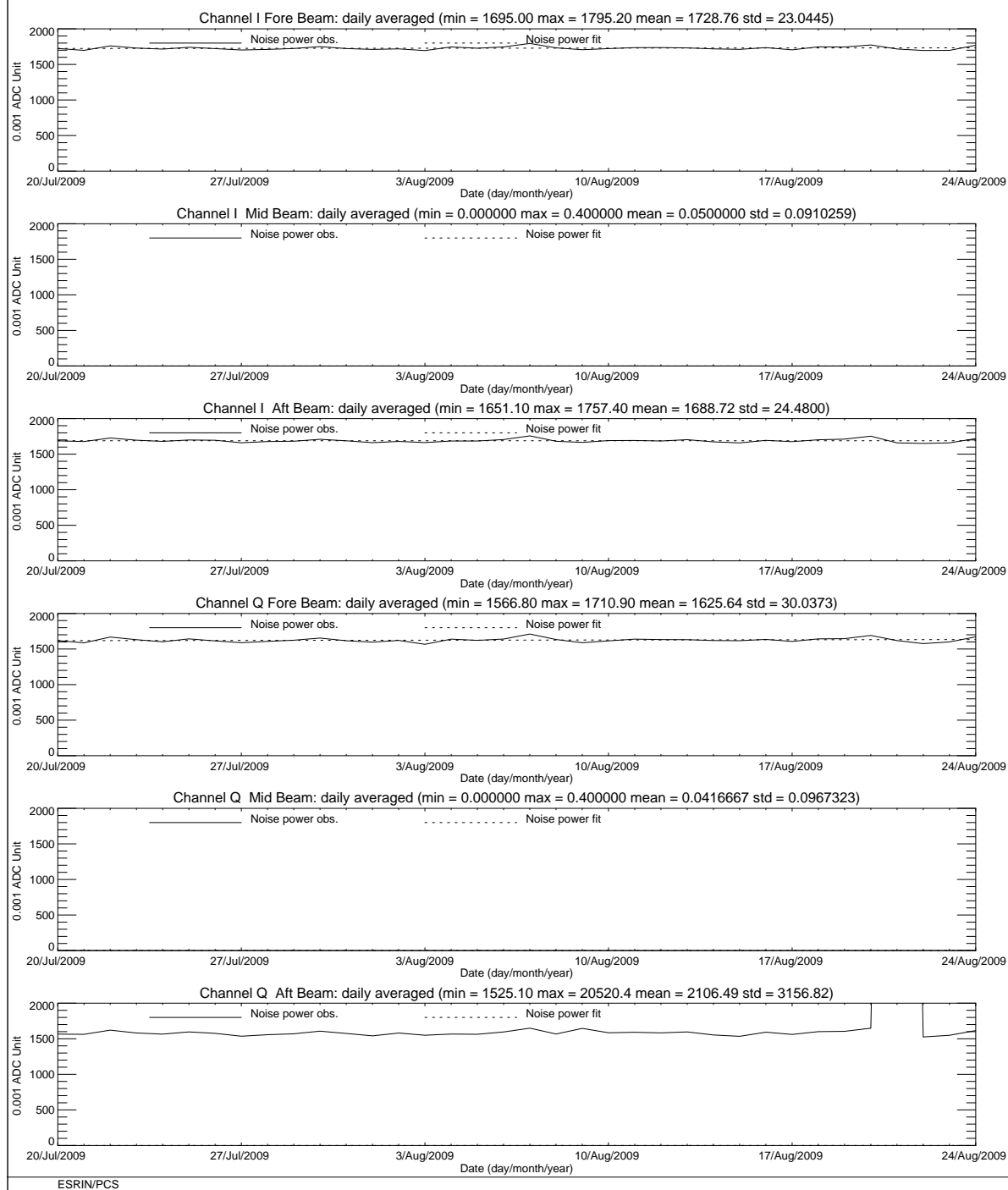
FIGURE 8 ERS-2 Scatterometer: noise power I and Q channel for cycle 149.
