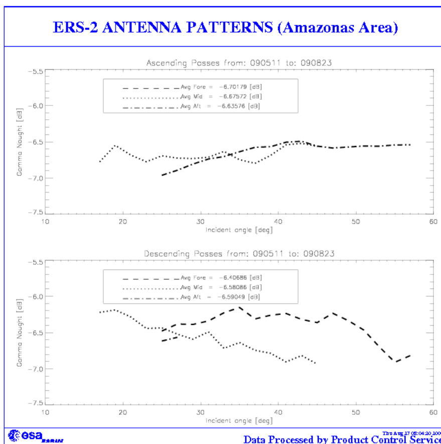
FIGURE 2 ERS-2 Scatterometer antenna pattern as function of the incidence angle: cycle 147, 148 and 149.
