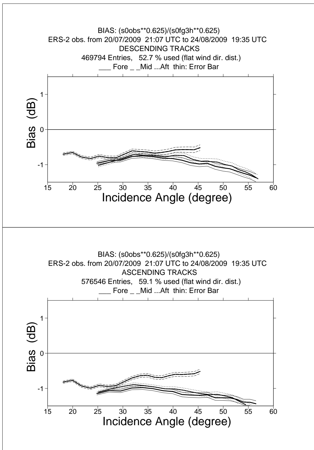
FIGURE 1 ERS-2 Scatterometer Ocean Calibration cycle 149. Ratio of \langle \sigma_0^{0.625} \rangle / \langle \text{CMOD4}(\text{First Guess})^{0.625} \rangle converted in dB for the fore beam (solid line), mid beam (dashed line) an aft beam (dotted line), as a function of incidence angle for descending and ascending tracks. The thin lines indicate the error bars on the estimated mean. First-guess winds are based on the in time closest (+3h, +6h, +9h, or +12h) T511 forecast field, and are bilinearly interpolated in space.
