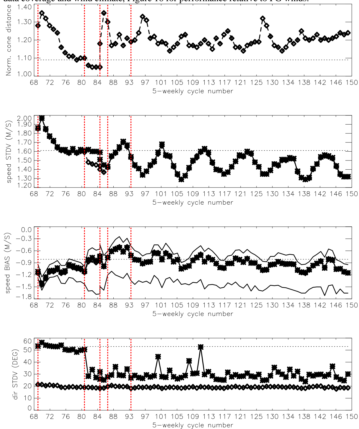
FIGURE 14 Evolution of the performance of the ERS-2 Scatterometer averaged over 5-weekly cycles from 12 December 2001 (cycle 69) to 24 August 2009 (end cycle 149) for the UWI product (solid, star) and de-aliased winds based on CMOD4 (dashed, diamond). Results are based on data that passed the UWI QC flags. For cycle 85 two values are plotted; the first value for the global set, the second one for the regional set. Dotted lines represent values for cycle 59 (5 December 2000 to 17 January 2001), i.e. the last stable cycle of the nominal period. From top to bottom panel are shown the normalized distance to the one (CMOD4 only) the standard deviation of the wind speed compared to FG winds, the corresponding bias (for UWI winds the extreme inter-node averages are shown as well), and the standard deviation of wind direction compared to FG.
