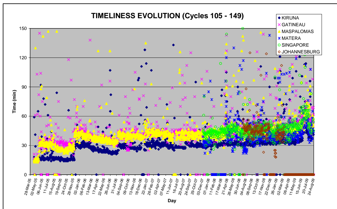
FIGURE 29 Timeliness evolution from 19 th April 2005 to 24 th August 2009 for Kiruna, Gatineau, Maspalomas, Matera, Singapore and Johannesburg ground stations.
