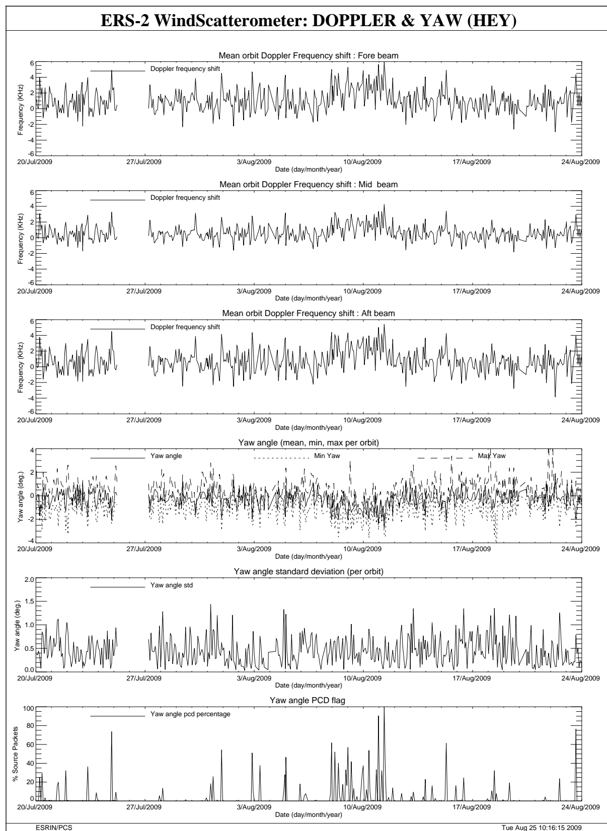
FIGURE 32 Doppler frequency shift and Yaw error angle evolution cycle 149.
