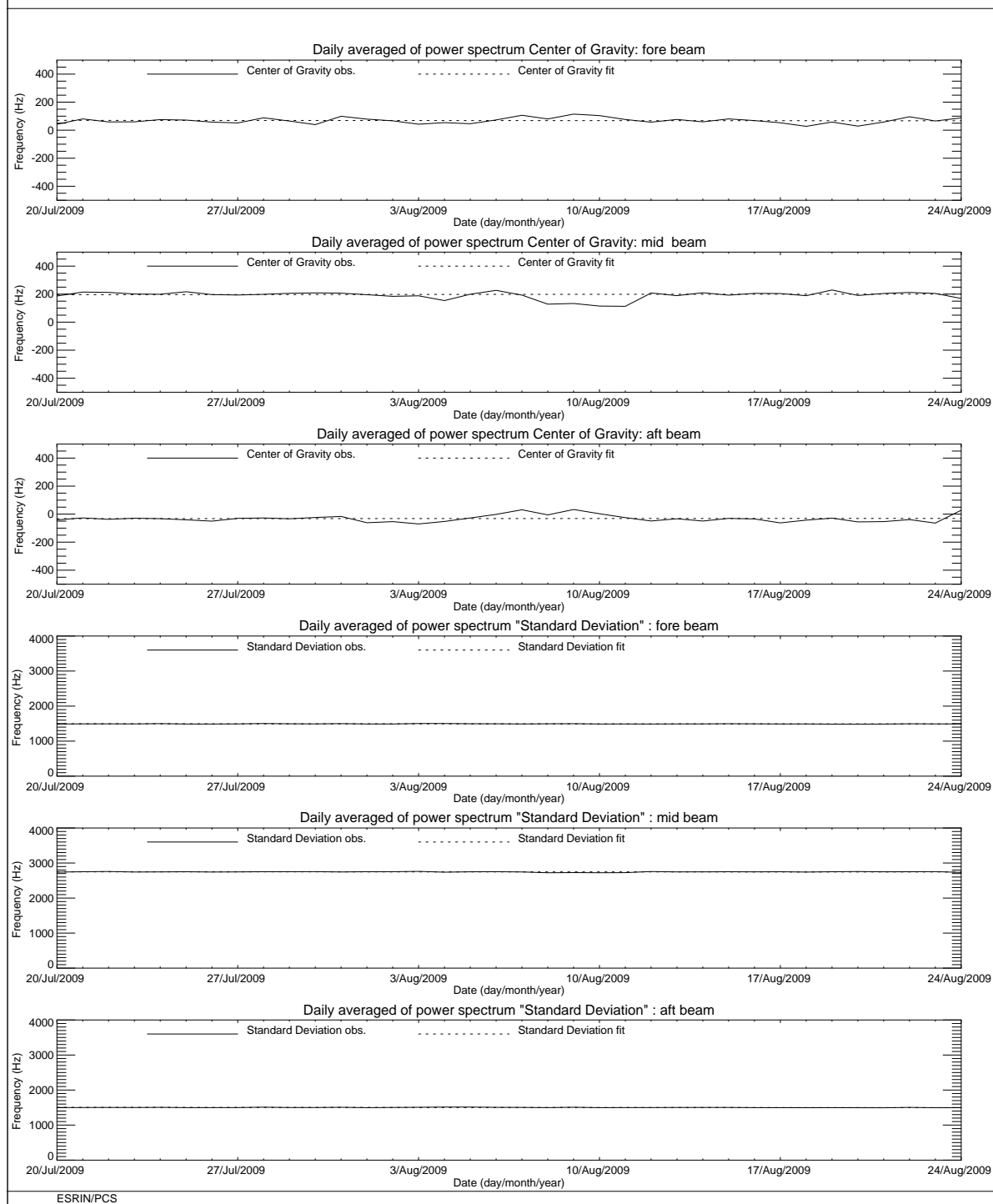
FIGURE 6 ERS-2 Scatterometer: Centre of Gravity and standard deviation of received power spectrum for cycle 149.
