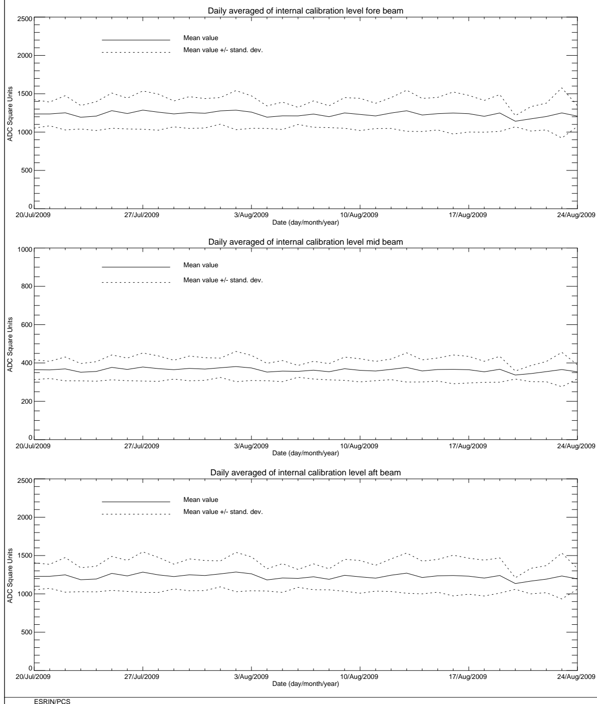
FIGURE 10 ERS-2 Scatterometer: power of internal calibration level cycle 149.
