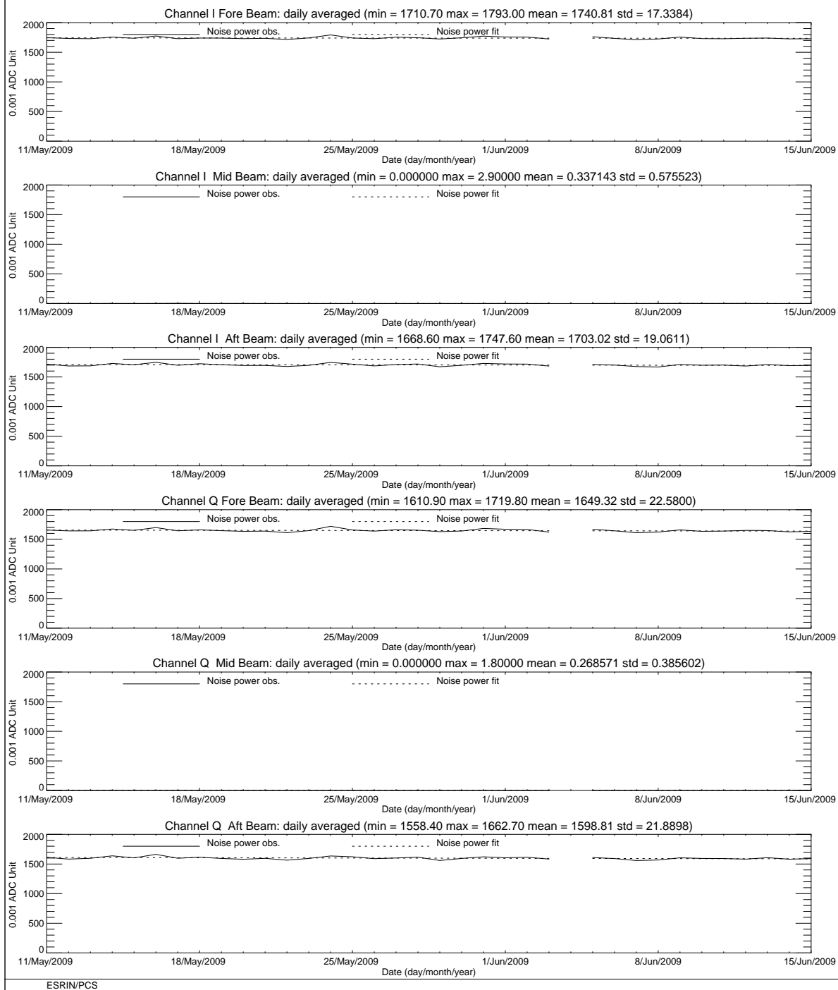
FIGURE 5 ERS-2 Scatterometer: noise power I and Q channel for cycle 147.
