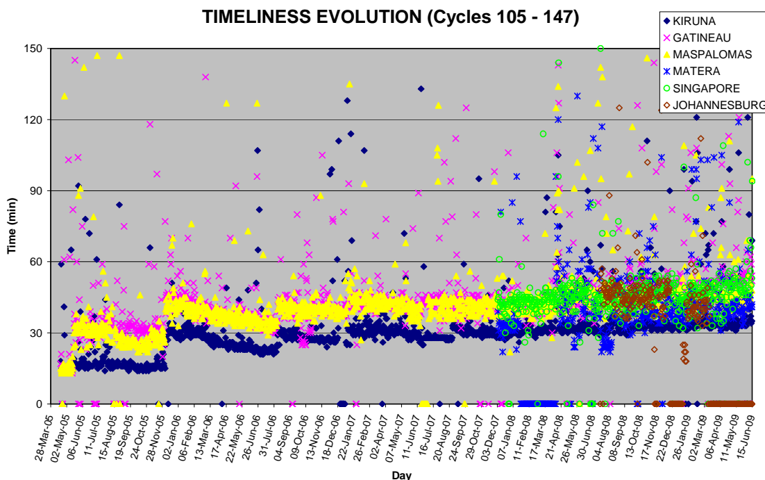
FIGURE 26 Timeliness evolution from 19 th April 2005 to 15 th June 2009 for Kiruna, Gatineau, Maspalomas, Matera, Singapore and Johannesburg ground stations.
