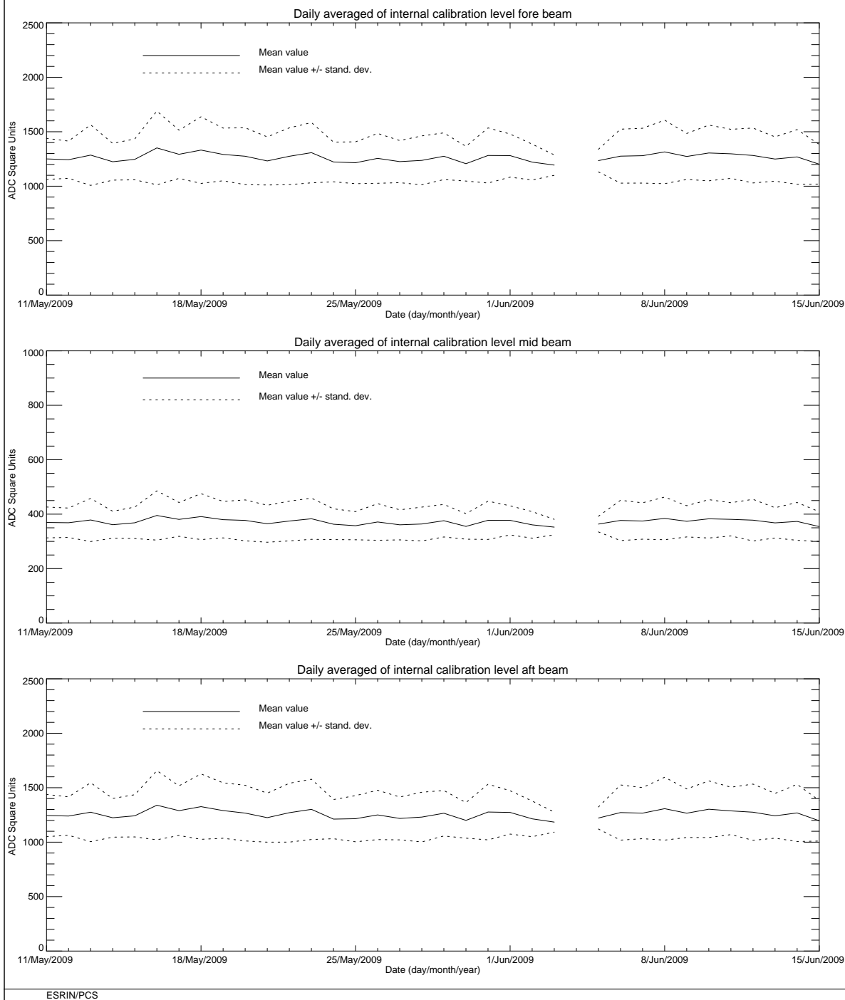
FIGURE 7 ERS-2 Scatterometer: power of internal calibration level cycle 147.
