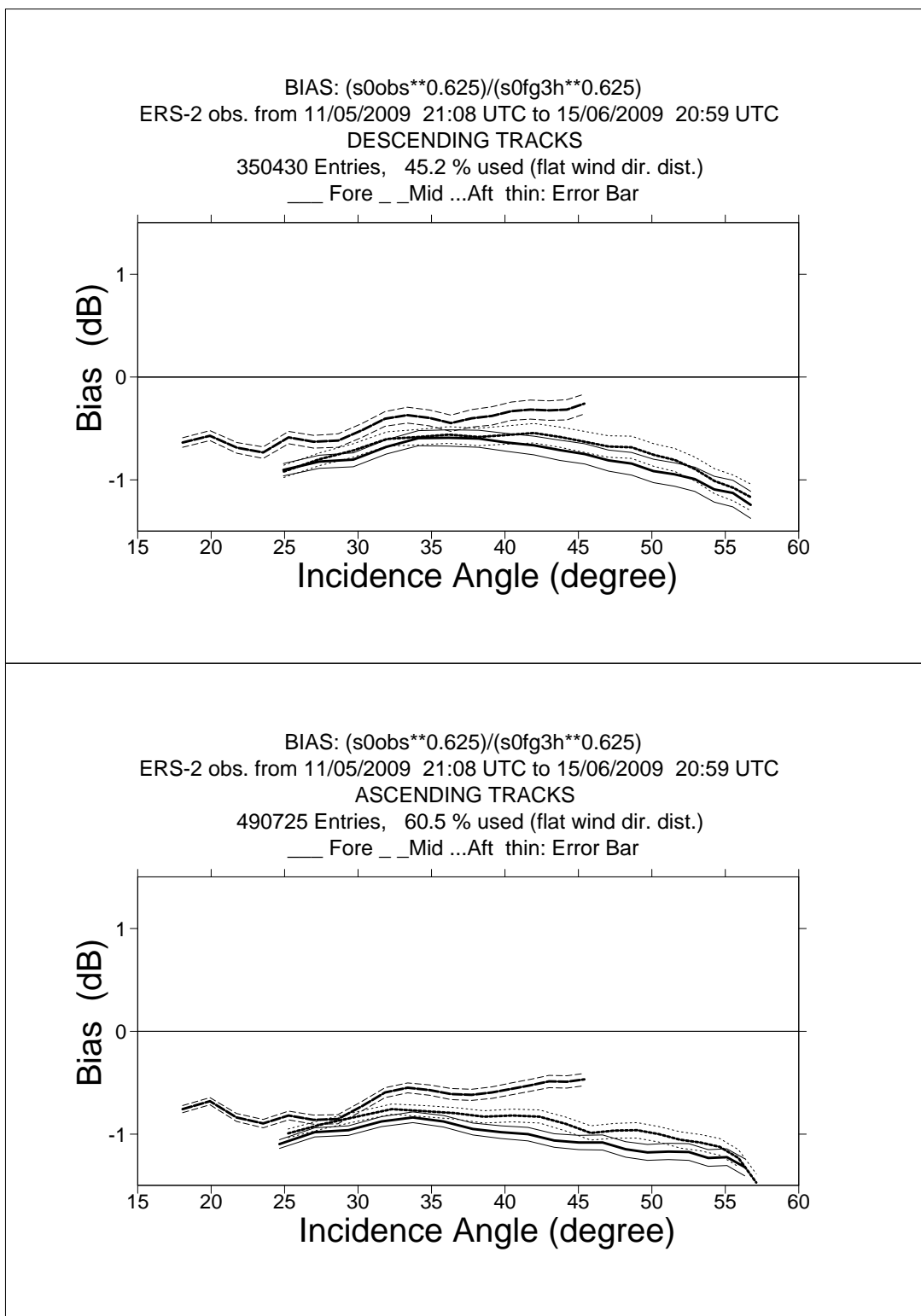
FIGURE 1 ERS-2 Scatterometer Ocean Calibration cycle 147. Ratio of \langle \sigma_0^{0.625} \rangle / \langle \text{CMOD4}(\text{First Guess})^{0.625} \rangle converted in dB for the fore beam (solid line), mid beam (dashed line) an aft beam (dotted line), as a function of incidence angle for descending and ascending tracks. The thin lines indicate the error bars on the estimated mean. First-guess winds are based on the in time closest (+3h, +6h, +9h, or +12h) T511 forecast field, and are bilinearly interpolated in space.
