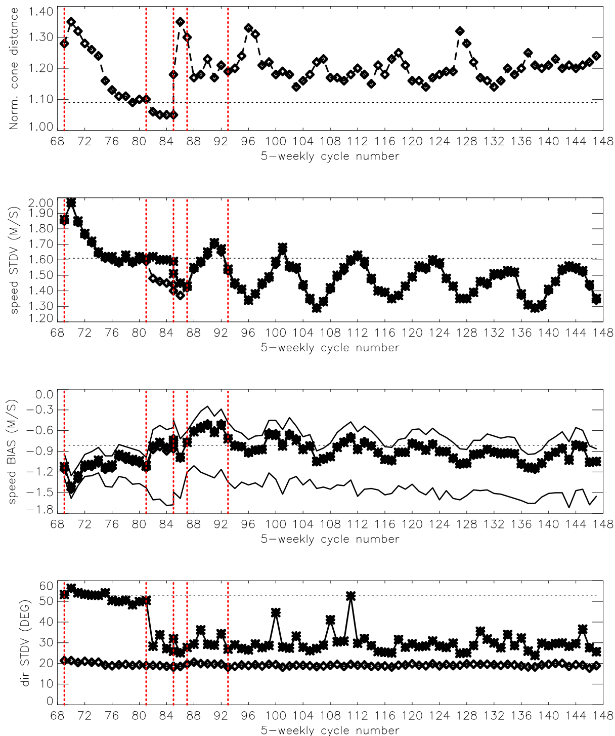
FIGURE 11 Evolution of the performance of the ERS-2 Scatterometer averaged over 5-weekly cycles from 12 December 2001 (cycle 69) to 15 June 2009 (end cycle 147) for the UWI product (solid, star) and de-aliased winds based on CMOD4 (dashed, diamond). Results are based on data that passed the UWI QC flags. For cycle 85 two values are plotted; the first value for the global set, the second one for the regional set. Dotted lines represent values for cycle 59 (5 December 2000 to 17 January 2001), i.e. the last stable cycle of the nominal period. From top to bottom panel are shown the normalized distance to the one (CMOD4 only) the standard deviation of the wind speed compared to FG winds, the corresponding bias (for UWI winds the extreme inter-node averages are shown as well), and the standard deviation of wind direction compared to FG.
