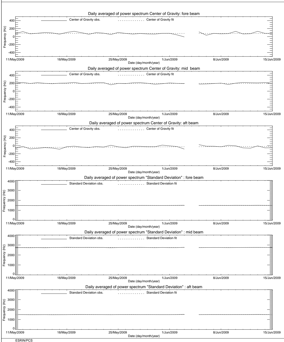
FIGURE 3 ERS-2 Scatterometer: Centre of Gravity and standard deviation of received power spectrum for cycle 147.
