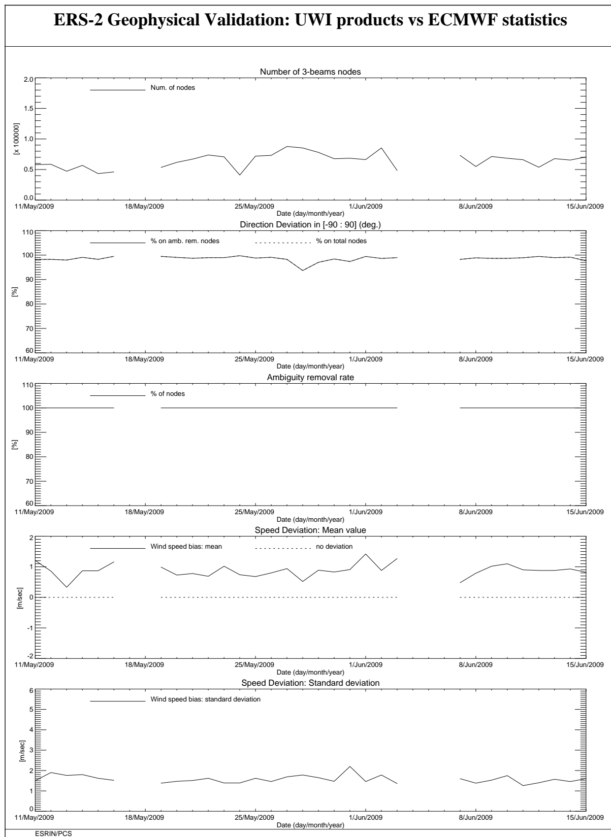
FIGURE 10 ERS-2 Scatterometer: wind products performance for cycle 147.
