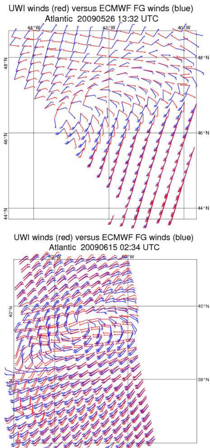
FIGURE 20 Comparison between UWI winds (in red) and ECMWF FG winds (in blue) for a case in the North Atlantic on 26 May 2009 (top panel) and on 15 June 2009 (lower panel).
