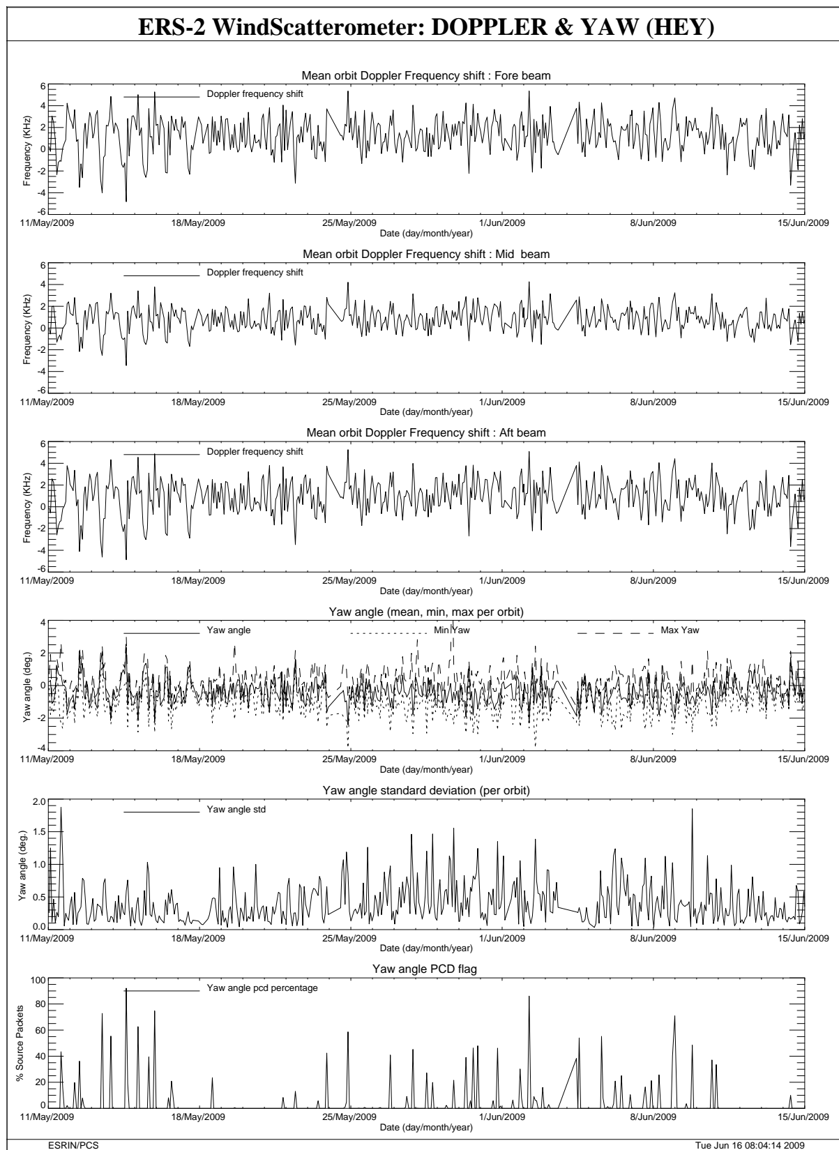
FIGURE 29 Doppler frequency shift and Yaw error angle evolution cycle 147.
