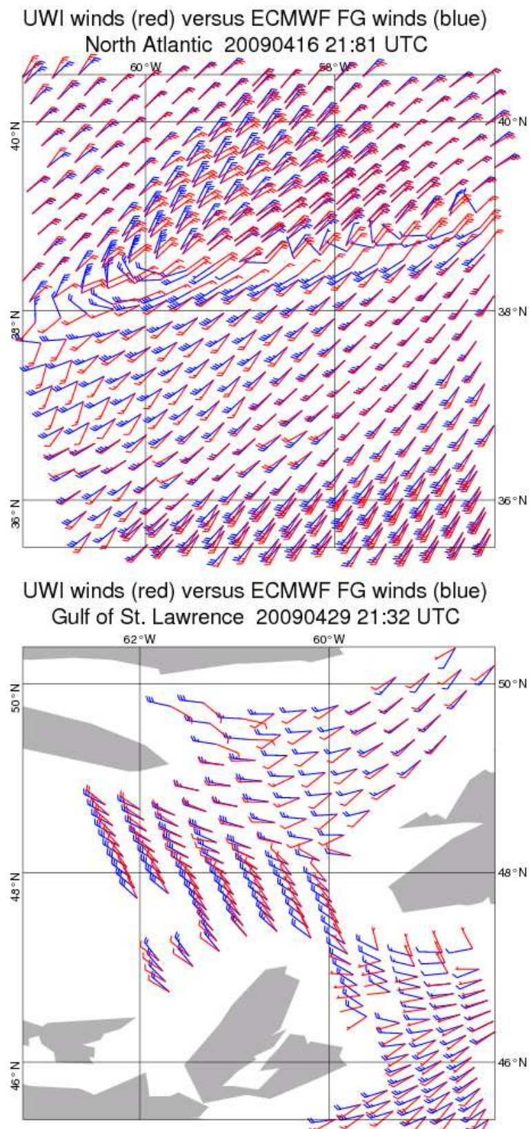
FIGURE 20 Comparison between UWI winds (in red) and ECMWF FG winds (in blue) for a case in the North Atlantic on 16 April 2009 (top panel) and a case for the Gulf of St. Lawrence on 29 April 2009 (lower panel).
