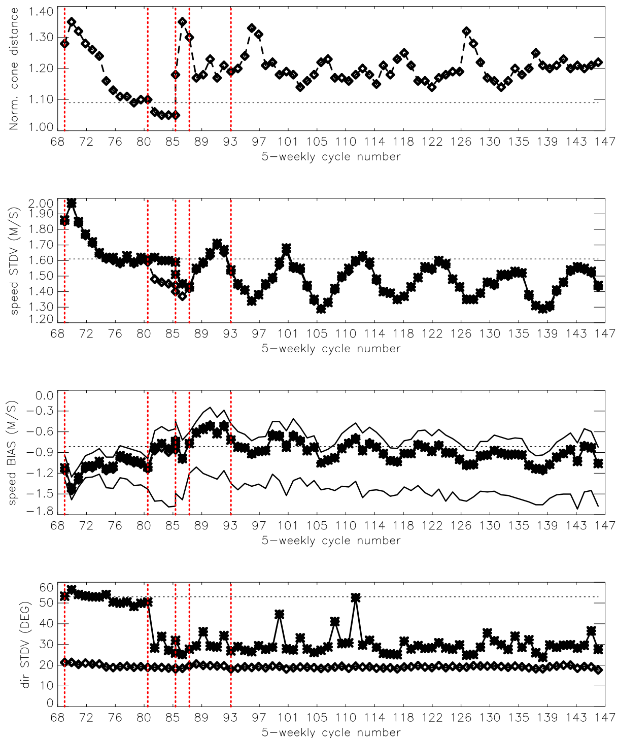
FIGURE 11 Evolution of the performance of the ERS-2 Scatterometer averaged over 5-weekly cycles from 12 December 2001 (cycle 69) to 11 May 2009 (end cycle 146) for the UWI product (solid, star) and de-aliased winds based on CMOD4 (dashed, diamond). Results are based on data that passed the UWI QC flags. For cycle 85 two values are plotted; the first value for the global set, the second one for the regional set. Dotted lines represent values for cycle 59 (5 December 2000 to 17 January 2001), i.e. the last stable cycle of the nominal period. From top to bottom panel are shown the normalized distance to the one (CMOD4 only) the standard deviation of the wind speed compared to FG winds, the corresponding bias (for UWI winds the extreme inter-node averages are shown as well), and the standard deviation of wind direction compared to FG.
