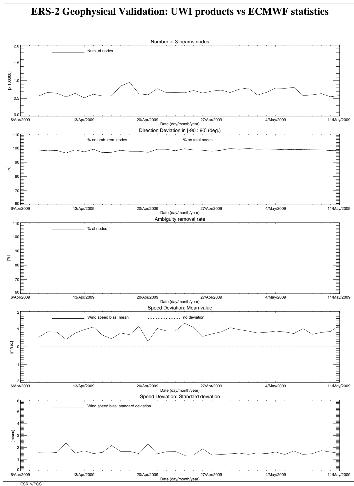
FIGURE 10 ERS-2 Scatterometer: wind products performance for cycle 146.
