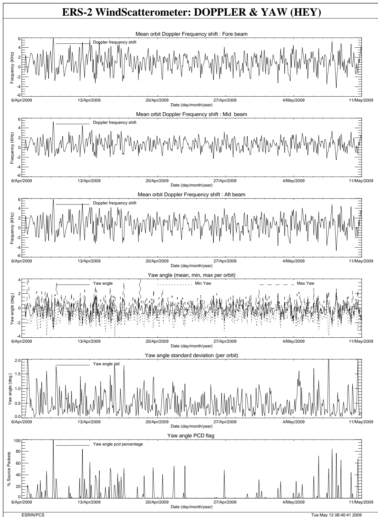
FIGURE 29 Doppler frequency shift and Yaw error angle evolution cycle 146.
