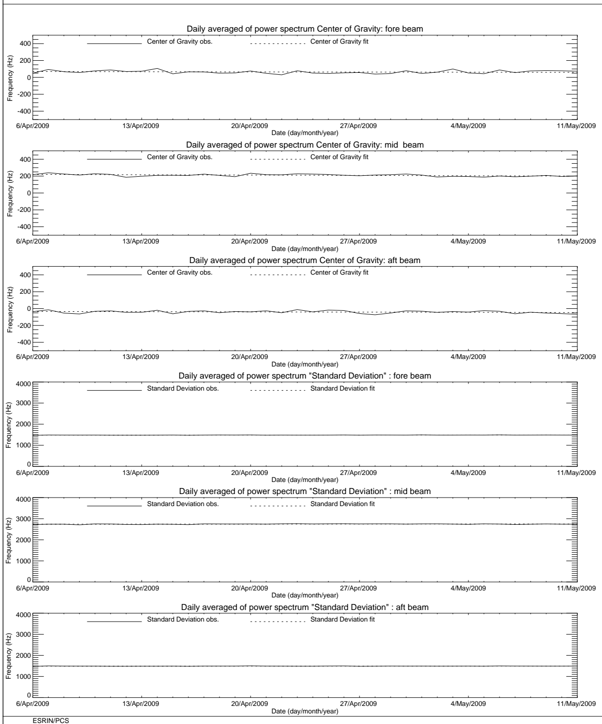
FIGURE 3 ERS-2 Scatterometer: Centre of Gravity and standard deviation of received power spectrum for cycle 146.
