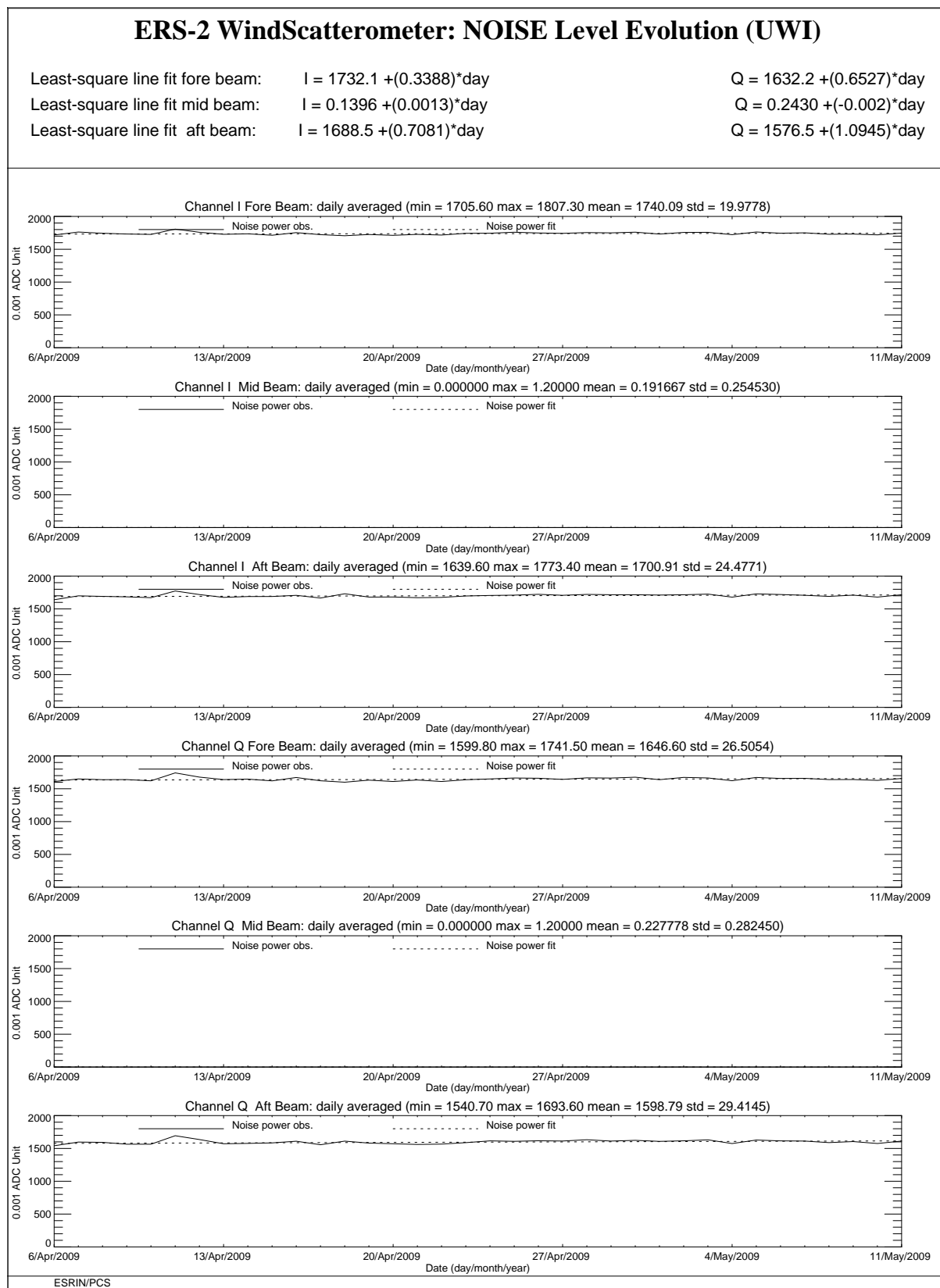
FIGURE 5 ERS-2 Scatterometer: noise power I and Q channel for cycle 146.
