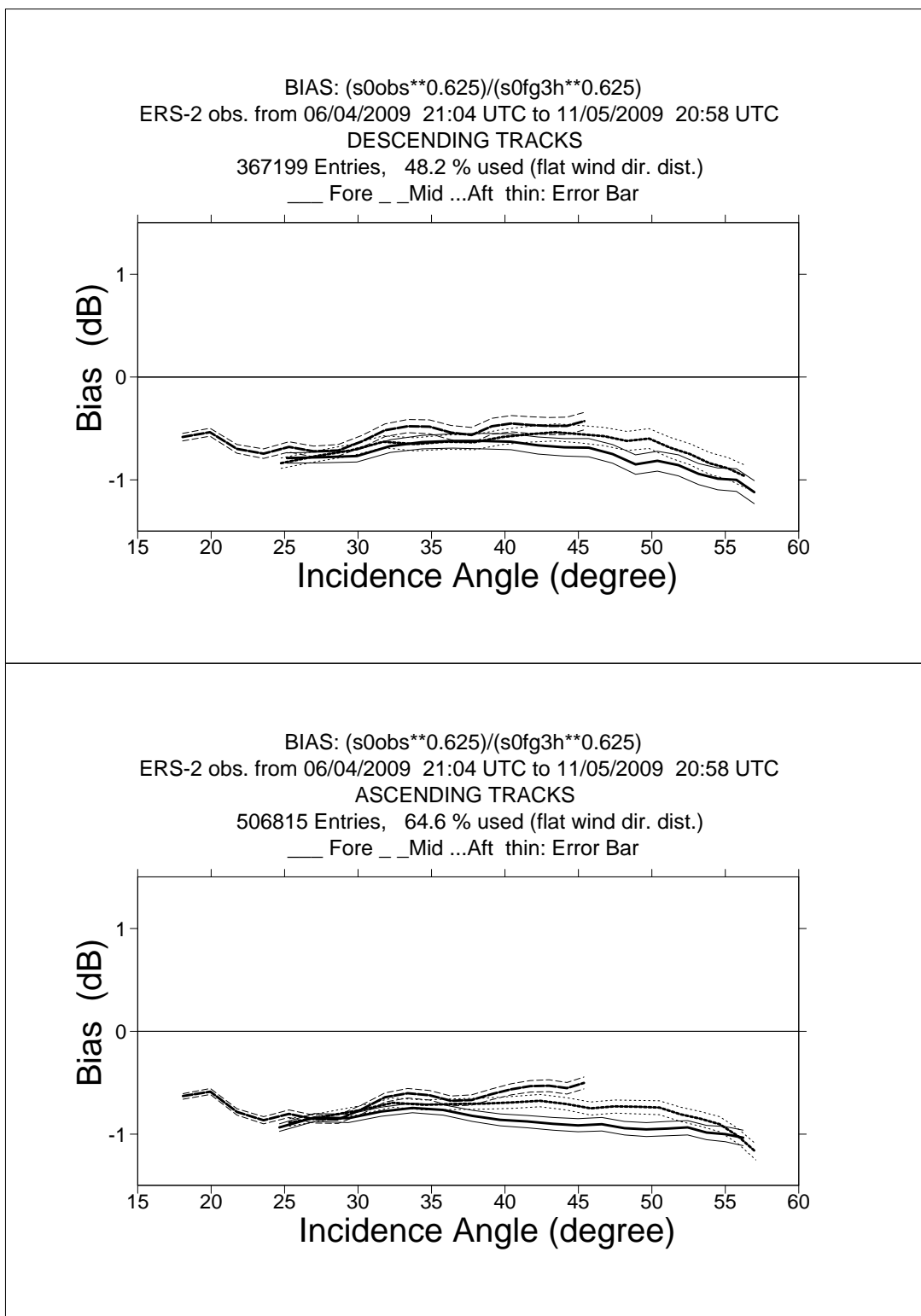
FIGURE 1 ERS-2 Scatterometer Ocean Calibration cycle 146. Ratio of \langle \sigma_0^{0.625} \rangle / \langle \text{CMOD4}(\text{First Guess})^{0.625} \rangle converted in dB for the fore beam (solid line), mid beam (dashed line) an aft beam (dotted line), as a function of incidence angle for descending and ascending tracks. The thin lines indicate the error bars on the estimated mean. First-guess winds are based on the in time closest (+3h, +6h, +9h, or +12h) T511 forecast field, and are bilinearly interpolated in space.
