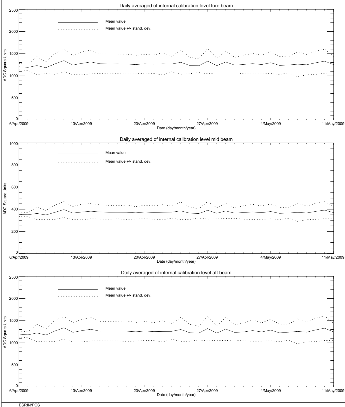
FIGURE 7 ERS-2 Scatterometer: power of internal calibration level cycle 146.
