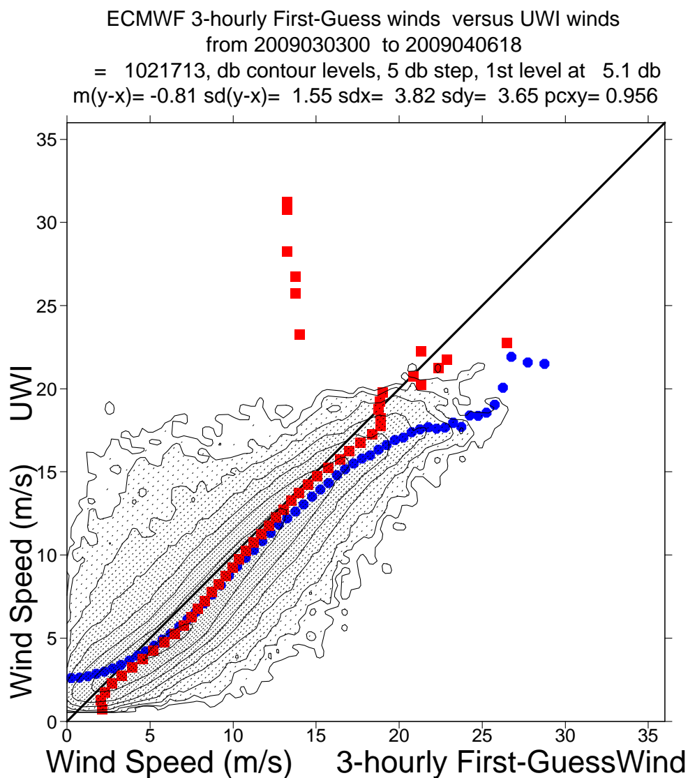
FIGURE 21 Two-dimensional histogram of first guess and UWI wind speeds, for the data kept by the UWI flags, and QC based on the ECMWF ice and land and sea-ice mask. Circles denote the mean values in the y-direction and squares those in the x-direction.
