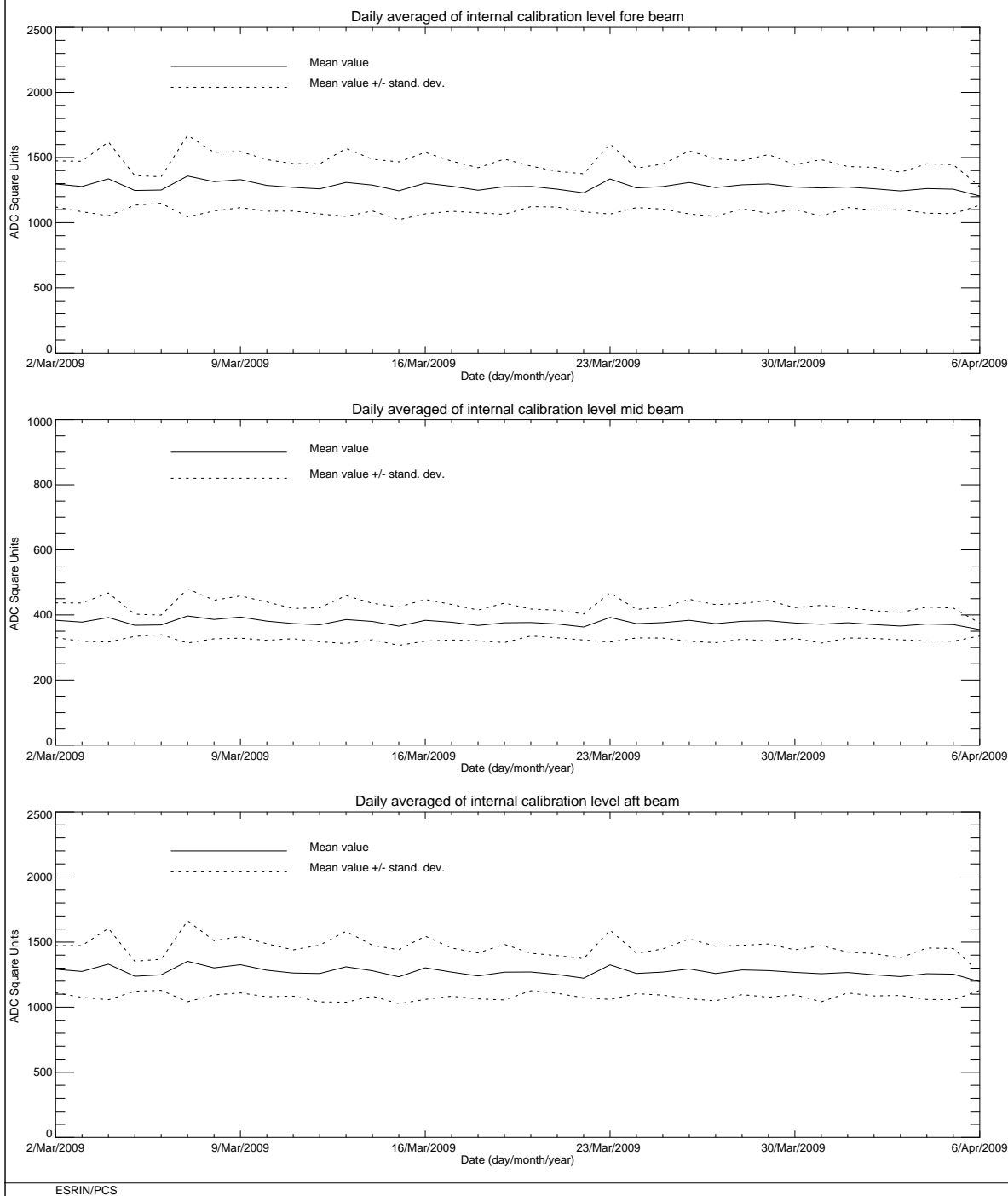
FIGURE 7 ERS-2 Scatterometer: power of internal calibration level cycle 145.
