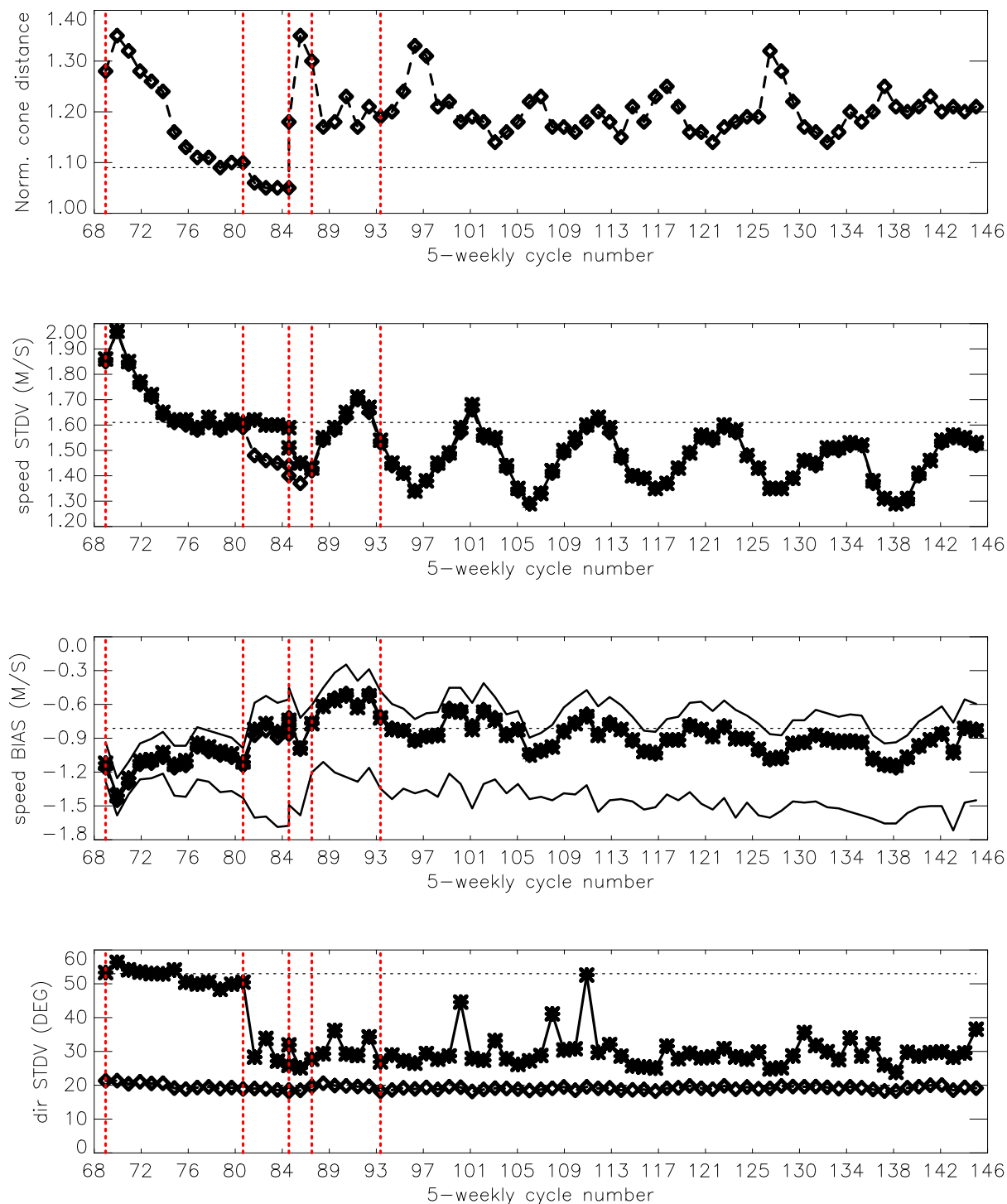
FIGURE 11 Evolution of the performance of the ERS-2 Scatterometer averaged over 5-weekly cycles from 12 December 2001 (cycle 69) to 6 April 2009 (end cycle 145) for the UWI product (solid, star) and de-aliased winds based on CMOD4 (dashed, diamond). Results are based on data that passed the UWI QC flags. For cycle 85 two values are plotted; the first value for the global set, the second one for the regional set. Dotted lines represent values for cycle 59 (5 December 2000 to 17 January 2001), i.e. the last stable cycle of the nominal period. From top to bottom panel are shown the normalized distance to the one (CMOD4 only) the standard deviation of the wind speed compared to FG winds, the corresponding bias (for UWI winds the extreme inter-node averages are shown as well), and the standard deviation of wind direction compared to FG.
