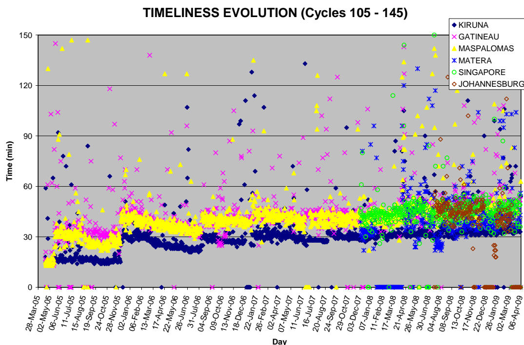
FIGURE 26 Timeliness evolution from 19 th April 2005 to 6 th April 2009 for Kiruna, Gatineau, Maspalomas, Matera, Singapore and Johannesburg ground stations.
