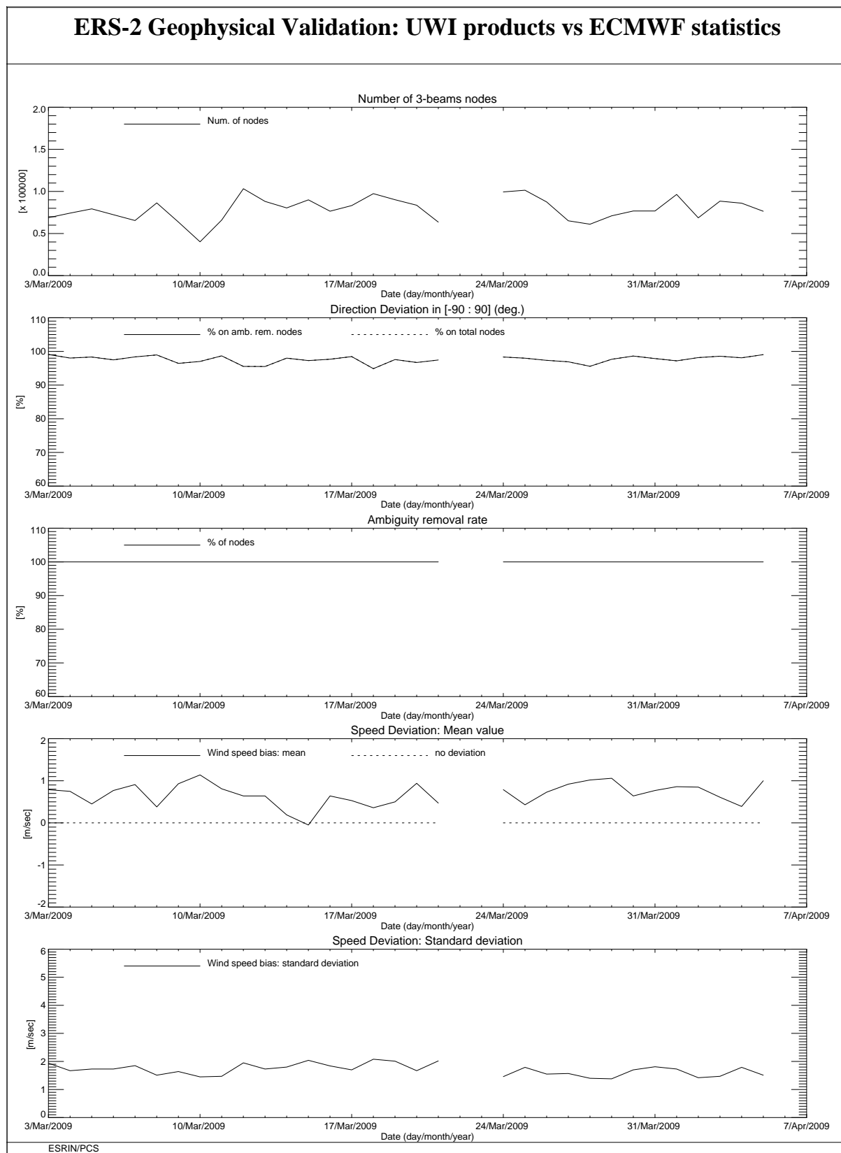
FIGURE 10 ERS-2 Scatterometer: wind products performance for cycle 145.
