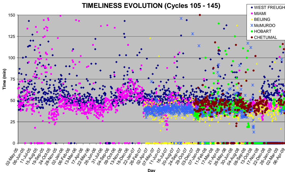
FIGURE 27 : Timeliness evolution from 19 th April 2005 to 6 th April 2009 for West Freugh, Miami, Beijing, McMurdo, Hobart and Chetumal ground stations.
