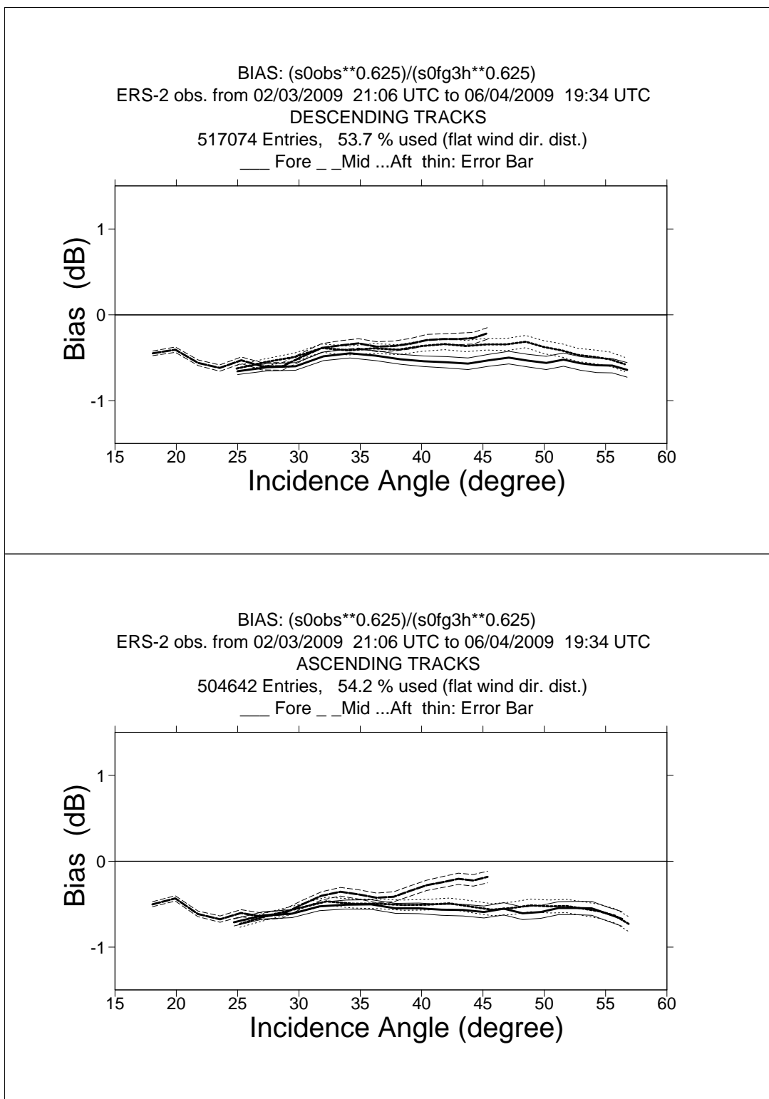
FIGURE 1 ERS-2 Scatterometer Ocean Calibration cycle 145. Ratio of \langle \sigma_0^{0.625} \rangle / \langle \text{CMOD4}(\text{First Guess})^{0.625} \rangle converted in dB for the fore beam (solid line), mid beam (dashed line) an aft beam (dotted line), as a function of incidence angle for descending and ascending tracks. The thin lines indicate the error bars on the estimated mean. First-guess winds are based on the in time closest (+3h, +6h, +9h, or +12h) T511 forecast field, and are bilinearly interpolated in space.
