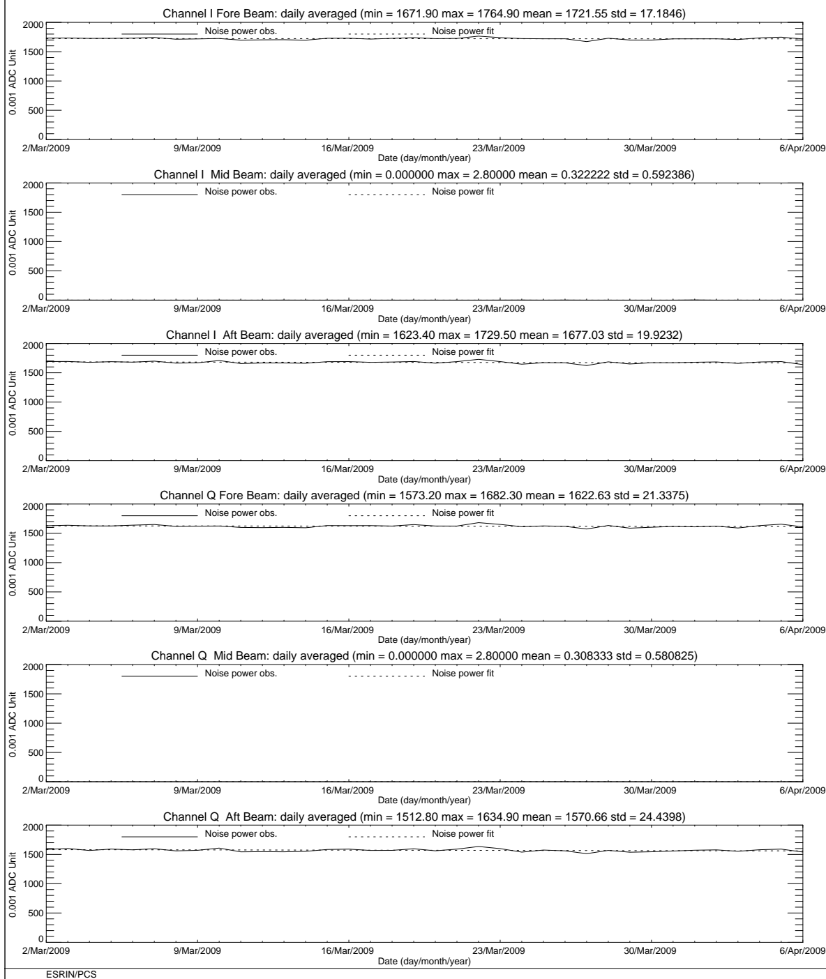
FIGURE 5 ERS-2 Scatterometer: noise power I and Q channel for cycle 145.
