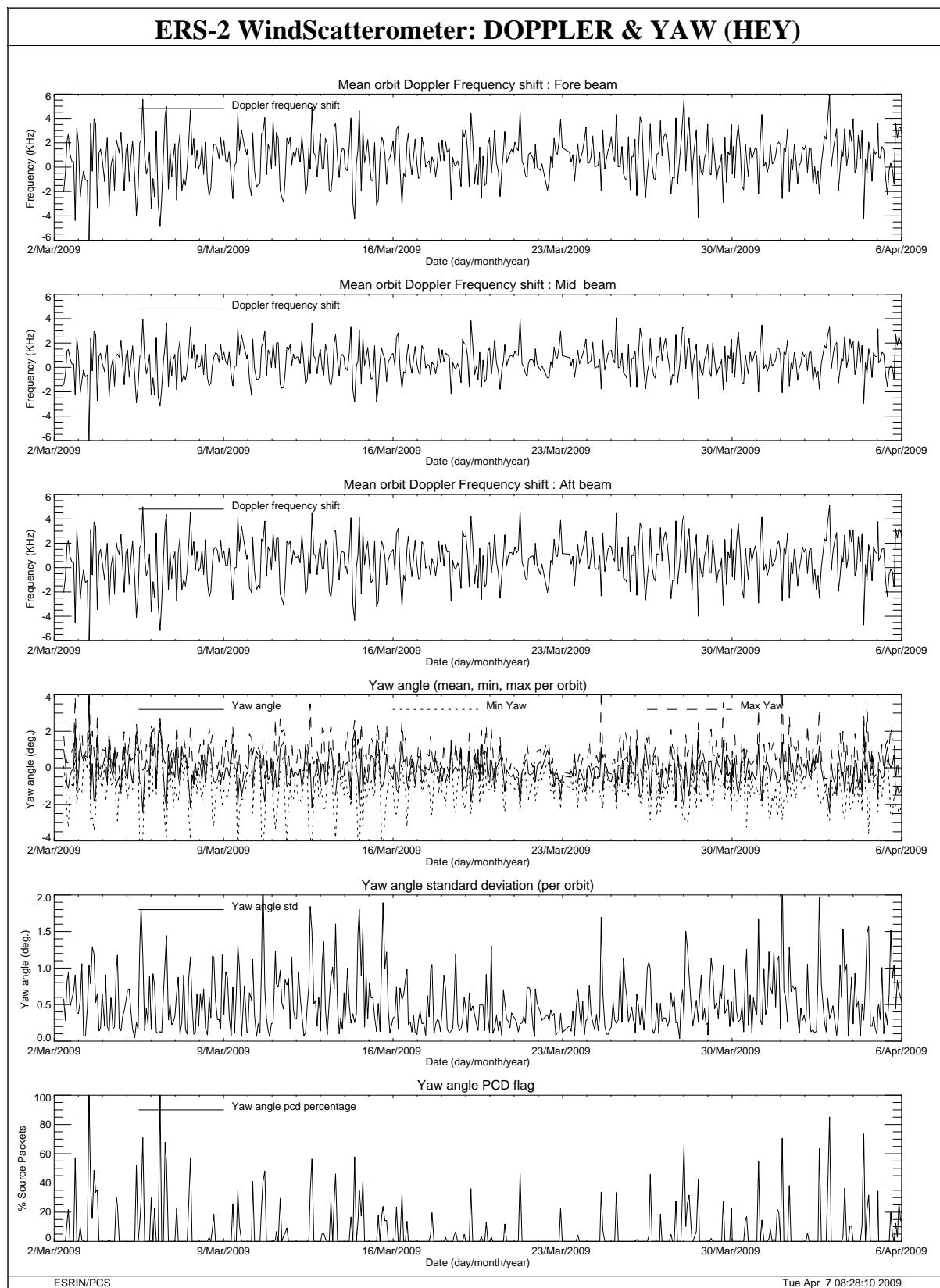
FIGURE 29 Doppler frequency shift and Yaw error angle evolution cycle 145.
