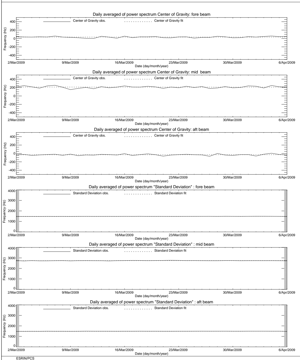
FIGURE 3 ERS-2 Scatterometer: Centre of Gravity and standard deviation of received power spectrum for cycle 145.
