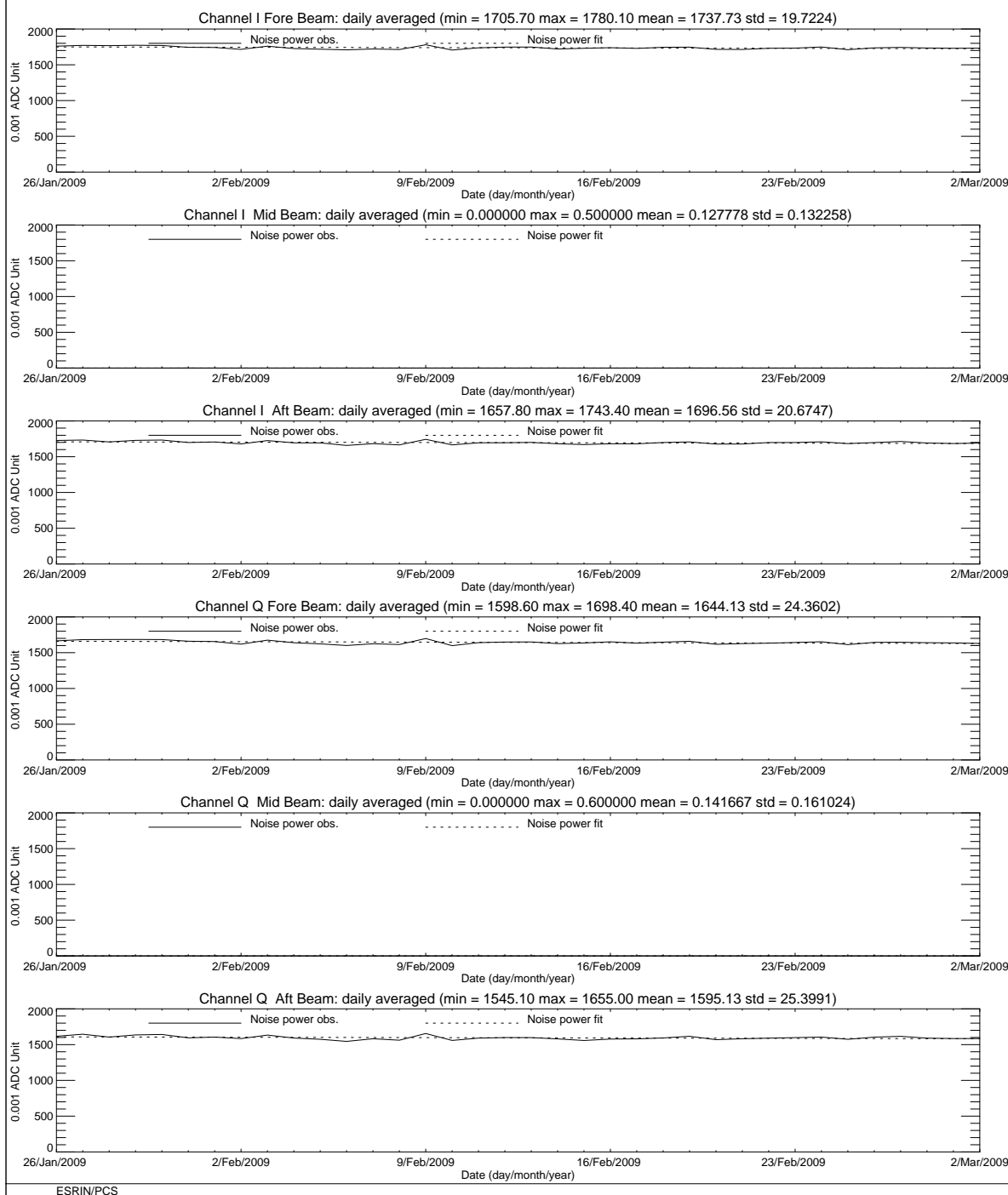
FIGURE 5 ERS-2 Scatterometer: noise power I and Q channel for cycle 144.
