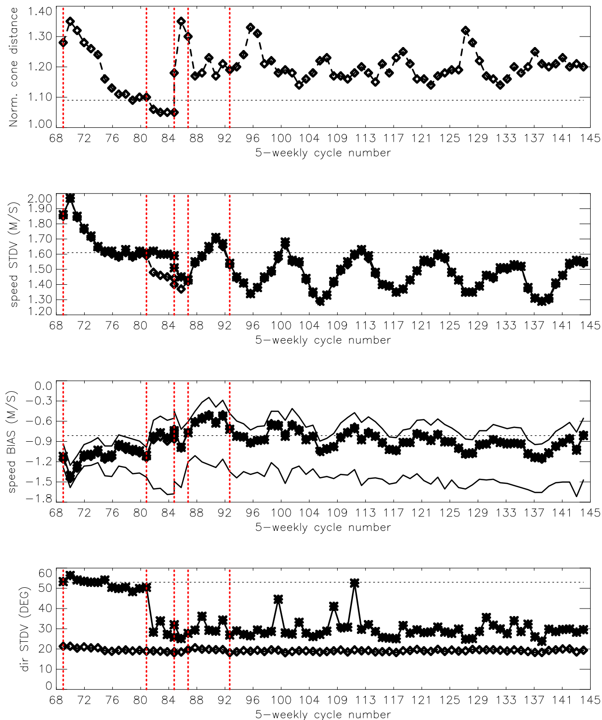
FIGURE 11 Evolution of the performance of the ERS-2 Scatterometer averaged over 5-weekly cycles from 12 December 2001 (cycle 69) to 2 March 2009 (end cycle 144) for the UWI product (solid, star) and de-aliased winds based on CMOD4 (dashed, diamond). Results are based on data that passed the UWI QC flags. For cycle 85 two values are plotted; the first value for the global set, the second one for the regional set. Dotted lines represent values for cycle 59 (5 December 2000 to 17 January 2001), i.e. the last stable cycle of the nominal period. From top to bottom panel are shown the normalized distance to the one (CMOD4 only) the standard deviation of the wind speed compared to FG winds, the corresponding bias (for UWI winds the extreme inter-node averages are shown as well), and the standard deviation of wind direction compared to FG.
