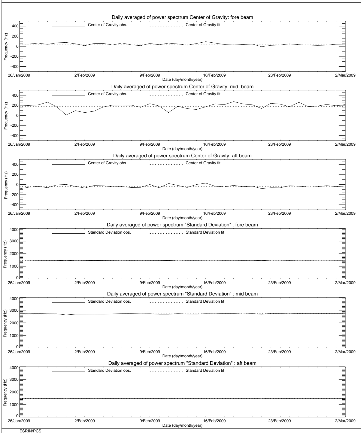
FIGURE 3 ERS-2 Scatterometer: Centre of Gravity and standard deviation of received power spectrum for cycle 144.
