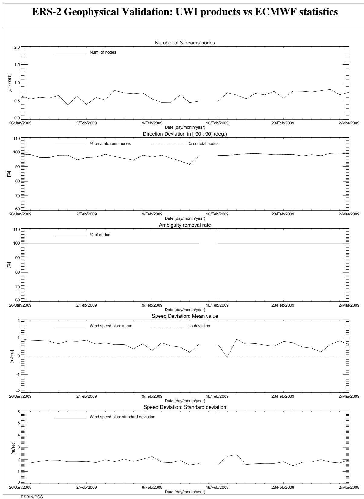
FIGURE 10 ERS-2 Scatterometer: wind products performance for cycle 144.
