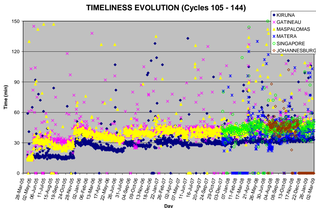
FIGURE 26 Timeliness evolution from 19 th April 2005 to 2 nd March 2009 for Kiruna, Gatineau, Maspalomas, Matera, Singapore and Johannesburg ground stations.
