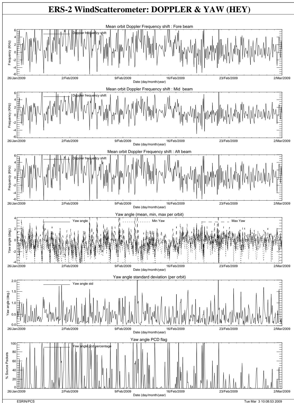
FIGURE 29 Doppler frequency shift and Yaw error angle evolution cycle 144.
