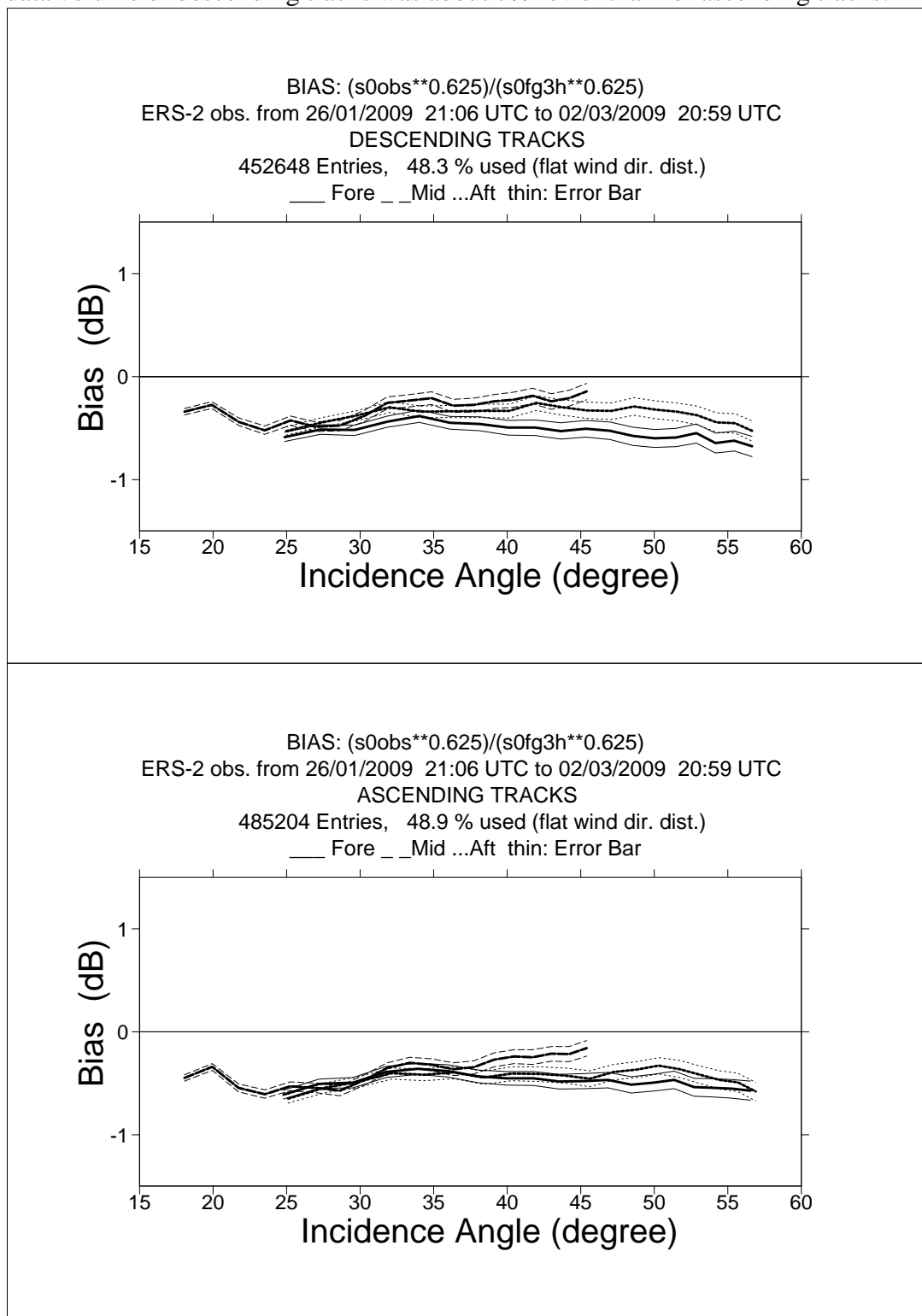
FIGURE 1 ERS-2 Scatterometer Ocean Calibration cycle 144. Ratio of \langle \sigma_0^{0.625} \rangle / \langle CMOD4(\text{First Guess})^{0.625} \rangle converted in dB for the fore beam (solid line), mid beam (dashed line) an aft beam (dotted line), as a function of incidence angle for descending and ascending tracks. The thin lines indicate the error bars on the estimated mean. First-guess winds are based on the in time closest (+3h, +6h, +9h, or +12h) T511 forecast field, and are bilinearly interpolated in space.
