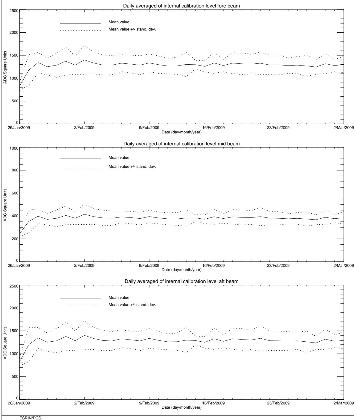
FIGURE 7 ERS-2 Scatterometer: power of internal calibration level cycle 144.
